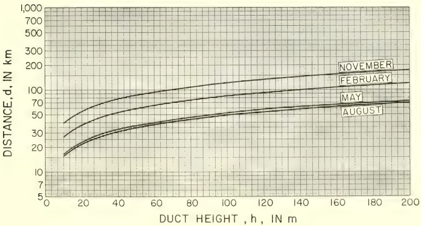
FIGURE 4.45. Shadow zone half-lengths for mean ducting conditions at Washington, D.C.
