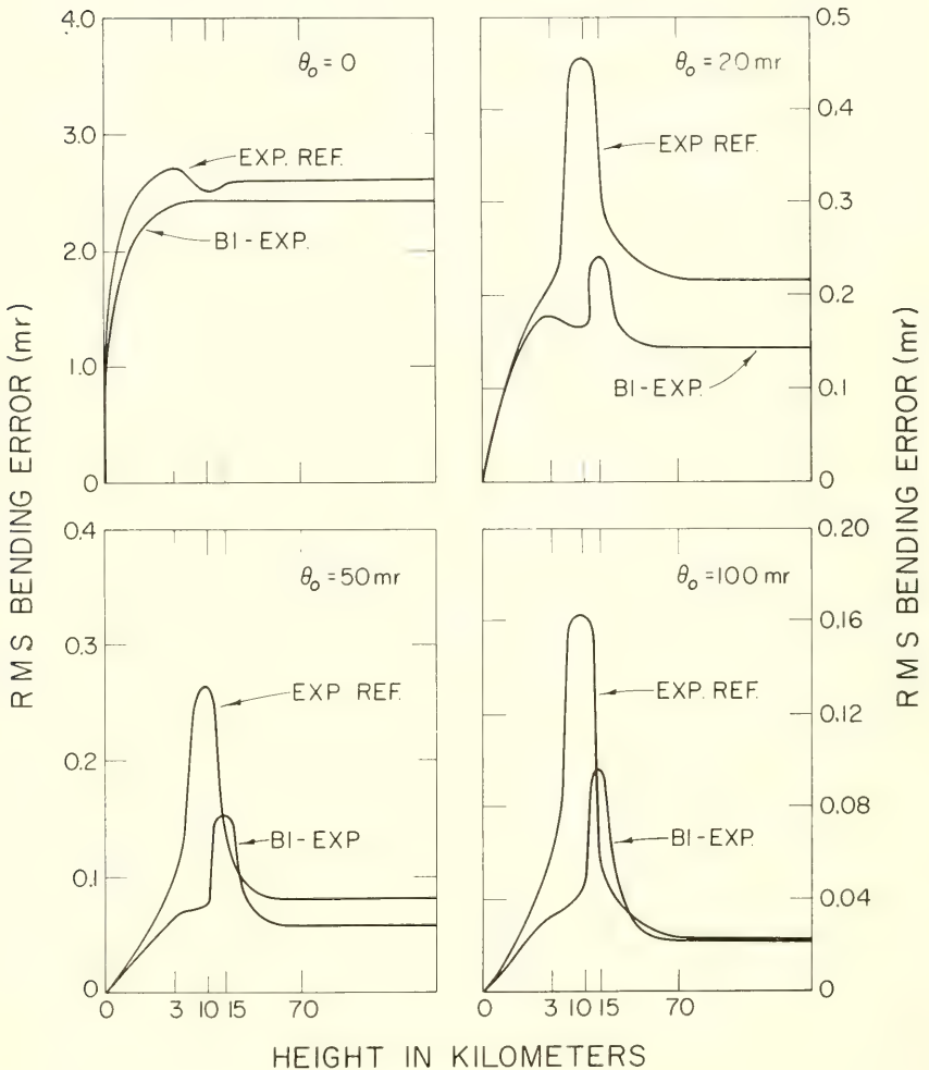
FIGURE 8.9. Root-mean-square errors of predicting bending for both the bi-exponential refractive index model and the C.R.P.L. (single) exponential atmosphere. Height is used here to indicate the actual thickness of atmosphere traversed by the radio ray
