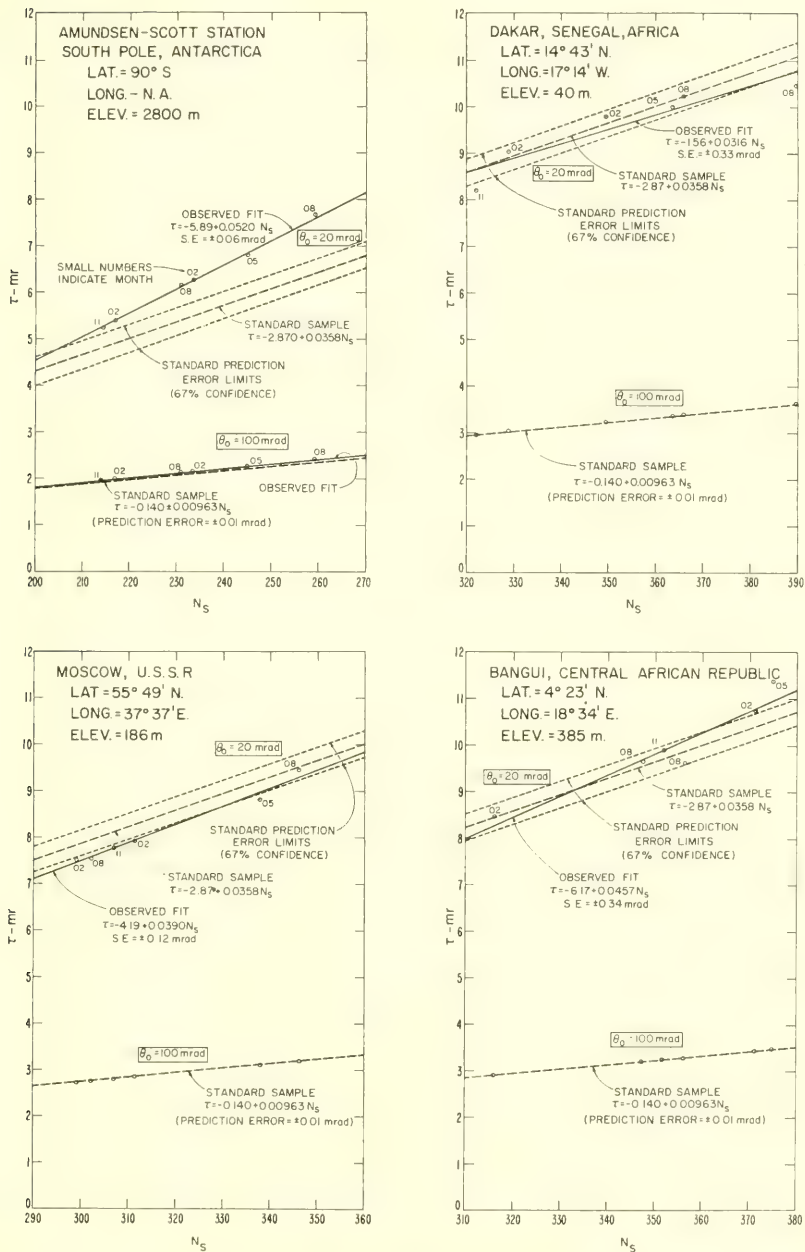
FIGURE 8.19. Comparison of predicted refraction at h equals 70 km for \theta_0 's of 20 mrad and 100 mrad from regressions of the CRPL standard sample and ray-traced values from four independent locations.
