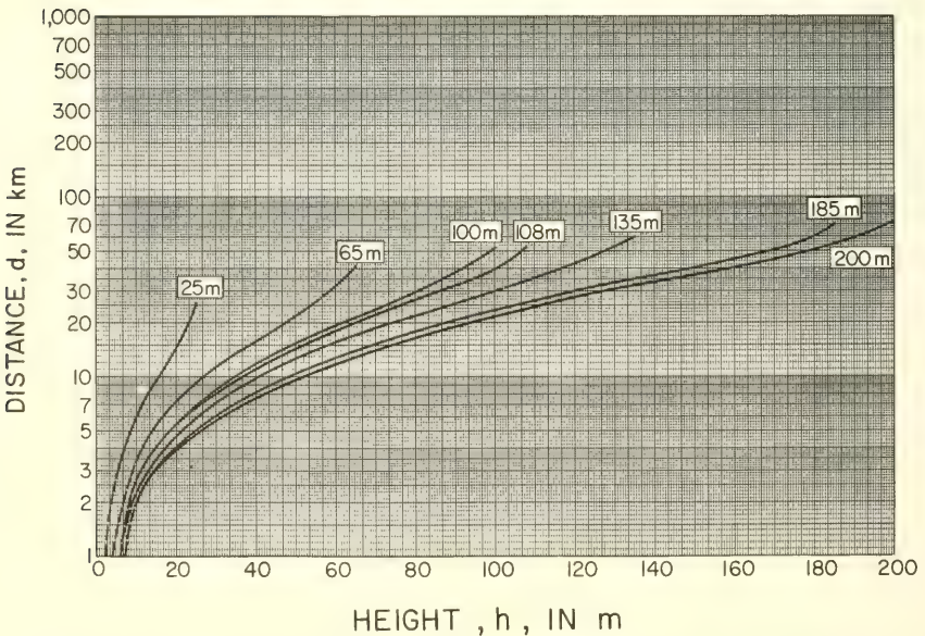
FIGURE 4.50. Height versus distance at Washington, D.C., for mean midspring (May) ducting conditions.
