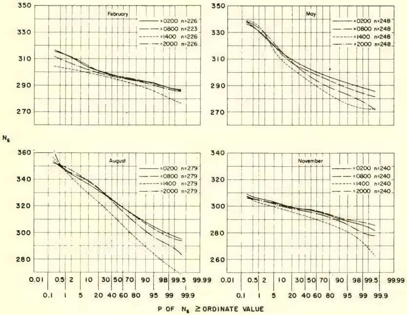
FIGURE 9.17. Cumulative probability distribution of N_8 , Bismarck, N.Dak.
