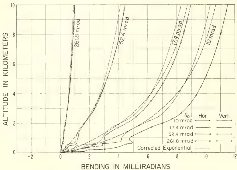
FIGURE 8.12. Canterbury, 0 to 10 km, altitude versus ray bending.
