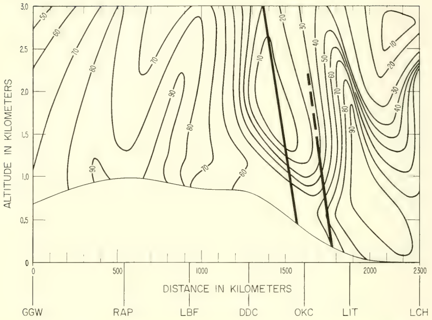
FIGURE 5.44. Relative humidity cross section (percent), 1500Z, 19 Feb. 1952.
