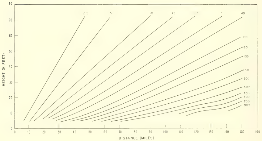
FIGURE 8.31. Standard error of \epsilon_h versus N_s .
