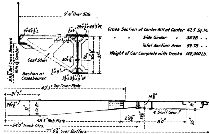
Fig. 1—Underframe with Deep Center Sills and Light Side Girders
