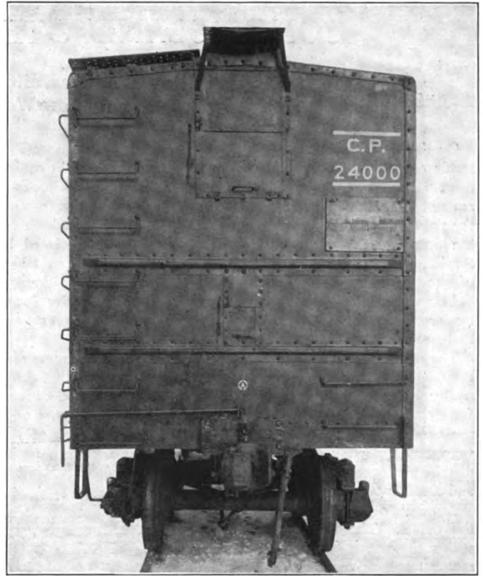
End View of the Canadian Pacific Car
