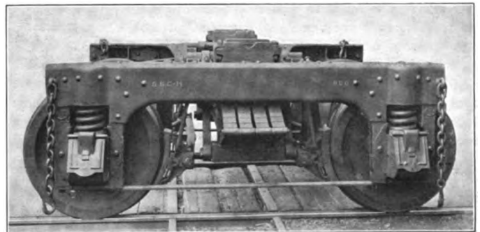
Four-Wheel Truck for Long Island Steel Trailers
