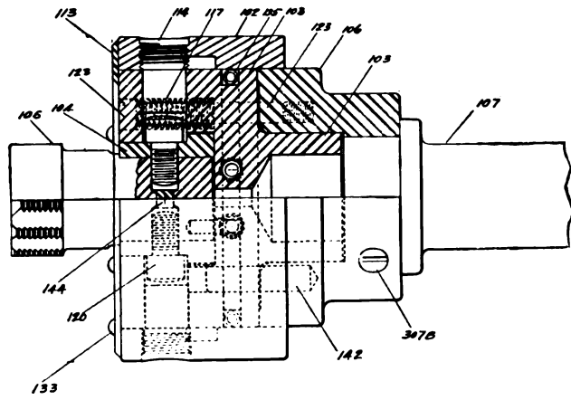
Details of Modern Collapsible Tap
