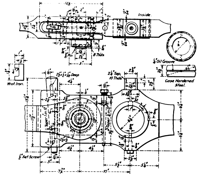
Fig. 25—Side Rod Stubs of Burlington Locomotives
