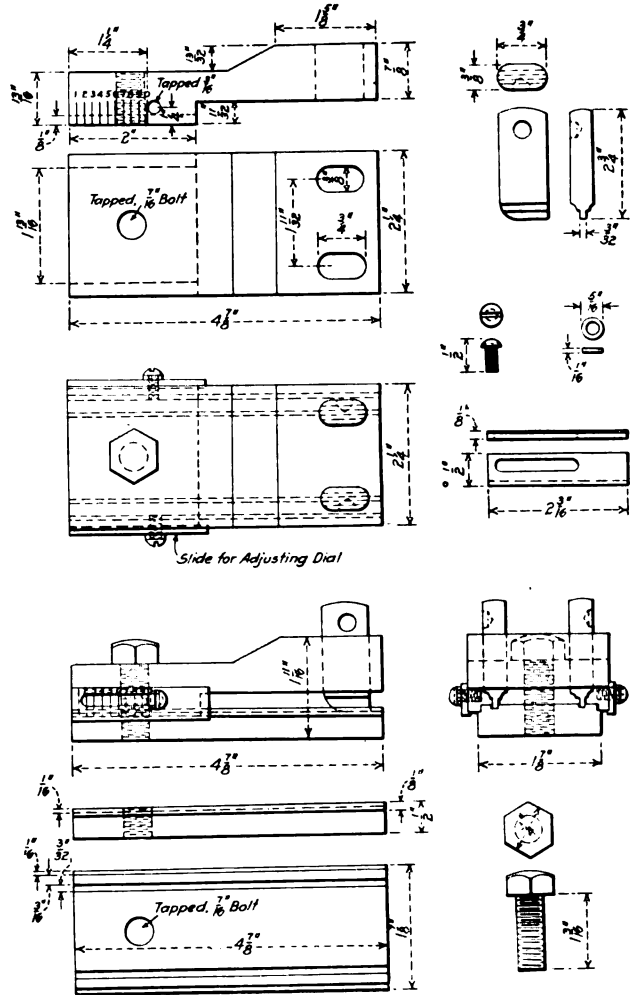
Fig. 3.—Tool for Punching Clips in Gage Dials
