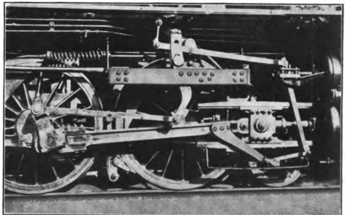
Application of the Kingan-Ripken Valve Gear Device
