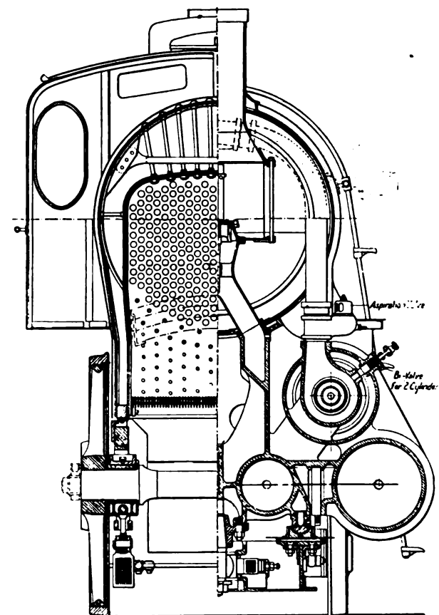
Half Sections Through Cylinders and Firebox
