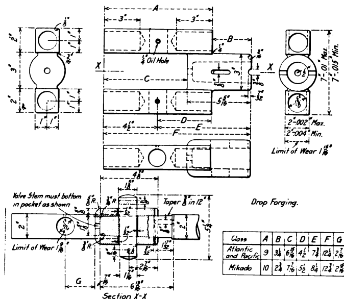
Fig. 14—Valve Stem Crosshead of Pennsylvania Locomotive
