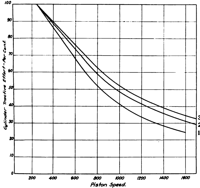
Curves Showing Possibilities of Increased Capacity from Superheating
