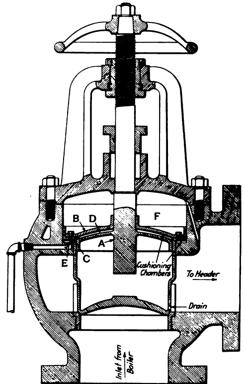
Golden-Anderson Automatic Non-Return Valve
