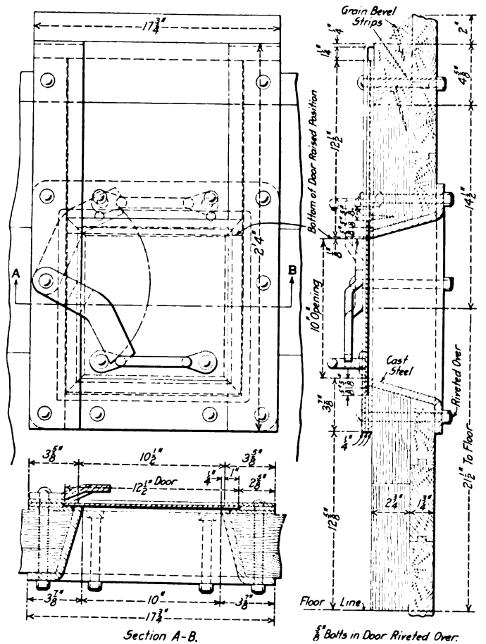
Lower Rail End Door, Canadian Government Railways
