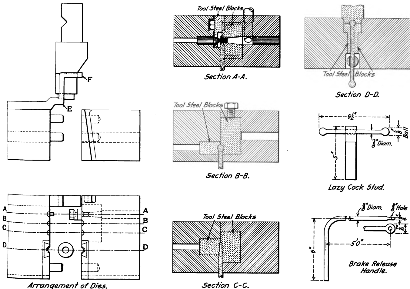
Forging Machine Dies with Insets of Tool Steel
