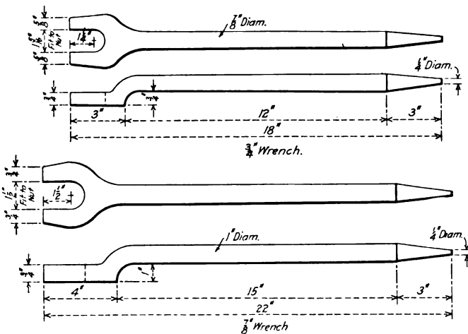
Wrenches for Use in Assembling Steel Cars
