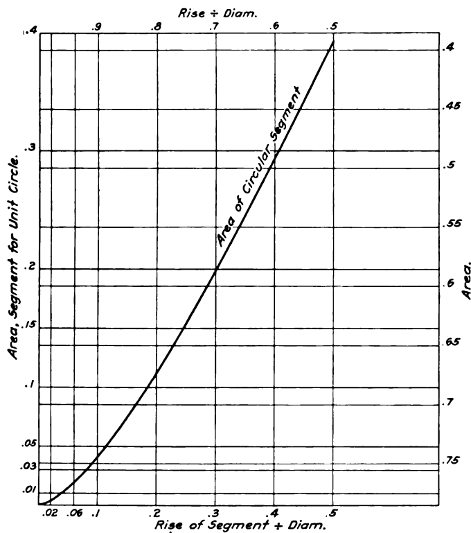
Fig. 2—Area of Circular Segments
