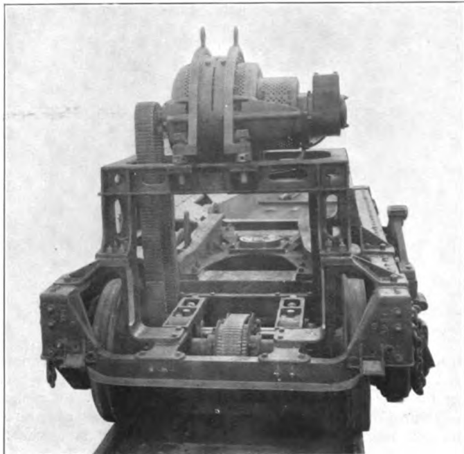
Axle Train Lighter Mounted on Truck
