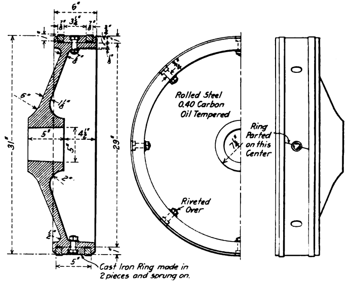
Fig. 21—Another Redesign of the Burlington Piston
