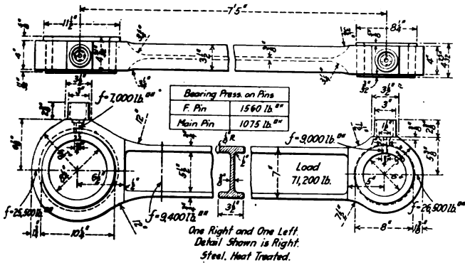
Fig. 7—Side Rod of Pennsylvania Atlantic Type Locomotive
