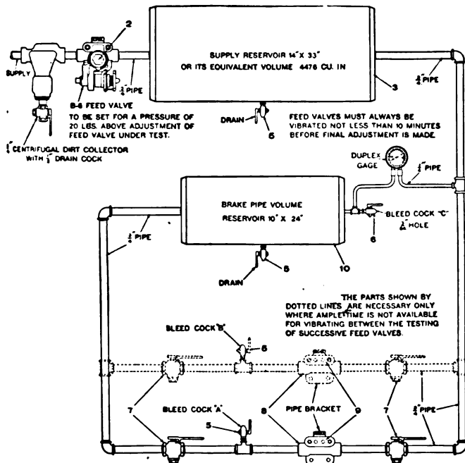
Diagrammatic Arrangement of Slide Valve Feed Valve Test Rack
