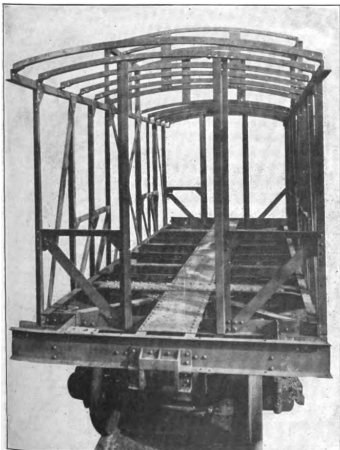
The Assembled Steel Frame of the B. R. & P. Caboose
