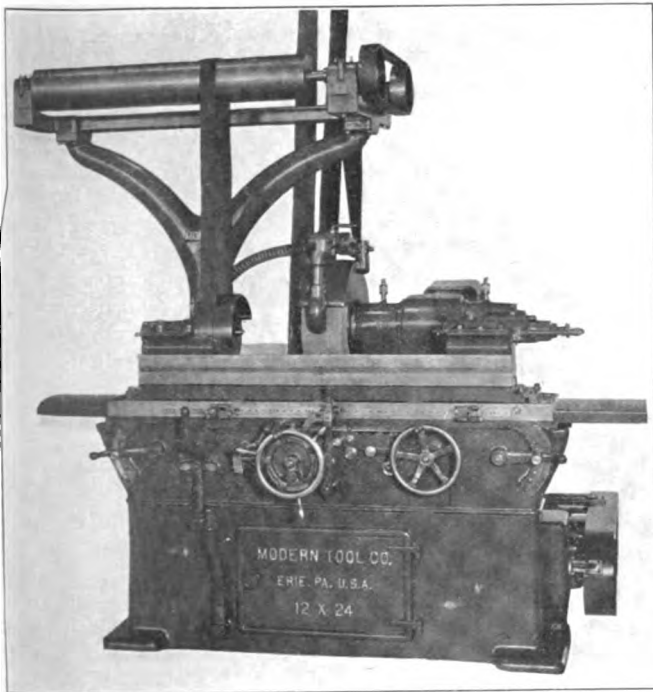
Self-Contained Single Pulley Universal Grinder
