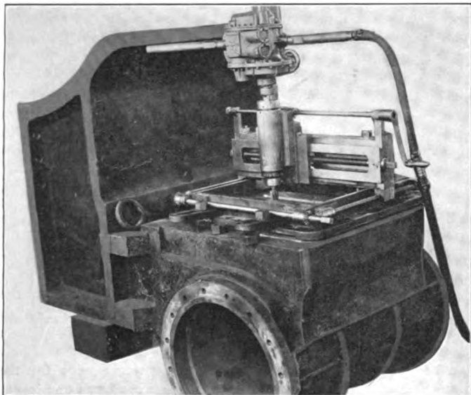
Fig. 7—Valve Seat Port Miller
