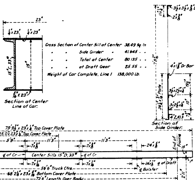
Fig. 5—Underframe Used on the Canadian Northern
