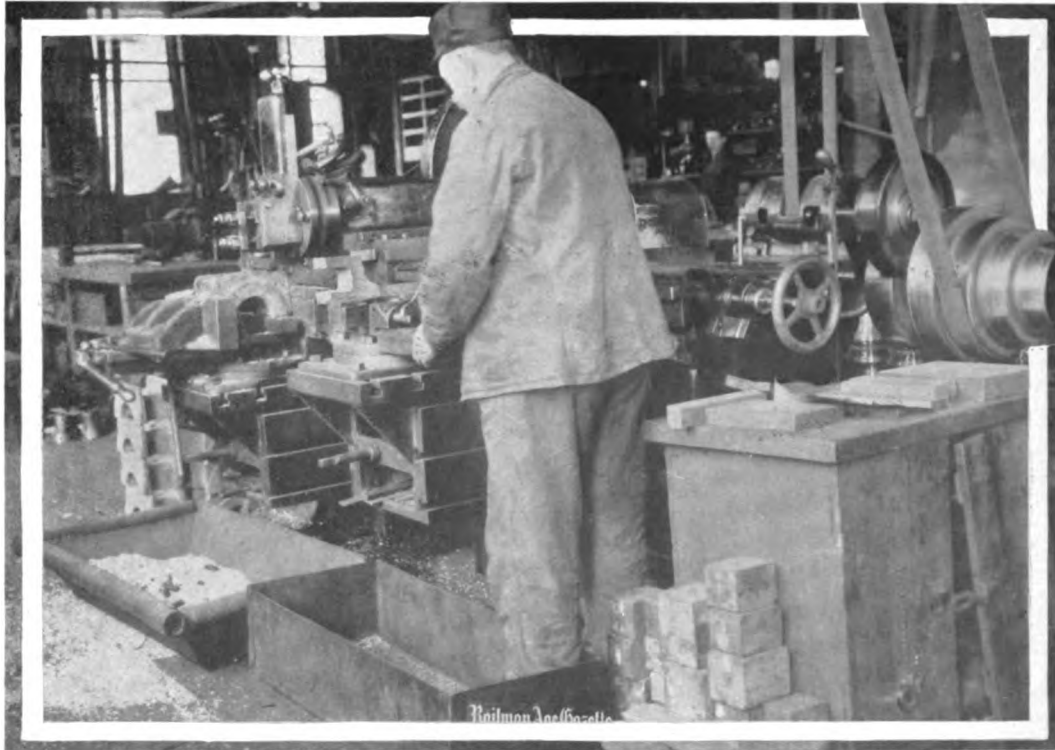
Regular 26-Inch Single Head Cincinnati Traverse Shaper in Railroad Service. The Operator is setting up a job, link clevice, on one table, while the head is at work on a main rod brass, on the other table.
