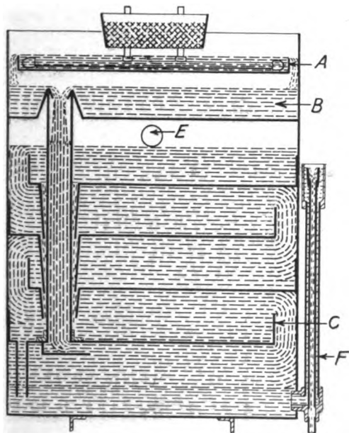
Fig. 2—Method of Operation of the Precipitation Compartment
