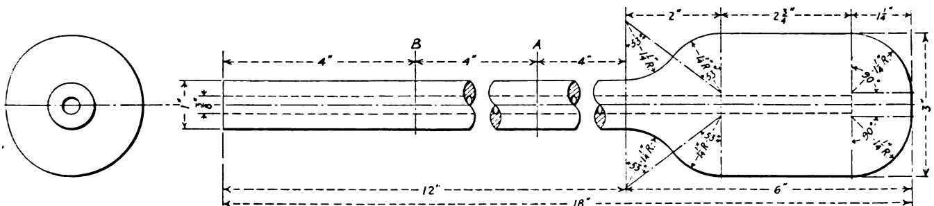
Fig. 1—Test Piece Used in Quenching Tests
