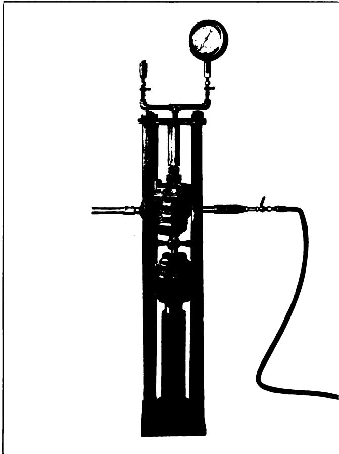
Fig. 12—Apparatus for Testing Air Motors
