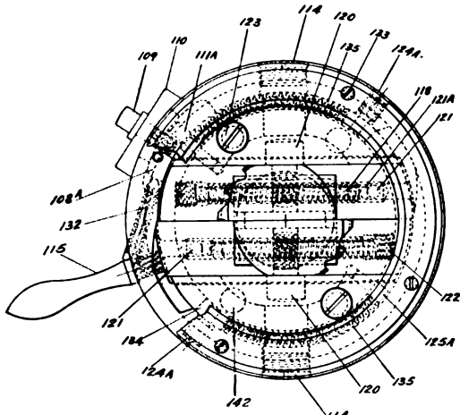
Details of Modern Collapsible Tap
