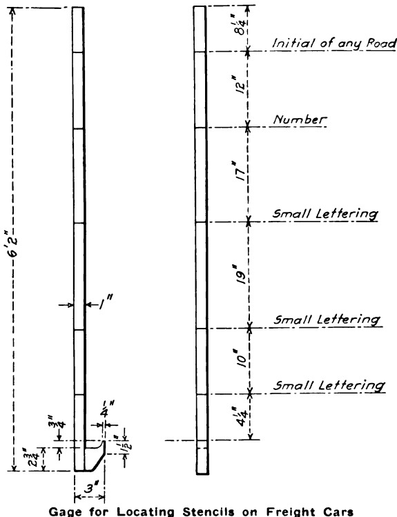
Gage for Locating Stencils on Freight Cars
