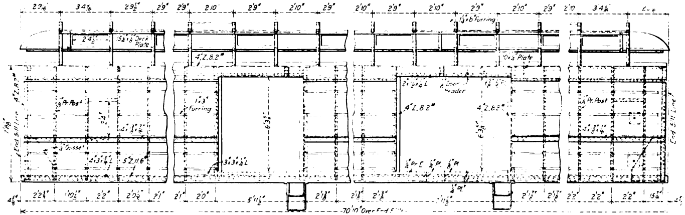
Side Frame of Northern Pacific Baggage Cars
