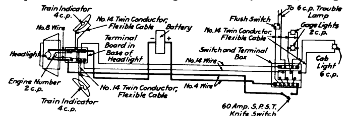
Wiring Diagram for Six-Volt Electric Headlight and Cab Lights
