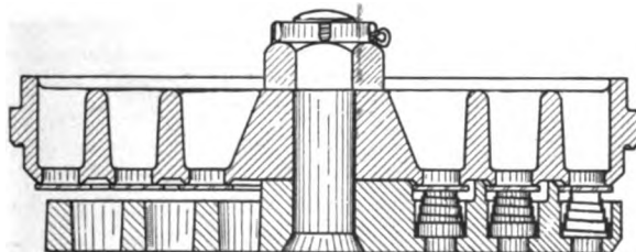
The Inlet Valve
