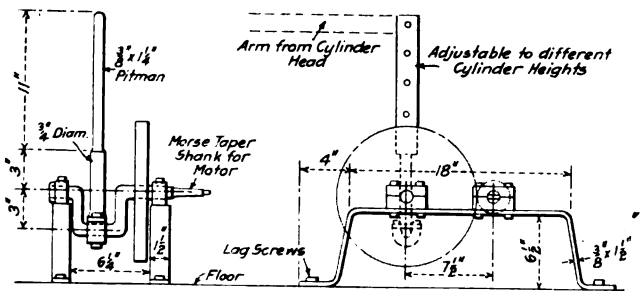
Attachment for Grinding Cylinder Heads
