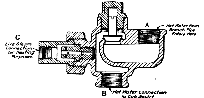
Sectional View of the Heater Check
