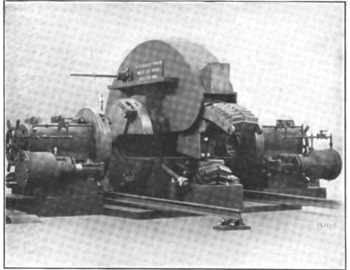
Back of the Car Wheel Lathe Showing Automatically Operated Gap in the Herringbone Gear
