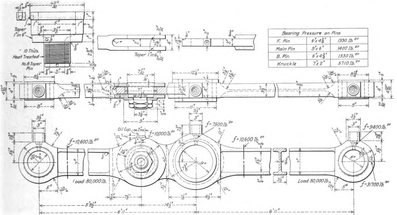
Fig. 12—Side Rods of Pennsylvania Pacific Type Locomotive
