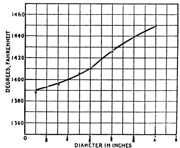
Fig. 14—Temperature-Size Curve for Hardening Tools
