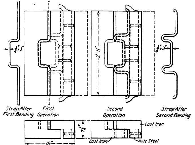
Fig. 11—Former for Making Brake Beam Safety Straps
