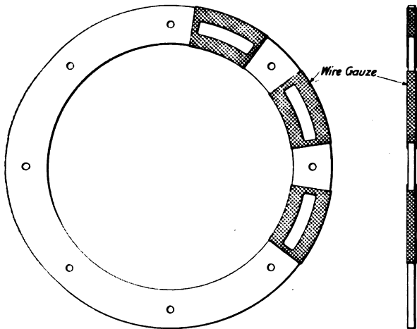
Reinforced Asbestos Fibre Gasket for Air Pumps
