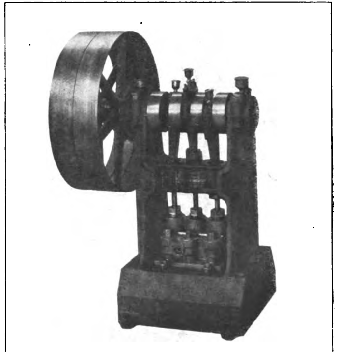
Small Single Acting Triplex Pump
