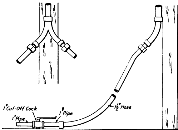
Arrangement of Y-Fitting for Washing Out Boilers.
