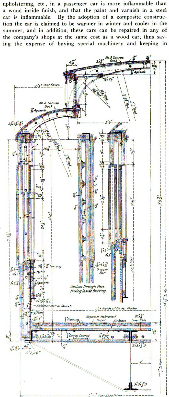
Cross Sections of the Grand Trunk Car
