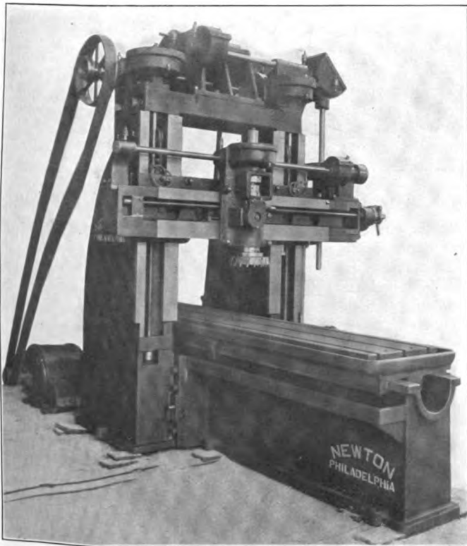
Single Pulley Driven Vertical Slabbing Machine
