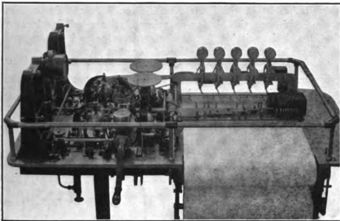
A Side View of the Recording Table
