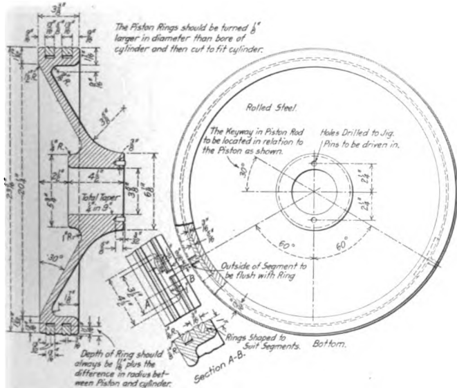
Fig 3—Piston of Pennsylvania Atlantic Type Locomotive
