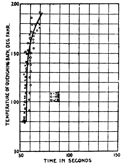
Fig. 3—Quenching Power of Brine Solutions
