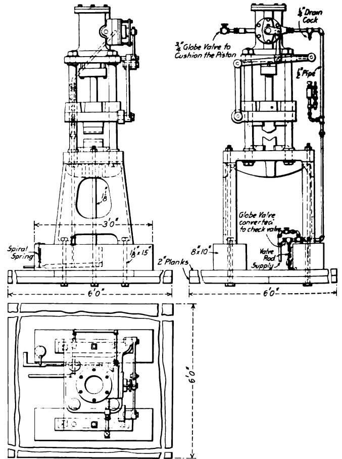
Pneumatic Hammer Assembled
