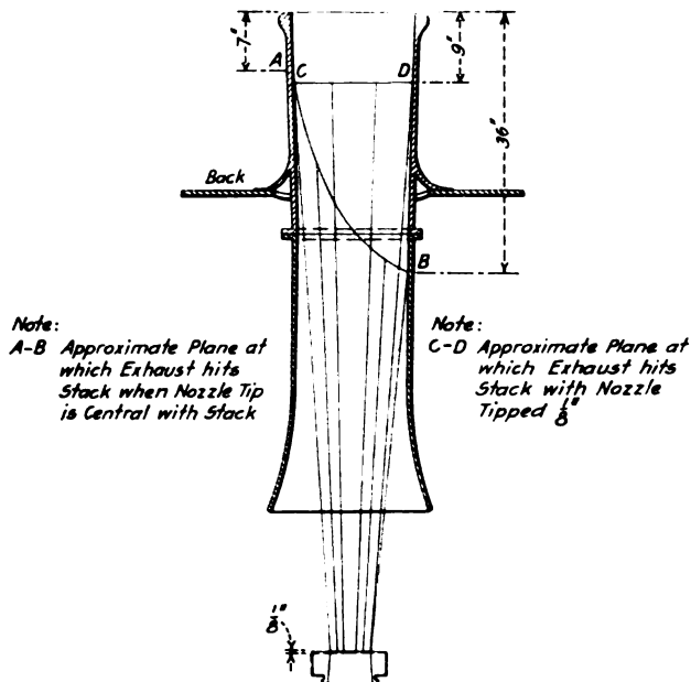
Fig. 5—Stack Conditions as Determined by the Apparatus Shown in Fig. 4
