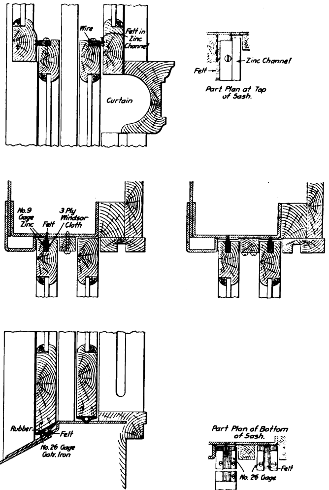
Metal Weather Strips with Cloth Lining
