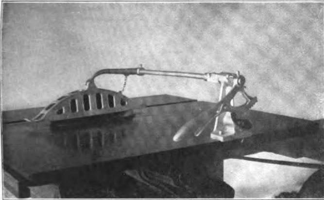
Fig. 1—Guard in Position Over the Saw
