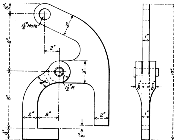
Lifting Hook for Tire Setting
