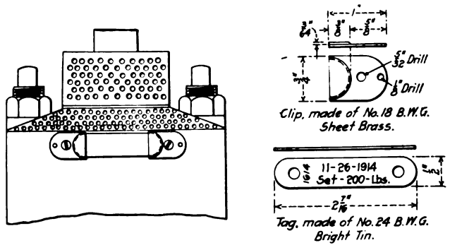
Fig. 4—Method of Securing Date Tags to Safety Valves
