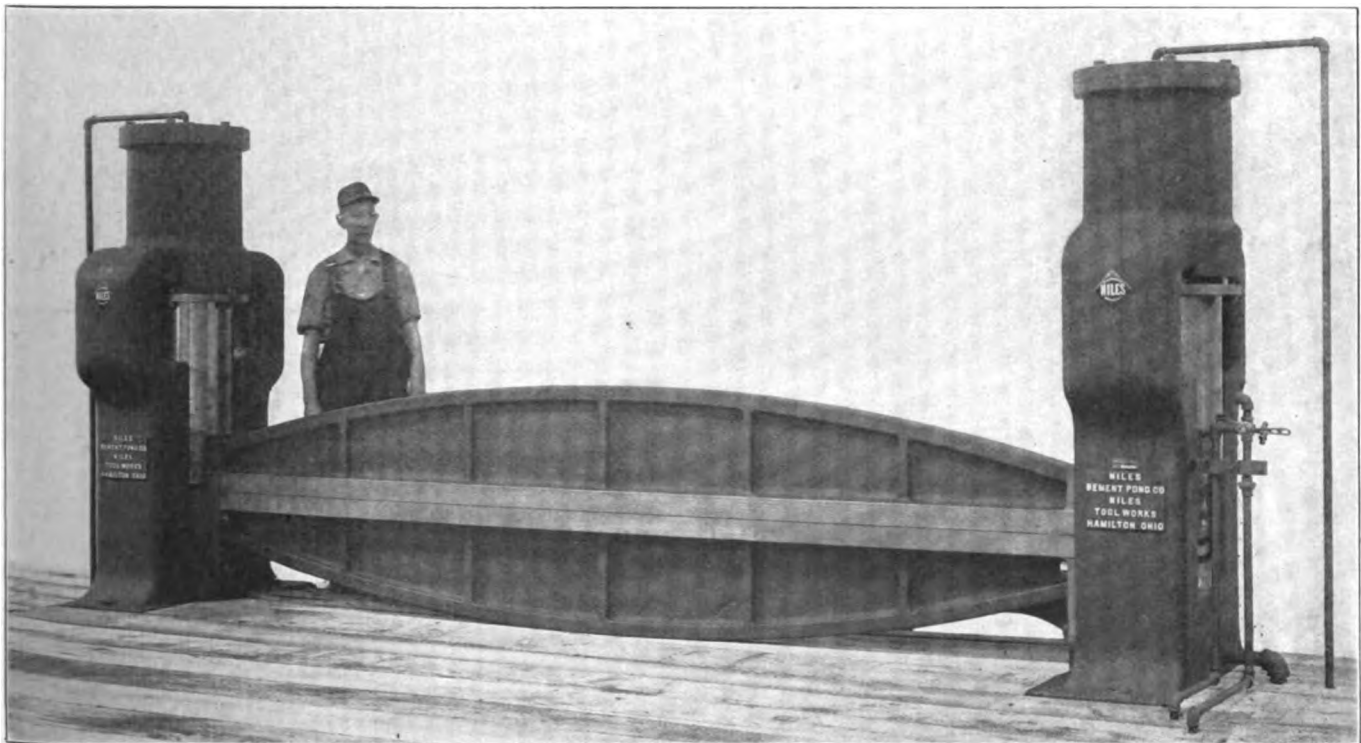
Pneumatic Plate Flanging Clamp
