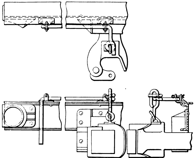
Coupler Rigging Having Few Parts
