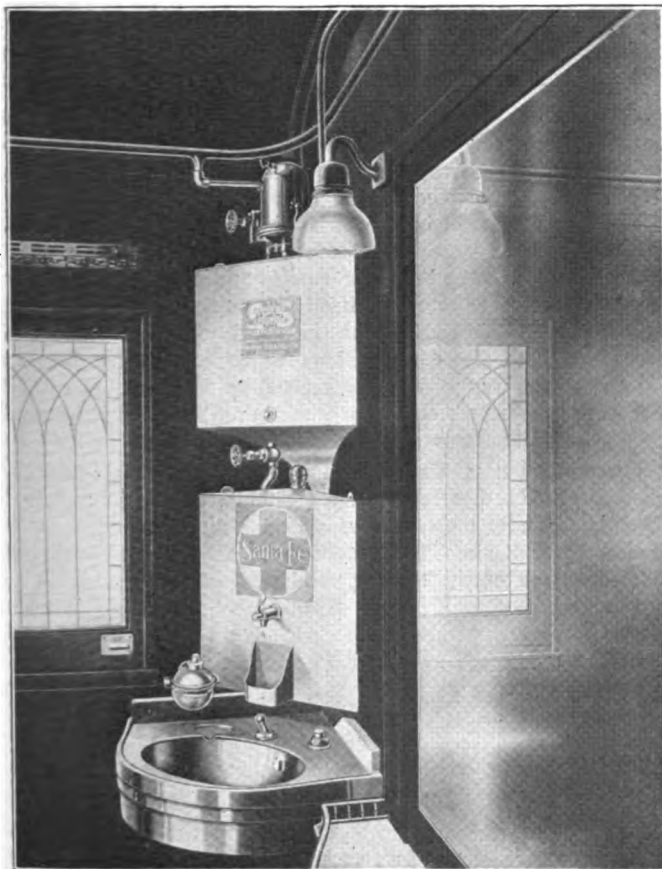
Sanitary Drinking Fountain Applied to a Passenger Car
