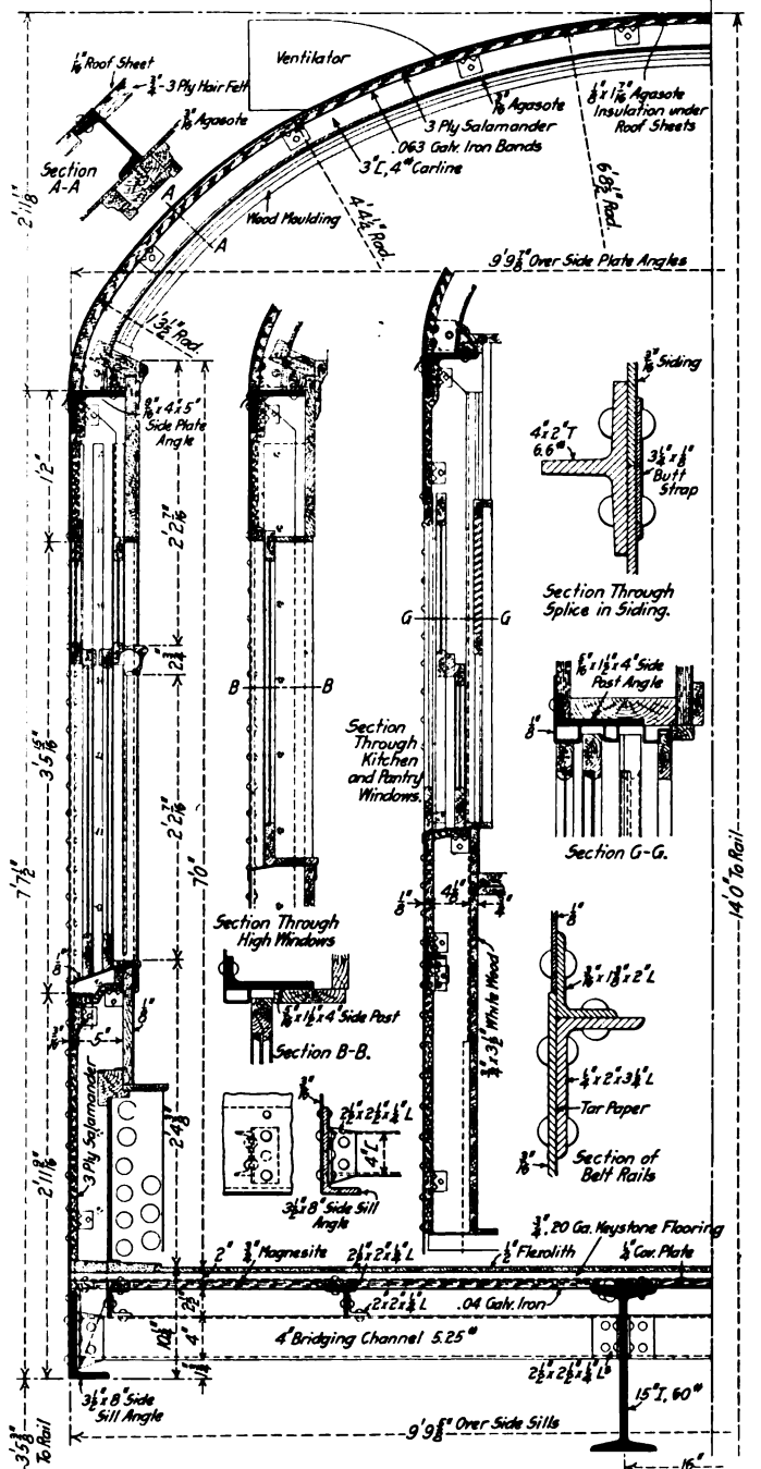
Cross Sections of the Dining Car
