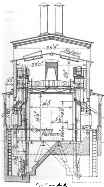
Sectional View Showing the Arrangement of the Machinery for Cleaning Steel Cars by Sand Blasting
