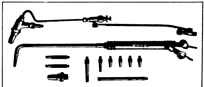
Welding Torch Showing the Cutting Attachment Removed
