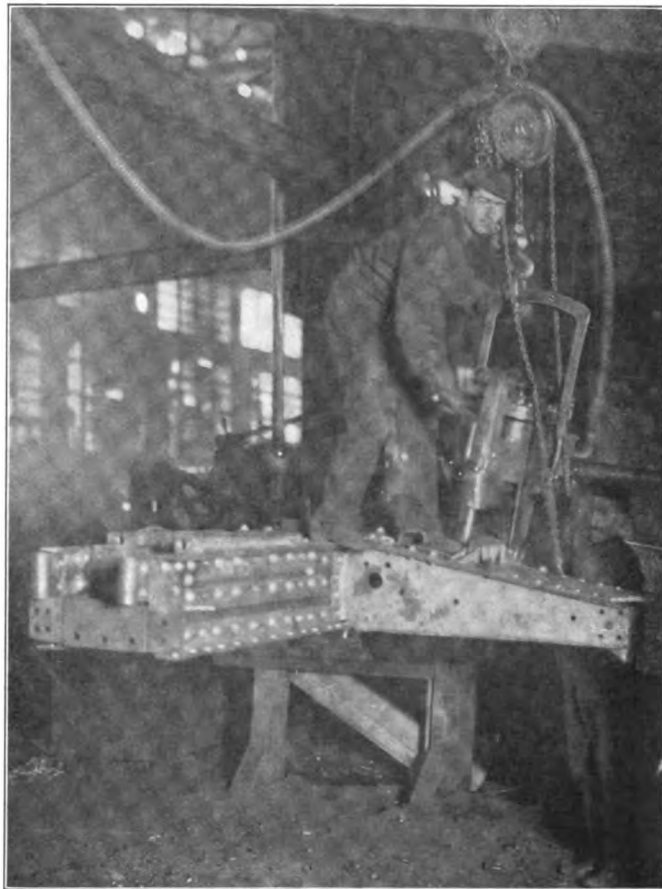
A Jaw-Riveter In Use on an Underframe, Showing Method of Suspension
