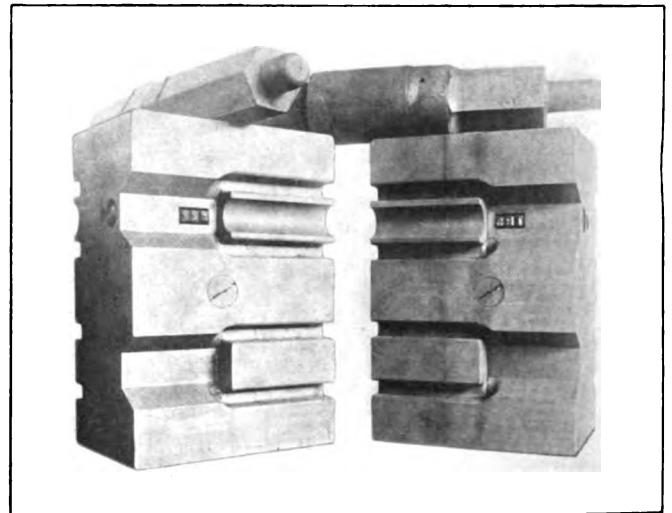
Fig. 6—Dies for Forming Turnbuckles
