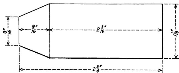
Taper Piston for Riveting Hammers
