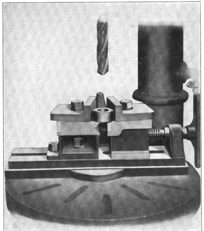
Supplementary Jaws for Holding Irregularly Shaped Piece
