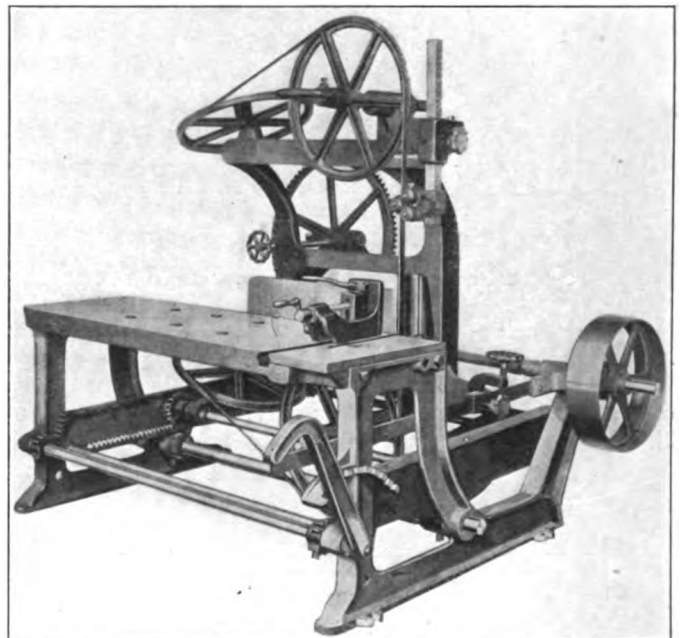
Gravity Feed Metal Band Saw
