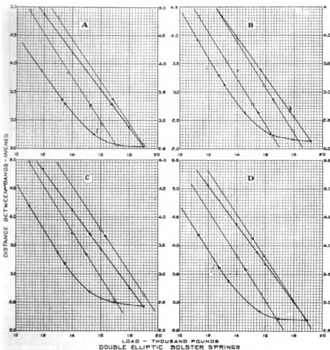
Fig. 15 ○ PLATES 4\frac{1}{2} \times \frac{3}{8} STEEL 3\frac{1}{2} \times \frac{3}{8} BANDS LENGTH LOADED 48" —○— SPRINGS WHEN NEW-OIL AND GRAPHITE BETWEEN PLATES —●— SPRINGS AFTER 7½ MONTHS SERVICE
