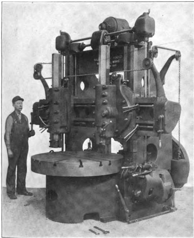
Niles Boring and Turning Mill
