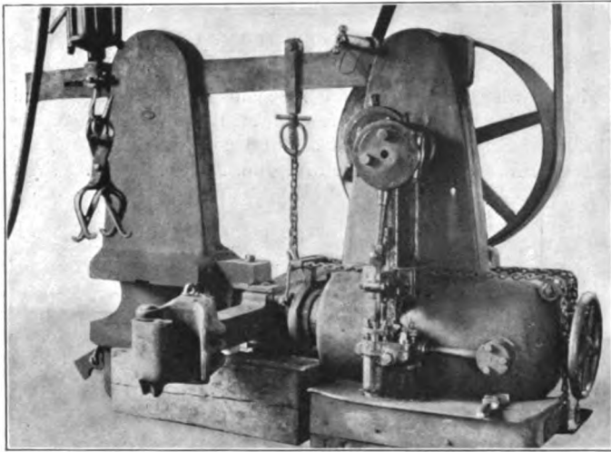
Fig. 1—Hydraulic Press for Removing Coupler Yokes
