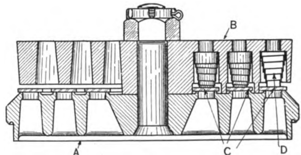
Flat Plate Discharge Valve of Three Separate Concentric Rings
