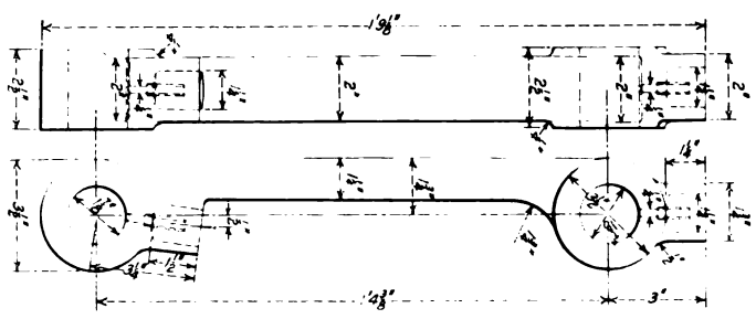
Fig. 49—Radius Rod Lifter for 4-6-4 Type Locomotive
