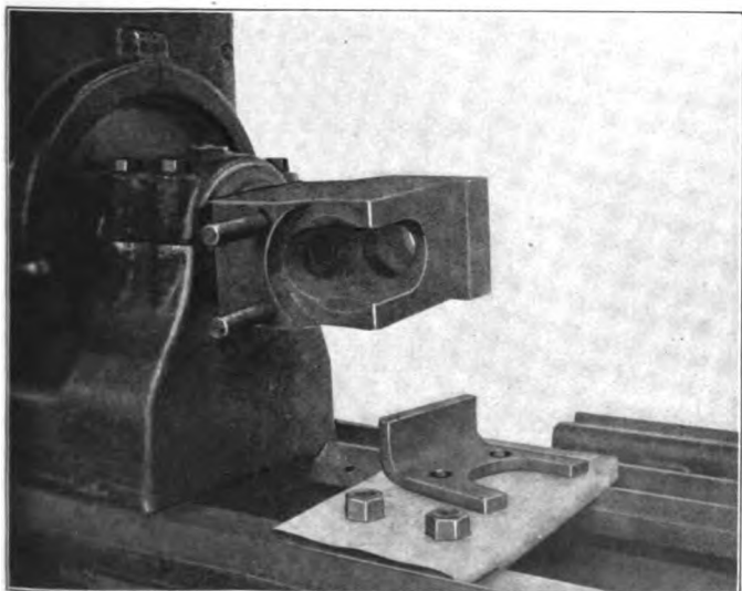
Chuck for Finishing Boiler Check Bodies
