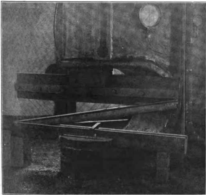
Fig. 13—Form for Bending Channels Into Stakes for Steel Cars
