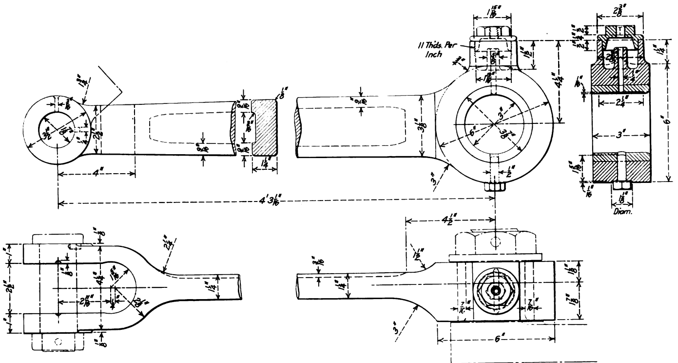
Fig. 52—Eccentric Rod for 4-6-4 Type Locomotive
