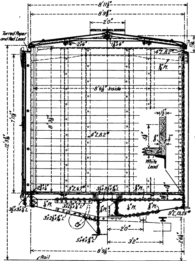
Cross Sections of the Illinois Central Car
