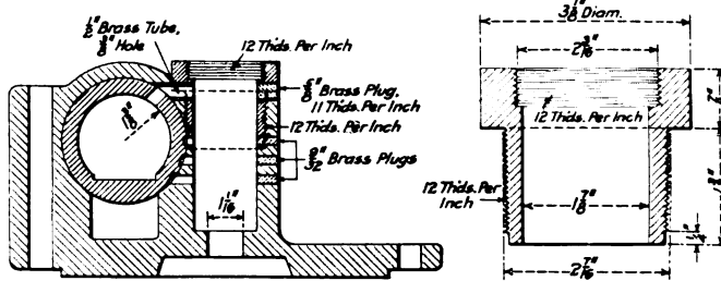
Method of Repairing Worn Air Pump Cylinder Heads
