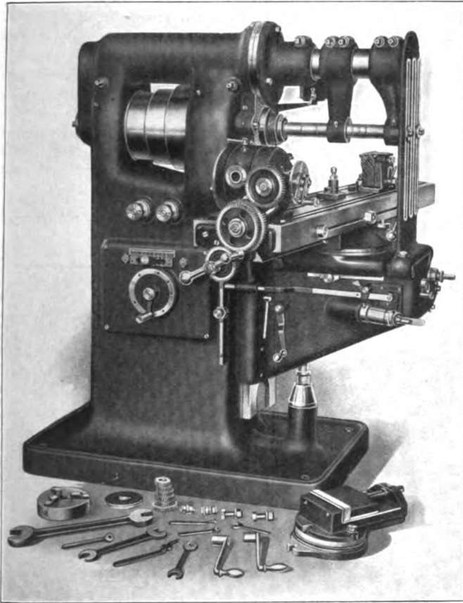
Double Back Geared Universal Milling Machine
