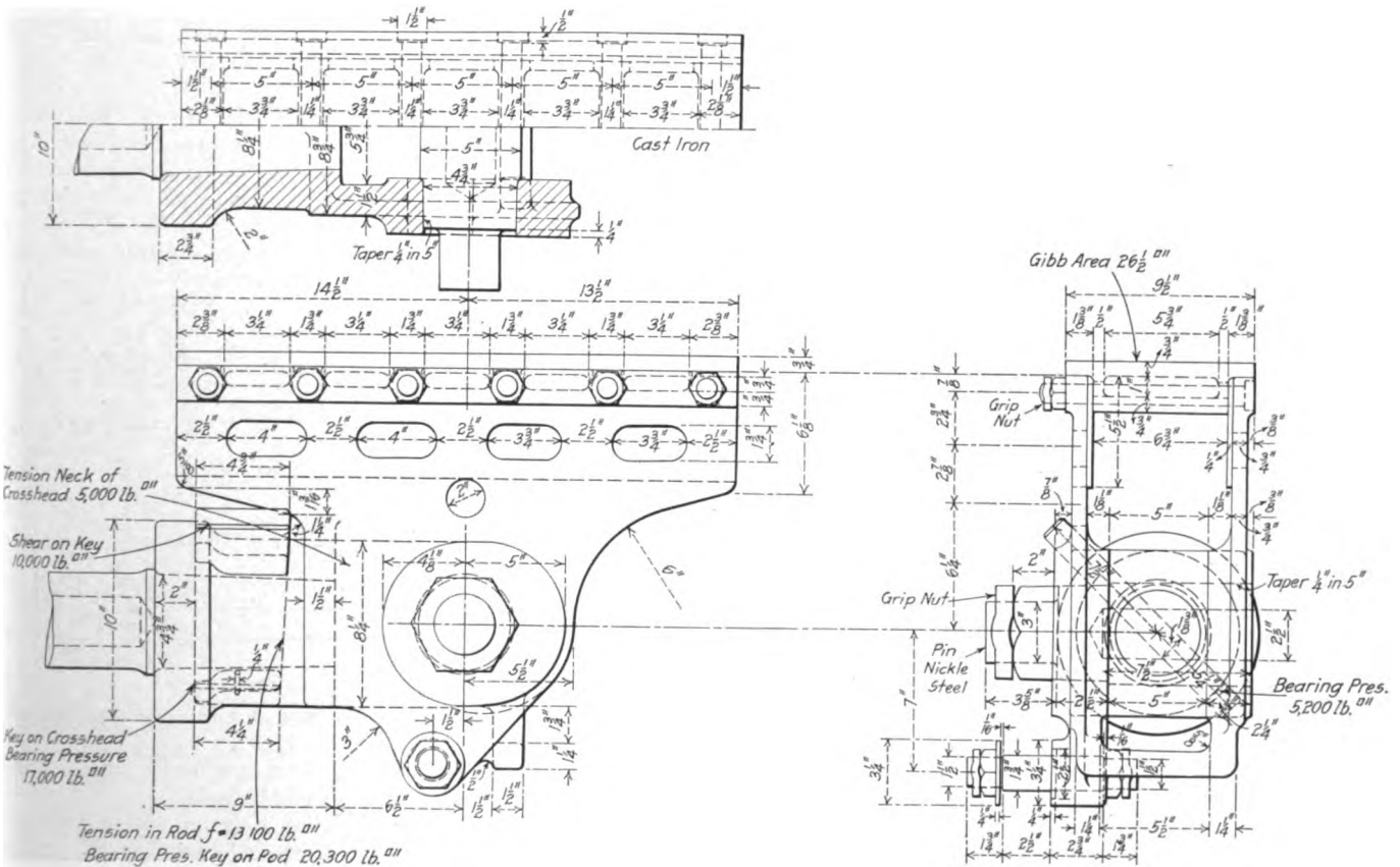
Fig. 24—Crosshead Used on the Burlington 2-10-2 Type Locomotives
