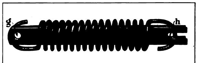
Fig. 4—Belt Tension Spring Assembled on Its Carrier
