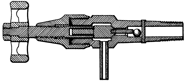
Glenn Gage Cock
