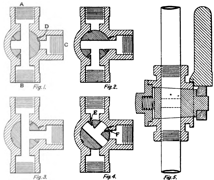
Safety Cut Out Valve for Locomotives
