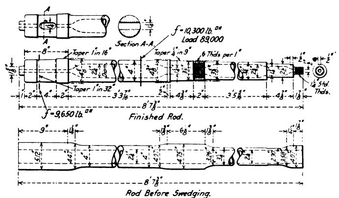
Fig. 4—Piston Rod of Pennsylvania Atlantic Type Locomotive
