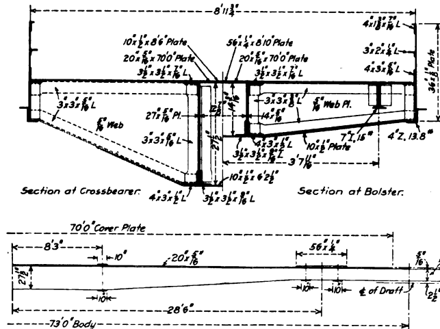
Fig. 2—Underframe Designed to Carry the Weight on the Center Sills, with a Sustaining Side Girder
