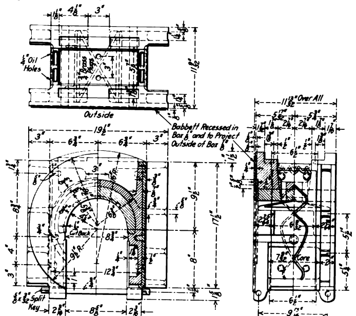
Type of Cast-Steel Driving Box Handled
