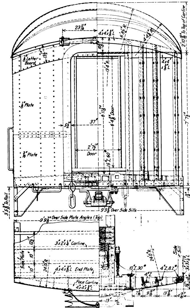
End Construction of Postal and Baggage Car
