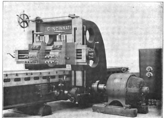
Planer for Finishing Switch Point Slide Plates
