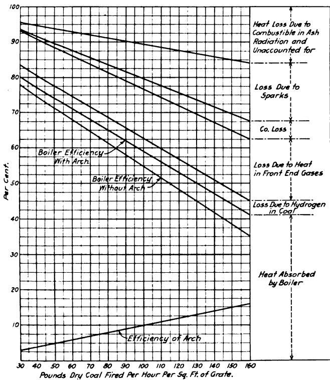
Fig. 3—Chart Showing Effect of Rate of Combustion on Efficiency of Boiler and Arch and on Heat Losses
