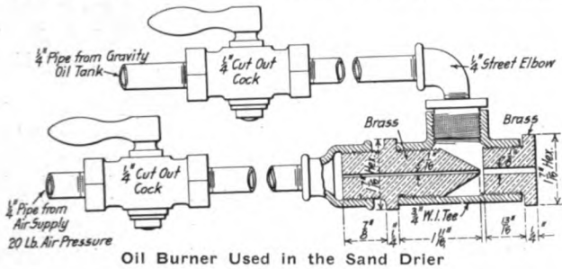
Oil Burner Used in the Sand Drier
