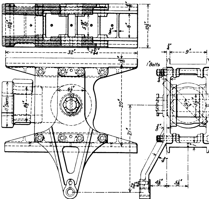
Crosshead of the Erie 2-10-2 Type Locomotive
