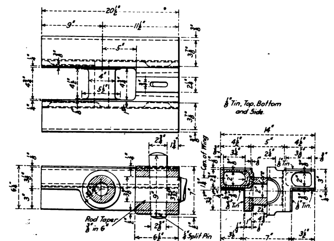
Fig. 9B—Four-bar Crosshead
