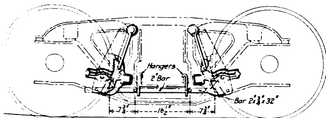
Brake Beam Safety Bar Attached to a Truck
