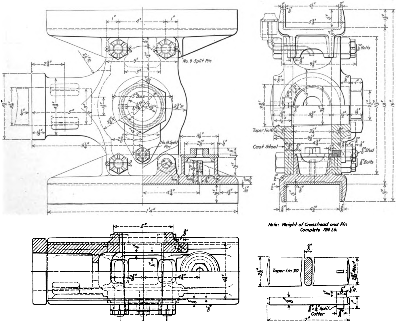
Fig. 34—Outside Crosshead of the Great Western Engine
