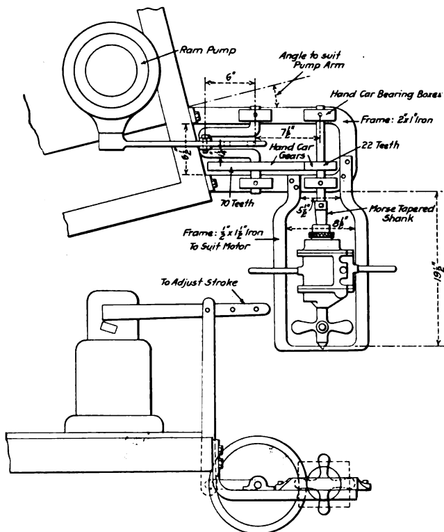
Hydraulic Press Attachment
