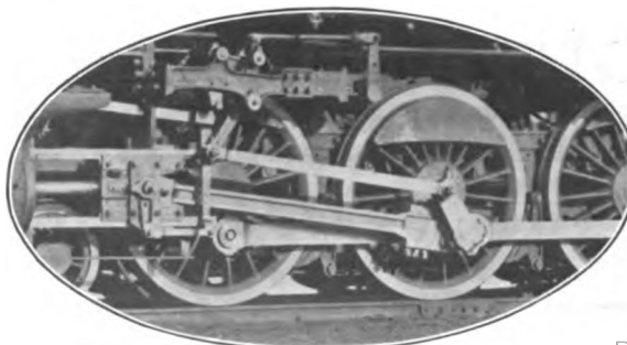
STANDARD BAKER VALVE GEAR FOR PACIFIC TYPE LOCOMOTIVES
