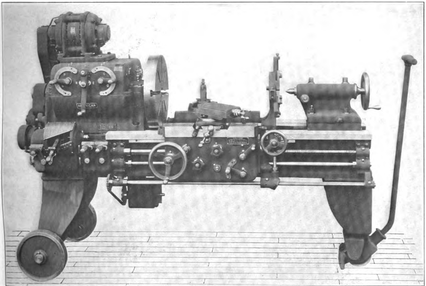
Portable Lathe for Railway Shops
