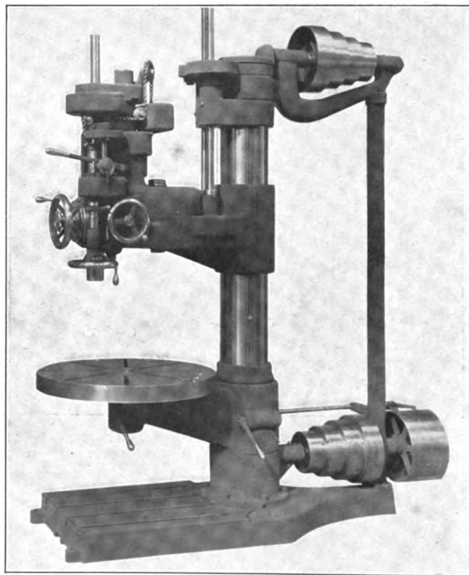
Willmarth Radial Drill
