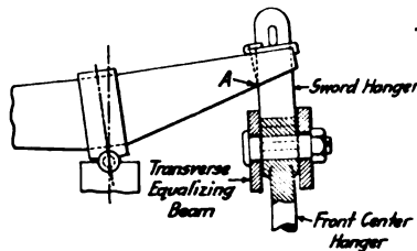
Fig. 10—Showing Restricted Movement of Sword Hanger in Spring
