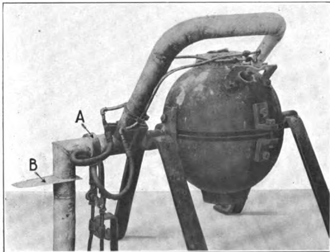
Furnace for Melting Small Quantities of Brass
