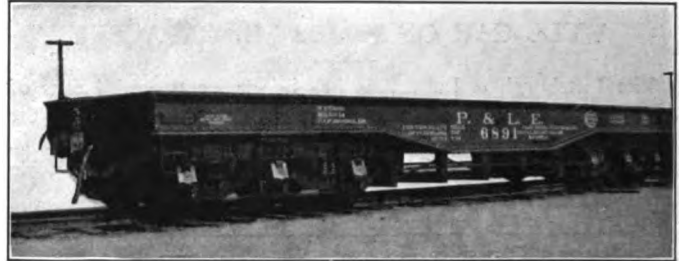
Pittsburgh & Lake Erie Well Car
