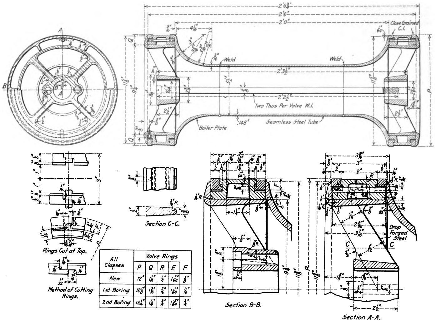
Fig. 15—Piston Valve Used on the Pennsylvania Locomotives
