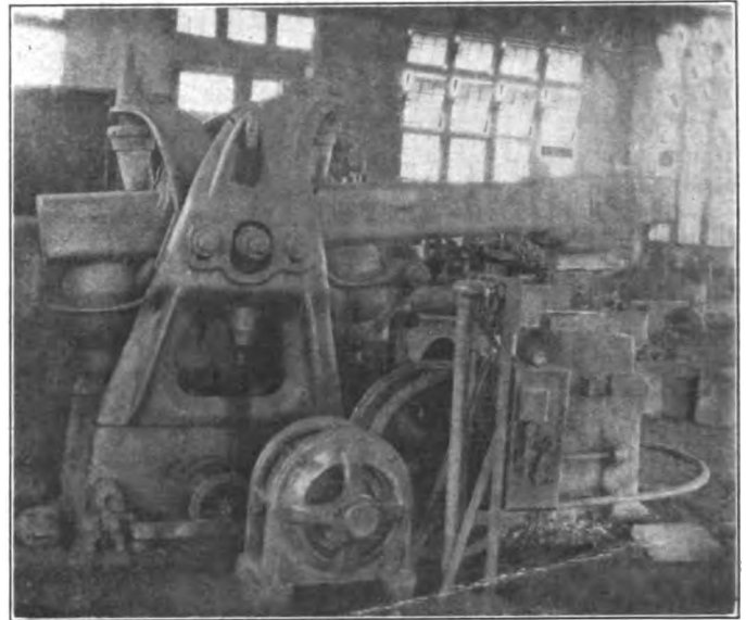
Location of Driving Motor for Helve Hammer
