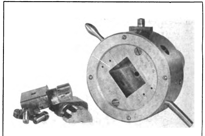
Collapsible Tap with Chasers Removed
