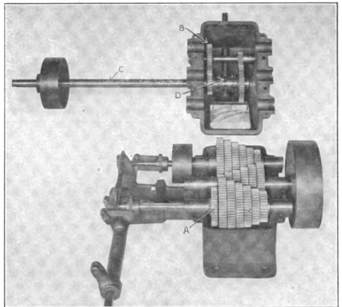
Arrangement of Gears in the Speed Box
