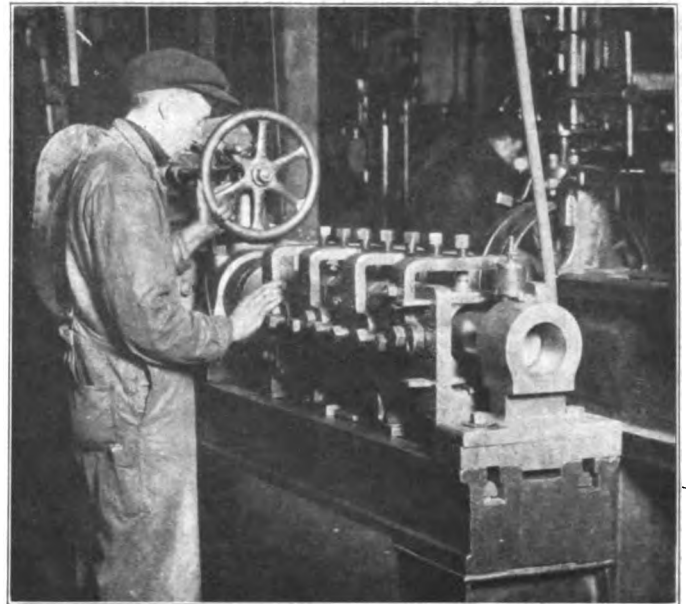
Front End Main Rod Brasses Set Up in Old Horizontal Boring Mill
