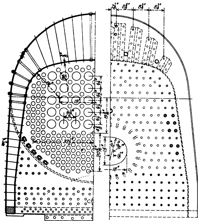
Cross Sections of the Boiler
