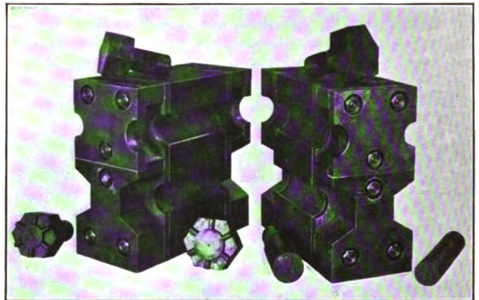
Fig. 11—Dies for Forming Large Castle Nuts
