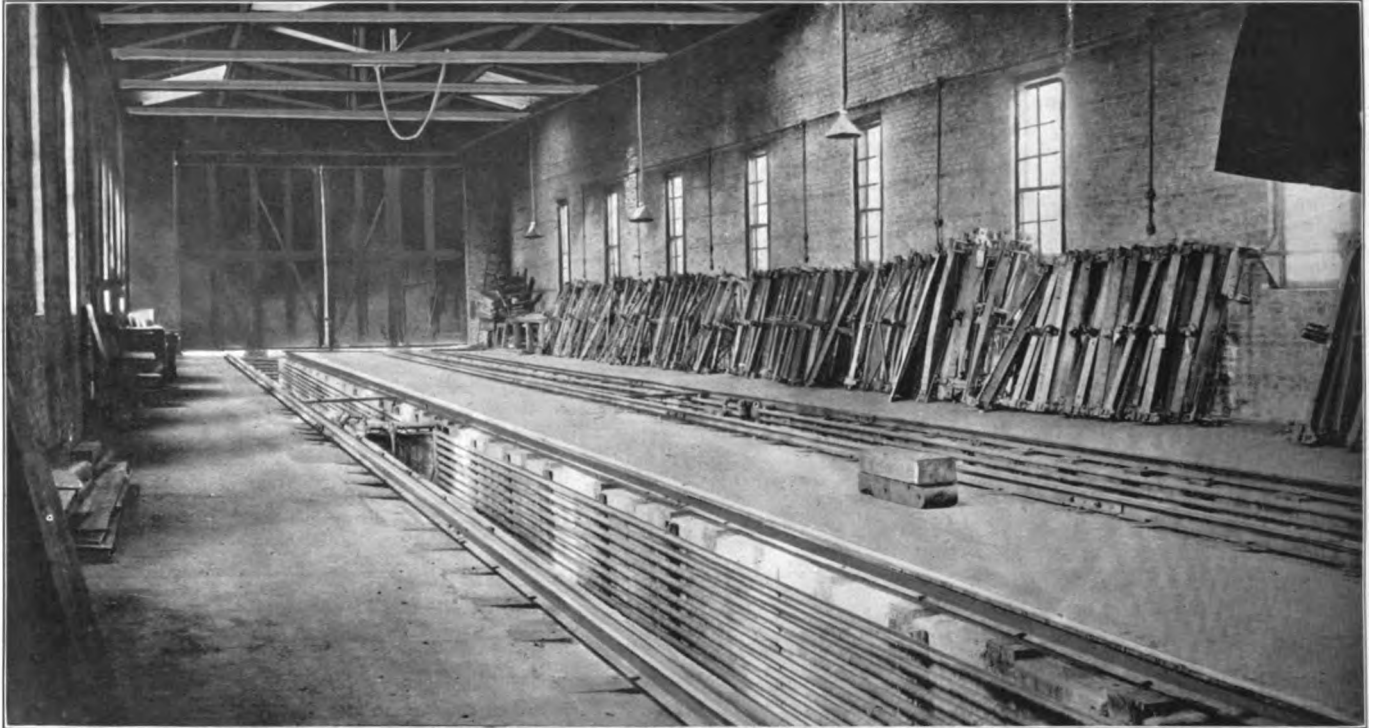
Interior of Thawing House, Chicago & Western Indiana
