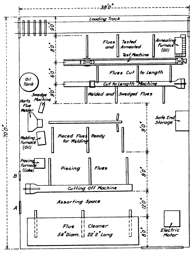
Fig. 3—Plan of the Flue Shop Showing the Location of the Machines
