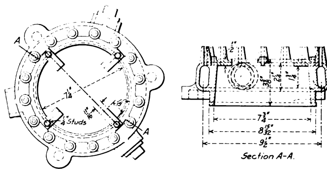
Internal Projection Exhaust Nozzle
