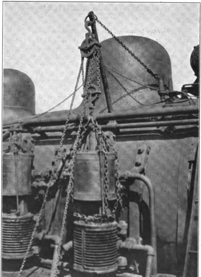
Air Pump Being Placed in Position on the Locomotive
