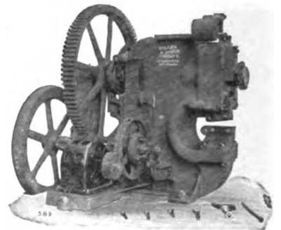
Vertical Open Throat Bar Shears. All sizes. Cam shaft bearings bronze bushed. Driving shaft easily removed without disturbing gears or keys.
