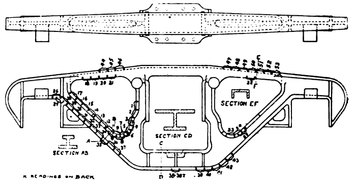
Fig. 2—Truck Frame Design B
