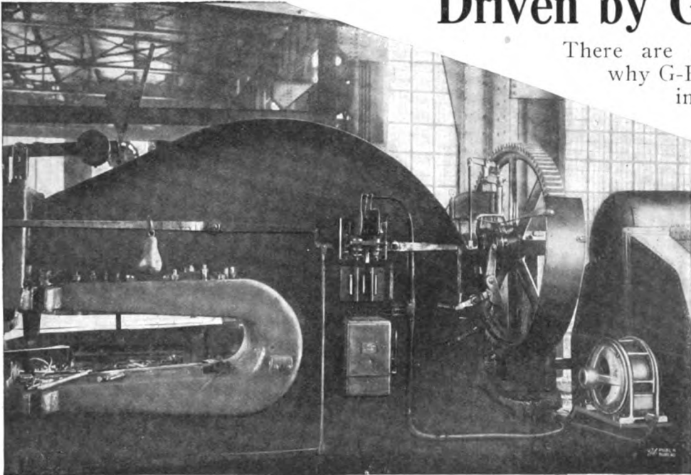
7 1/2 H. P. Induction Motor Driving Boiler Punch Press, G. C. C. and St. L. R. R. Company, Beech Grove, Ind., Shops.
