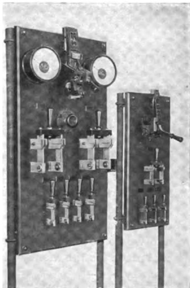
ARC WELDING GENERATOR CONTROL PANEL AND OPERATOR'S PANEL.
