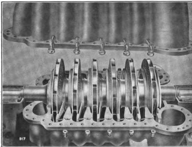
Six-Stage Compressor with Top Casing Removed
