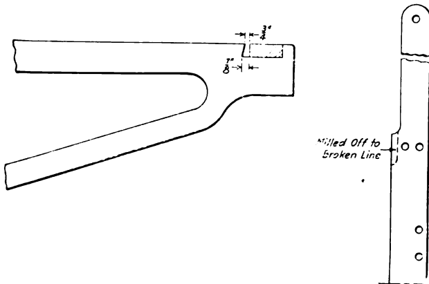
Method of Refitting Worn Tail Braces
