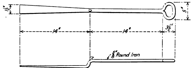
Journal Box Packing Iron with Improved Features
