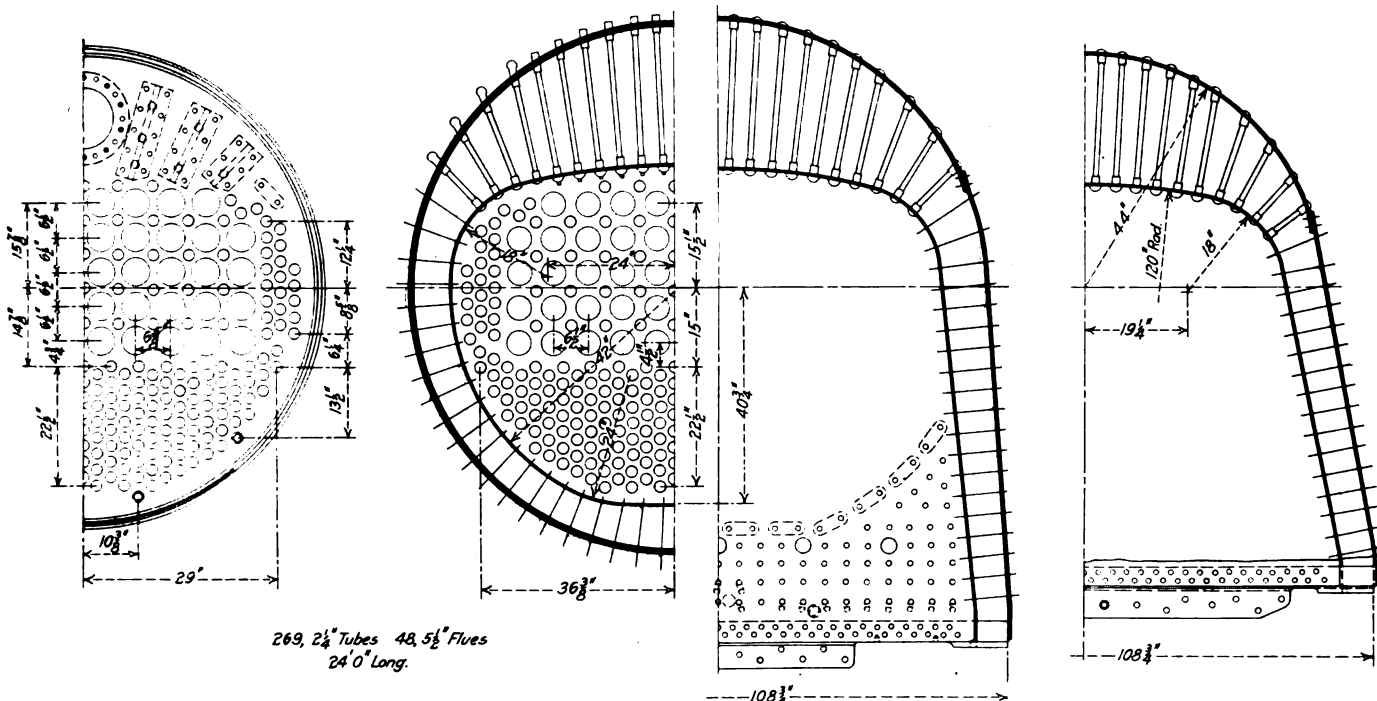
Cross-sectional Elevations of the Boiler
