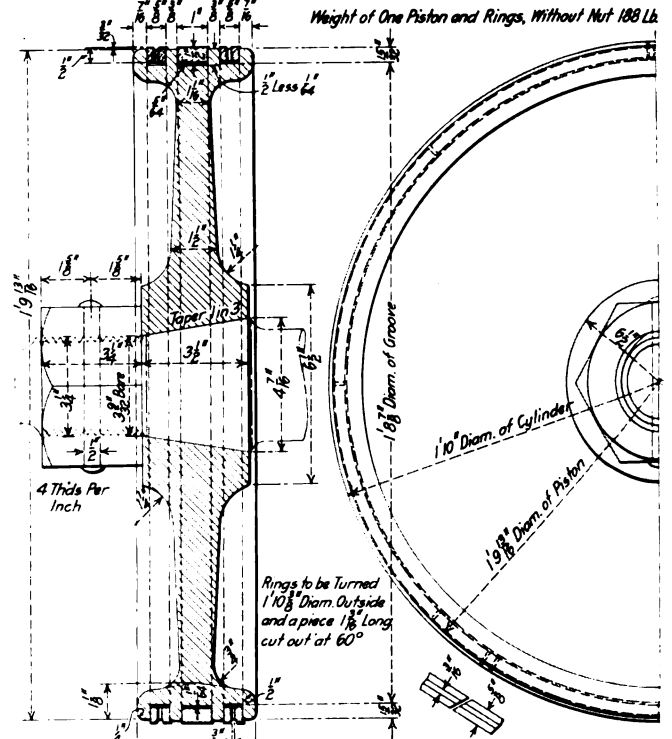
Fig. 41—Cast Steel Piston Head of London, Brighton & South Coast 4-6-4 Type Locomotive
