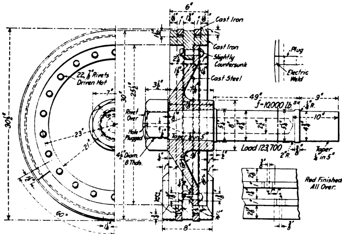
Fig. 19—Piston and Rod for Burlington Locomotives
