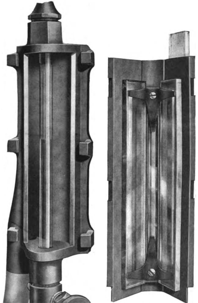
Water Glass Guard with Slot for Illumination.
