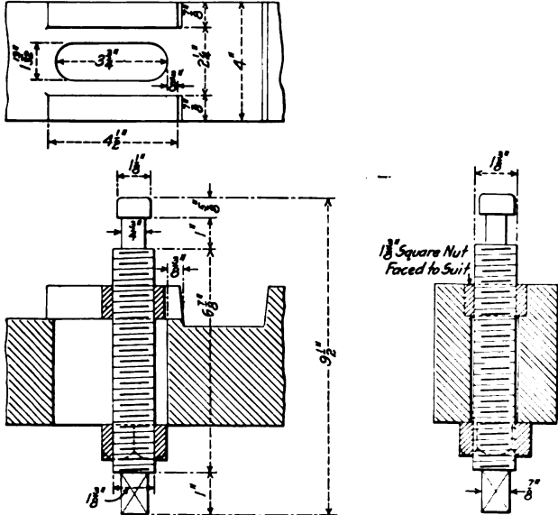
Wedge Bolt Which May Be Removed with Binders in Place
