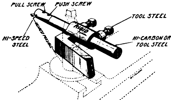
The Rigid Tool Post Holder
