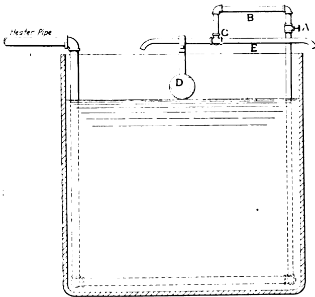
Automatic Regulating Device for Lye Tanks
