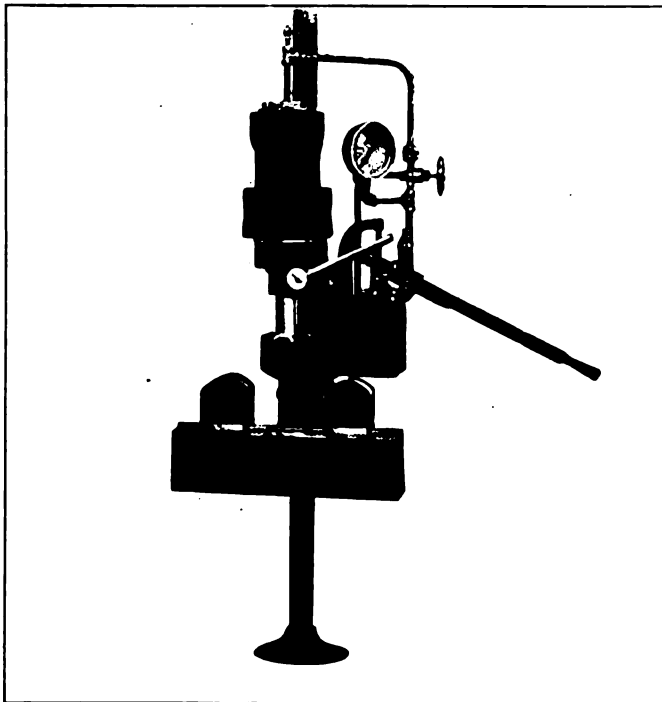
Hand-Operated Hydraulic Pipe Bender
