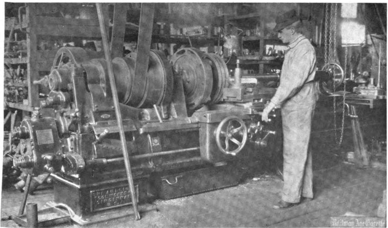
Job:—Finishing complete a cast-iron piston. Size:—See drawing below. Time:—Including two settings, 1½ hour. Operations:—Face both ends, removing an average of ½ inch of metal. Bore for rod fit. Turn down and finish outside of piston, and cut grooves for packing rings.
