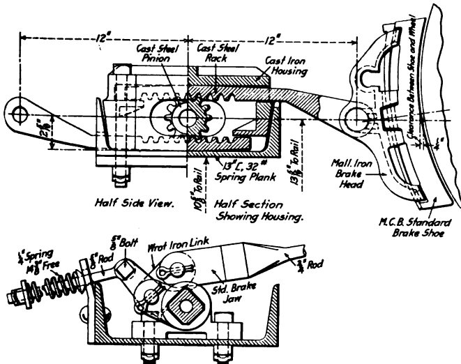
Fig. 2—Section Through the Berdan Brake Rigging
