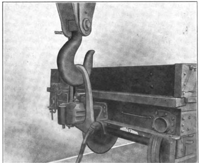
Wrecker Yoke In Operation
