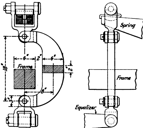
Fig. 12—Another Spring Hanger Suggestion
