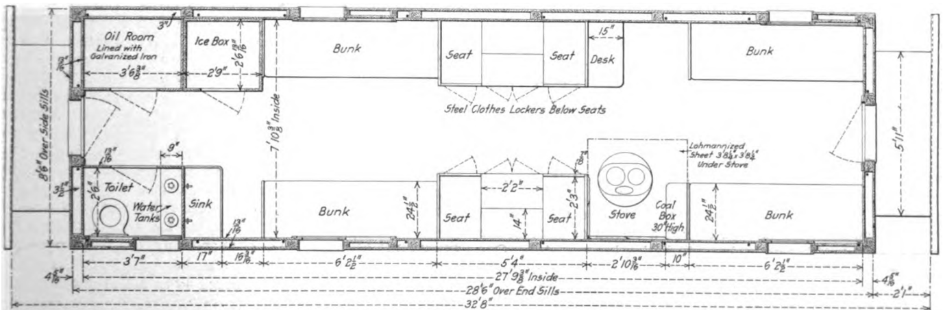
Floor Plan of the Erie Caboose
