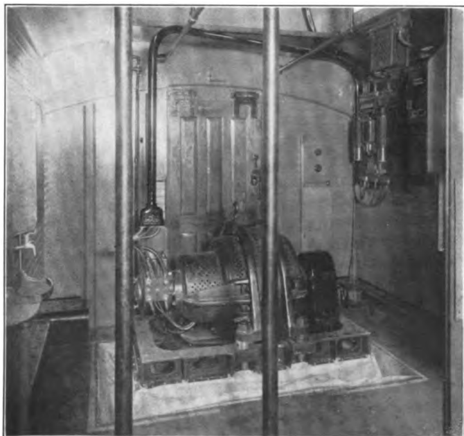
Axle Train Lighter In Northern Pacific Mail and Express Car
