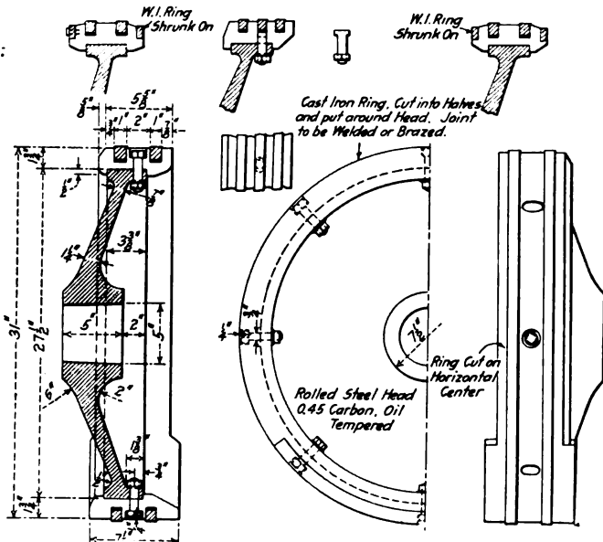
Fig. 20—Burlington Piston Redesigned
