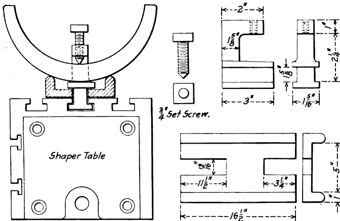
Jig for Holding Crown Brasses on the Shaper
