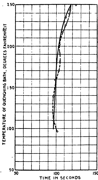
Fig. 8—Quenching Power of New Extra-Bleached Fish Oil
