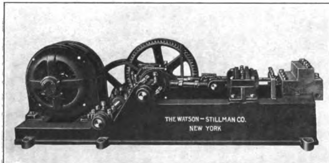
Motor-Driven Hydraulic Pump
