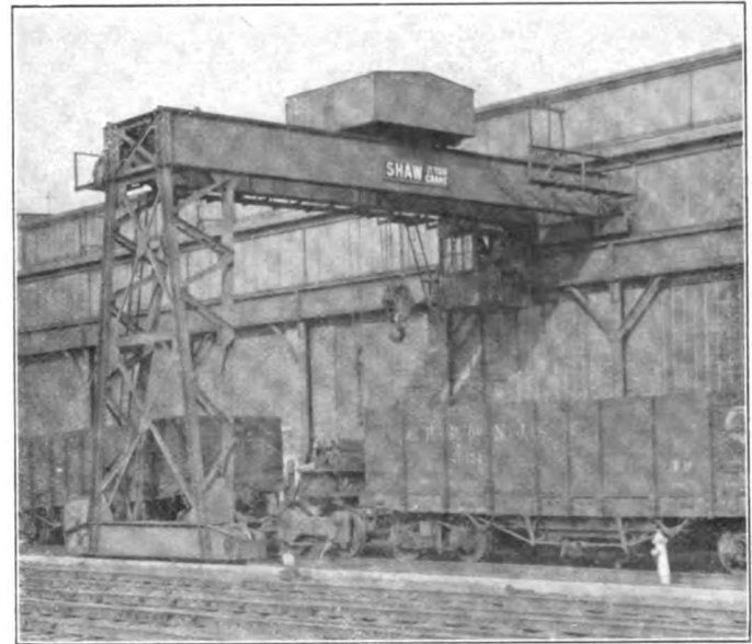
Gantry Crane over Heavy Material Storage
