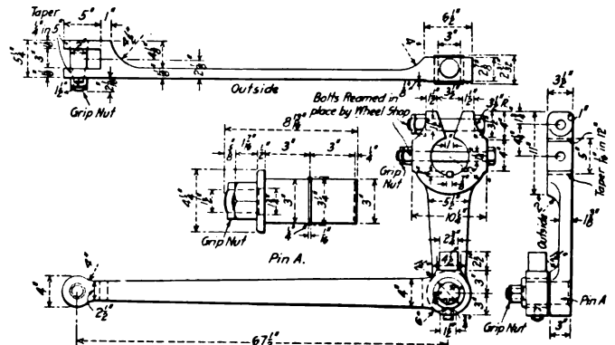
Fig. 28—Eccentric Crank and Rod of Burlington Locomotive
