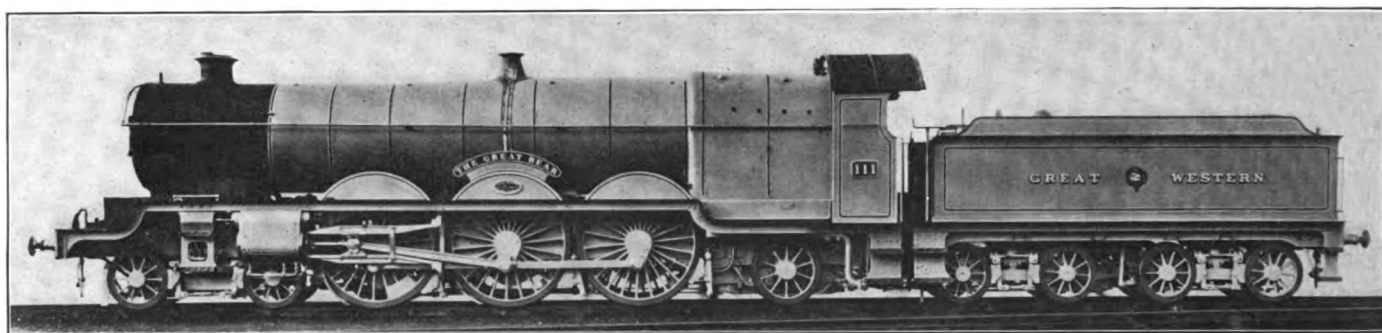
Four-Cylinder Simple Pacific Type Locomotive; Great Western of England
