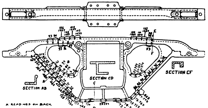
Fig. 1—Truck Frame Design A
