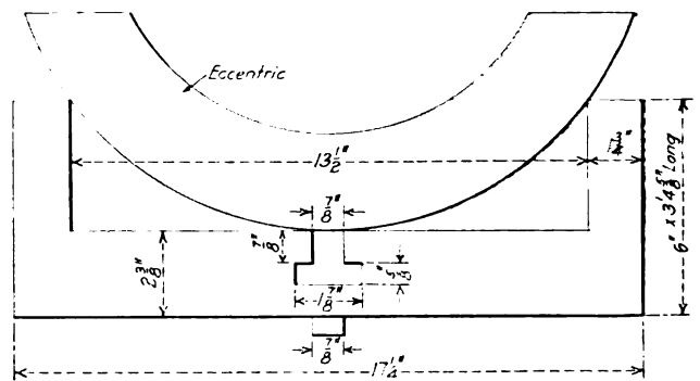
Jig with Eccentric in Place
