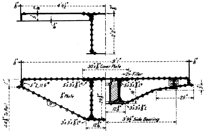
Cross Sections of the Underframe
