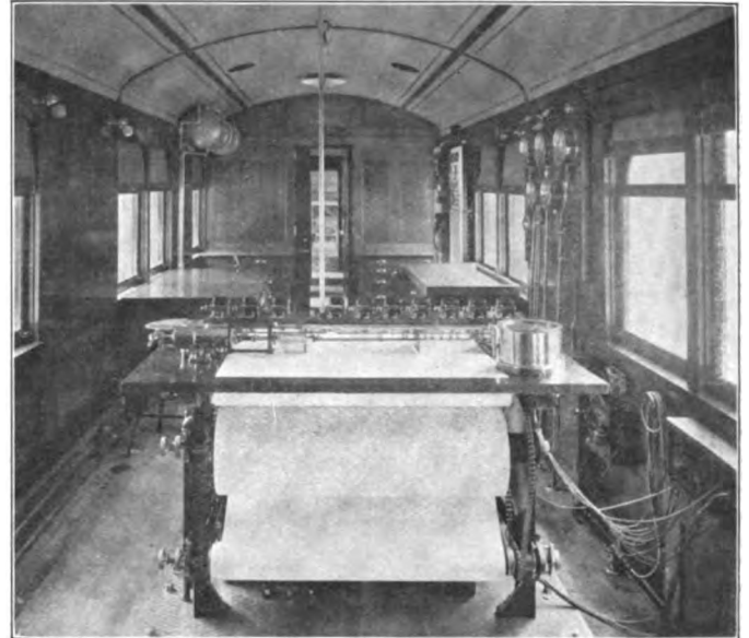
Interior of the Dynamometer Car
