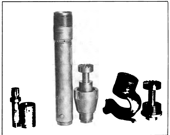
Fig. 13—Tools for Facing Air Hammer Connections
