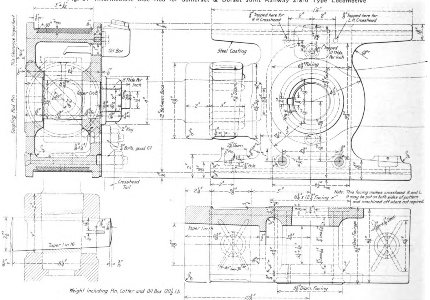
Fig. 55—Crosshead of 2-8-0 Type Locomotive
