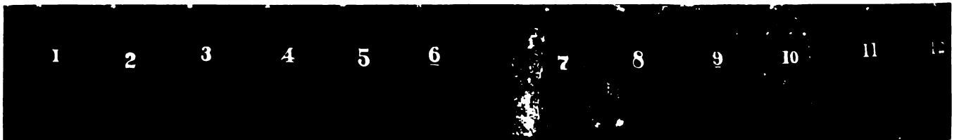
Exhibit B—Exposure Test of Sandblasted Steel Plates Which Were Given Two Coats of Paint and Bolted to Underframe of Locomotive Tender. Nos. 7 to 12 Inclusive Were so Placed that Water from the Tank Dripped on Them
