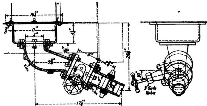
Fig. 5—Outside Tank Valve
