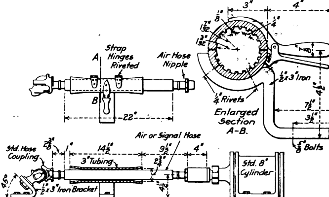
Device for Mounting Air Hose
