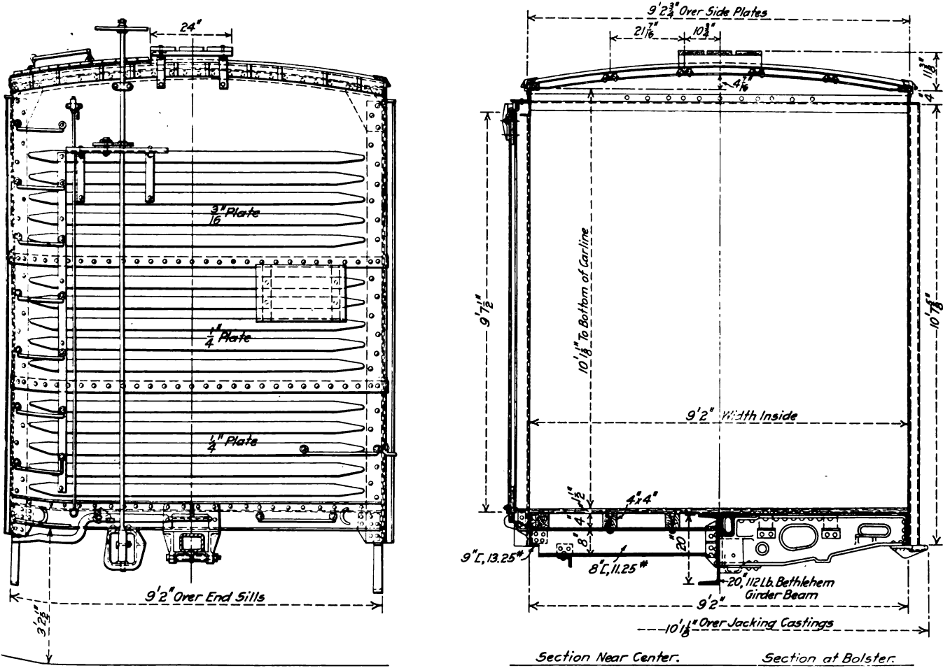
End Elevation and Cross Sections of the Automobile Car
