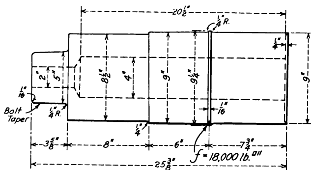
Fig. 27—Main Crank Pin of Burlington Locomotive
