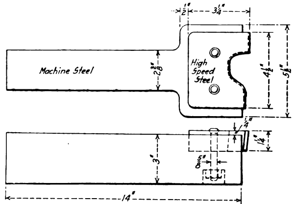
Flanging Tool for Light Wheel Lathes
