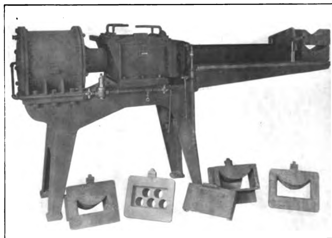
Press for Forming Driving Box Grease Cakes
