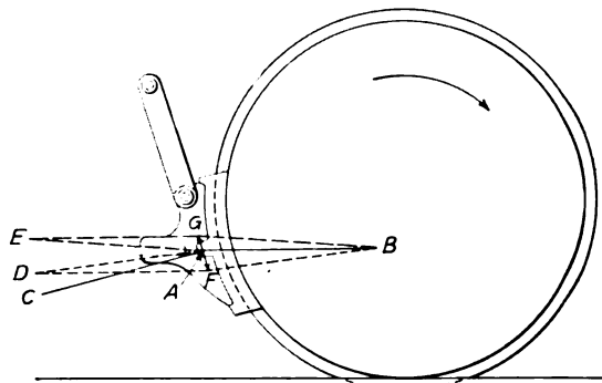
Diagram illustrating the Stress in Brake Hangers
