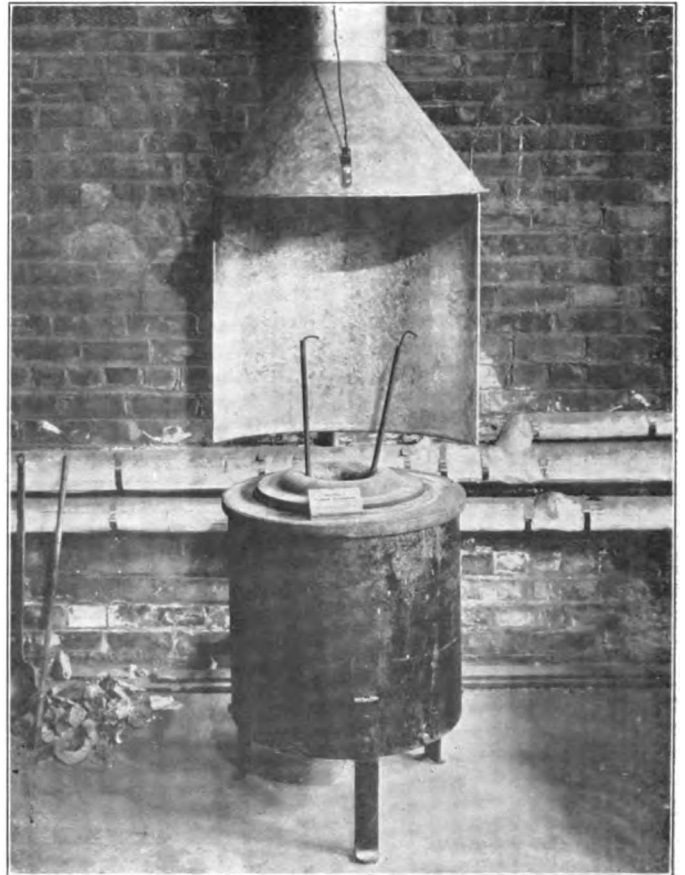
Method of Temperature Indication in Metal or Salt Bath Furnace
