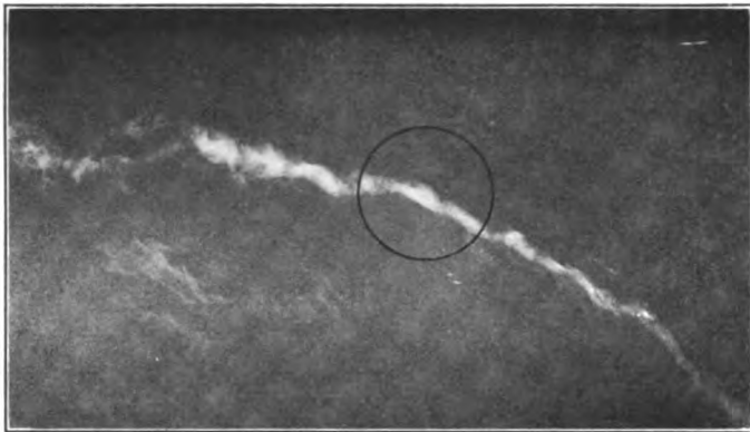
Fig. 1—Radiograph of Steel Casting Showing a Blow Hole Below the Surface. The Circle Shows Where the Button Was Removed
