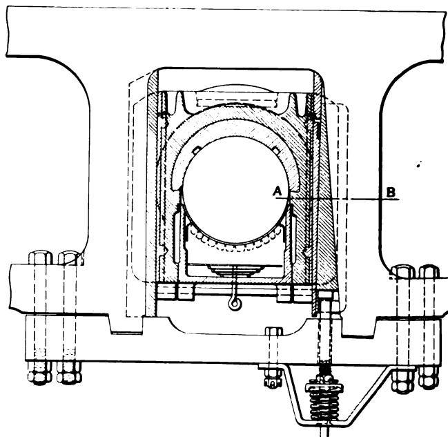
Franklin Automatic Adjustable Wedge
