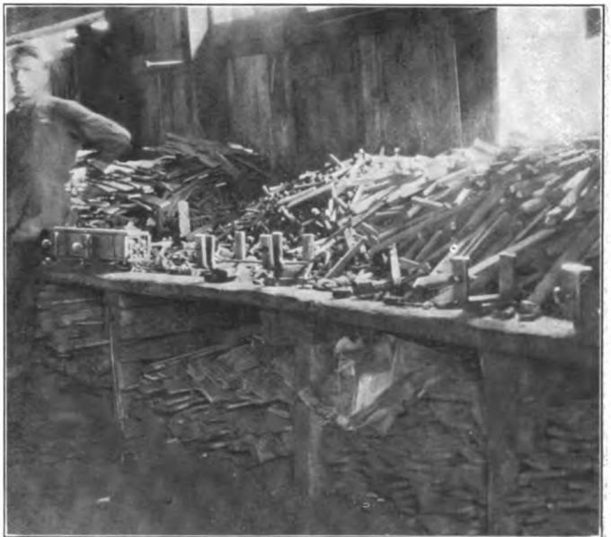
Fig. 3—Piling Bench at St. Cloud Rolling Mill
