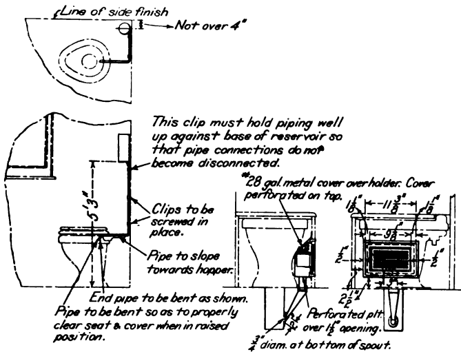
Arrangement of Disinfectant Holders in Passenger Cars
