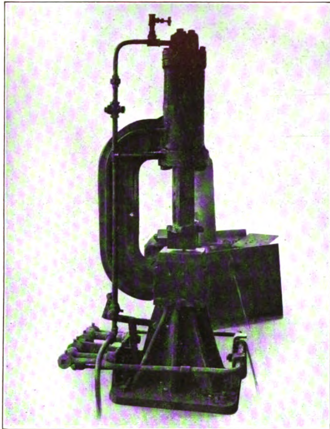
Pneumatic Hammer Used in Reclaiming Track Spikes
