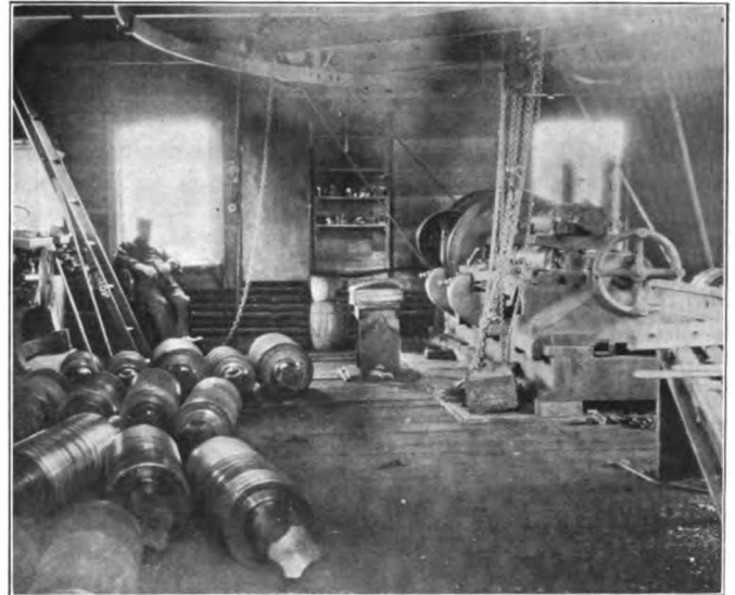
Fig. 6—Shop for Maintaining the Mill Rolls
