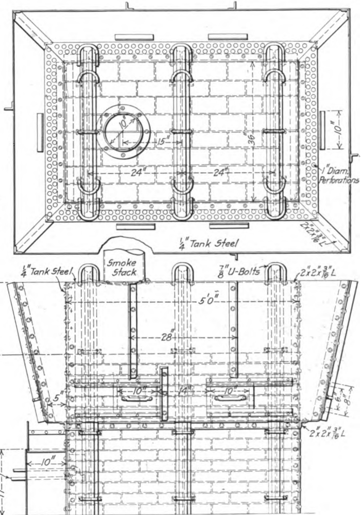
Steel Sand Drier Which Uses Fuel Oil
