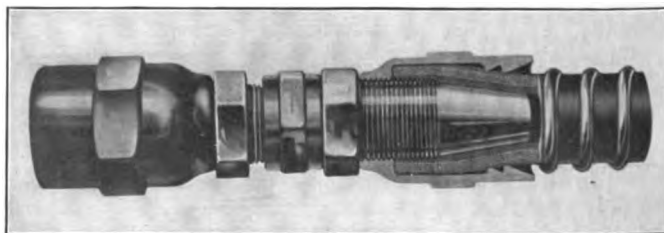
Sectional View of the National Hose Coupling
