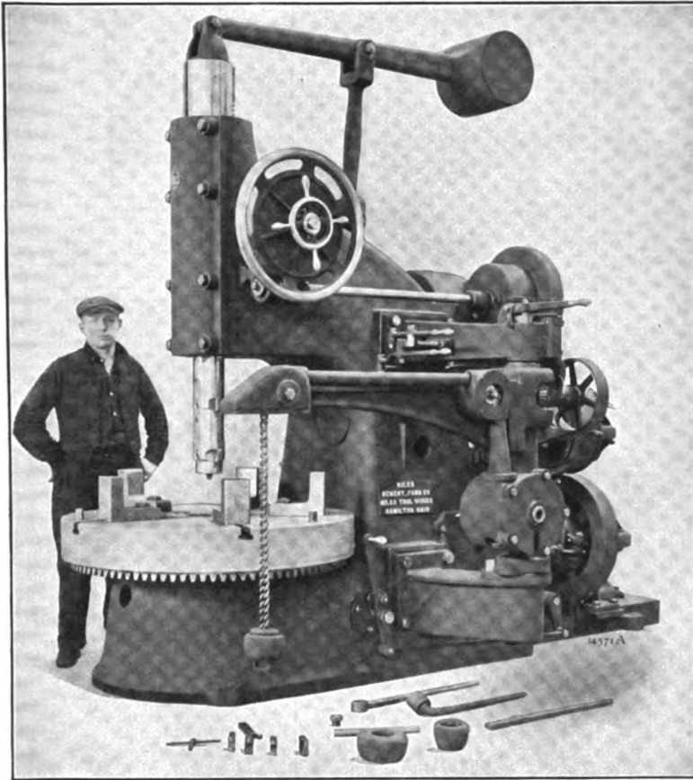
48 inch 1915 Design Car Wheel Borer
