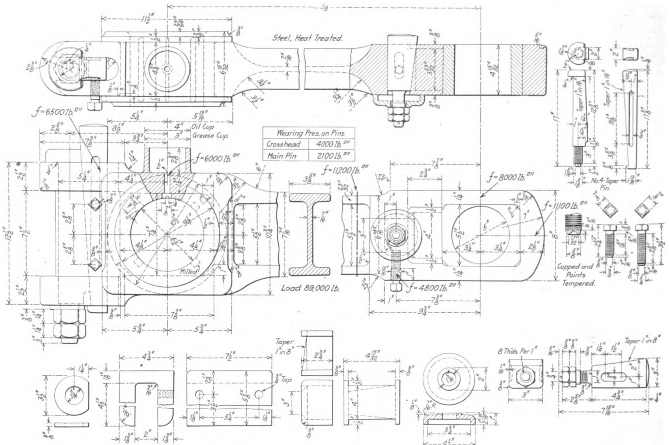
Fig. 6—Main Rod of Pennsylvania Atlantic Type Locomotive
