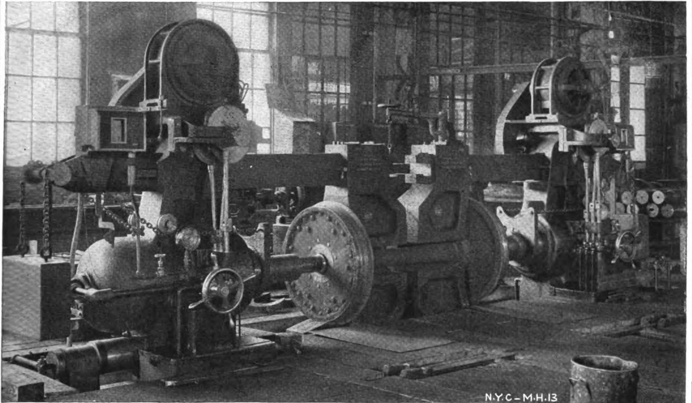
Showing machine in operation at the Mott Haven shops of the New York Central Railroad: Pressing off Wheels.
