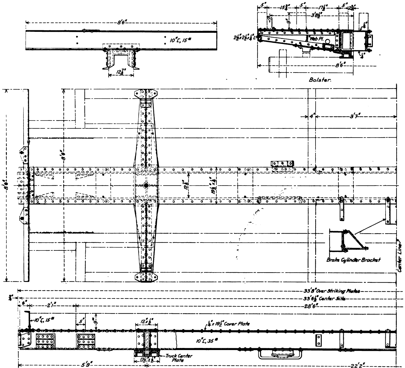
Arrangement of the Steel Members of the Caboose Underframe
