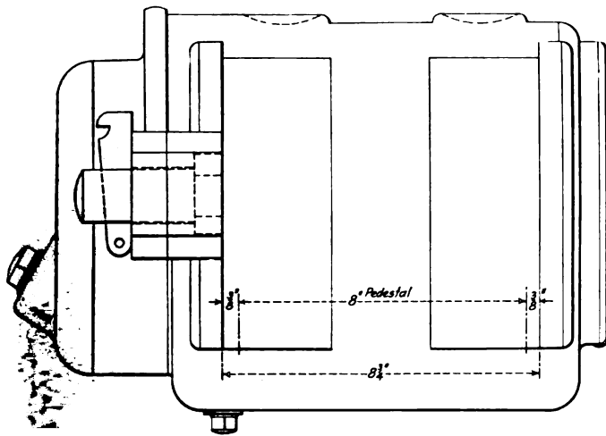
Side Elevation of Roller Bearing Journal Box
