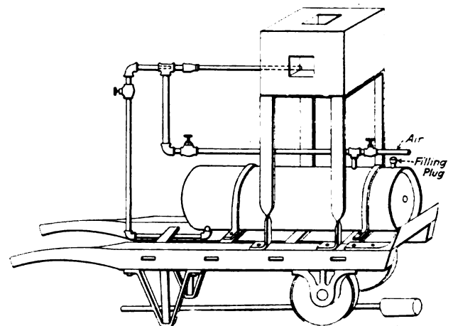
Portable Forge and Blow Torch for Use in Roundhouse
