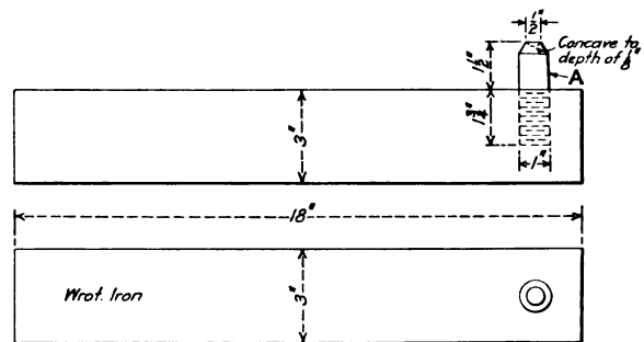
Drilling Jig for Renewing Dry Pipe Collars
