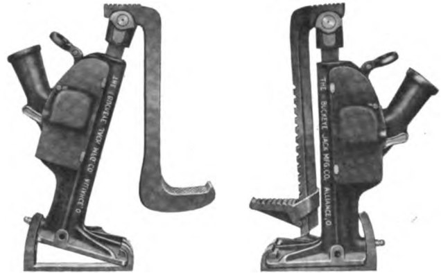
Jacks with Adjustable Heel Plates
