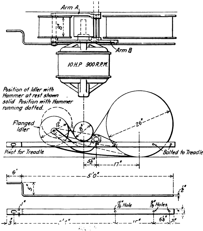
Method of Operation and Details of Motor Drive for Helve Hammer
