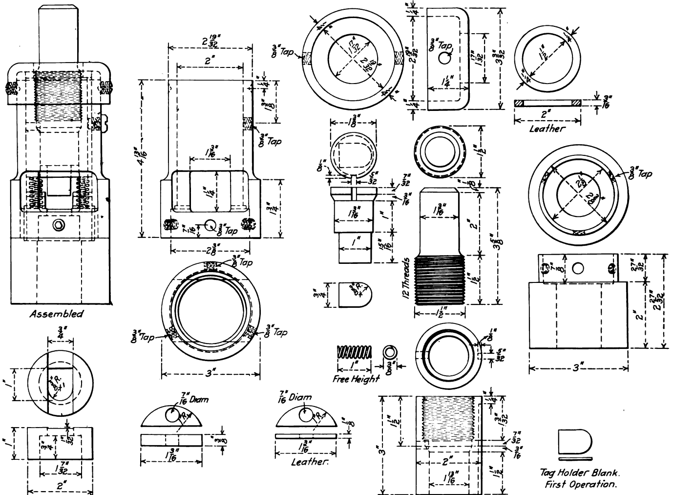
Fig. 5—Punch for Cutting Tag Holder Blanks
