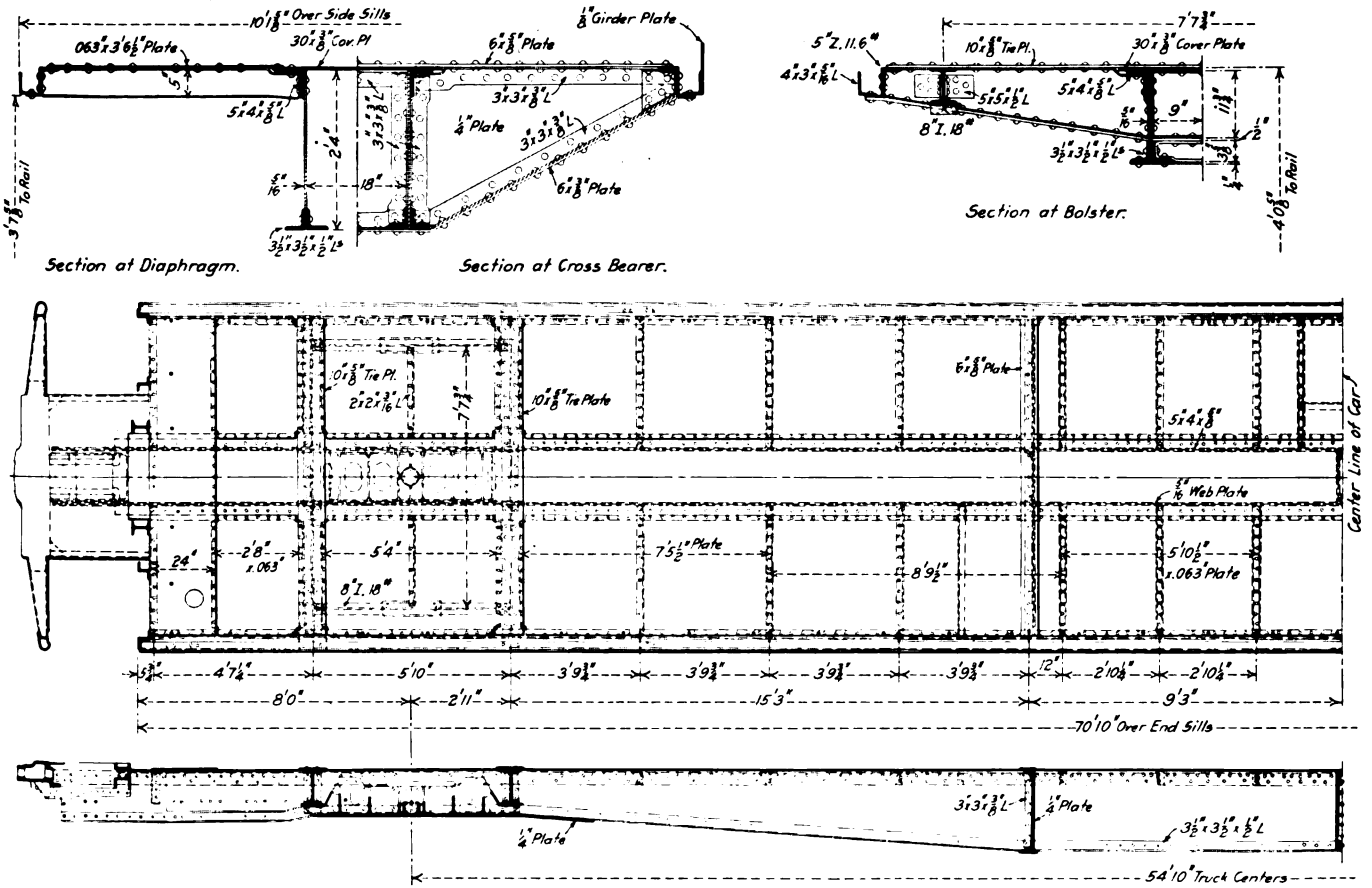
Underframe Construction of Northern Pacific Passenger Cars
