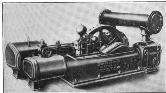
Air Compressor with Piston Valves and Automatic Cut-Off Valves
