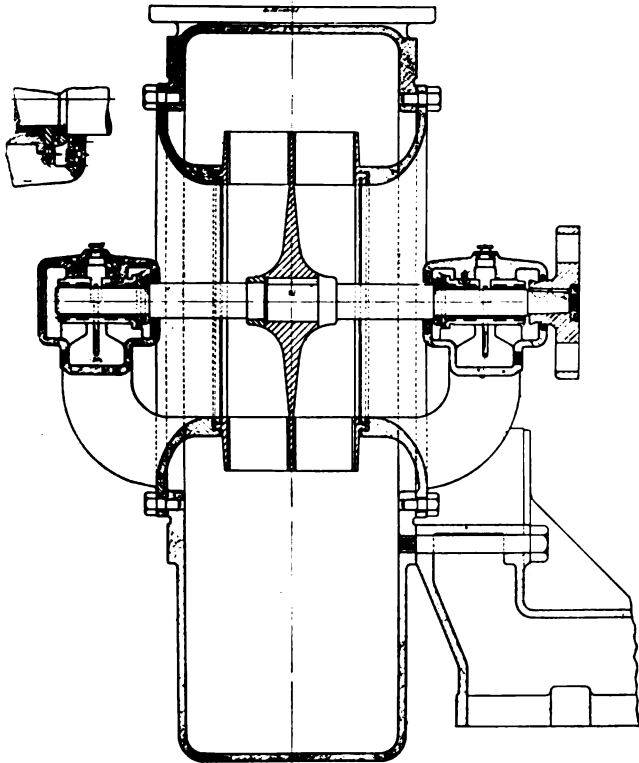
Sectional View of a Single Stage Double Suction Blower
