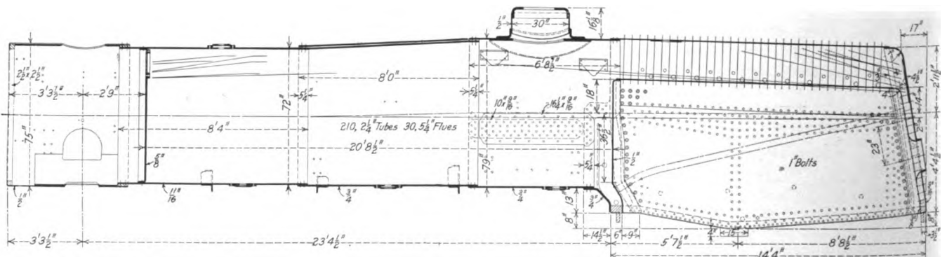
Longitudinal Section of the Boiler of Engine 2900
