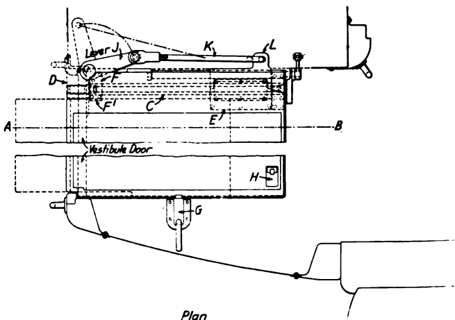
Arrangement of Sickles Extensible Trap Door
