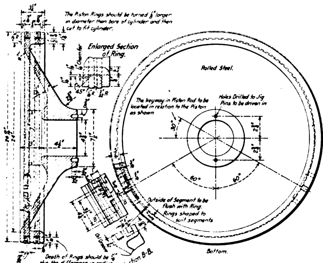
Fig. 8—Piston of Pennsylvania Pacific Type Locomotive
