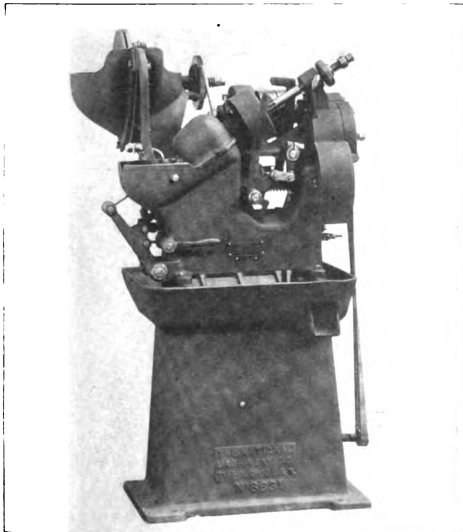
Automatic Nut Tapping Machine in Which a Bent Tap is Used
