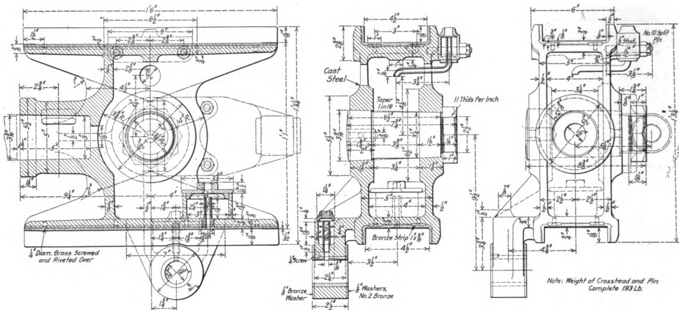
Fig. 35—Inside Crosshead of the Great Western Engine
