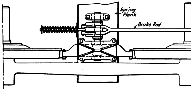
Fig. 1—Top View of the Berdan Brake Rigging
