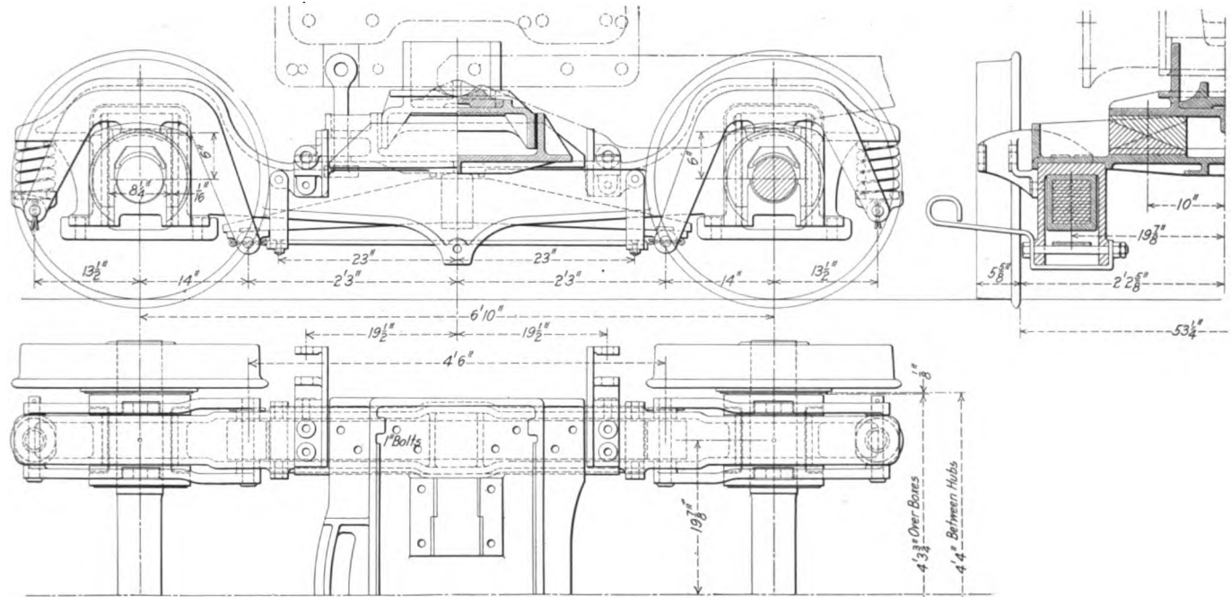
Arrangement of Details of the Leading Truck
