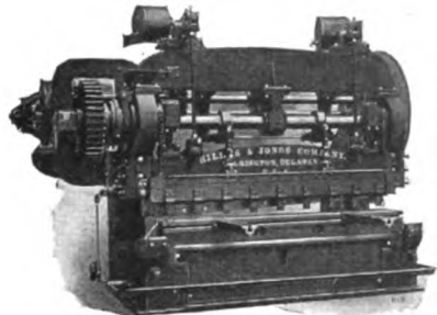
Guillotine Plate Shears. Capacity, 1/4" to 1 1/2". No overhung gearing. Automatic Stop and Hold-down.
