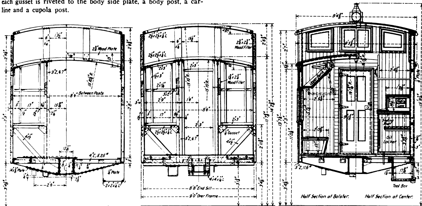
End and Cross-Sectional Elevations Showing the End Frame and Finished Interior of the B. R. & P. Caboose
