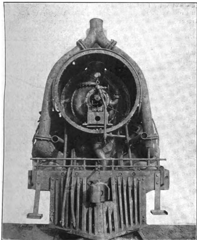
Arrangement of the MacFarland Fan Draft
