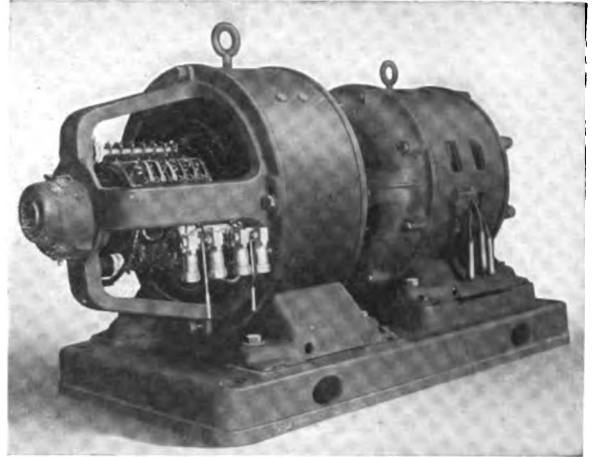
ARC-WELDING MOTOR-GENERATOR SET. CAN BE SUPPLIED FOR OPERATION ON ANY COMMERCIAL POWER CIRCUIT.
