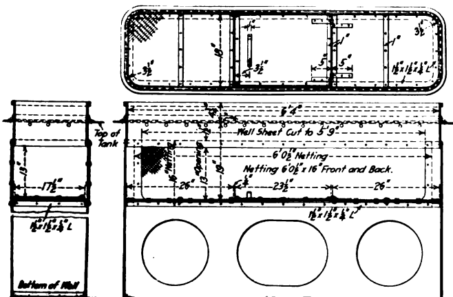
Fig. 3—Long Tank Manhole with Enclosed Well
