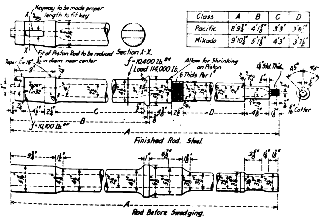
Fig. 9—Piston Rod of Pennsylvania Pacific Type Locomotive
