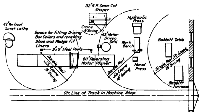
Layout of the Driving-Box Group
