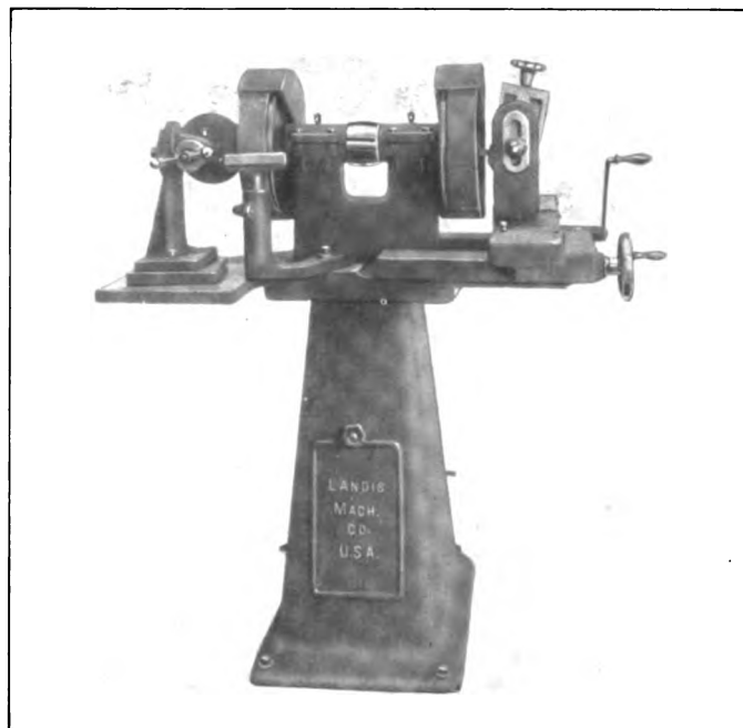
Chaser Grinder and Disc Sharpener for the Cutters of Roller Pipe Cutting Machines
