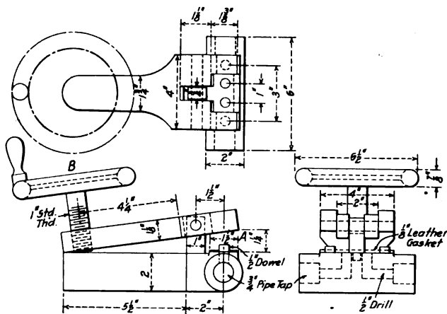
Clamp for Testing Feed and Reducing Valves
