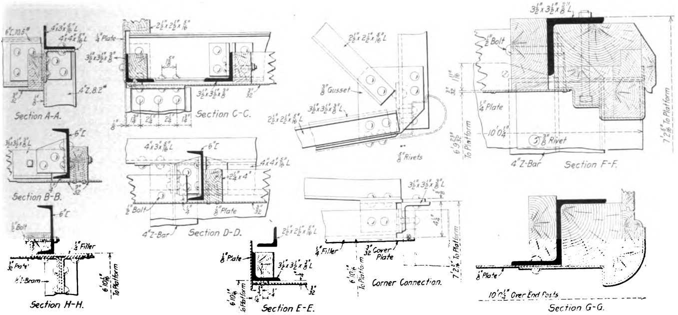
Details of the End Framing; the Section Letters refer to the Drawing of the End Arrangement
