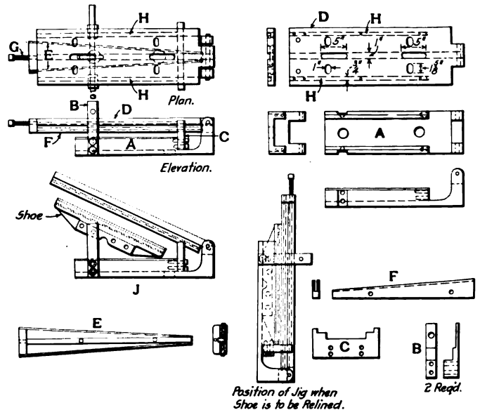
Fig. 6—Jig for Babbitting Crosshead Shoes
