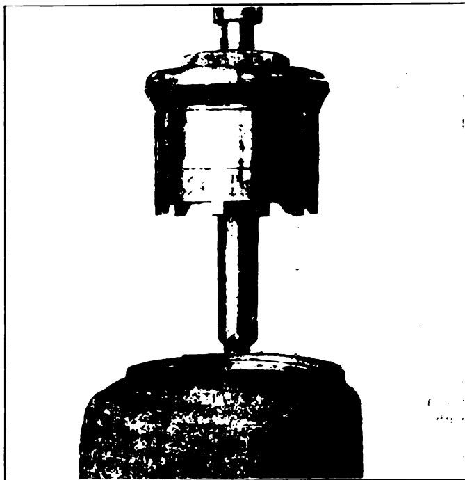
Fig. 9—Reamer for Throttle Valve Seats
