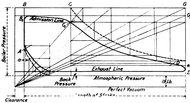
Fig. 5—Locomotive Indicator Card
