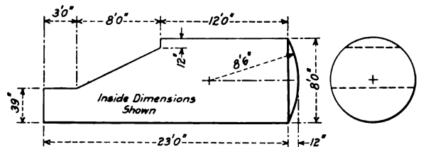
Fig. 1—Water Space Dimensions for a Vanderbilt Tank
