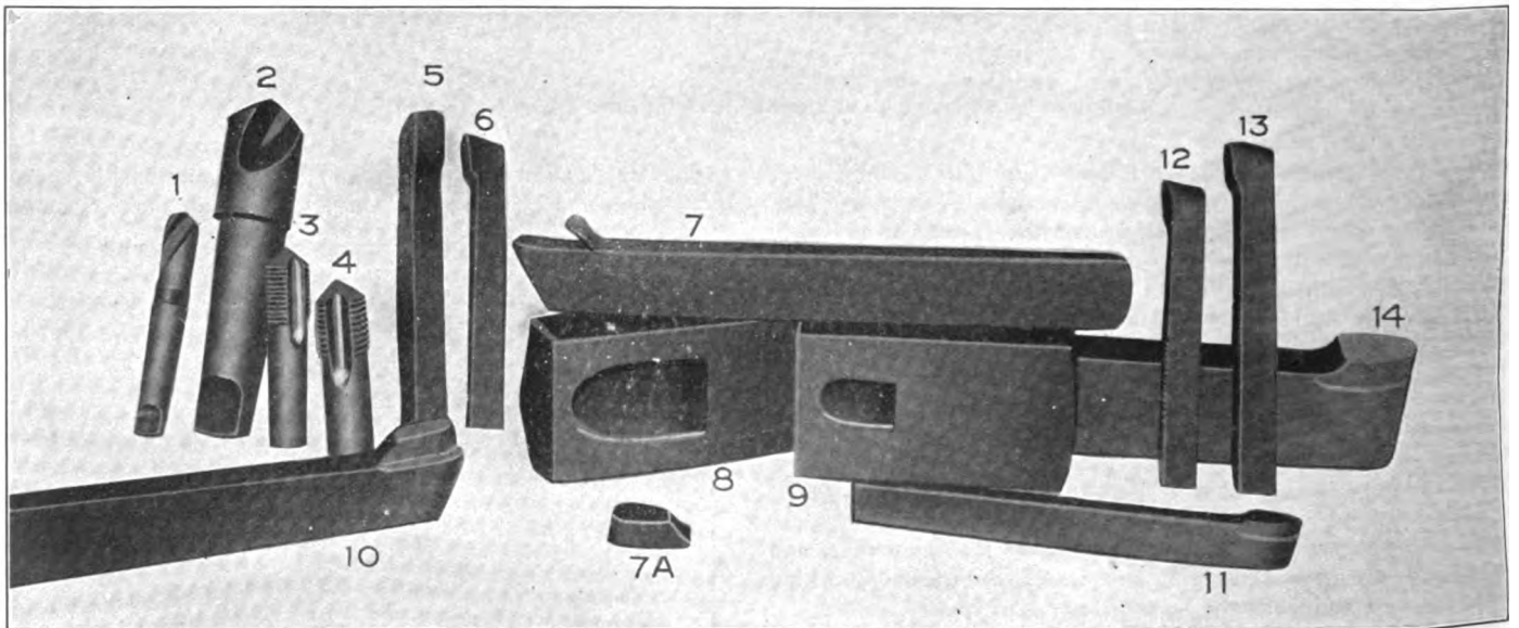
Group of High Speed Steel Tipped Tools with Dies for the Tips and the Tool Shanks
