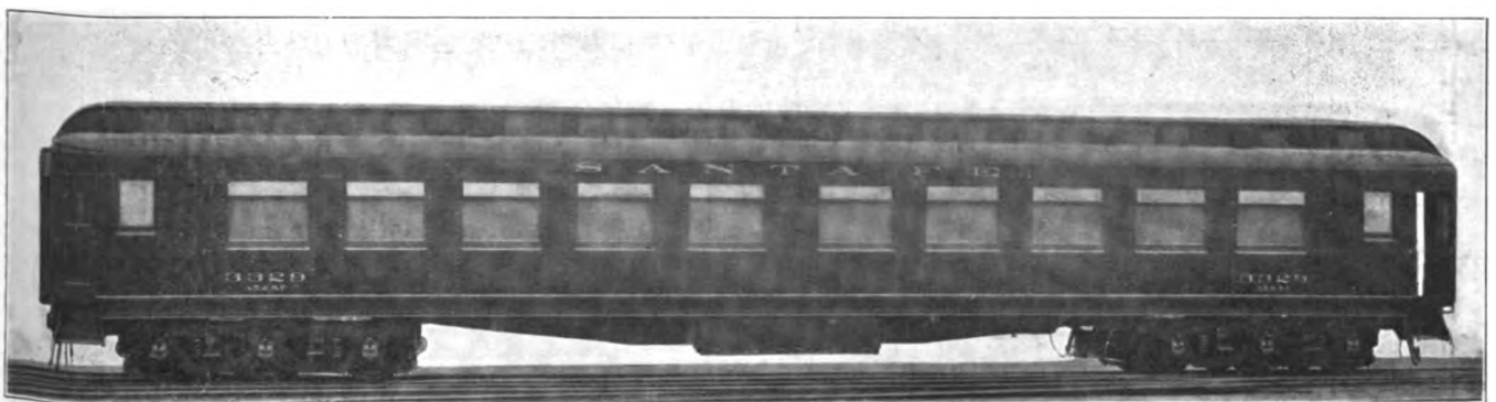
Steel Passenger Equipment for the Atchison, Topeka & Santa Fe
