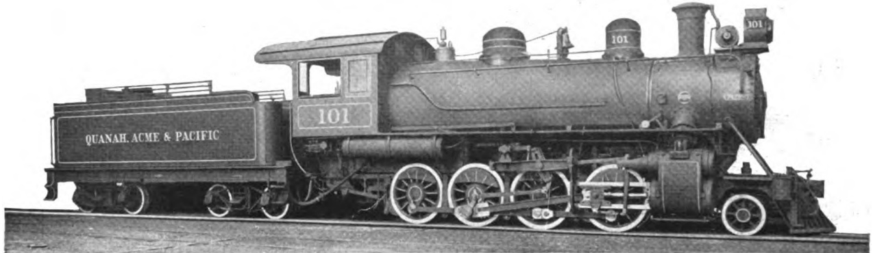
Consolidation Type Locomotive, Quanah, Acme & Pacific Ry. C. H. Sommer, First Vice-President.
