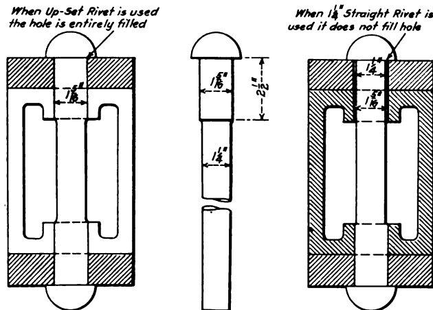
Illustrating the Advantage of Using the Upset Rivet for Fastening the Yoke to the Coupler
