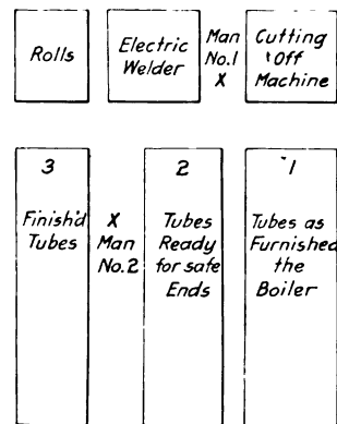
Fig. 2—Grouping of the Equipment
