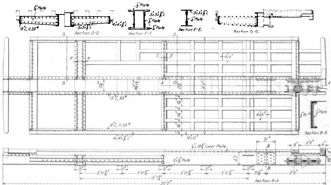
Arrangement of the Underframe Members
