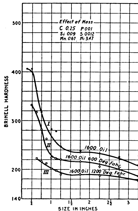
Fig. 13—Effect of Mass Upon Hardness; Nickel Steel Quenched in Oil
