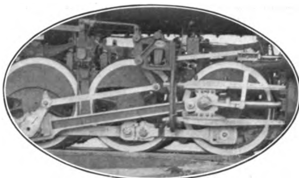
STANDARD BAKER VALVE GEAR FOR SANTÉ FE TYPE LOCOMOTIVES
