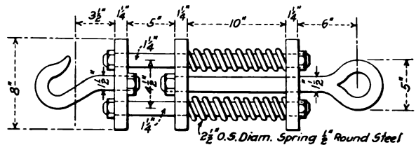
Lifting Hook for Heavy Work
