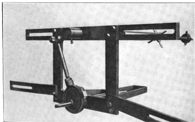
Fig. 8—Jig for Grinding Dry Pipe Joints
