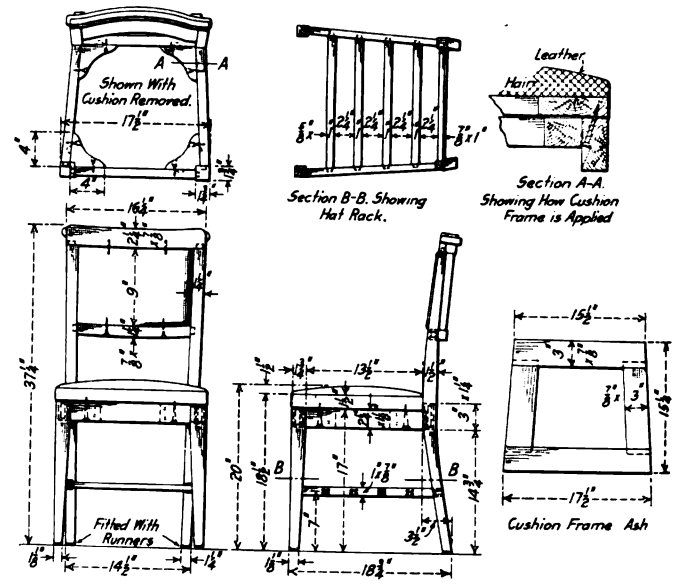
Canadian Northern Dining Car Chair
