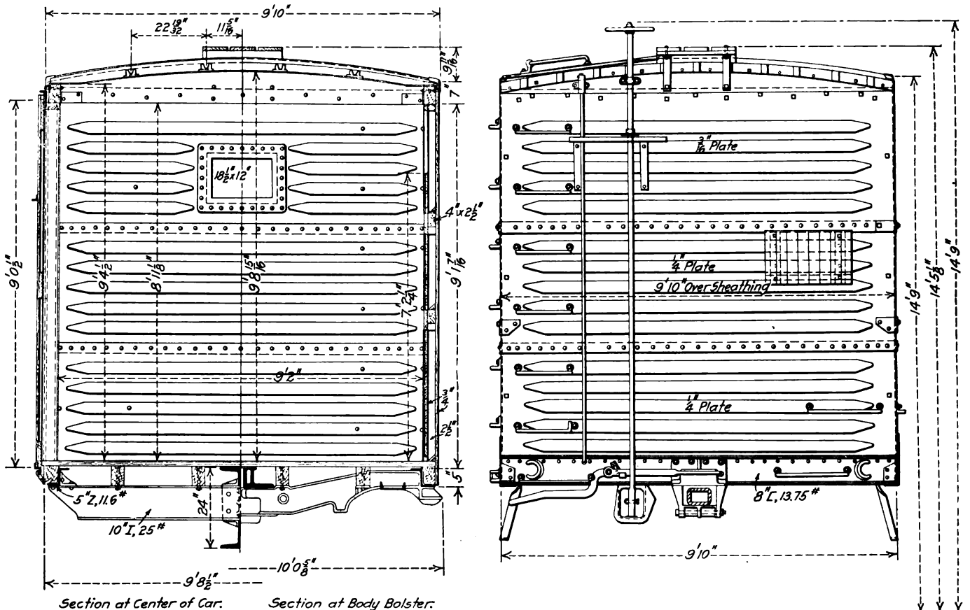
End Elevation and Cross Sections of Union Pacific Steel Underframe Box Car
