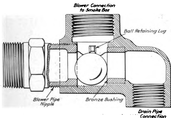
Automatic Drain Valve for Blower Pipe
