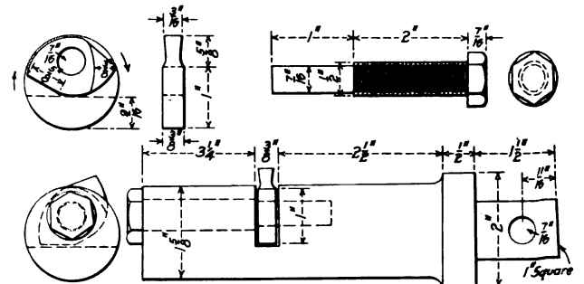
Simple Flue Cutter with Automatic Feed
