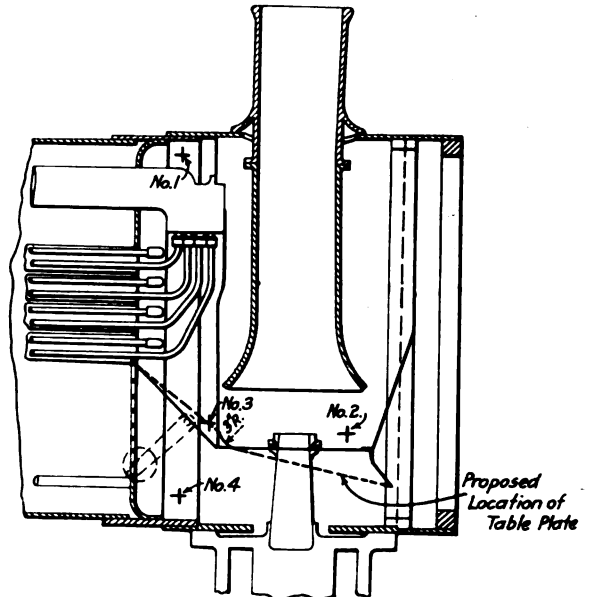
Fig. 1—Draft Readings to Determine Condition of Passages
