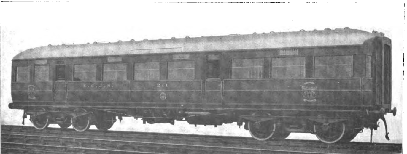
All-Steel Kitchen Car Used on the East Coast Route in England
