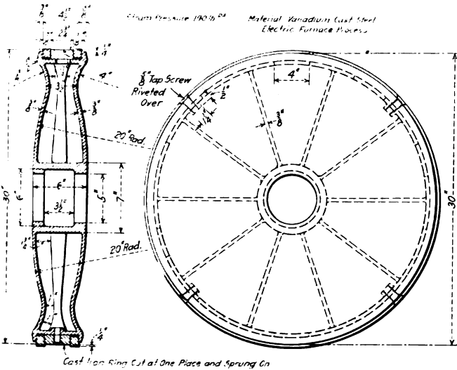
Fig. 23—Hollow Box Type Piston
