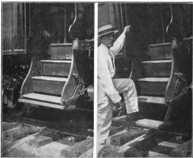
Adjustable Step in Raised and Lowered Positions
