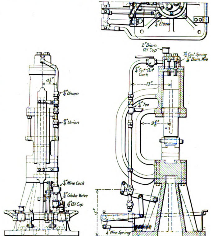
Details of Construction of the Pneumatic Hammer
