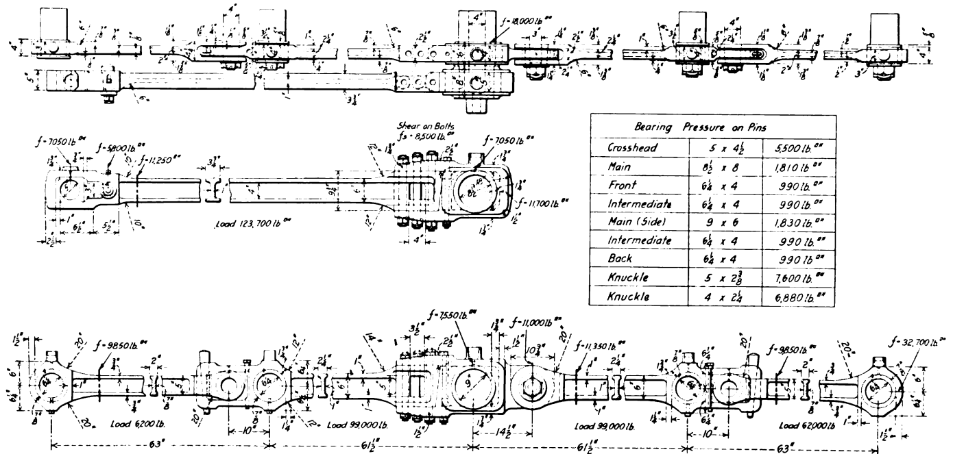
Fig. 26—Connecting Rods of the Burlington Locomotives
