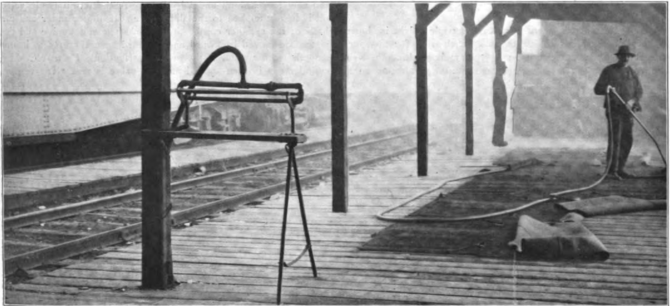
Apparatus Used for Cleaning Carpets by Compressed Air on the Chicago & Western Indiana
