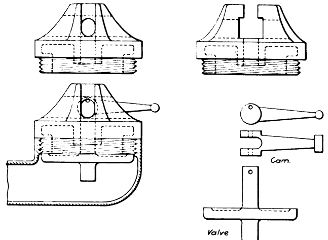
Cam-Operated Relief Valve for Superheater Locomotive
