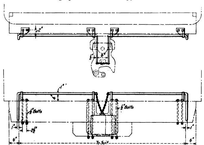
Double Uncoupling Lever for Switch Engines
