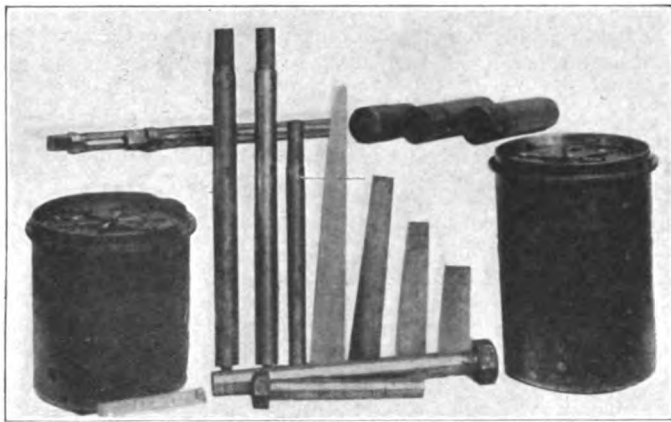
Cutter Heads, Blades and Gages for Adjusting the Heads; Hollow Gages for Testing Turned Bolts
