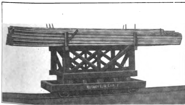
Fig. 6—Rotary Car for Transporting Repaired Tubes to the Erecting Shop
