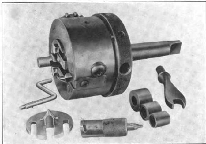
Facing Tool for Drill or Milling Machine
