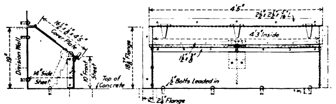
Hot Air Duct Outlet Used in the Erecting Shop
