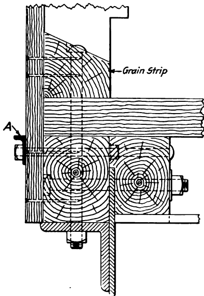
Methods of Preventing Grain Leakage
