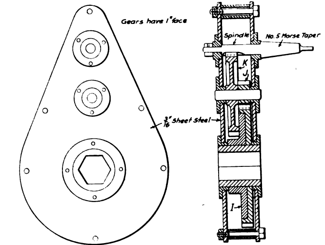
Fig. 3—Gear Train Used in Pulling In Valve Chamber Bushings
