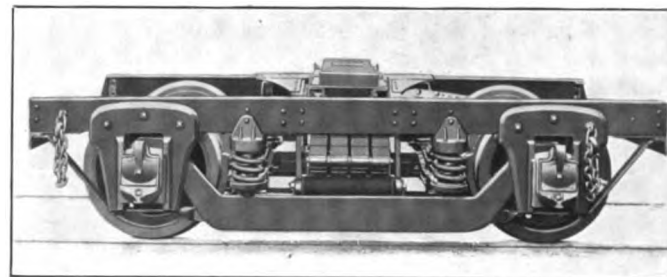
Four-Wheel Truck with Rolled Steel Frame
