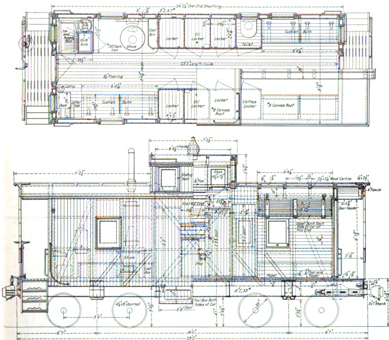
Part-Sectional Views of the Finished Caboose
