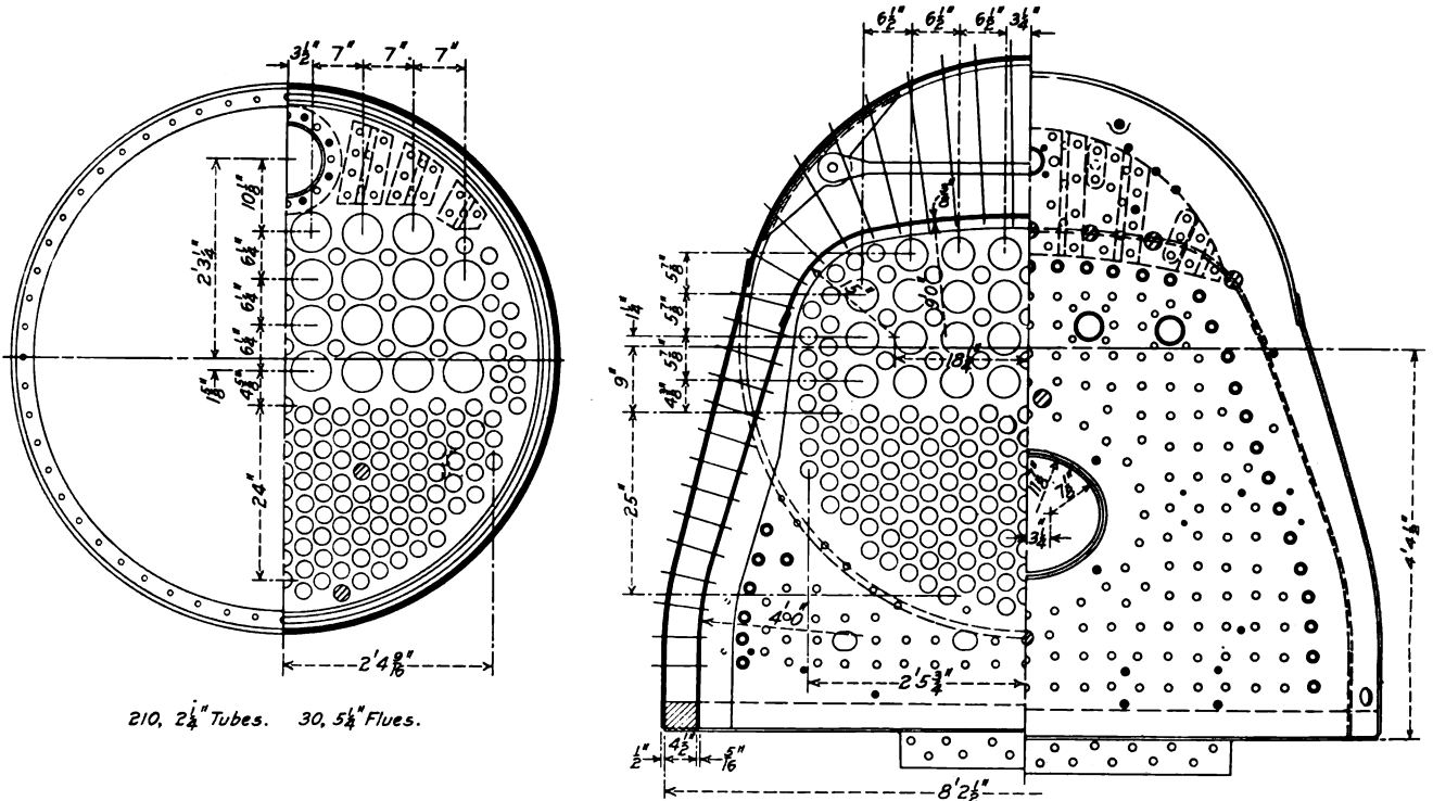
Cross Sections of Boiler of Engine 2900
