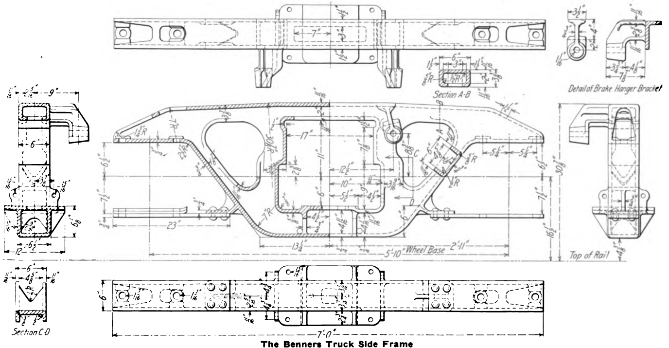
The Benners Truck Side Frame
