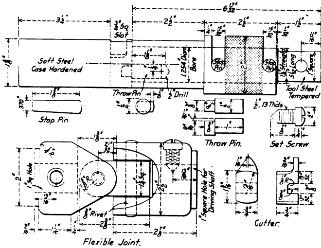
Fig. 1—Flue Cutter Made of Soft Steel Casehardened
