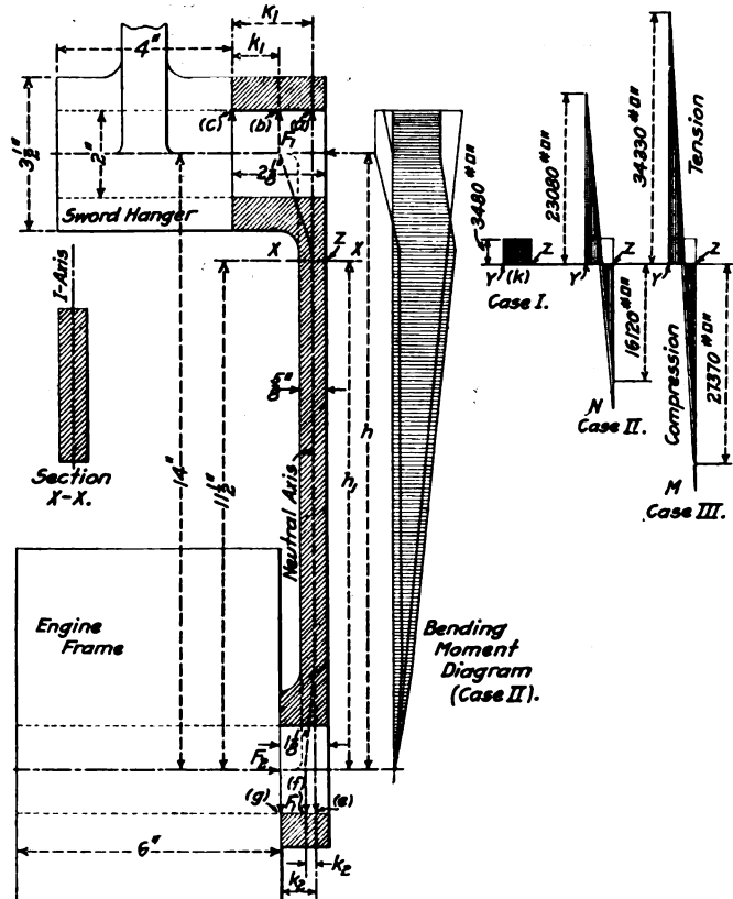
Fig. 4—Diagram of Stresses in Middle Connection Hanger
