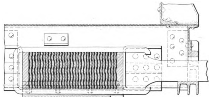
Slick Friction Draft Rigging
