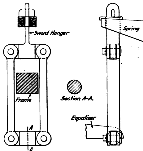
Fig. 11—Suggested Arrangement of Spring Hangers to Provide Flexibility
