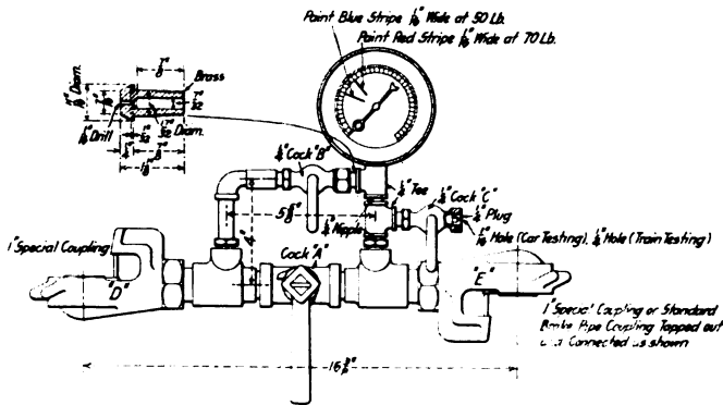
Fig. 1—Arrangement for Testing Air Brakes with Shop Line Pressure
