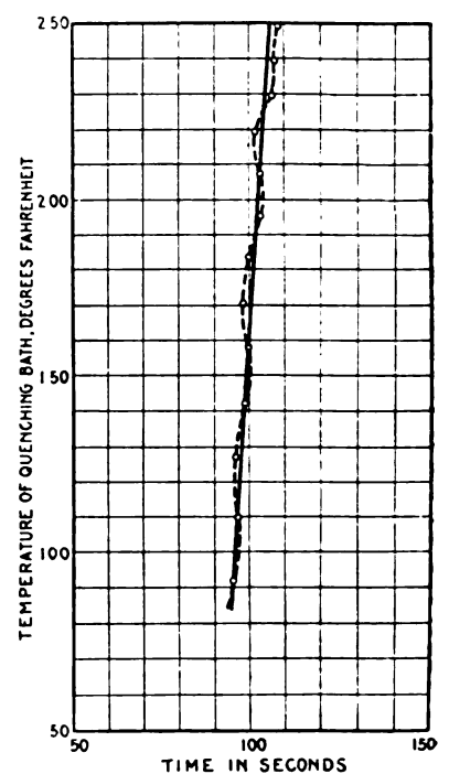
Fig. 6—Quenching Power of Raw Linseed Oil
