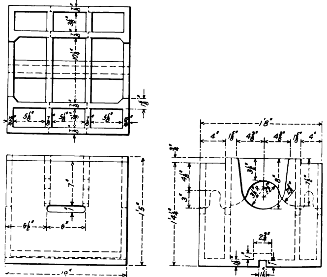
Face Plate Used on Planer for Finishing Driving-Box Shoe and Wedge Faces
