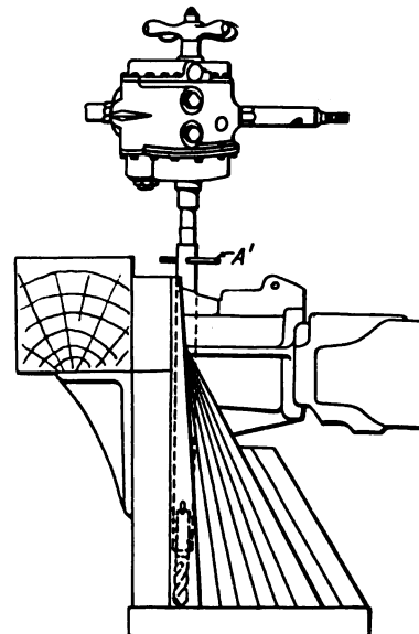
Fig. 4—Using the Drill Extension in Drilling a Pilot Heel Plate position. The motor is then set up and final adjustment made with the feed by turning on the pin A' .
