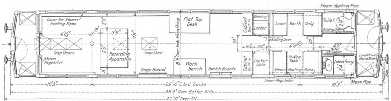
Floor Plan of the Dynamometer Car
