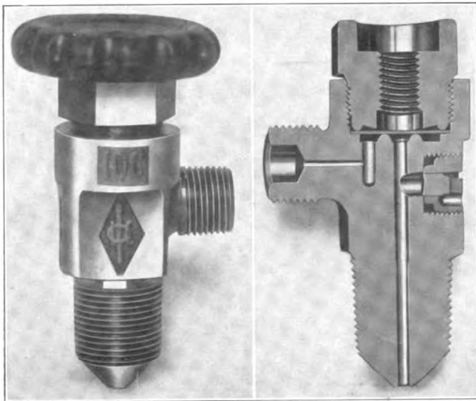
Stud Valve for High Pressure Gas Cylinders
