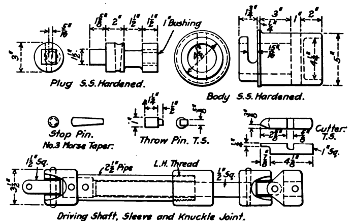
Fig. 2—Superheater Flue Cutter
