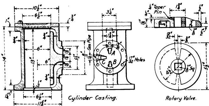
Cylinder and Rotary Valve for Pneumatic Hammer
