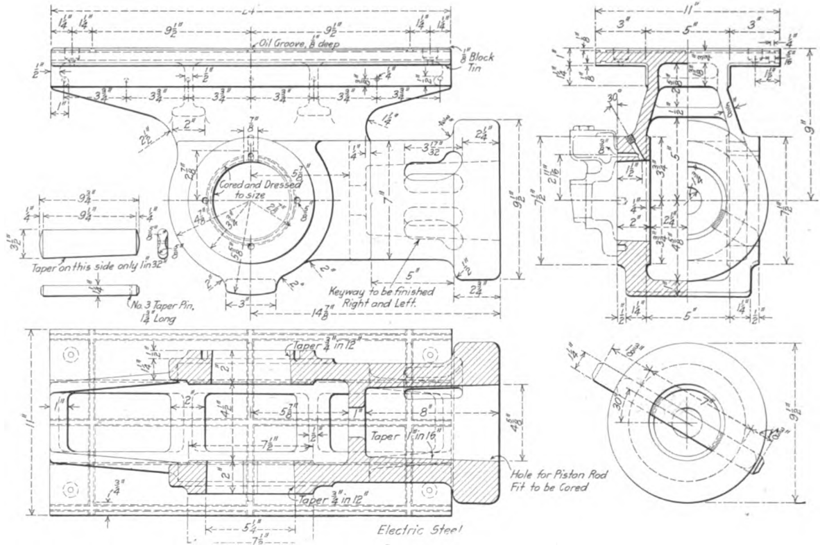
Fig. 5—Crosshead of Pennsylvania Atlantic Type Locomotive
