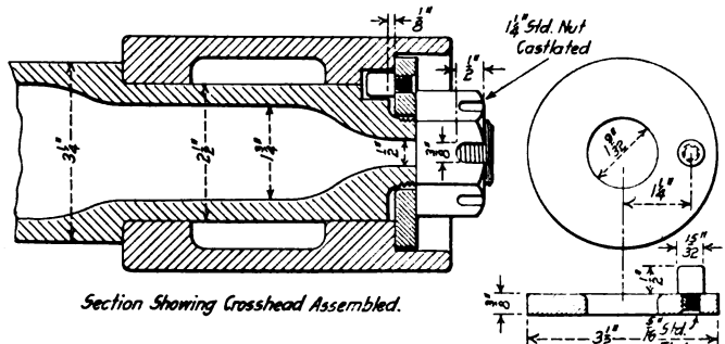
Fig. 9A—Extension Shoe for Piston Rod Shown in Fig. 9
