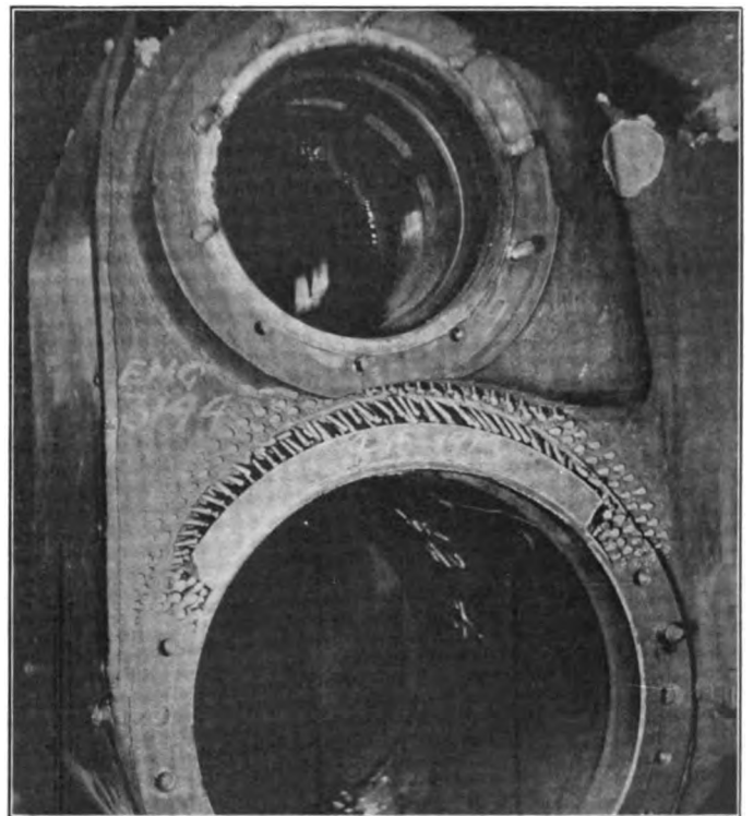
Fig. 9—Cylinder Prepared for Welding
