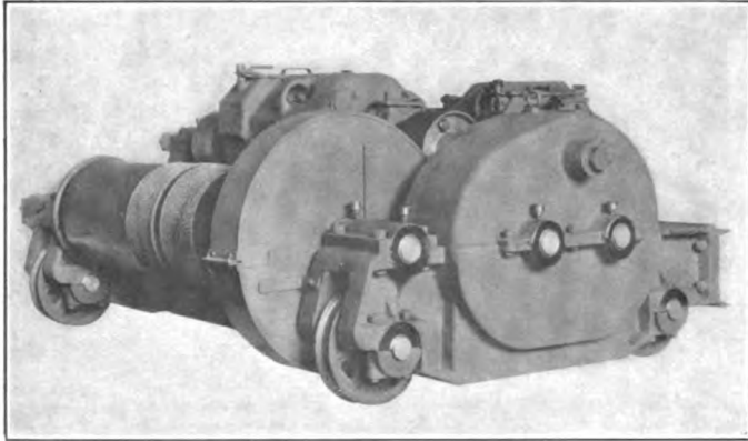
Electric Crane Trolley with Enclosed Gear Cases
