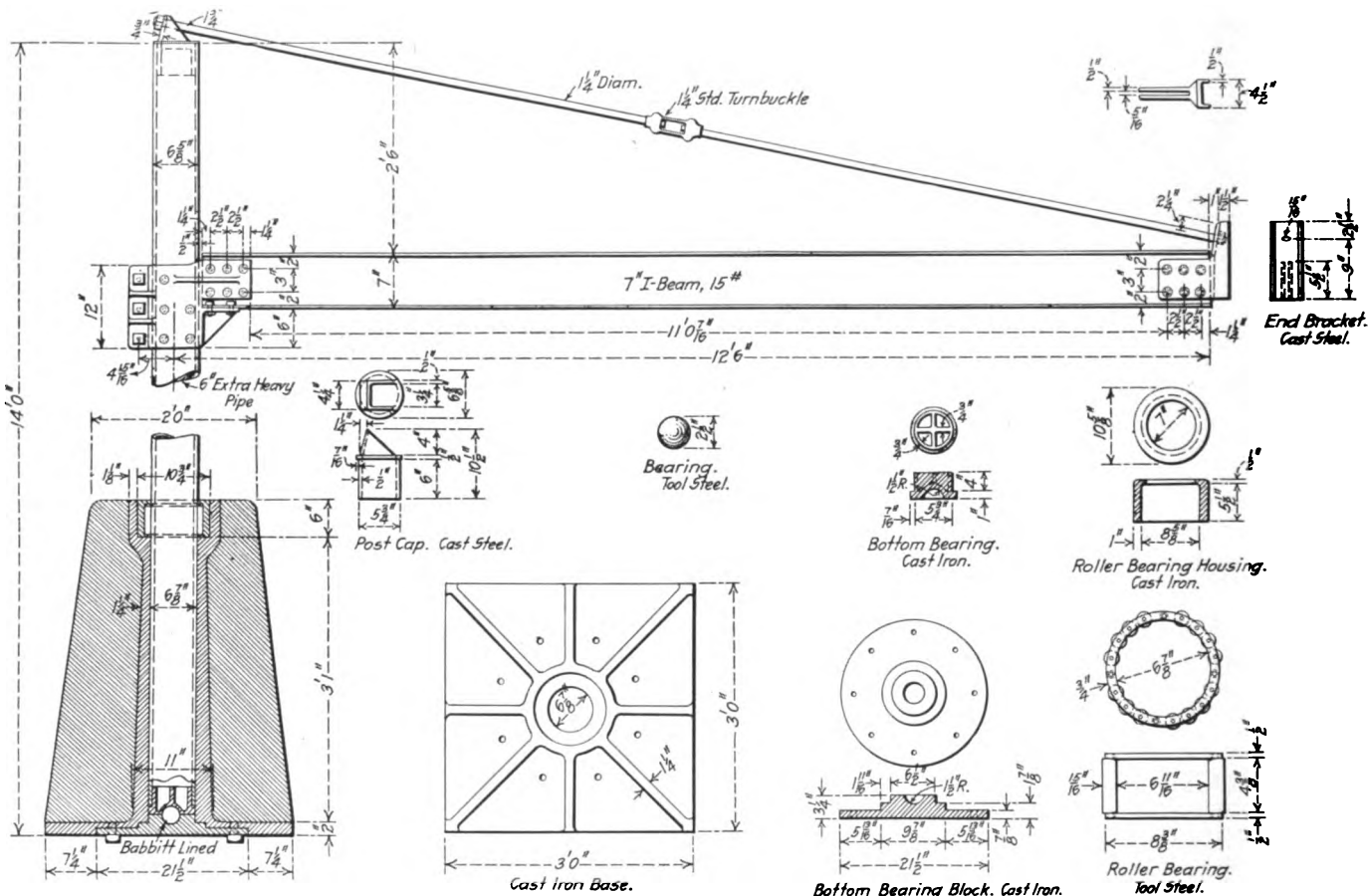
Details of Self-Contained Pillar Crane
