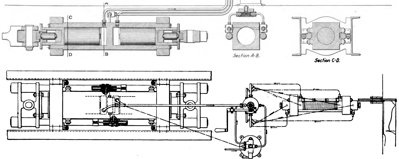
Details of the Dynamometer and Recording Mechanism
