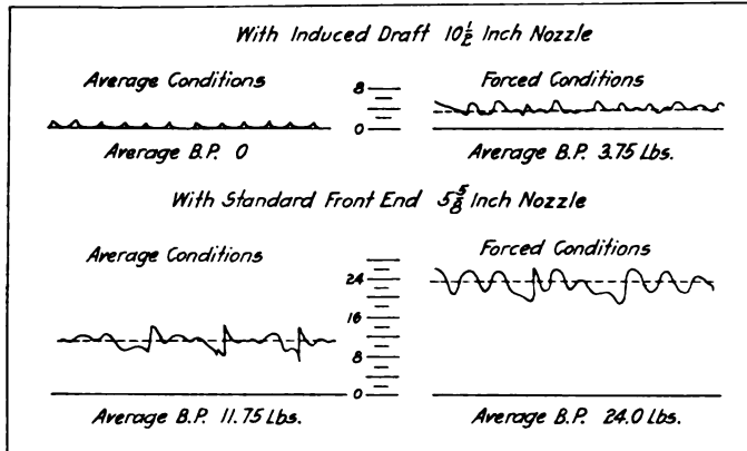
Exhaust Cavity Diagrams
