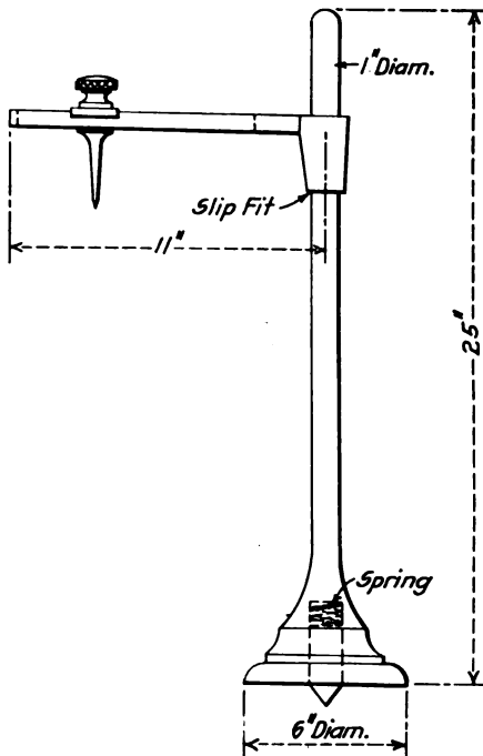
Fig. 4—Tool for Locating Eccentric Cranks
