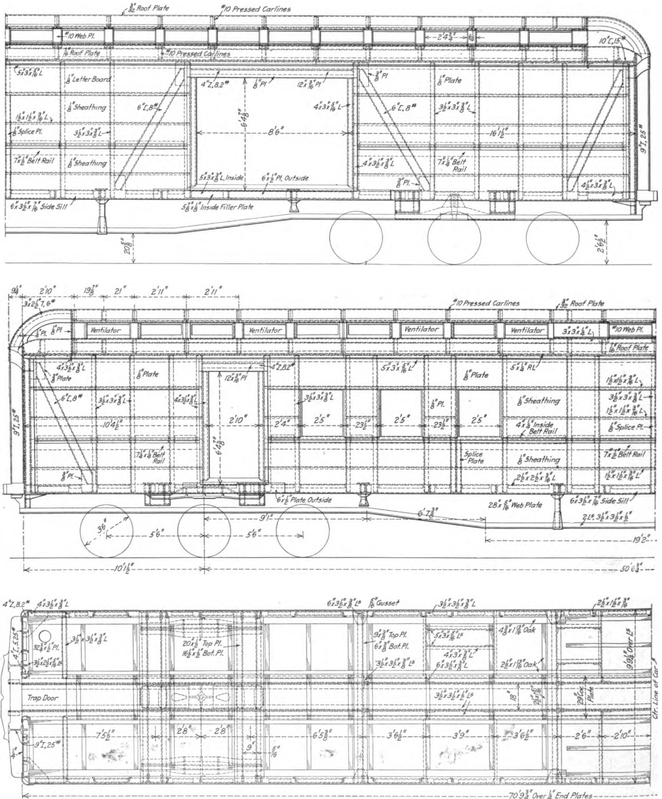
Arrangement of the Members of the Body Frame and Underframing
