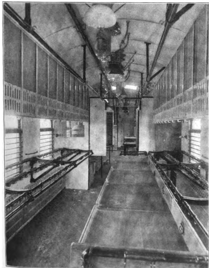
Arrangement of the Interior of the Postal Cars
