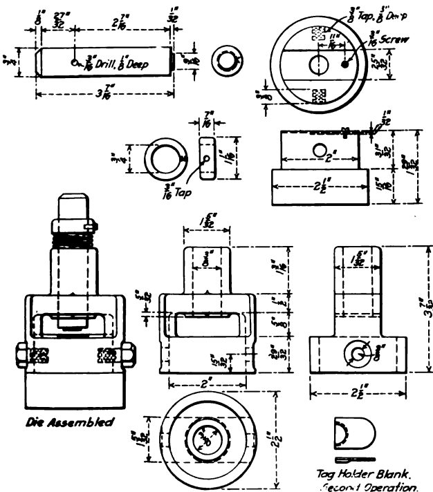
Fig. 2—Dies for Forming Tag Holders
