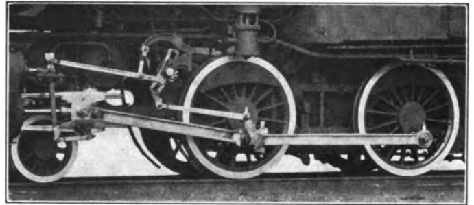
Fig. 30—Running Gear of Philadelphia & Reading, 4-4-0 Type Locomotive
