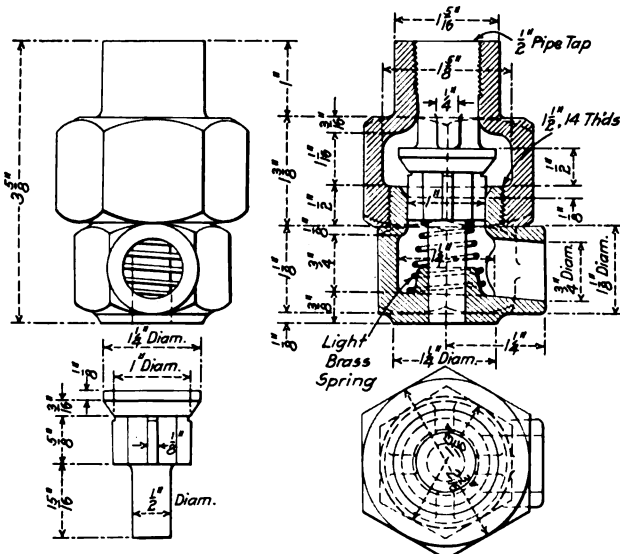
Automatic Drain Valve for Cylinder Exhaust Passages
