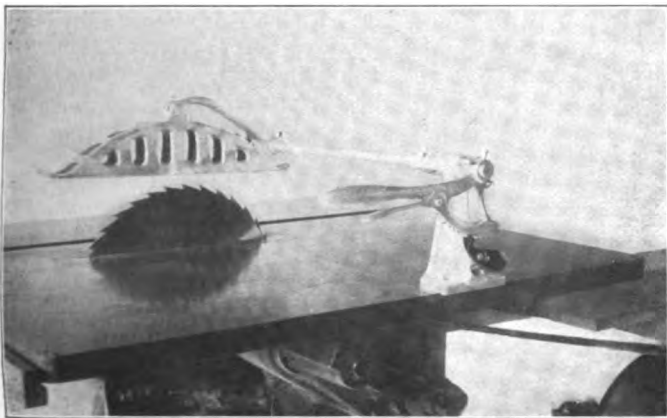
Fig. 2—Saw Guard Partially Raised
