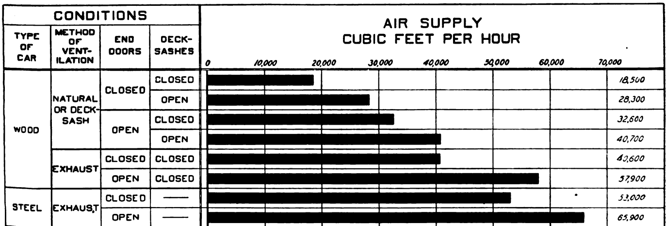
Fig. 1—Methods of Ventilating Sleeping Cars Compared*
