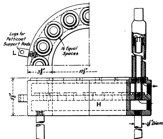
Details of the Feed Water Heater
