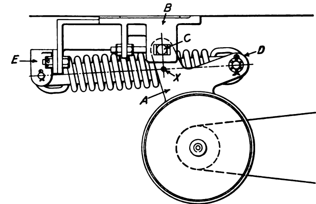
Fig. 3—Position of Generator when Effect of Weight is a Maximum
