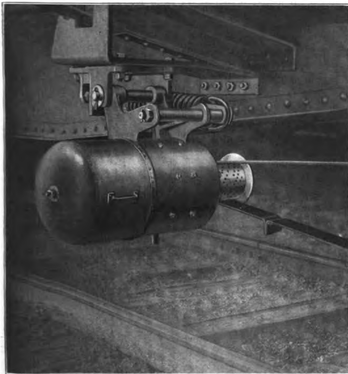
Fig. 1—Car Lighting Generator Suspended from the Underframe
