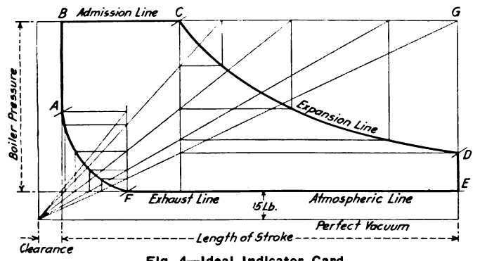
Fig. 4—Ideal Indicator Card
