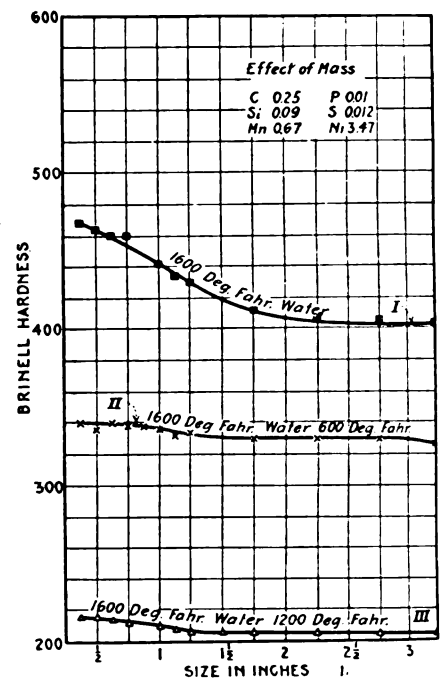
Fig. 12—Nickel Steel Quenched in Water
