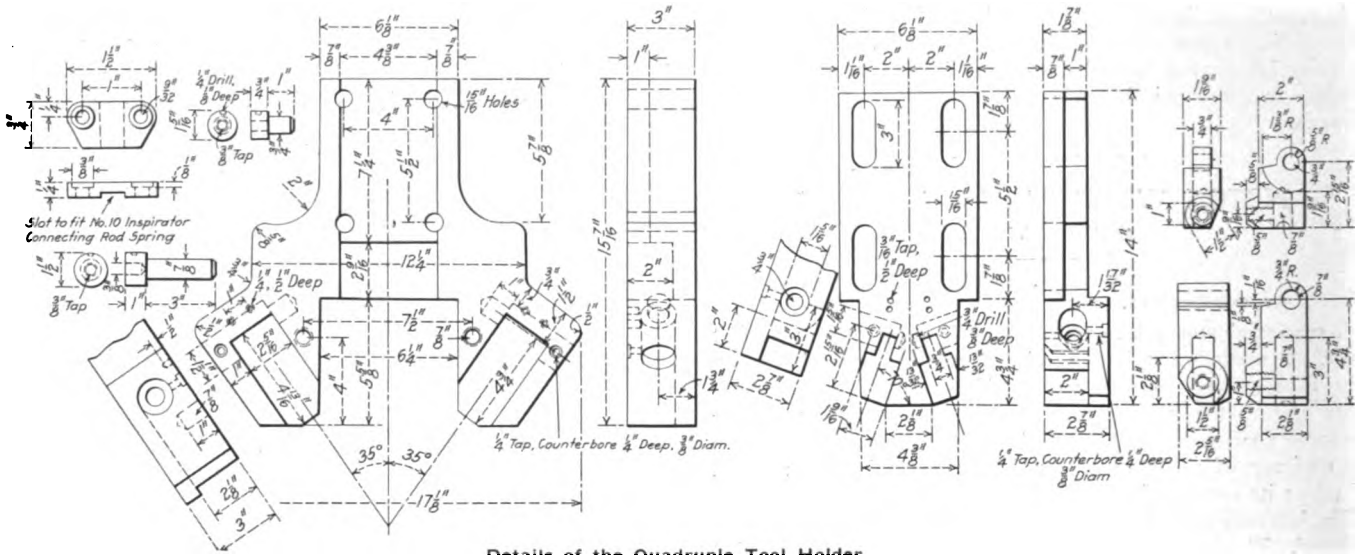
Details of the Quadruple Tool Holder
