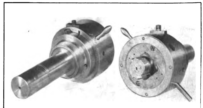
Modern Collapsible Tap
