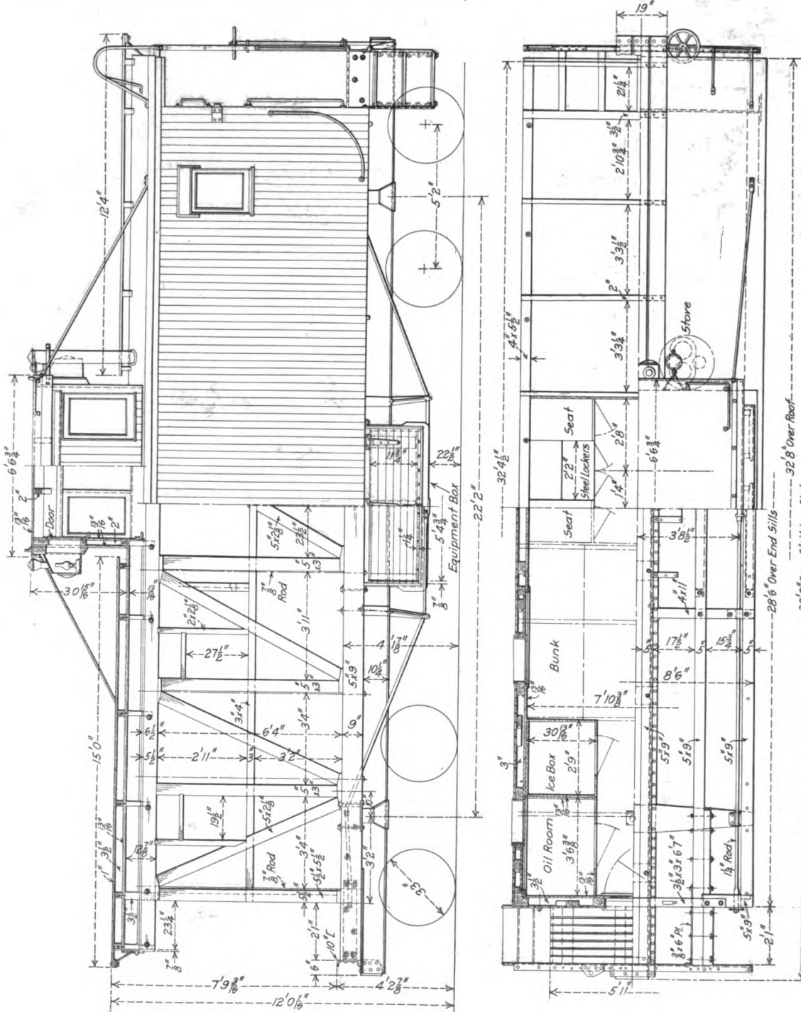
Elevations and Sections of the Erie Caboose with Steel Center and End Sills and Body Bolsters
