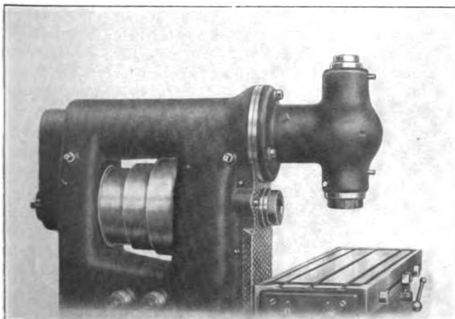
Vertical Milling Attachment in Place
