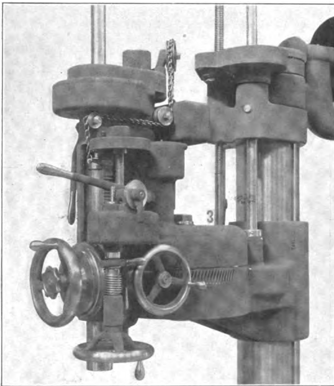
Rotating Head for Wilmarth Radial Drill
