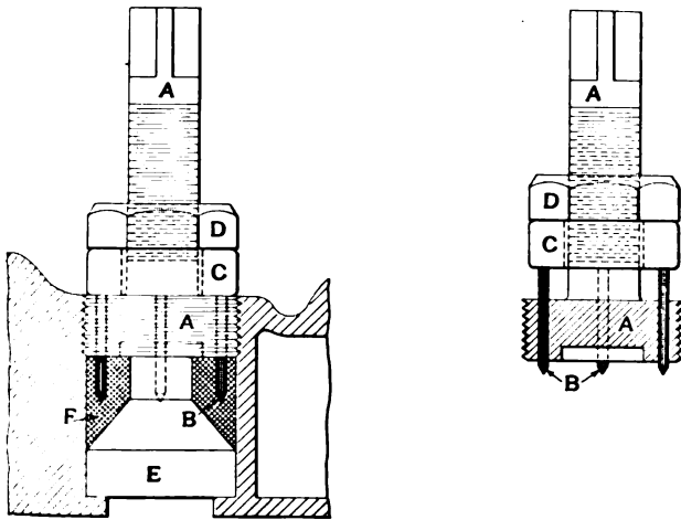
Device for Removing Gaskets from Bullseye Lubricators
