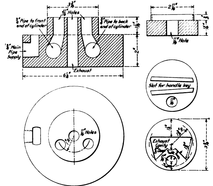
Four-Way Valve and Seat
