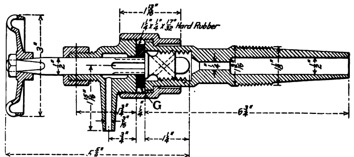
Water Gage Cock with Special Features
