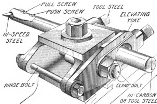
Double Reversible Tool Holder
