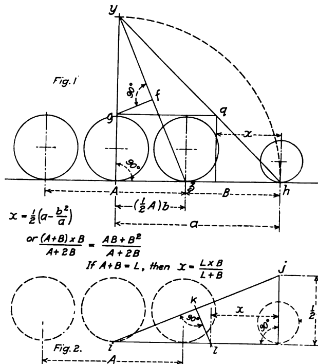
Graphic Methods of Locating Radius Bar Pins
