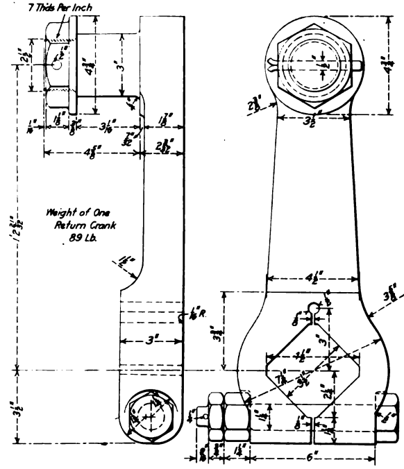
Fig. 48—Valve Motion Return Crank for 4-6-4 Type Locomotive
