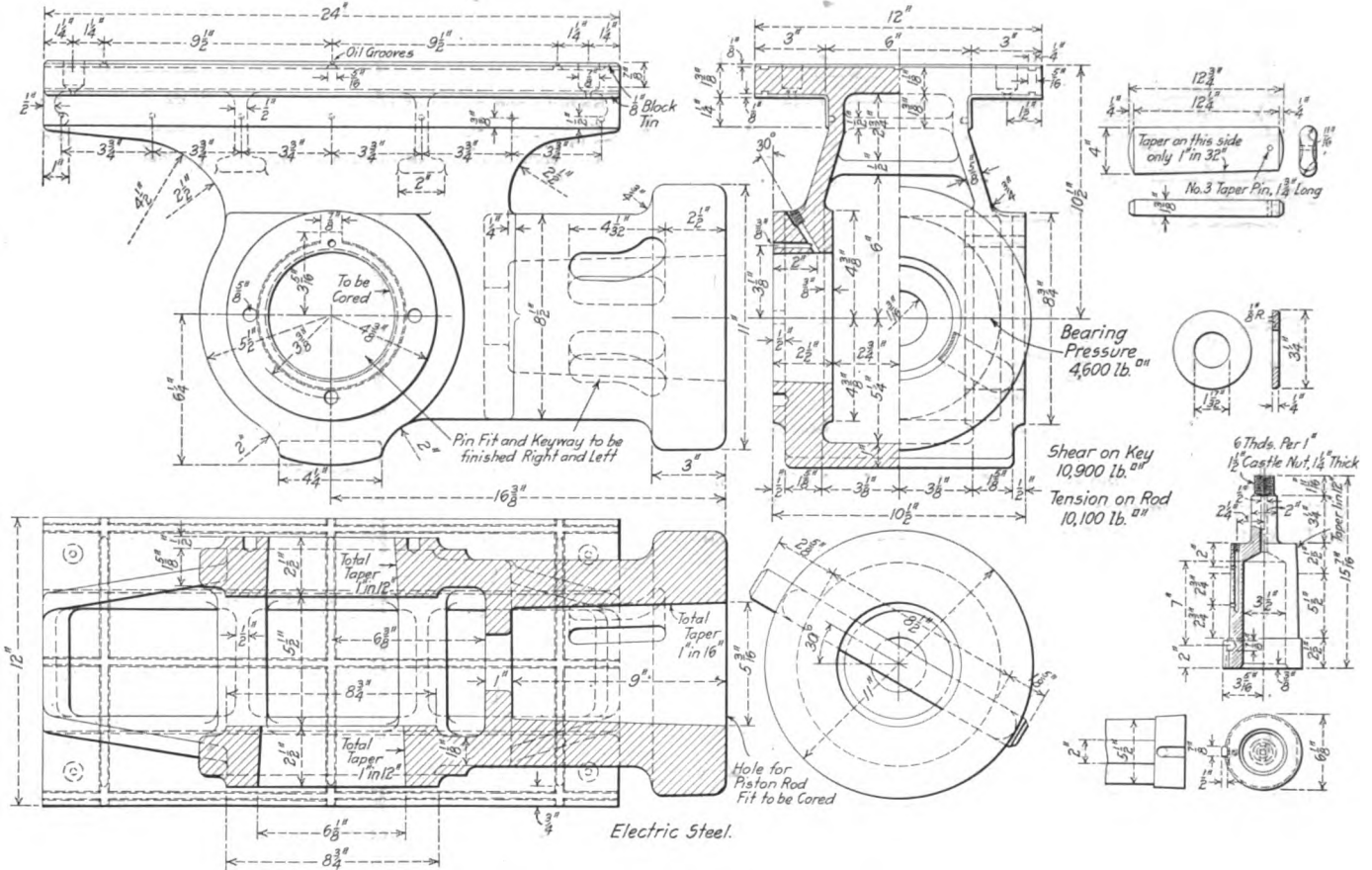
Fig. 10—Crosshead of Pennsylvania Pacific Type Locomotive
