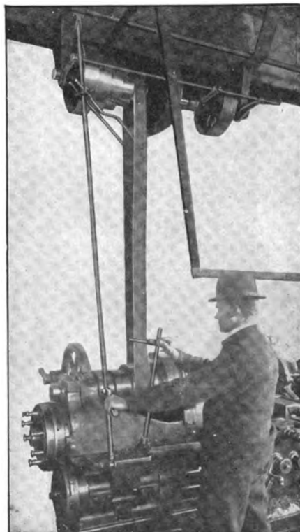
Belt Shifter for Step Cone Machines
