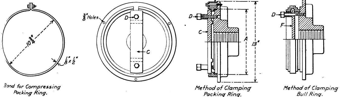
Fig. 2—Chuck for Finishing Valve Chamber Packing Rings and Bull Rings
