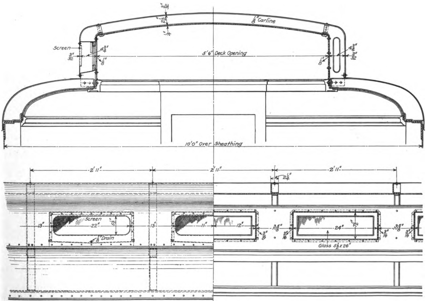
Simple Weather Proof Clere-Story Roof Construction
