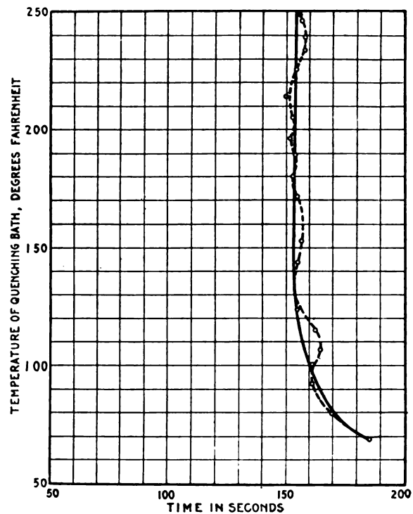
Fig. 9—Quenching Power of No. 1 Dark Tempering Oil
