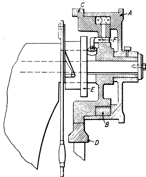
Friction Clutch for Motor Driven Beaudry Hammers
