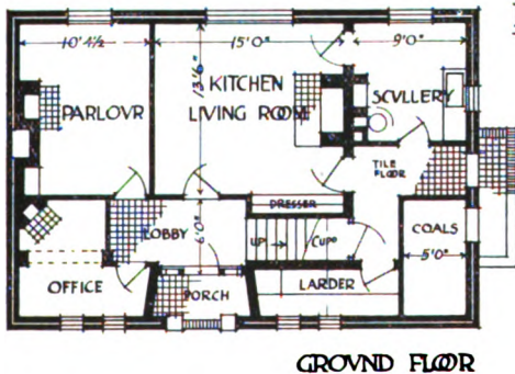
GROVND FLOOR
