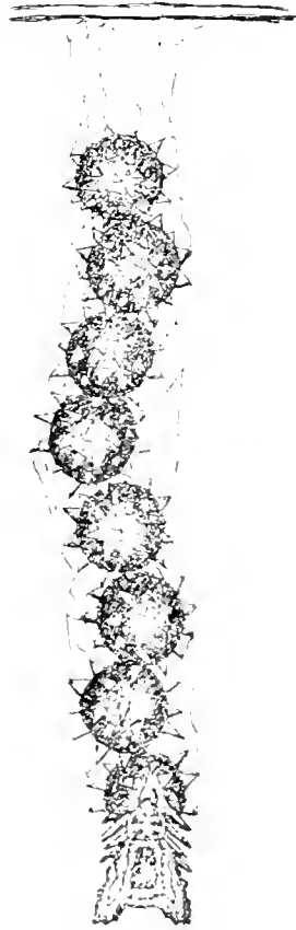
Fig. 2.—Cocoons with spider. C. calotoib. s. Rainb., attached.
