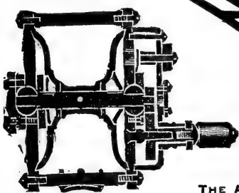
Globe Bearing.
