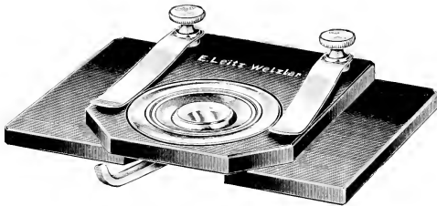
Reflecting Condenser B.
