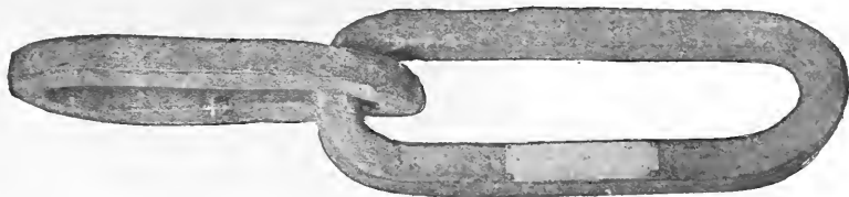
LINKS OF THE CHAIN ACROSS THE HUDSON RIVER AT WEST POINT, 1778
