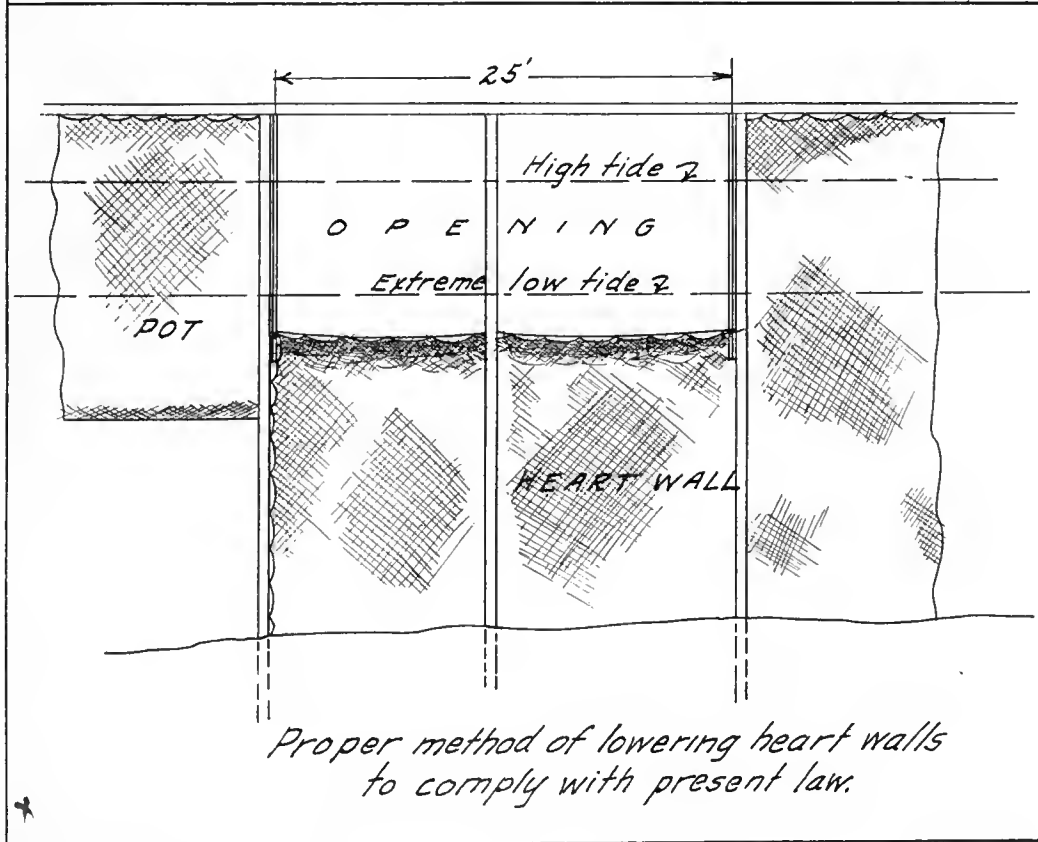
Improper and proper methods of arranging heart walls of fish traps in Alaska.
