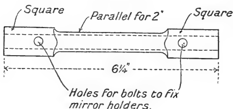
TEST SPECIMEN.
