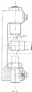
FIG. 2 Illustrating the Report on Stress Distributions in Engineering Materials.
