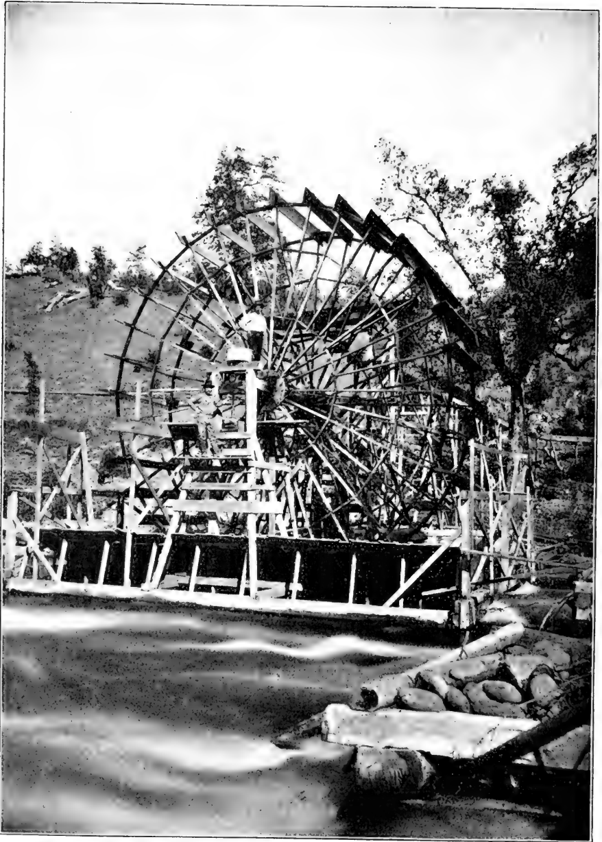
CURRENT-WHEEL FOR PUMPING WATER AT BAIRD, CALIFORNIA.
