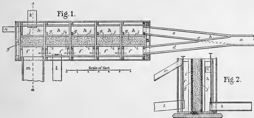
Gravel Filter.
