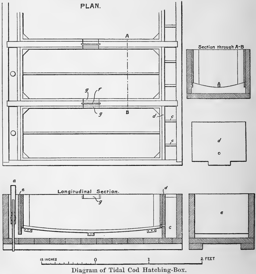
Diagram of Tidal Cod Hatching-Box.
