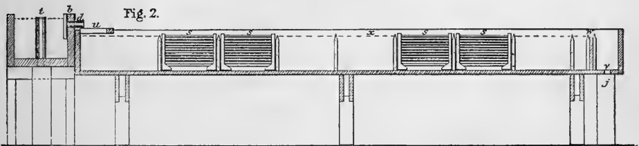
Trough Arranged for Eggs.
