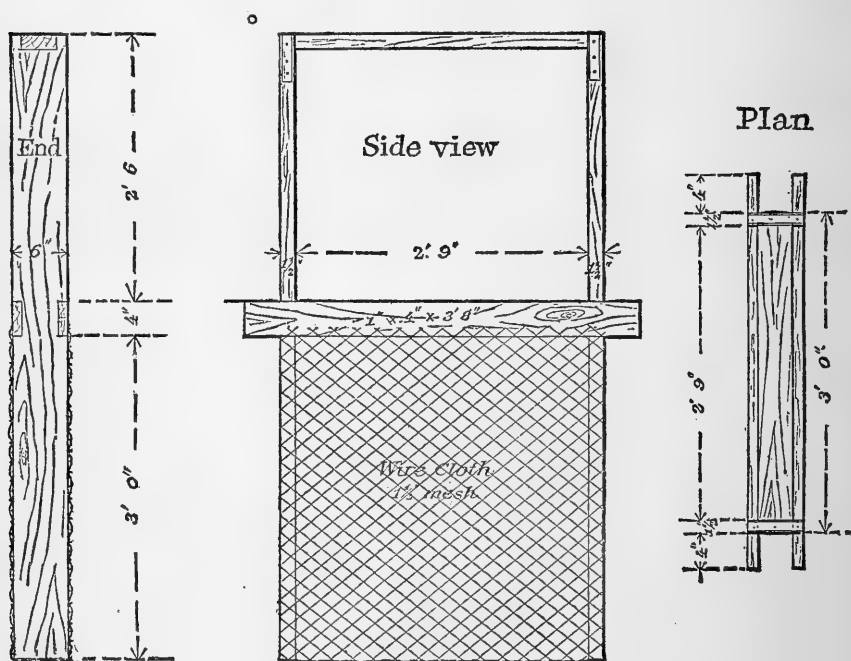
CUT 6.—Receptacle for cultch.
