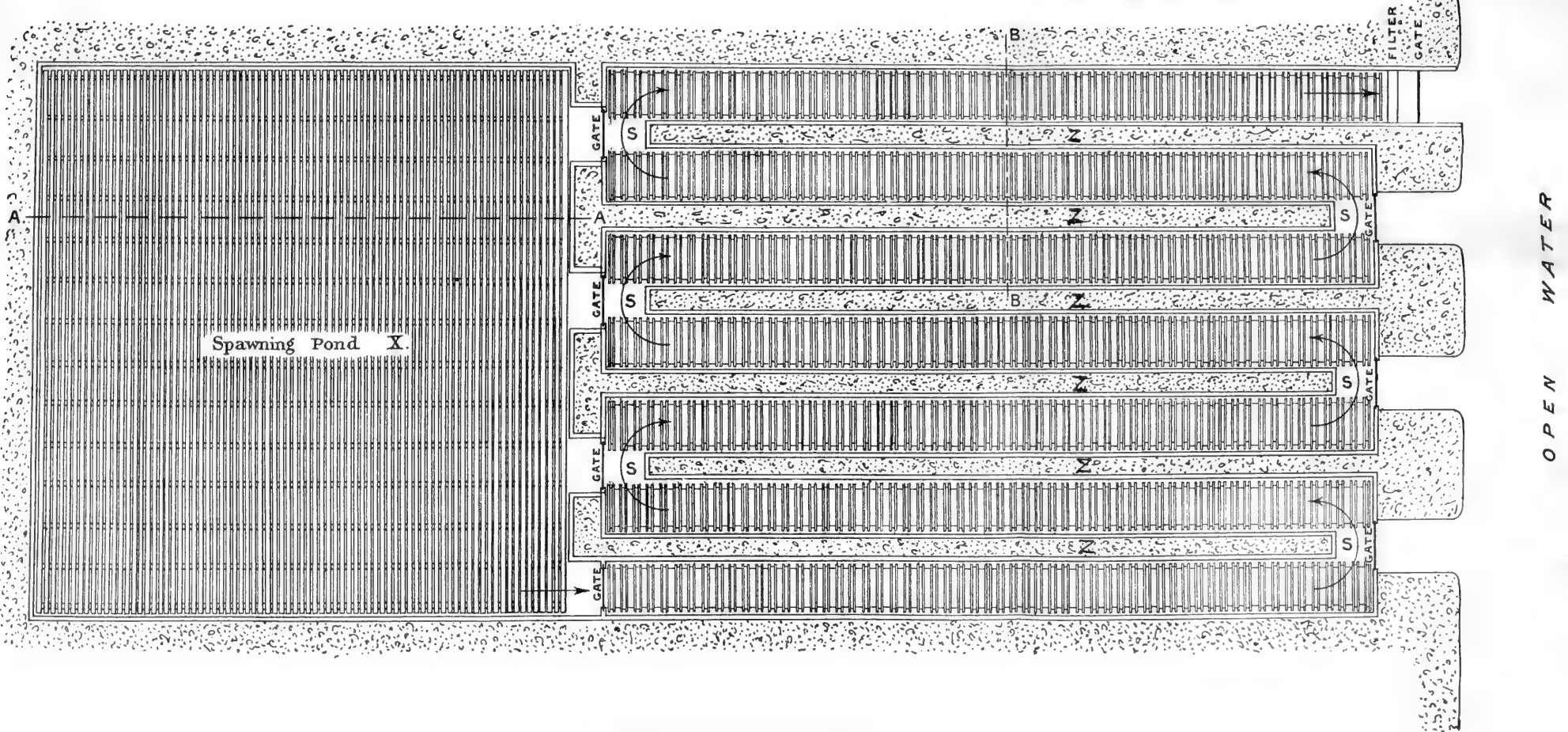
GROUND PLAN AND SECTIONS OF PONDS FOR SPAT-CULTURE. Adapted from John A. Ryder.
