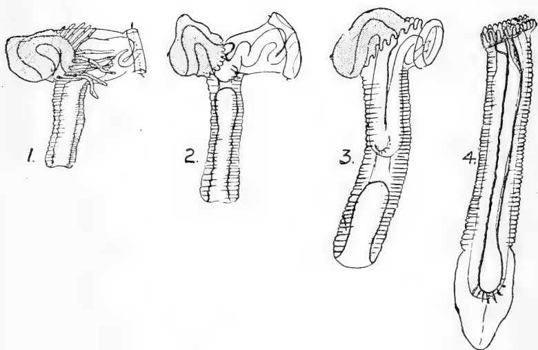
PHORONIDEA.—FIGURE II.
