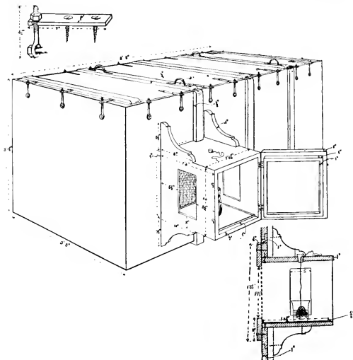
Fumigation Box. Sketch showing construction and external measurements.
