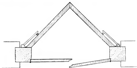
Fig. 2.—Details of double door to Insectary.
