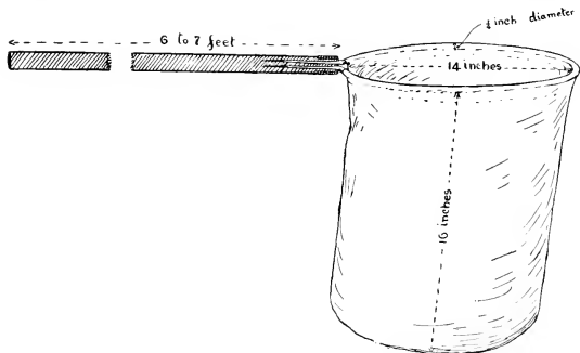
Fig. 1.—Details of Water Net.
