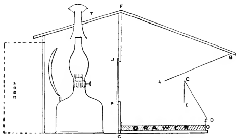
Fig. 3.—Light trap in section.
