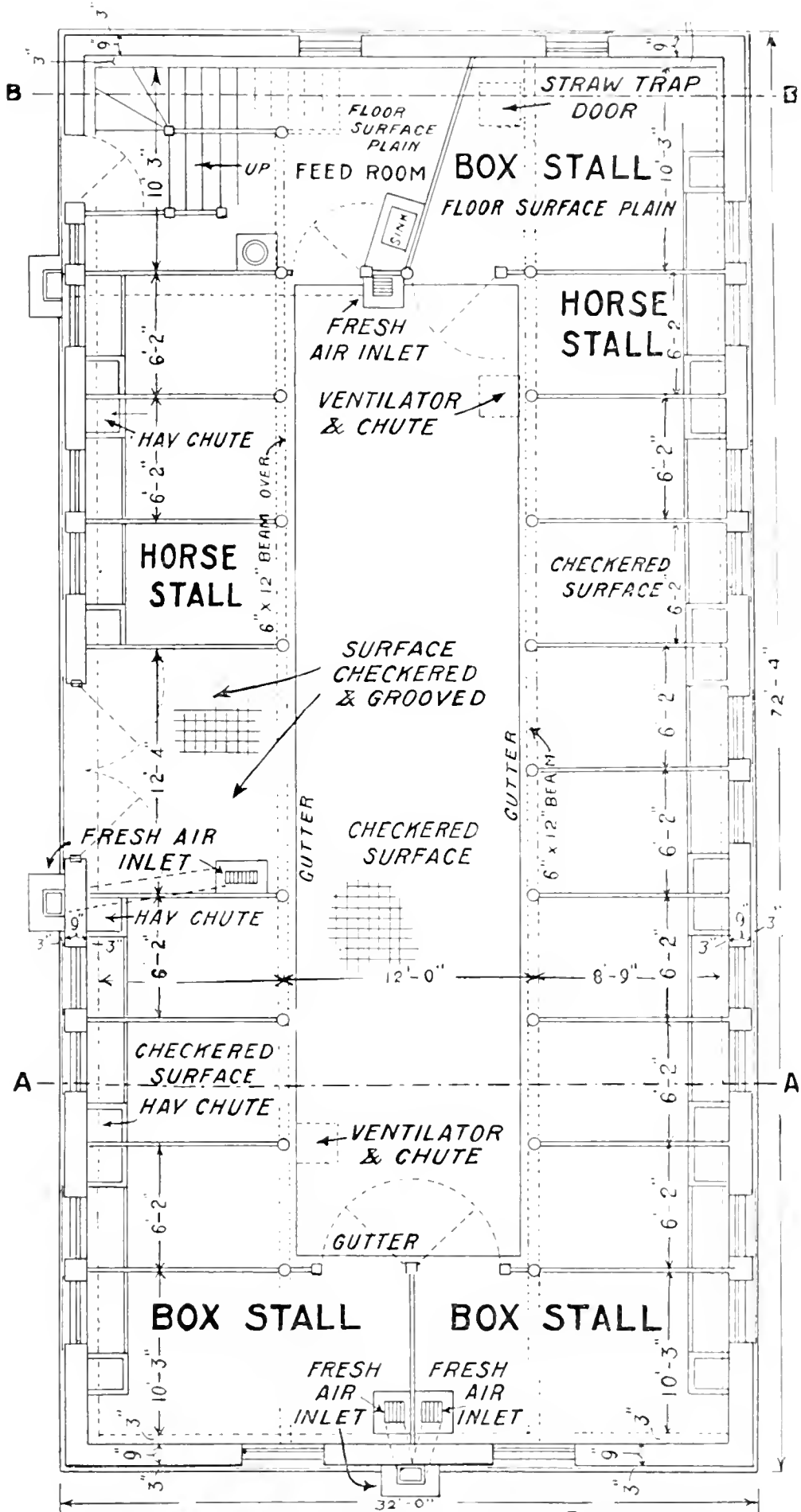
Ground Plan of Horse Stable, Brandon.
