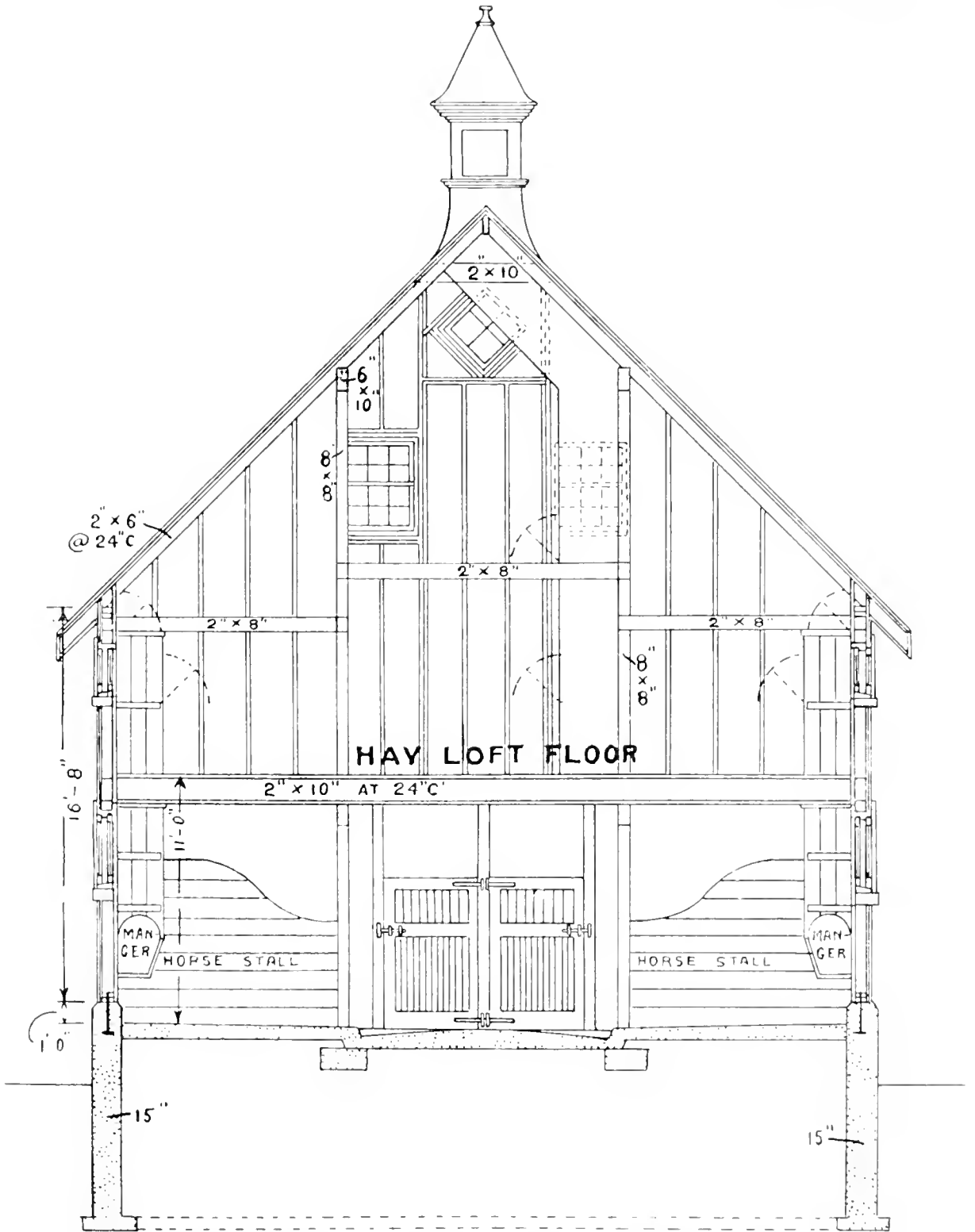
Cross Section of Horse Stable, Brandon.
