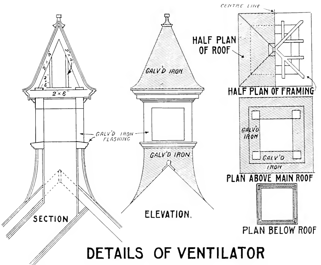
Ventilation of Horse Stable, Brandon (Showing Detail of Ventilator Outlet)
