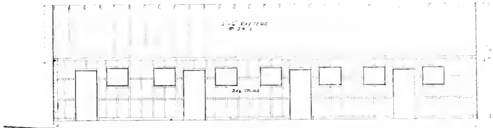
LONG SECTION, SHOWING FRAMING
