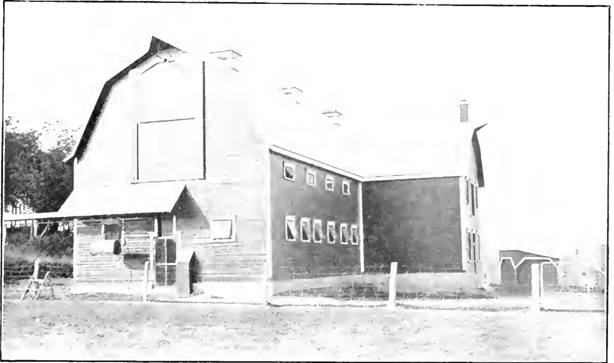
Western end of Horse Barn at Experimental Station, Cap Rouge, Que. Note the lighting, ventilation and conveniences for handling hay and manure.
