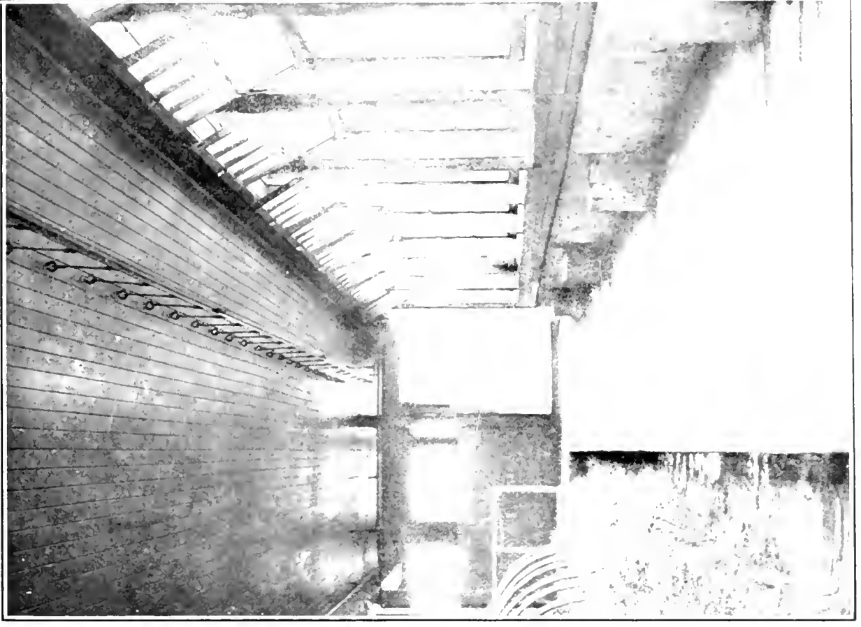
Cattle Barn, Ste. Anne de la Pocatiere. Manure Passage. Note the fresh air intakes.
