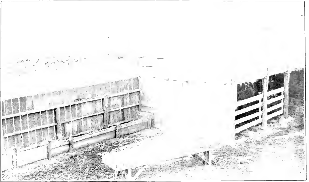
Steer Corral, Lethbridge, Alta. Note, 1, straw covered shed; 2, grain table; 3, roughage rack.
