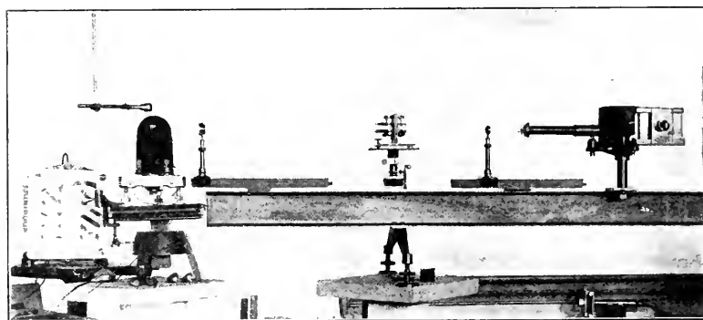
FIG. 13.—THE ANALYSIS OF A MAGNETISED SOURCE BY MEANS OF ÉTALON AND SPECTROSCOPE.
