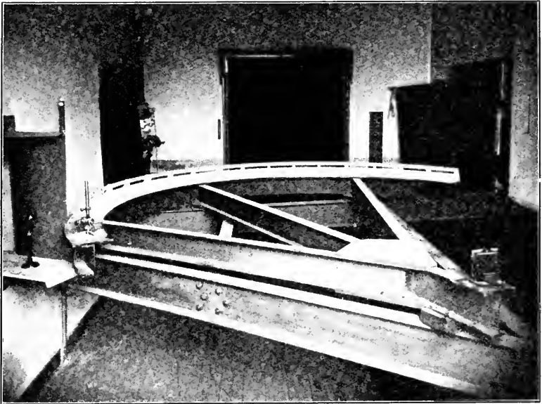
FIG. 7.—THE MOUNTING OF A ROWLAND GRATING.
