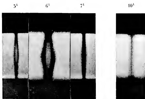
5 1 , 6 1 , 7 1 . Types of Magnetic Resolutions in Non-uniform Fields. 10 1 . Superposition of Magnetic Components.
