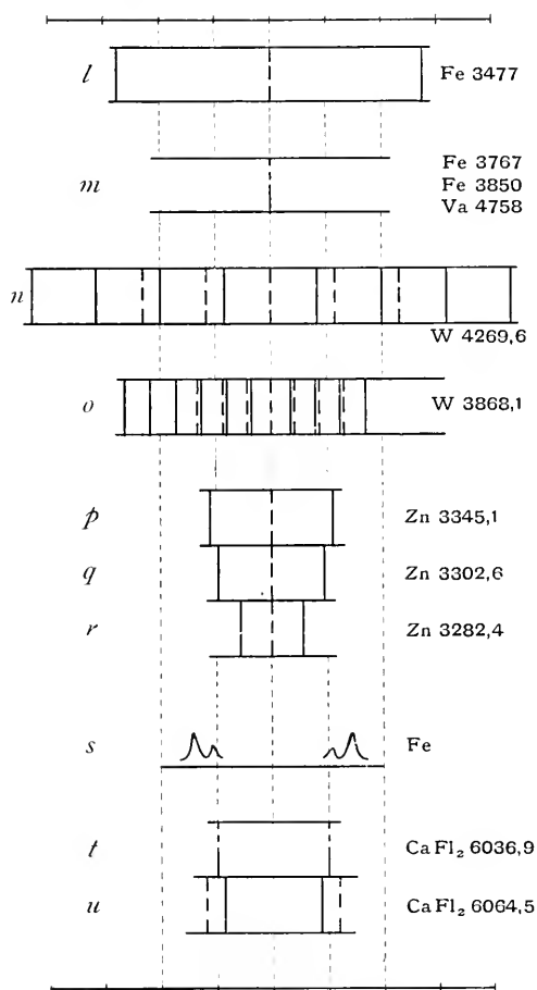
FIG. 73.—TYPES OF MAGNETIC RESOLUTIONS.
