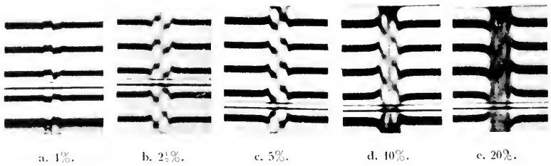
Fig. 48. Lithium Triplet and Magnetic Double Refraction.
