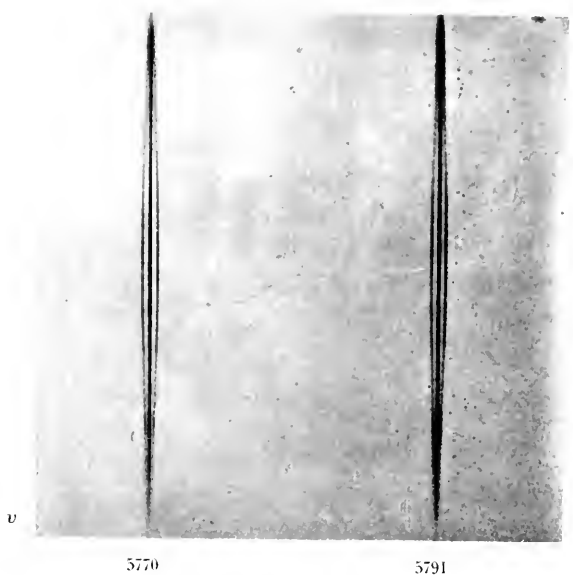
Fig. 52.—Yellow Mercury Lines in Non-uniform Field. 5791 Exhibits Dissymmetry.
