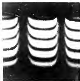
Fig. 40. Magnetic Rotation of plane of Polarisation.
