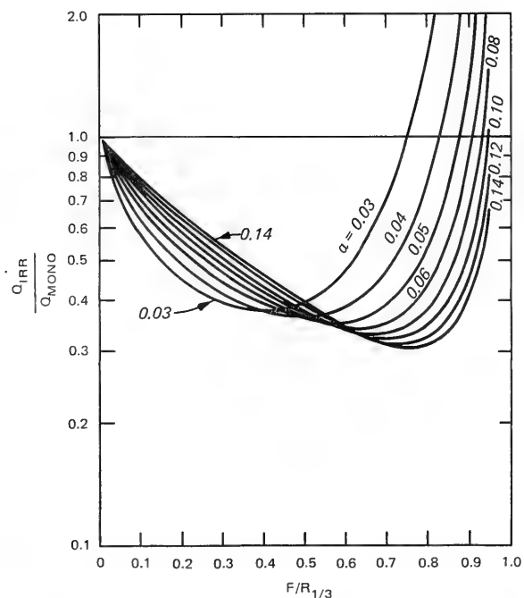
Figure 3. Ahrens' correction factors (from Ahrens 1977a)
