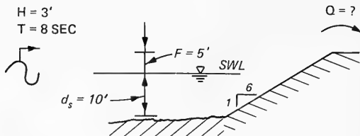
Figure 11. Definition sketch, Example 4
