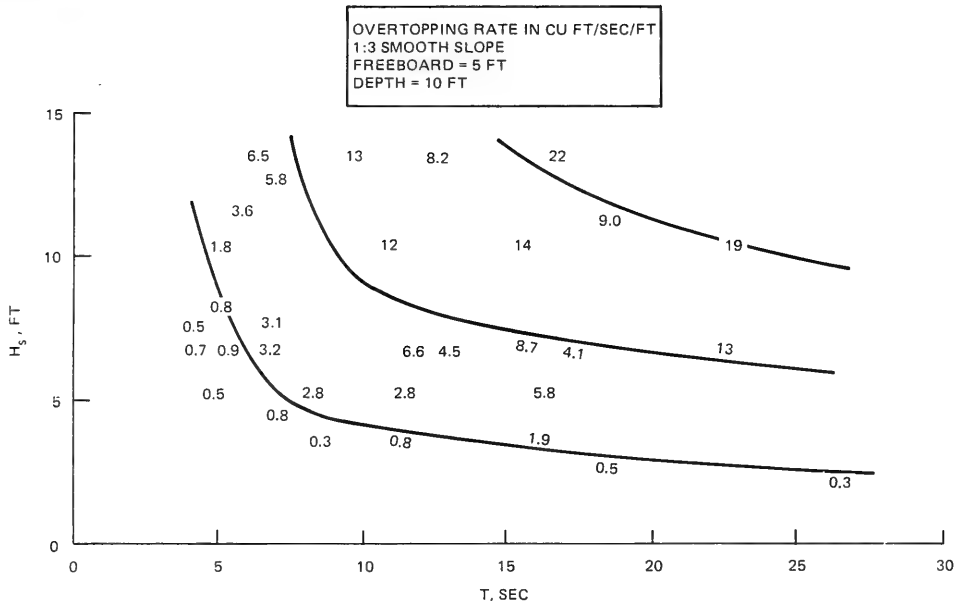
Figure 5. Dimensional overtopping rate plot, Example 2
