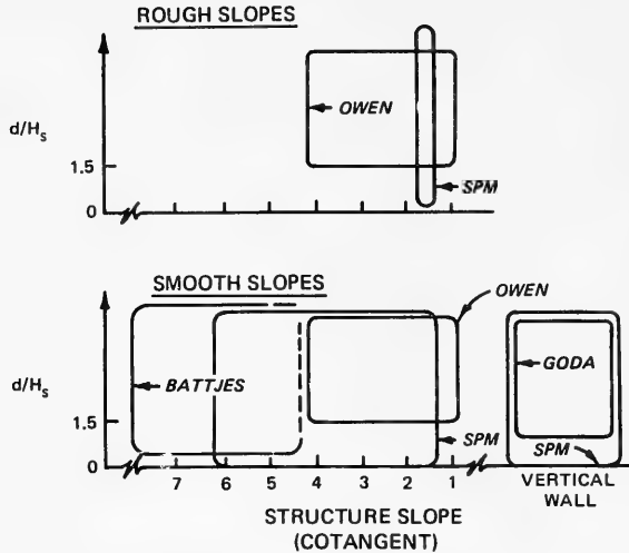
Figure 14. General regions of applicability of overtopping methods
