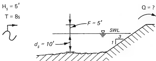
Figure 4. Definition sketch, Example 1
