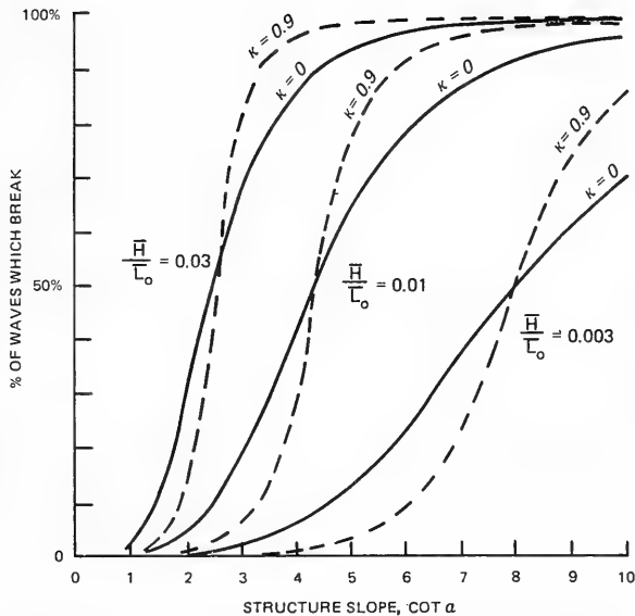
Figure 12. Rough estimate of the percentage of breaking waves
