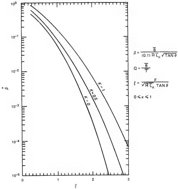
Figure 9. Battjes' irregular wave overtopping (from Battjes 1974)
