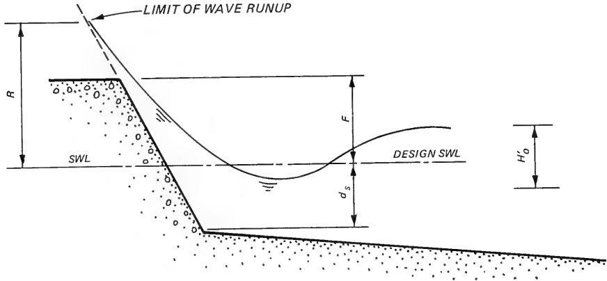
Figure 1. Wave runup definition sketch
