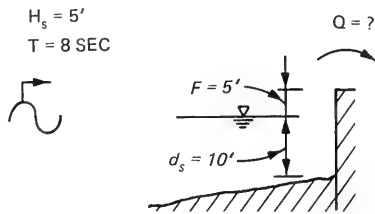
Figure 7. Definition sketch, Example 3
