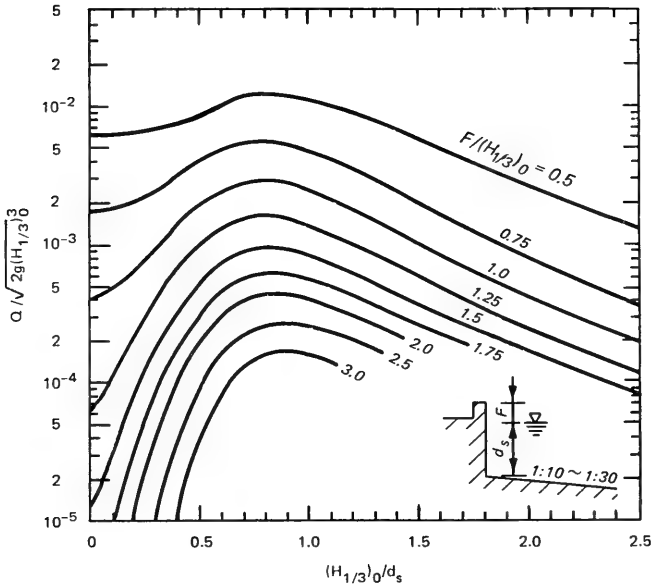
Figure 6. Goda's irregular-wave overtopping rate (from Goda 1971)
