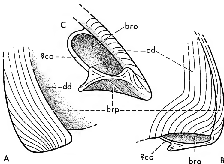
FIG. 18. Region of branchial opening of Protaspis (Eucyclaspis) erroli Denison, somewhat restored from PF 3814 (about \times 2\frac{1}{2} ). A, ventral view; B, dorsal view; C, posterior view. bro , branchial opening; brp , branchial plate; ? co , possible cornual plate; dd , dorsal disc.
