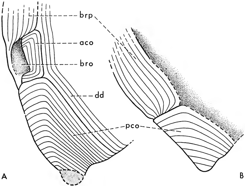
FIG. 25. Region of branchial opening of Lampraspis tuberculata , n. sp., somewhat restored ( \times 1\frac{1}{2} ). A, dorsal view, PF 4342; B, ventral view, PF 4925. aco , anterior cornual plate; bro , branchial opening; brp , branchial plate; dd , dorsal disc; pco , posterior cornual plate.
