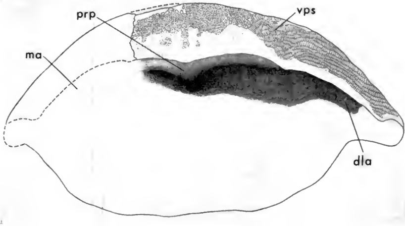
FIG. 14. Rostral plate of Protaspis ( Cosmaspis ) transversa , n. sp., ventral view, PF 5281 (about \times 2 ). dla , ventral surface of dorsal lamina; ma , matrix; prp , median preoral wall; vps , ventral preoral surface.
