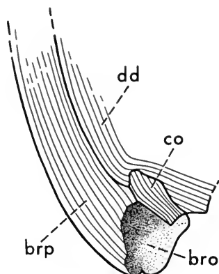
FIG. 12. Region of external branchial opening of Protaspis ( Europrotaspis ) crenulata White, after White, 1961. bro , branchial opening; brp , branchial plate; co , cornual plate; dd , dorsal disc.
