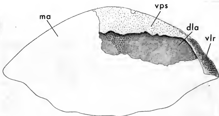
FIG. 26. Rostral plate of Lampraspis tuberculata , n. sp., ventral view, PF 5261 ( \times 3 ). dla , ventral surface of dorsal lamina, lacking the basal layer anteriorly; ma , matrix; vlr , ventro-lateral face; vps , ventral preoral surface.
