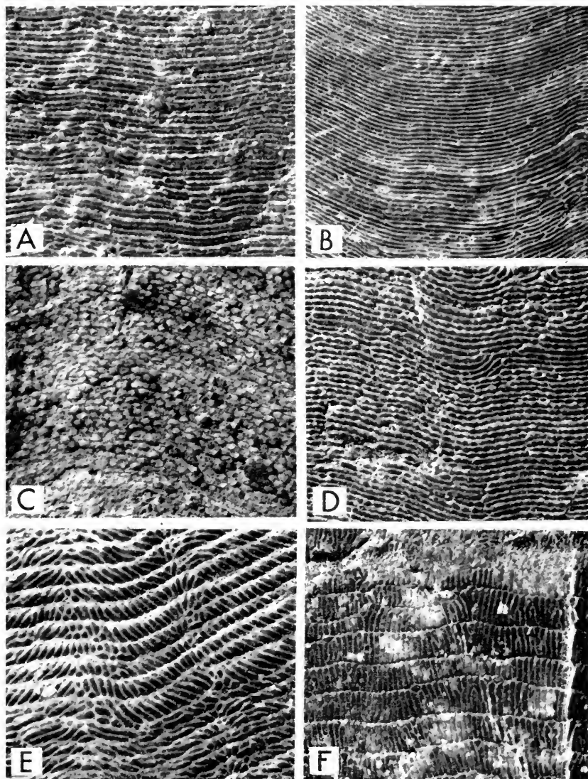
FIG. 7. Ornament of dorsal shield ( \times 6 ). A, P. (Protaspis) mcgrewi , n. sp., PF 4337; B, P. (Protaspis) brevispina , n. sp., PF 4343; C, P. (Cyrtaspidichthys) ovata (Bryant), PF 1523; D, Lampraspis tuberculata , n. sp., PF 4913; E, P. (Cosmaspis) transversa , n. sp., PF 4334; F, P. (Cosmaspis) sp. , PF 951.
