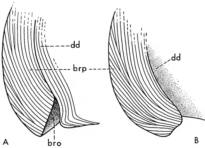
FIG. 6. Region of branchial opening of Protaspis (Protaspis) mcgrewi , n. sp. (about \times 1 ). A, dorsal view of PF 4337; B, ventral view of PF 4763. bro , branchial opening; brp , branchial plate; dd , dorsal disc.
