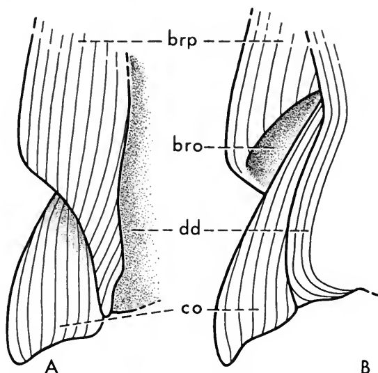
FIG. 1. Region of branchial opening of Protopteraspis primaeva (Kiaer), based largely on PF 1078 ( \times 7 ). A, ventral view, right side; B, dorsal view, left side. bro , branchial opening; brp , branchial plate; co , cornual plate; dd , dorsal disc.
