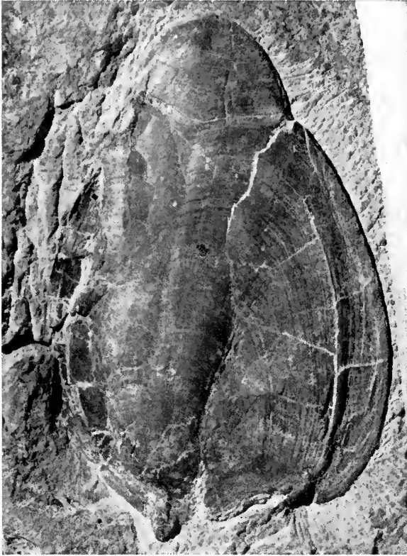
FIG. 8. Dorsal shield of type specimen of Protaspis (Protaspis) brevispina , n. sp., PF 4343 ( \times 3/4 ).
