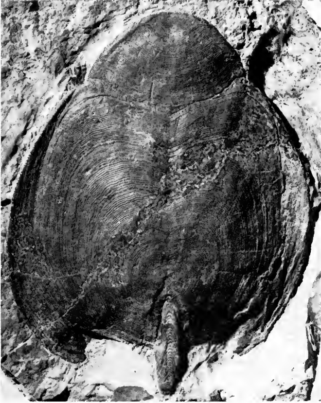
FIG. 13. Dorsal shield of type specimen of Protaspis (Cosmaspis) transversa , n. subgen., n. sp., PF 4334 ( \times 3/4 ).
