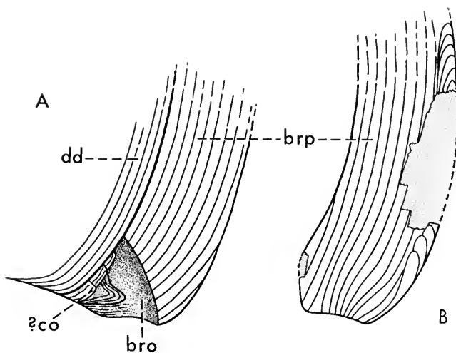
FIG. 11. Region of external branchial opening of Protaspis (Protaspis) brevispina , n. sp. (about \times 2 ). A, dorsal view, PF 4343; B, ventral view, PF 5322. bro , branchial opening; brp , branchial plate; ? co , possible cornual plates; dd , dorsal disc.
