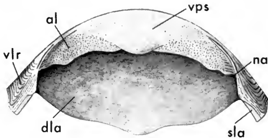
FIG. 19. Rostral plate of Protaspis (Eucycluspis) erroli Denison, ventral view, restored from PF 3814 ( \times 2\frac{1}{4} ). al , ascending lamella; dla , ventral surface of dorsal lamina; na , possible narial notch; sla , sutural area for lateral plate; vlr , ventro-lateral face; vps , ventral preoral surface.
