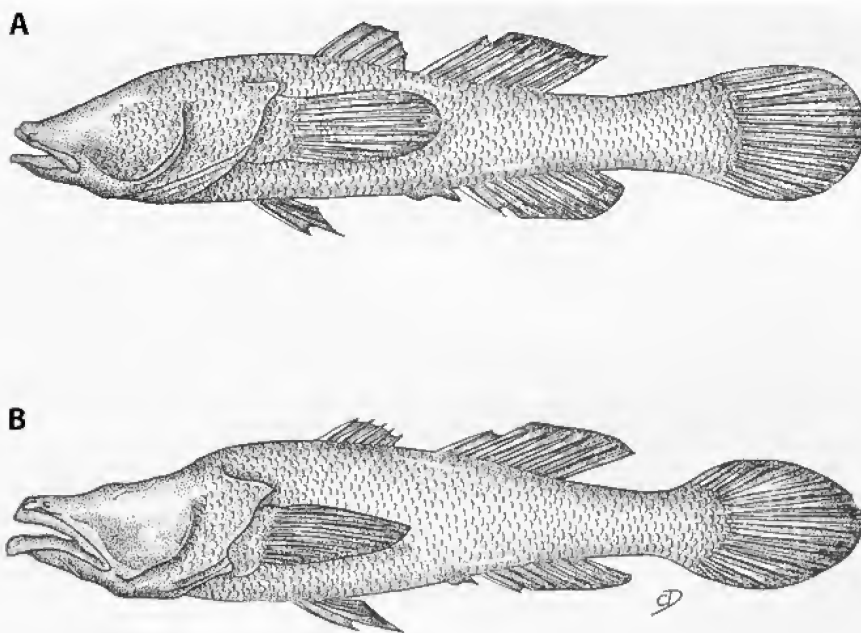
FIGURE 6. Illustration of A. Typhleotris madagascariensis and B. T. pauliani after Arnoult (1959b), showing general body and fin shape, as well as differences in extent of head squamation between species.
