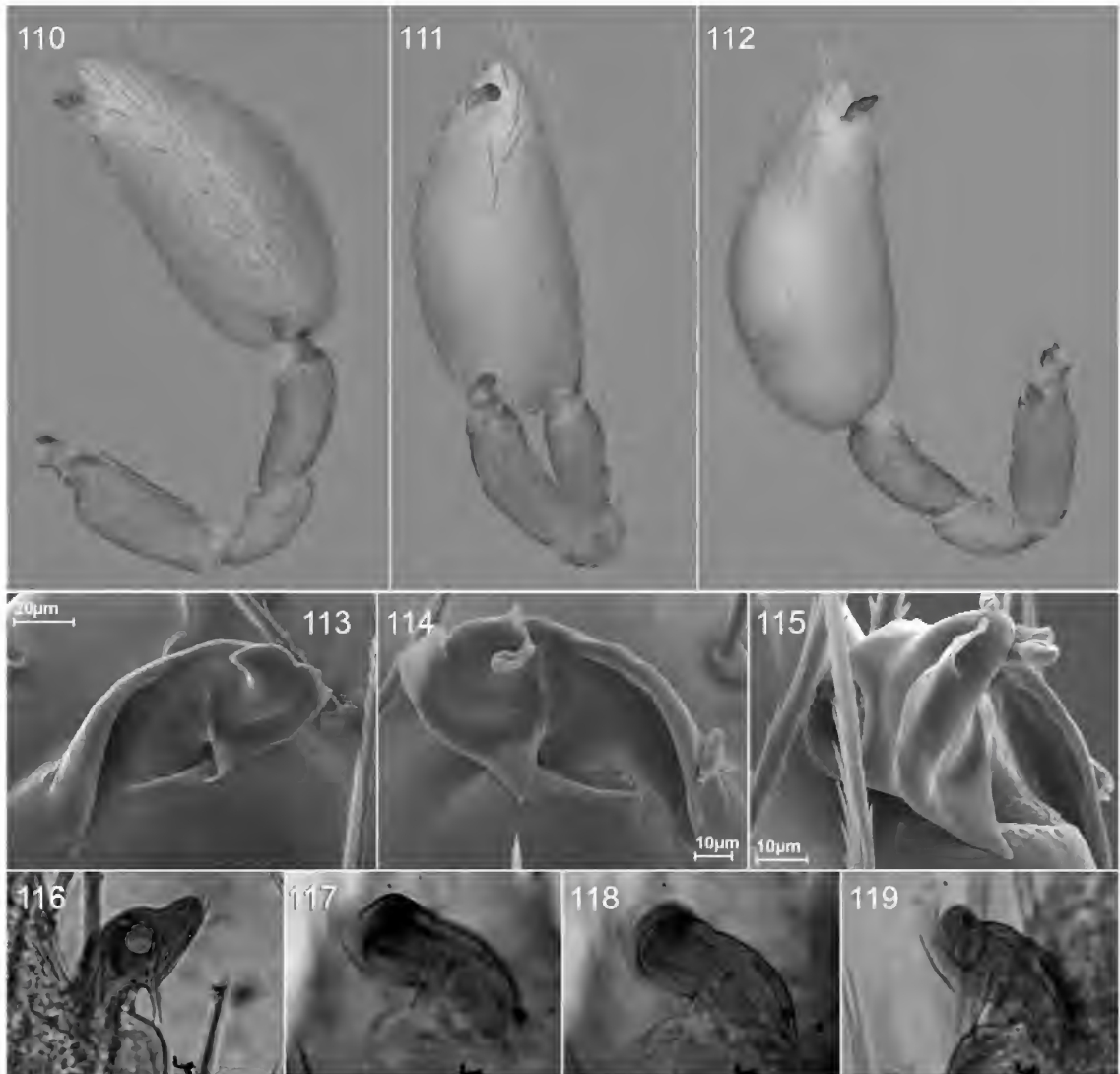
Figs. 110–119. Neoxyphinius gregoblin , new species, male. 110. Right palp, prolateral view. 111. Same, ventral view. 112. Same, retrolateral view. 113. Right embolus, ventral view. 114–119. Left embolus. 114, 117, 118. Ventral view (117, apex in focus; 118, base in focus). 115, 116. Prolateral view. 119. Retrolateral view.
