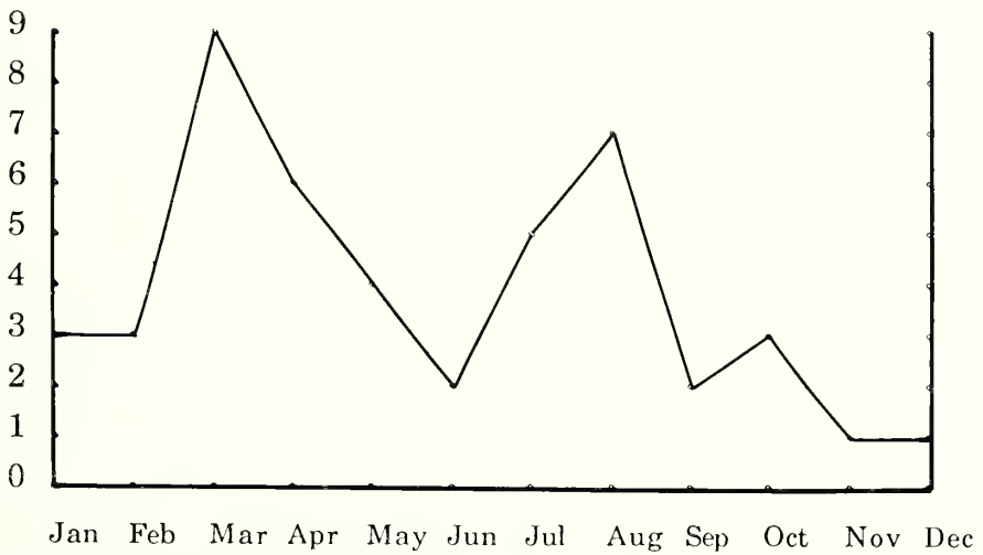
FIGURE 9.—Flowering phenology of Kohleria species. The number given is that of specimens with flowers recorded from each month.
