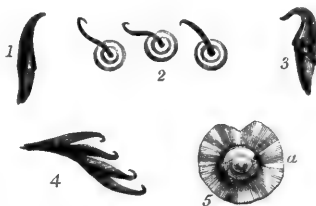
Horny rings and hooks of Belemnoteuthis antiquus .
