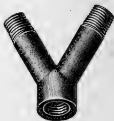
FIG. 16.—"Y" for attaching two nozzles to one lead of hose.
