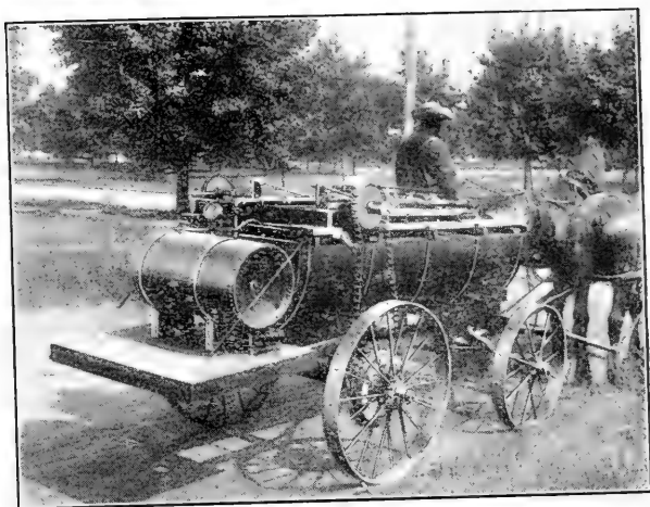
FIG. 1.—Invincible Mounted Sprayer—Wallace Machinery Co. The spray liquid is pumped into an airtight tank together with compressed air by pumps driven from the wheels. When machine is standing still the compressed air continues the work.
