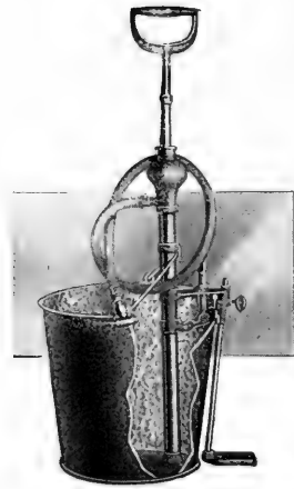
FIG. 2.—Bucket pump.
