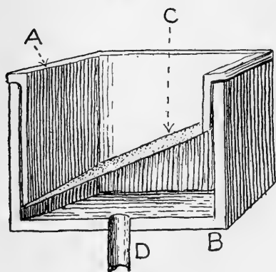
FIG. 22.—Home-made Strainers. See page 90.
