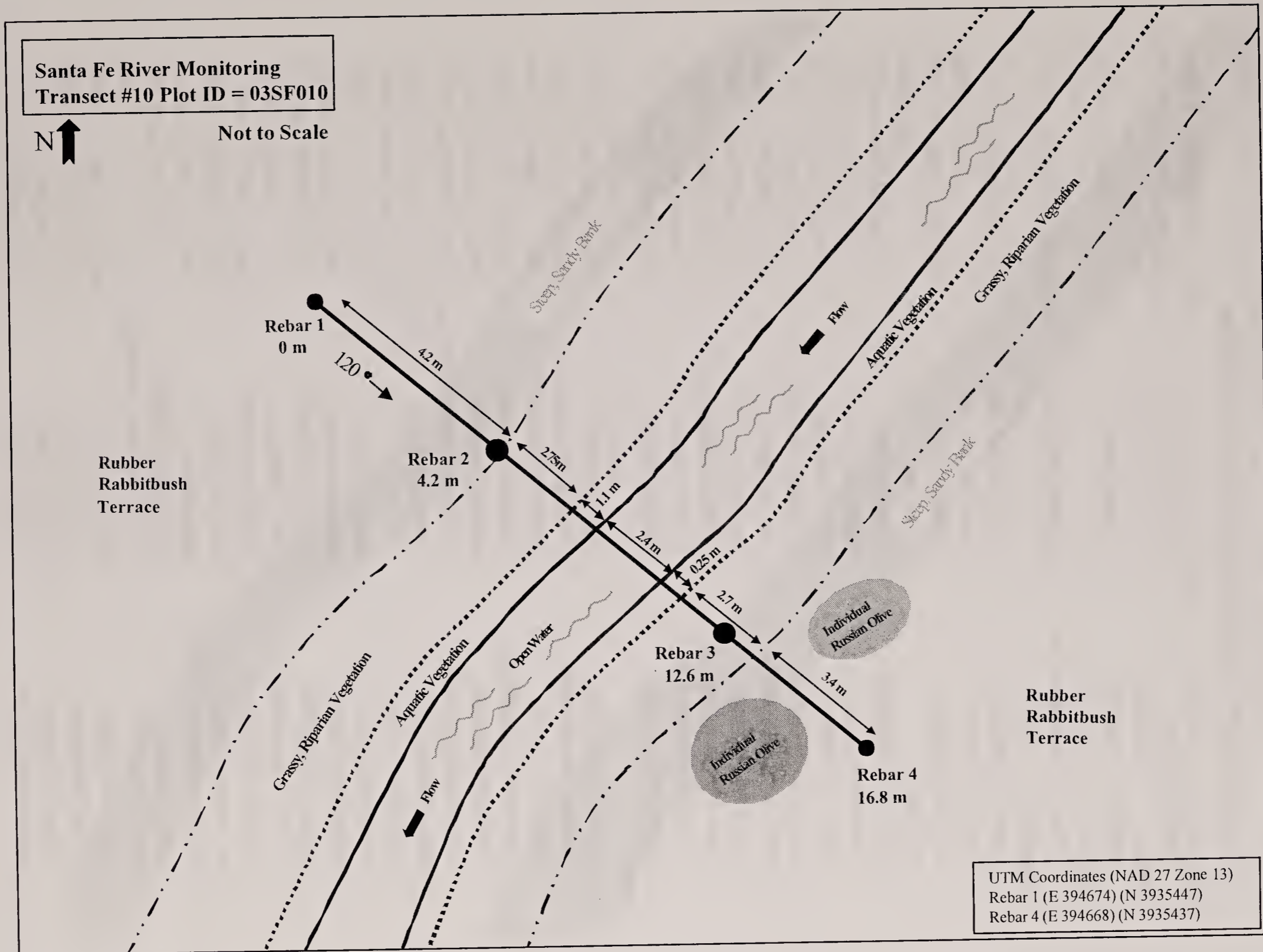
Figure 36: Diagram of transect 03SF010
