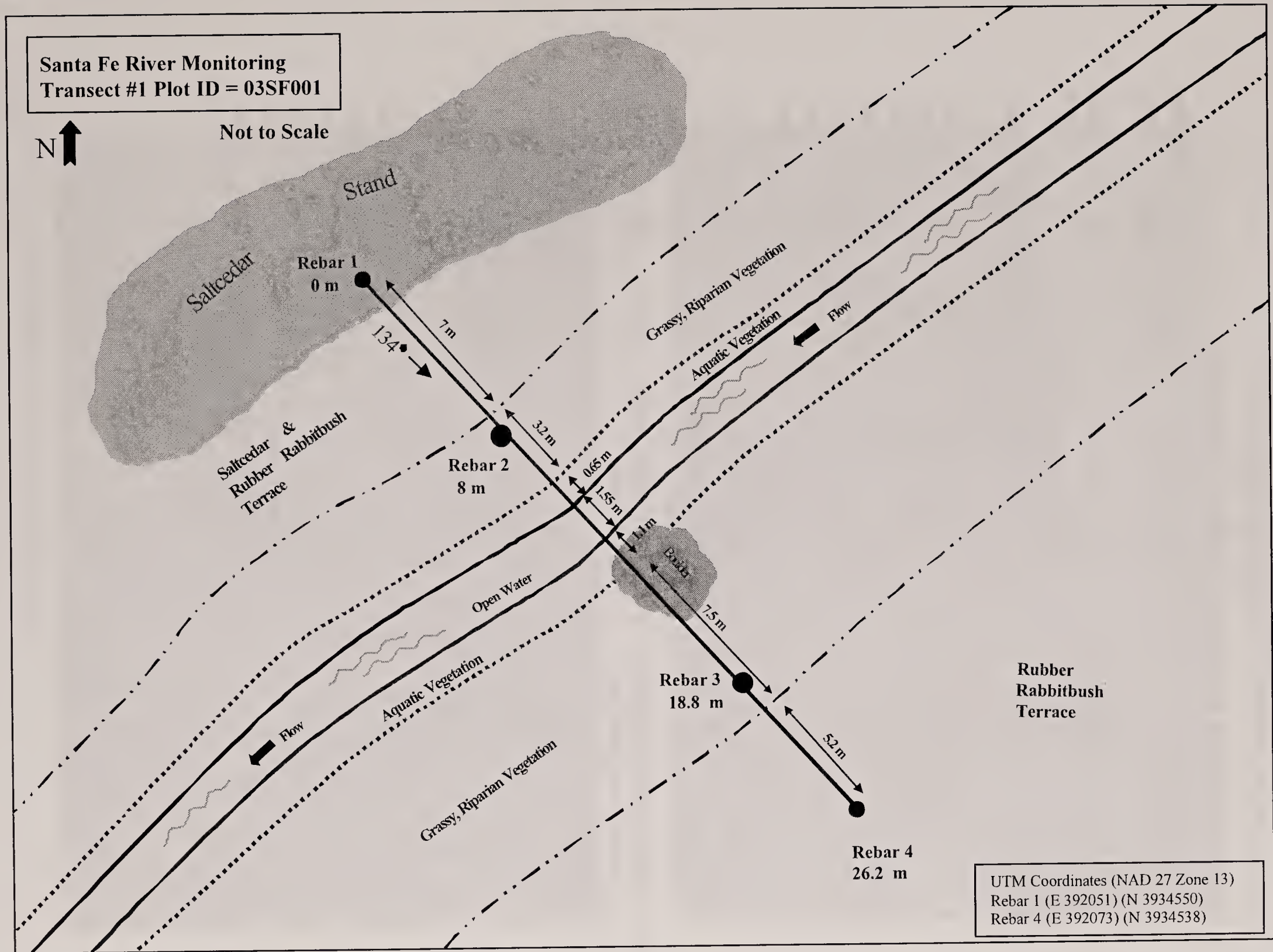
Figure 12: Diagram of transect 03SF001
