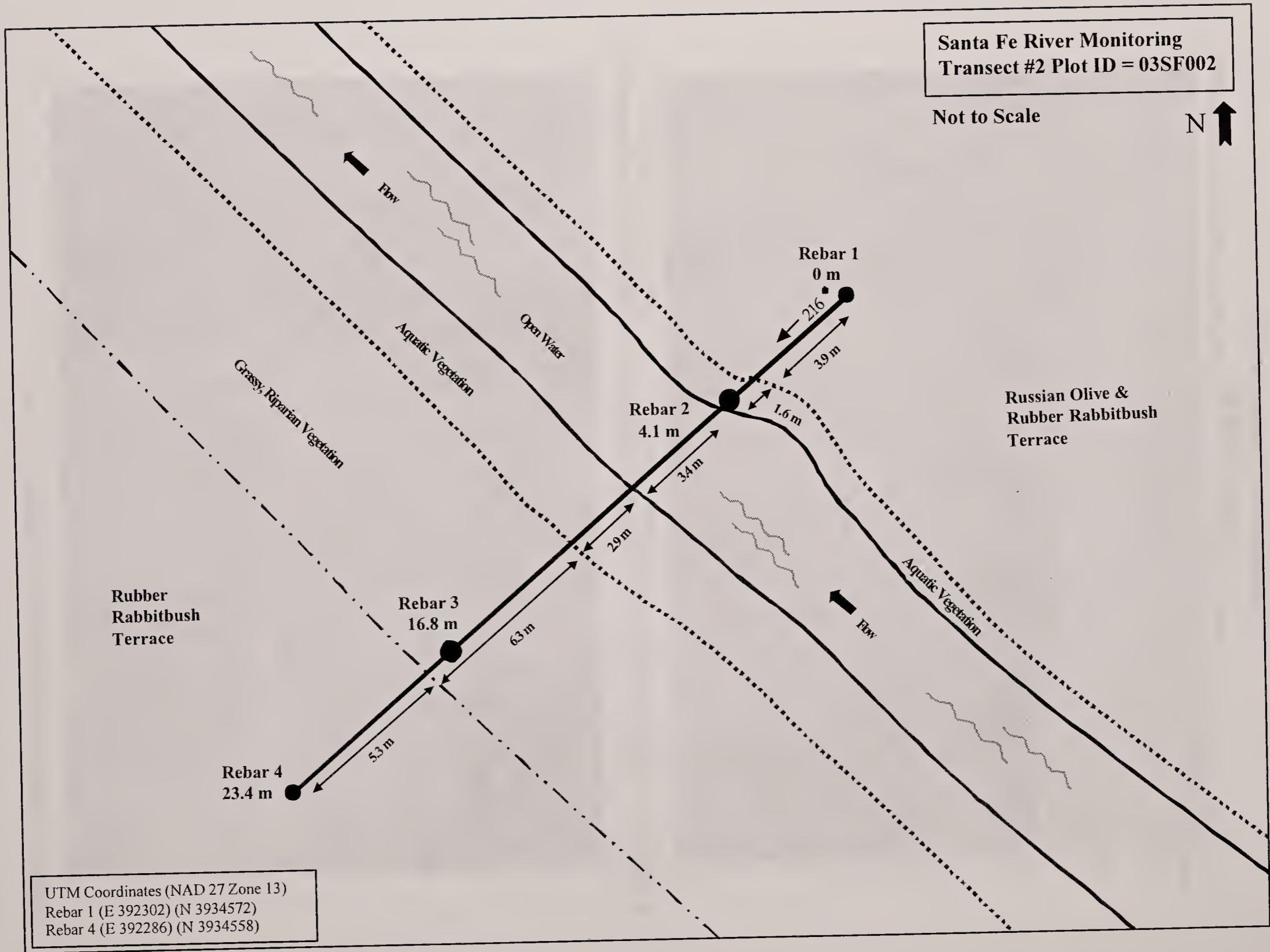
Figure 15: Diagram of transect 03SF002
