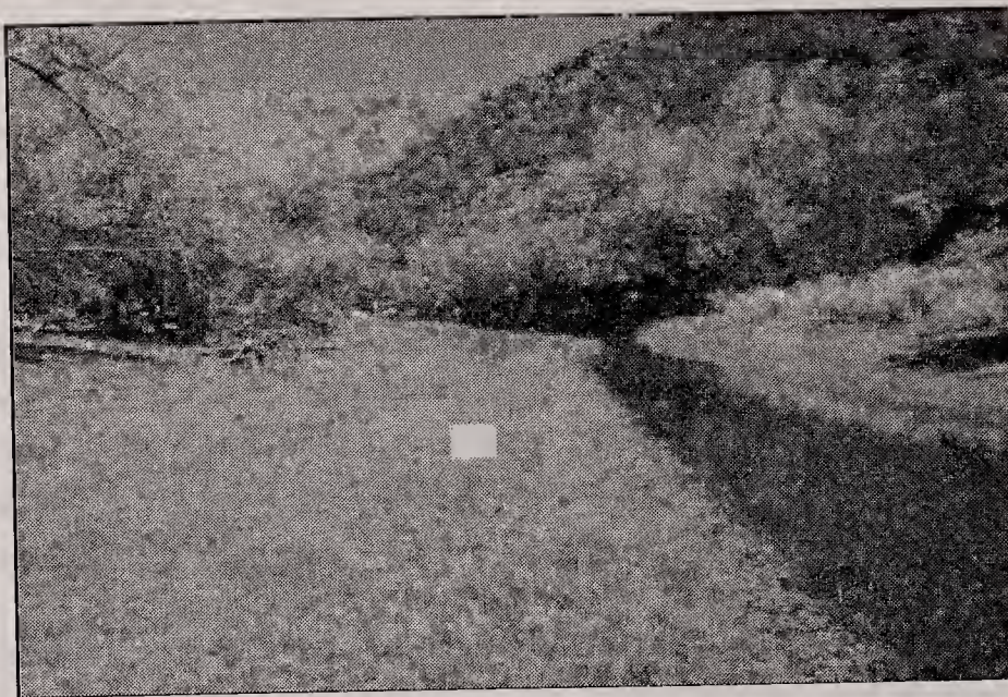
Figure 3. Typically, vegetation zones extend laterally from the open water of the channel through a narrow Aquatic Vegetation zone to Herbaceous Wetlands on the adjacent bars. The upper terraces support a Woody Riparian zone (dominated by Russian olive on the left side of the photo) or an Arroyo Riparian zone (the rubber rabbitbush on the right side of the photo) [photo: Transect 6 2003].
