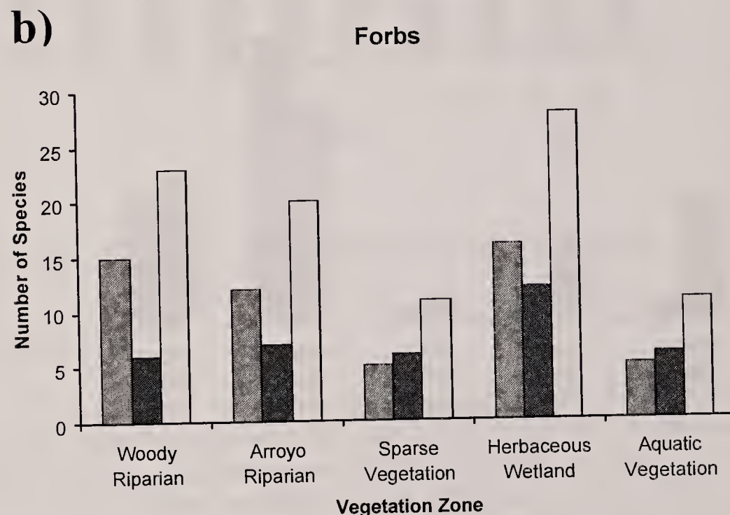
Figure 8. Species richness by origin for graminoids (a) and forbs (b) within each vegetation zone.
