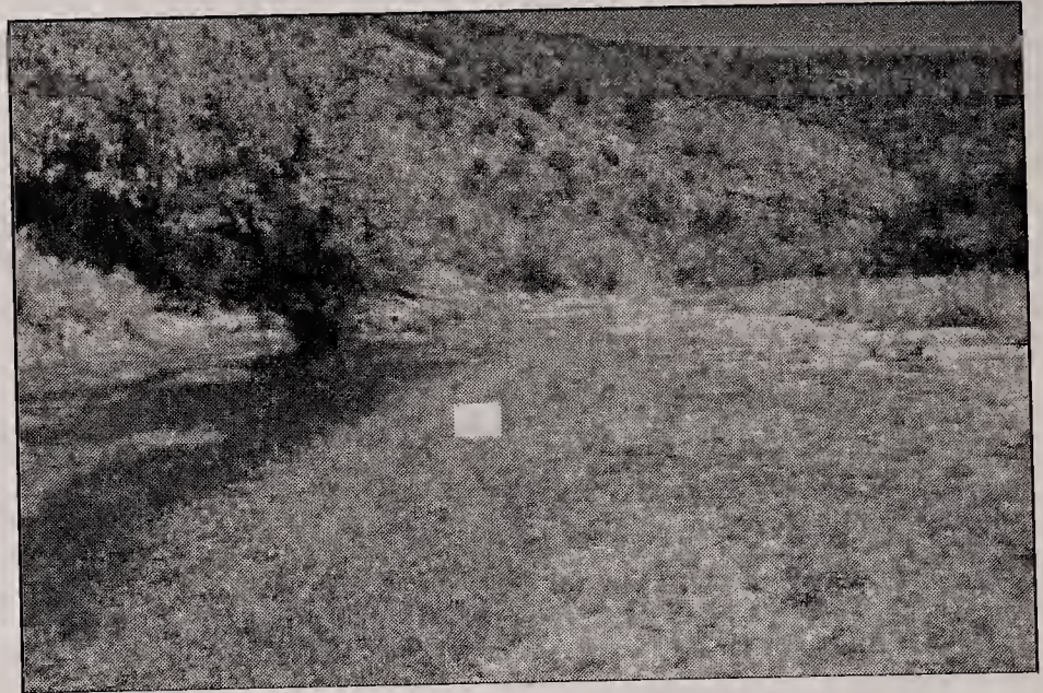
Figure 4. A Sparse Vegetation zone is often found on the side channel bars particularly on sandy and gravelly substrates. [photo: Transect 7 2003].
