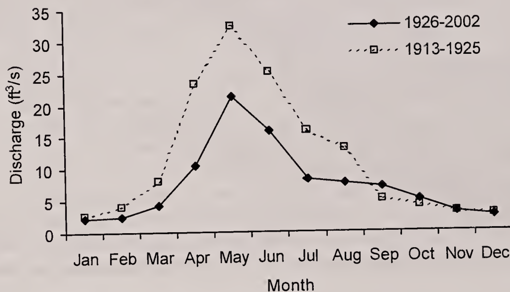
Santa Fe River Stream Flow
