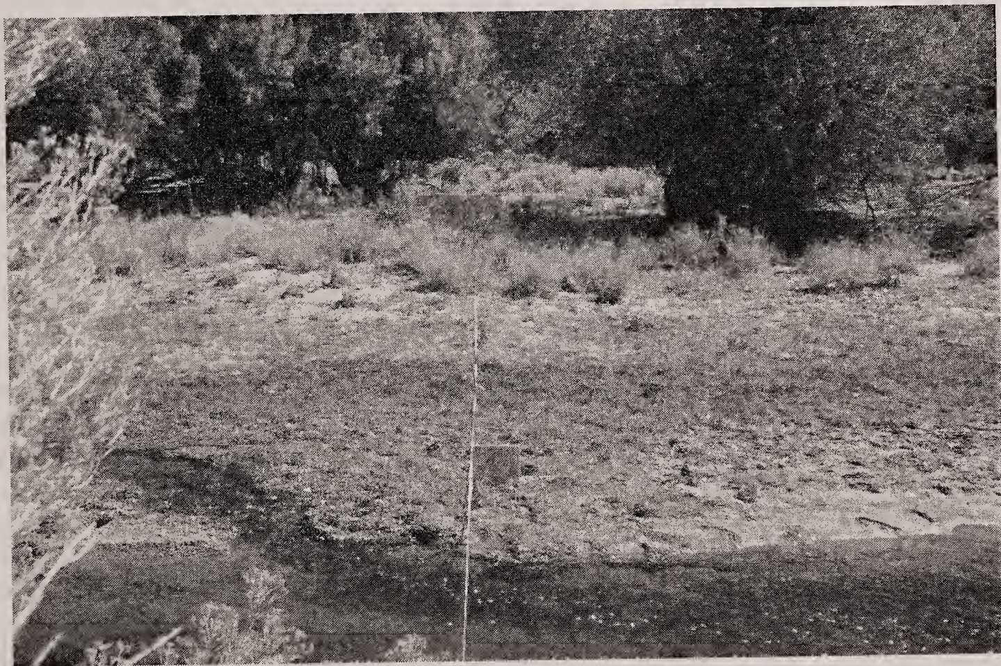
Figure 26: Transect 03SF007, from 2m looking to 28.3m
