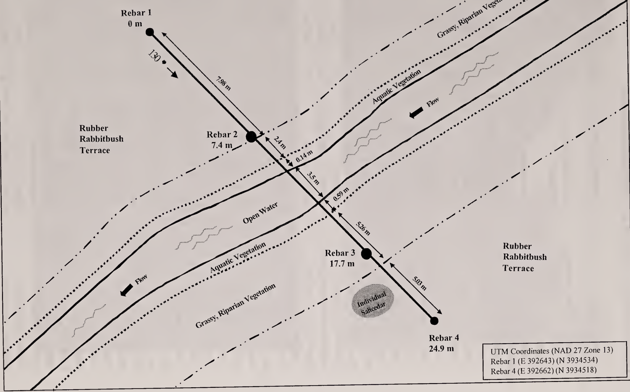
Figure 18: Diagram of transect 03SF003
