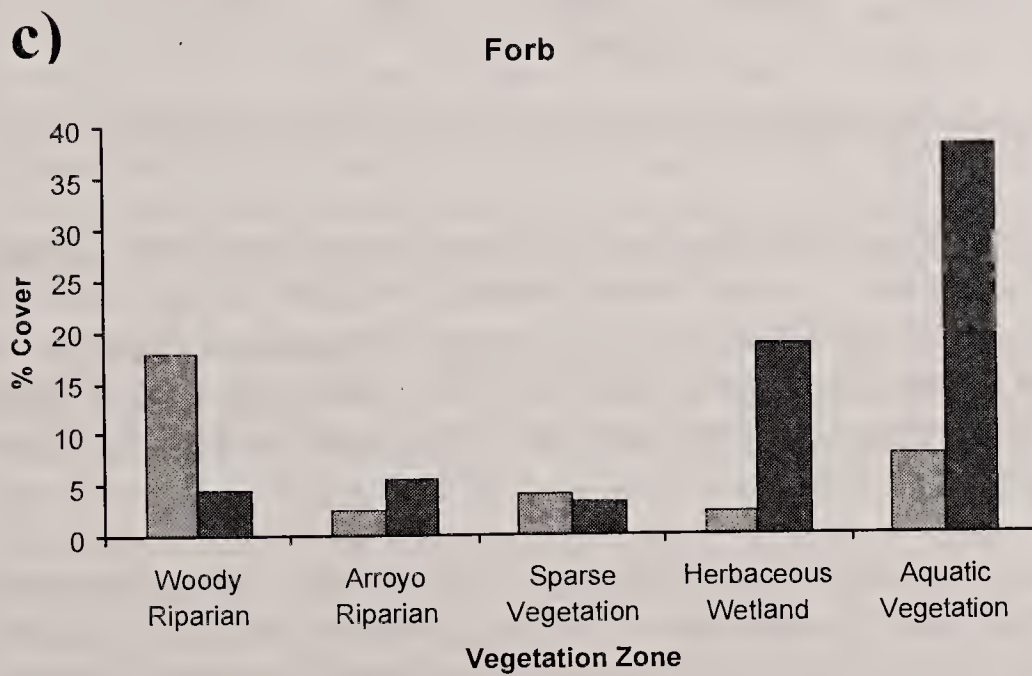
Figure 7. Average Woody (a), Graminoid (b), and Forb (c) cover by origin and vegetation zone.
