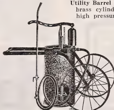
Binks' No. 1 Whitewash Spraying Machine
