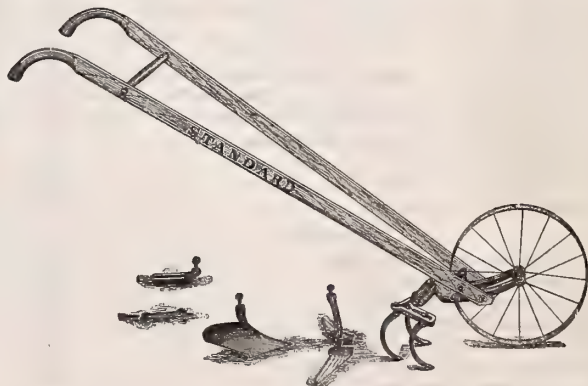
No. 22 Standard Single Wheel Hoe
