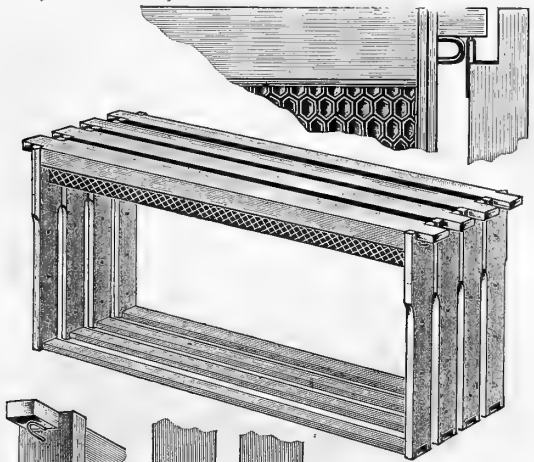
Hoffman Self-Spacing Frame
