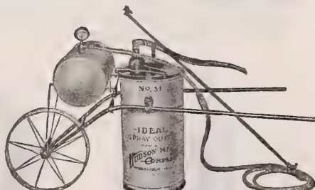
Ideal Portable Sprayer with Air Tank
