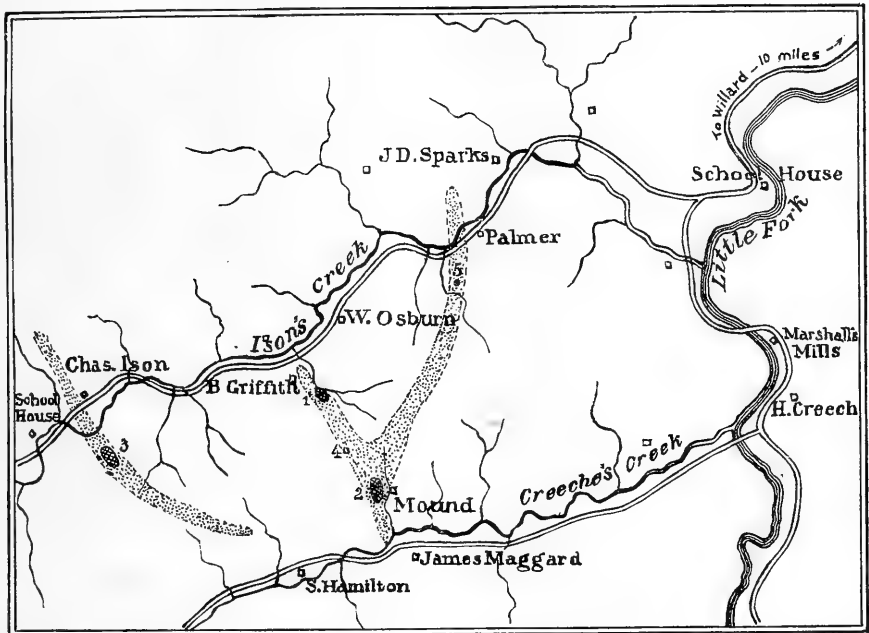
Exposed Peridotite. Soil containing Pyrope and Ilmenite. Local fragments of feldspathic Rocks.
