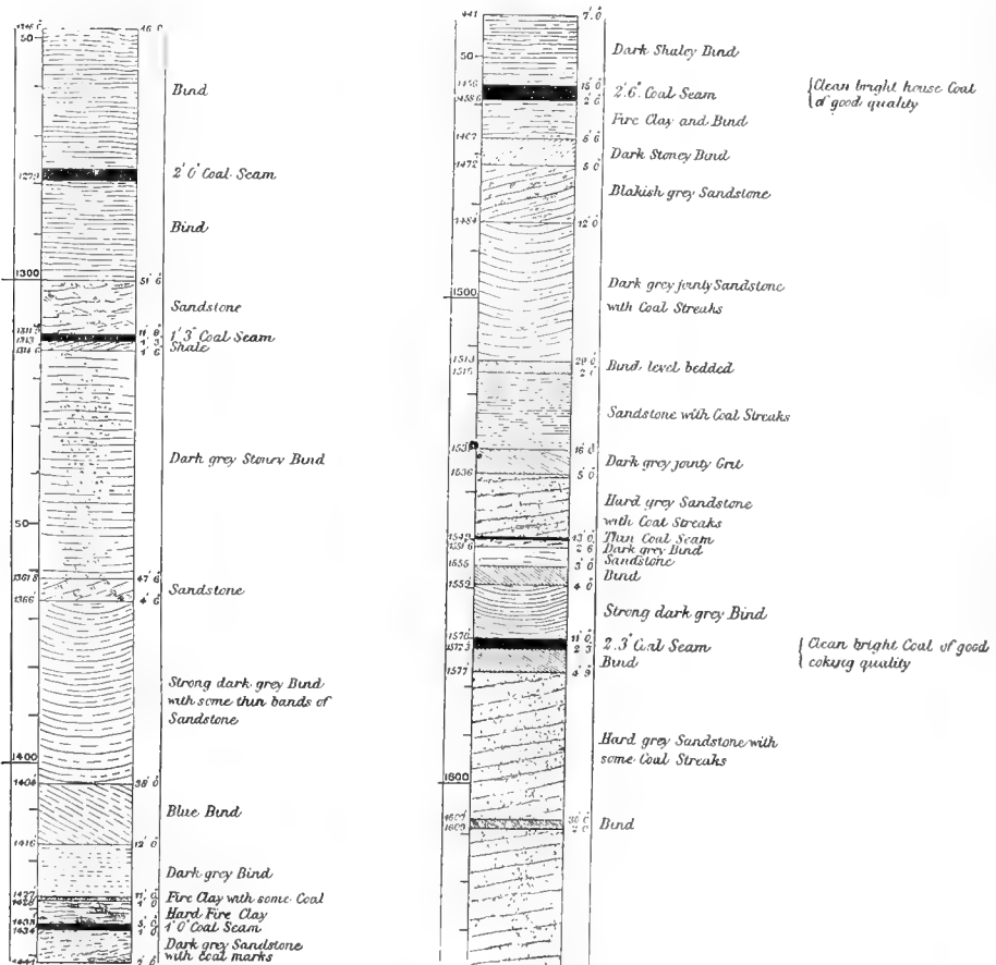
SECTIONS OF BORING, DOVER COLLIERY. (Continued from page 160.)
