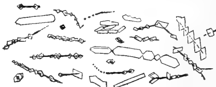
FIG. 2.—MICROSCOPIC CRYSTALS IN OBSIDIAN.
