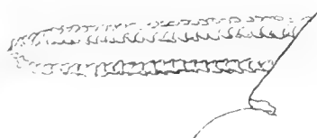
FIG. 5.—PART OF PROBOSCIS OF CHIGOE ( \times 300 ).
