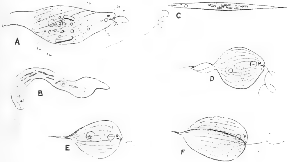
INFUSORIA \times 250 (approx.).
