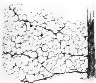
FIG. 1.— Stemonitis splendens —unusual type ( \times 147 ).
