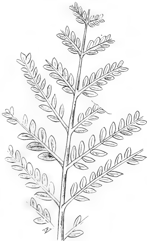
NELLOPTERIS RAVINERVIS. From Upper Coal Measures at Radstock.
