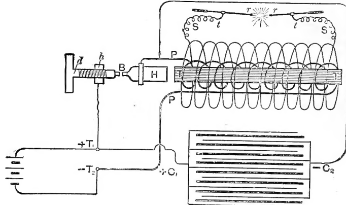
FIG. 6.—DIAGRAM SHOWING CONSTRUCTION OF SMALL INDUCTION COIL AND CONNECTIONS.—(1.)
