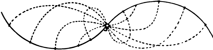
FIG. 28. THE ORIGIN OF A SPIRAL NEBULA, according to Moulton.
