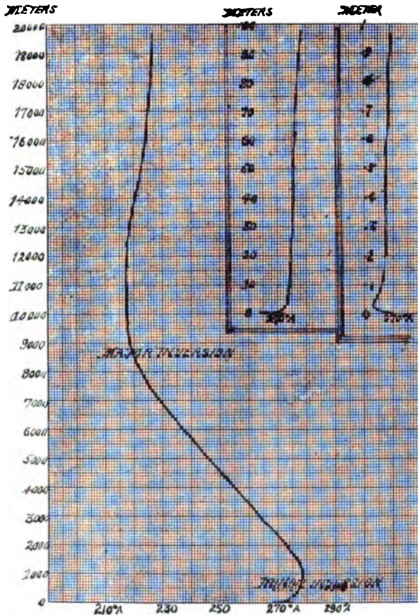
FIG. 1. TEMPERATURE INVERSIONS.
