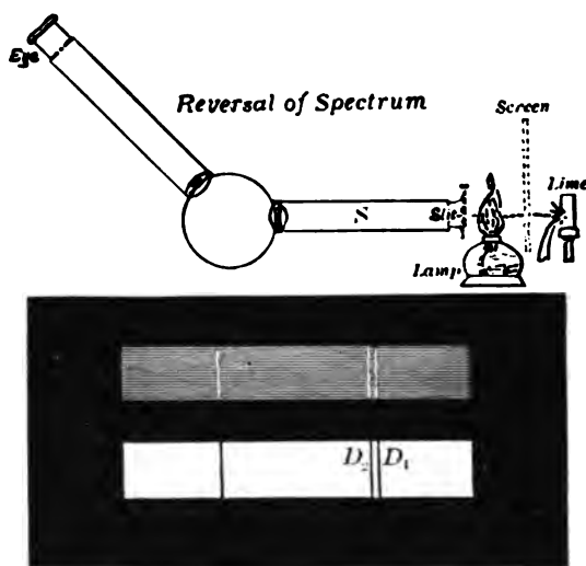
FIG. 12. THE SPECTROSCOPE.
