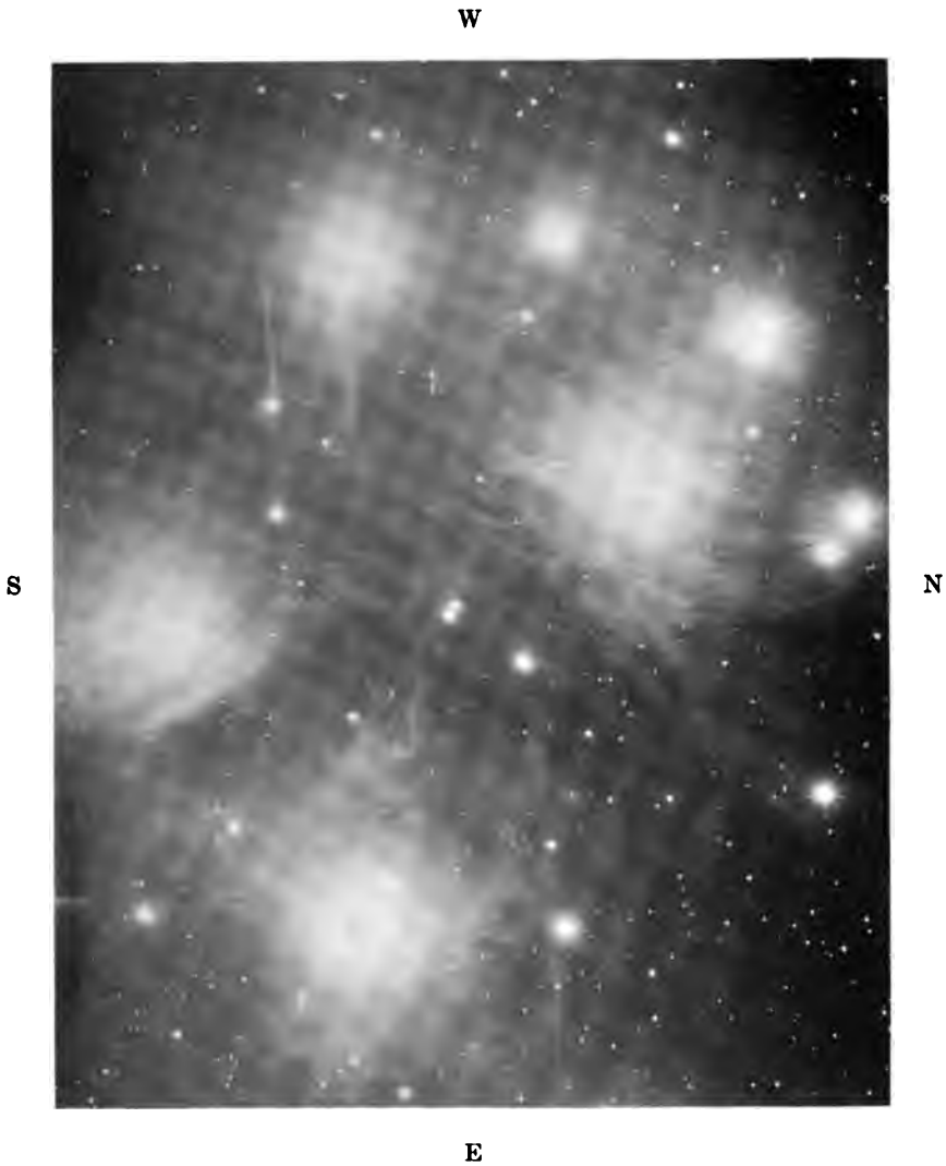
FIG. 20. THE PLEIADES NEBULA. Photographed at the Lick Observatory. ( By engraver's error, the plate is reversed in one direction.)
