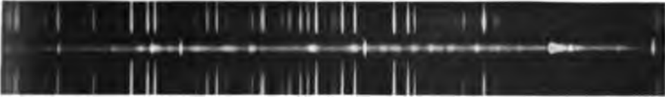
FIG. 21. SPECTRUM OF WOLF-RAYET STAR, PLANETARY NEBULA, B. D. +30.°3630. Photographed at the Lick Observatory.
