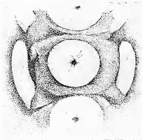
Fig. 4.— Stauroteuthis mawsoni . Sucker 11 of right dorsal arm. \times 36 .
