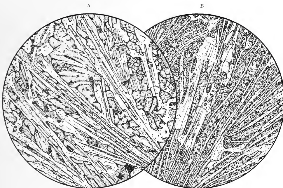
TEXT-FIG. 3.—Variolitic basalts, Carlsberg Ridge. A. \times 68 . Augite-basalt (St. 133, 8); the feldspar occurs as thin untwinned laths, and in places the augite is altered to chlorite (linear shading). B. \times 152 . Oxidized basalt (St. 133, 5); the variolitic character of this basalt can still be made out in spite of its alteration; most of the original glass is oxidized and the brownish alteration product is shown by lighter shading.
