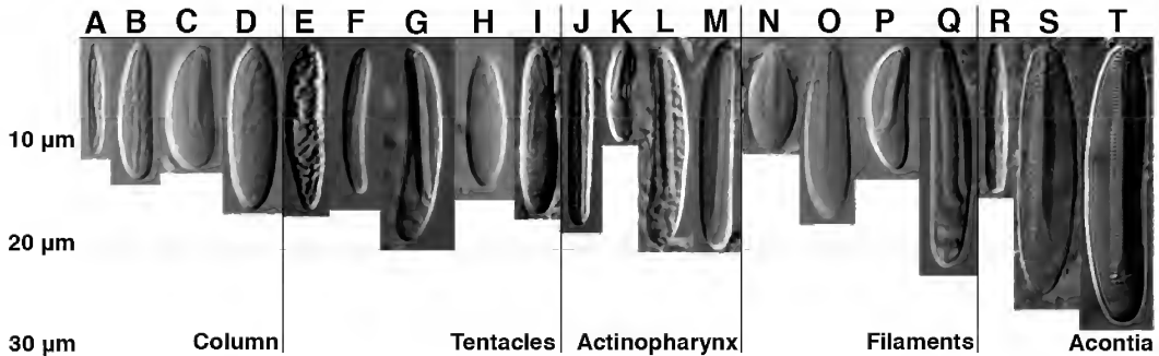
FIG. 5. Cnidom of Diadumene leucolena (Verrill, 1866). A, B, F, J, R, basitrich. C, G, K, L, M, P, Q, S, T, p -mastigophore B2a. D, H, I, holotrich. E, spirocyst. N, O, p -mastigophore B1.
