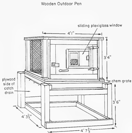
Fig. 4. Wooden sea otter ( Enhydra lutris ) pen. The floor was made of plastic grate, and the walls were made of plywood and herring net. A catch basin beneath the cage drained into a central raceway. These pens were replaced with pens that had pools.
