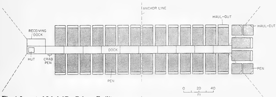
Fig. 4. Layout of Jakolof Pre-Release Facility.
