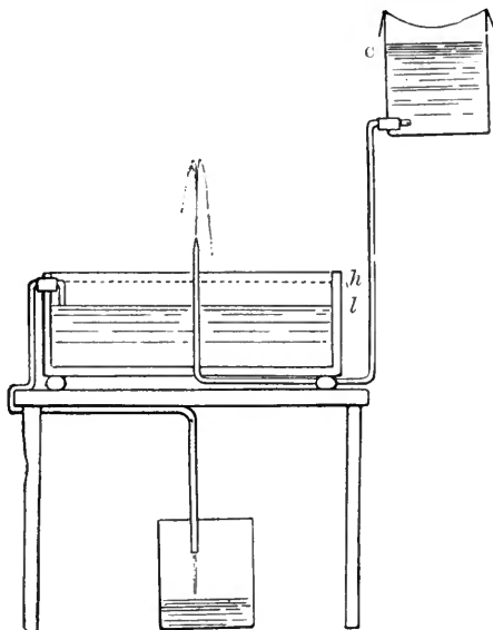
FIG. 39. —AQUARIUM FITTED WITH APPARATUS FOR PERIODIC OUTFLOW
