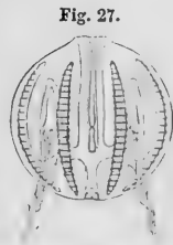
Fig. 27. Pleurobrachia seen at right angles to the plane in which the tentacles are placed. (Agassiz.)
