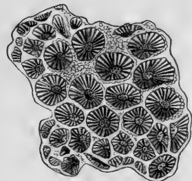
FIG. 6.—DEAD CORAL ( Asteroides calycularis , Milne-Edwards.)—The coral of Fig. 5.
