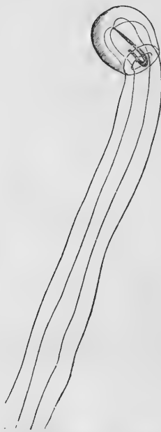
FIG. 11.— Sarsia (Coryne) mirabilis (Agassiz). Adult, Massachusetts Bay.
