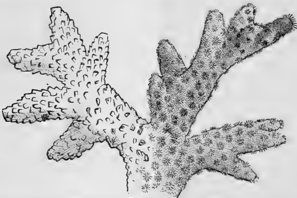
FIG. 7.—MADREPORE CORAL ( Madrepora aspera , Dana). Right-hand branches alive; the left, dead.
