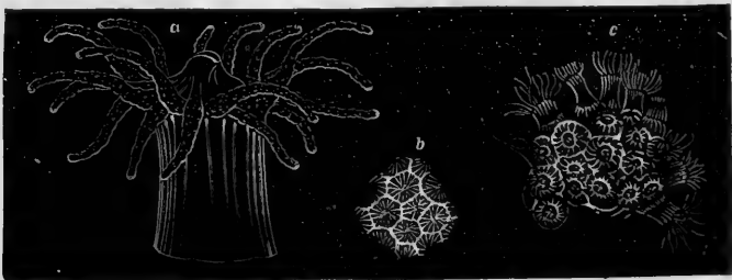
FIG. 8.—DANA'S ASTRANGIA ( Astrangia Danae , Agassiz): c, a growing cluster; a, a single polyp enlarged; b, the dead coral.
