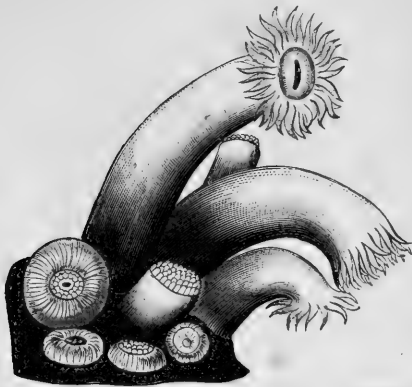
FIG. 5.—CLUSTER OF CORAL-POLYPS ( Asteroides calycularis , Milne-Edwards)—in various stages of expansion.
