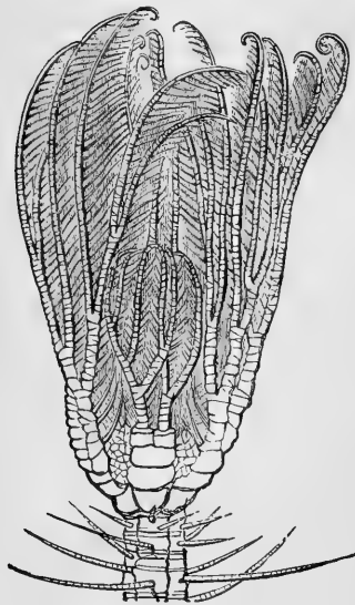
FIG. 25.—CRINOID ( Pentacrinus caput-medusæ ), West Indies.
