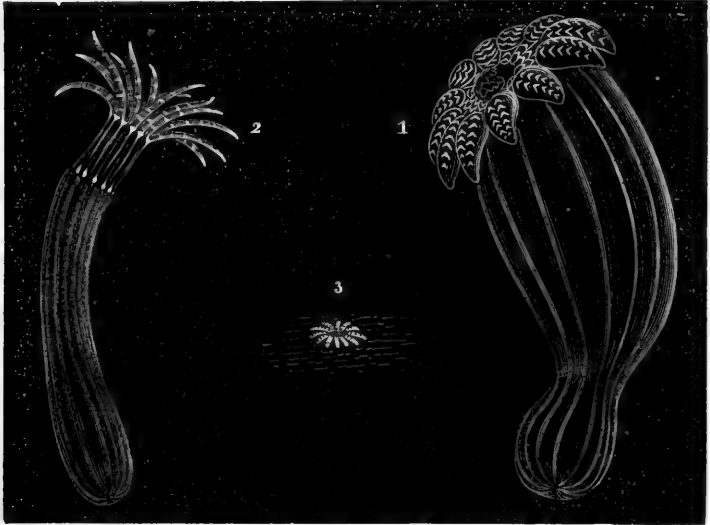
FIG. 2.—ACTINÆ OR SEA-ANEMONES WHICH LIVE IN THE SAND AND ARE OFTEN UNATTACHED. 1. Peachia hastata , Gosse.—2. Edwardsia callimorphia , Gosse.— Halocampa chrysanthellum , Gosse—the last mostly buried in the sand.
