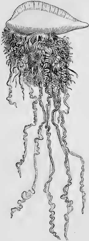
FIG. 15.—PORTUGUESE MAN-OF-WAR ( Physalia arethusa ).
