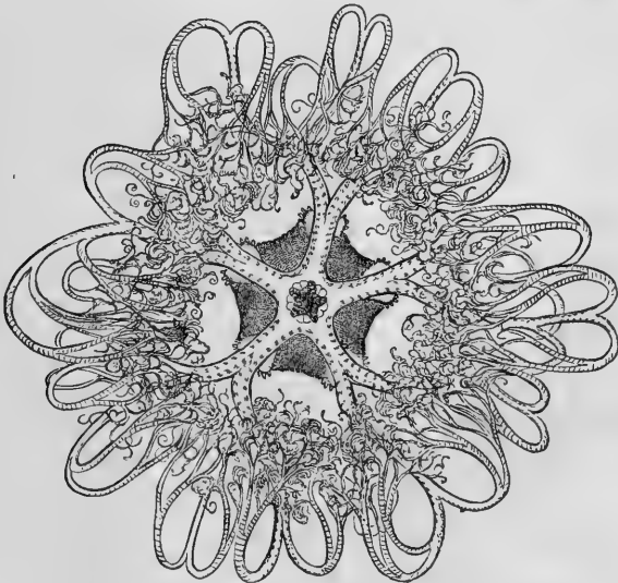
FIG. 24.—“BASKET-FISH” ( Astrophyton Agassizii , Stimpson).
