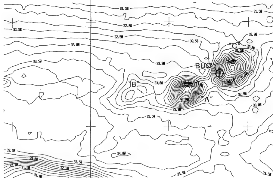
Figure 3-2. Contoured bathymetric chart of WLIS, October 1985. Depth in meters.
