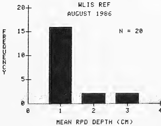
Figure 3-12. Frequency distributions of mean RPD depths at WLIS and WLIS reference.
