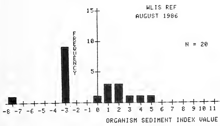
Figure 3-15. The frequency distribution and Organism-Sediment Index values at WLIS and WLIS reference.
