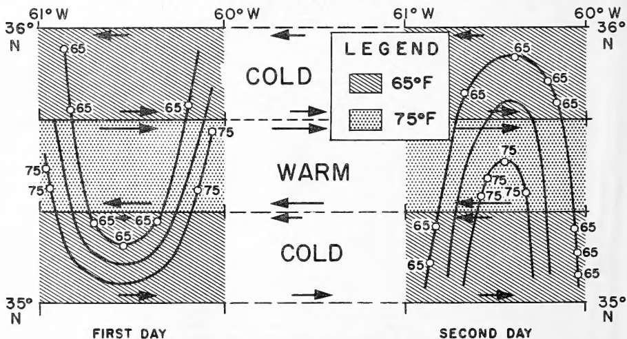
FIGURE 3 SURFACE TEMPERATURE (WAVE) PATTERNS DEDUCED FROM DIFFERENT DATA DISTRIBUTION IN ALTERNATE PARALLEL CURRENTS IN THE SAME AREA ON SUCCESSIVE DAYS
