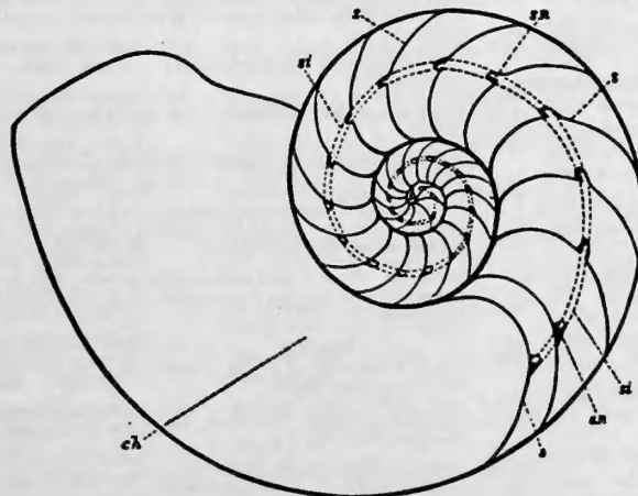
— Nautilus pompilius L., in section, showing the septa (s, s), the septal necks (s.n., s.n.), the siphuncle dotted in (si), and the large body chamber (cA).
