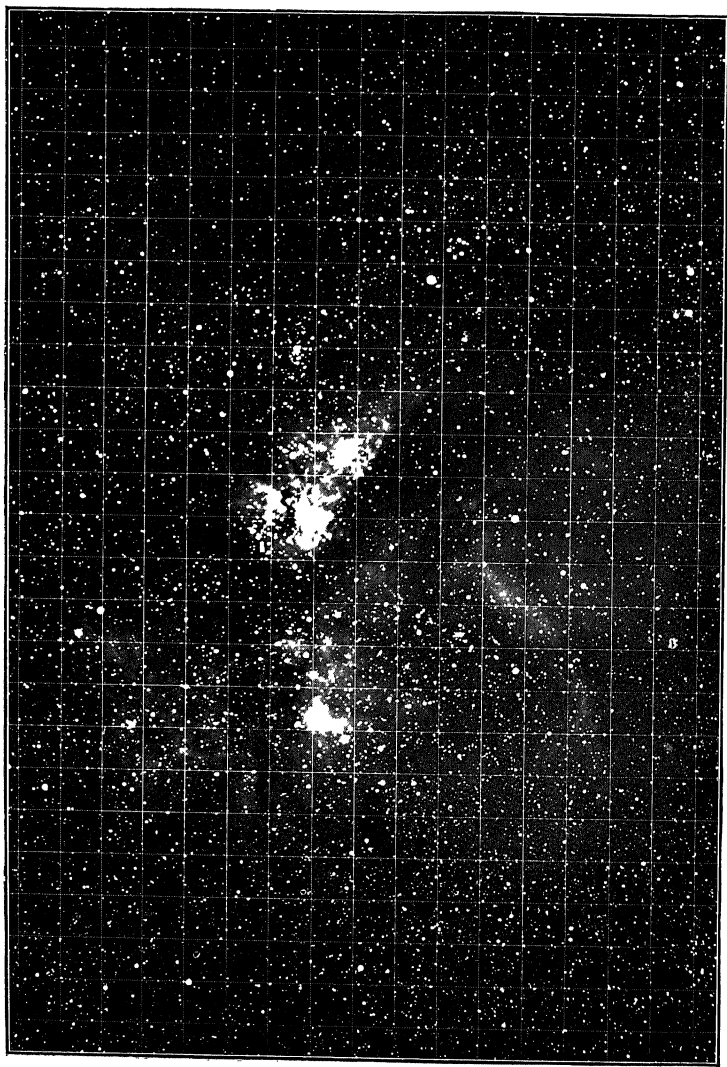
FIG 100—The nebula about \eta Aigittis From a photograph by Dr Gill
