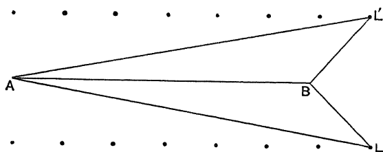
FIG. 84 —Illustrating the effect of the sun's motion in space
