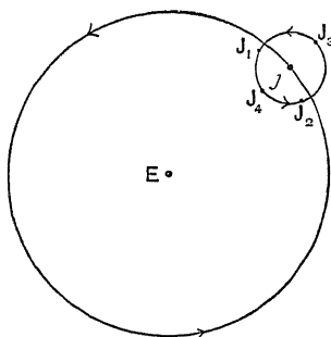
FIG. 34—Jupiter's epicycle and deferent
