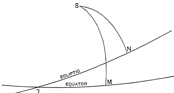
FIG. 14.—The equator and the ecliptic.
