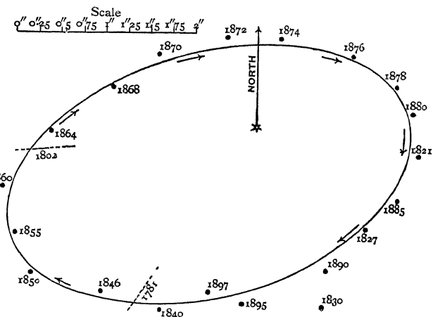
FIG. 101.—The orbit of \xi Ursae , shewing the relative positions of the two components at various times between 1781 and 1897 (The observations of 1781 and 1802 were only enough to determine the direction of the line joining the two components, not its length.)
