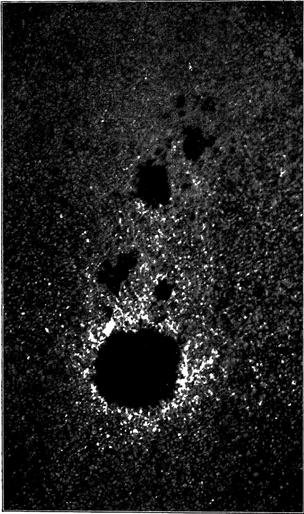
Fig 96.—A group of sun-spots From a photograph taken by M Janssen at Meudon on April 1st, 1894 [To face p 385
