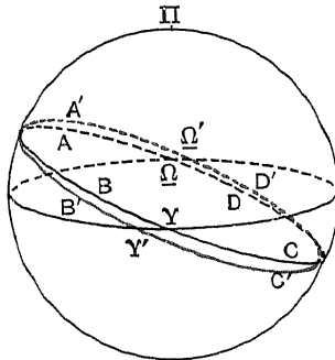
FIG. 23 —The precession of the equinoxes
