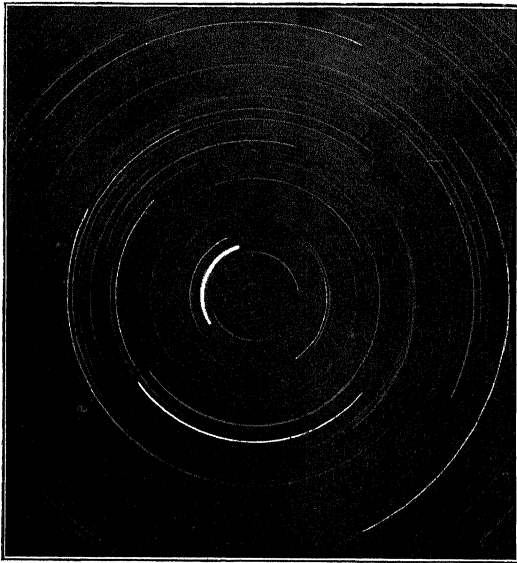
FIG 2 --The paths of circumpolar stars, shewing their movement during seven hours. From a photograph by Mr. H. P. Pan. The thickest line is the path of the pole star. [To face p. 8]
