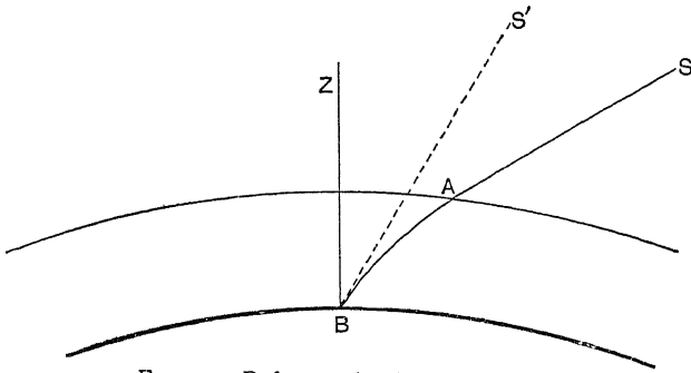
FIG. 32.—Refraction by the atmosphere
