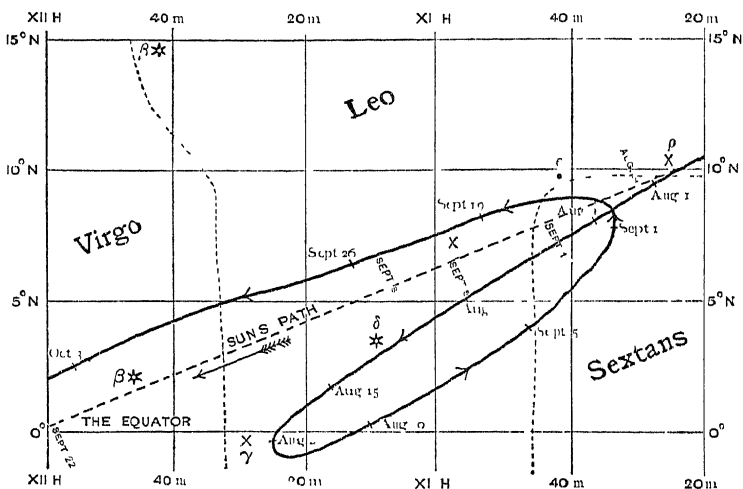
Fig 7—The apparent path of Mercury from Aug 1 to Oct 3, 1898. The dates printed in capital letters show the positions of the sun; the other dates show those of Mercury.
