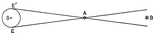
FIG. 57 — The differential method of parallax
