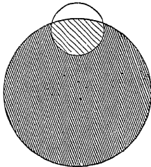
FIG 28 —Partial eclipse of the moon
