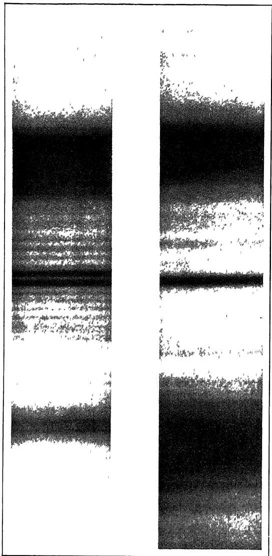
FIG 103—The spectrum of \beta Amiga , shewing the K line single and double
