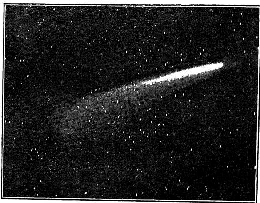
FIG 99 —The great comet of 1882 (11) on November 7th From a photograph by Dr. Gill [To face p 393
