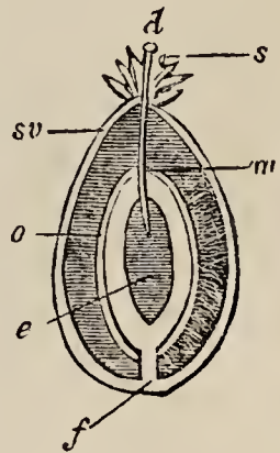
FIG. 27. Seed-vessel of nettle. s , Stigma ; sv , Covering of seed-vessel ; o , Ovule ; e , Embryo ; f , Funicle ; m , Micropyle ; d , Grain of pollen dust.
