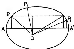
The three normals to the ellipse. Apollonius.
