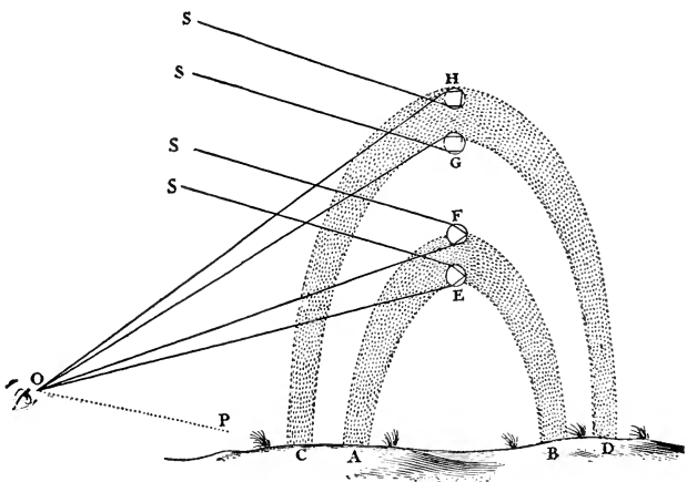
NEWTON'S THEORY OF THE RAINBOW (Opticks, 1704).
