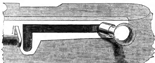
UNDER SIDE OF PRINCE'S RIFLE.
