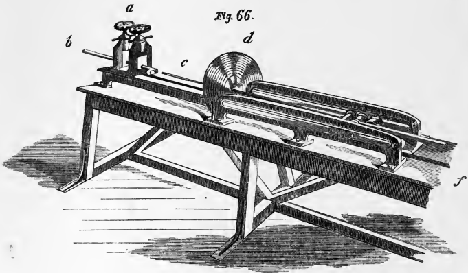
RIFLING MACHINE.
