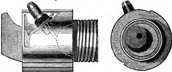
THE GREENER-HORTON BREECH. (FULL SIZE.)
