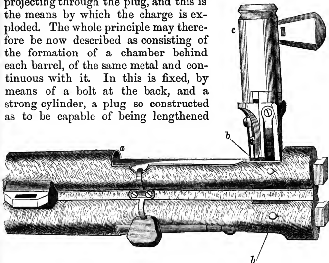
FIG. 42. UNDER SURFACE OF BARRELS. THE LEFT OPENED FOR INSERTION OF CARTRIDGE; THE RIGHT CLOSED. (HALF SIZE.)
