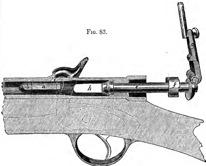
SECTION OF TERRY AND CALISHER'S RIFLE.
