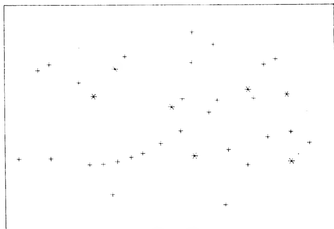
Pleiades; 30 Stars
