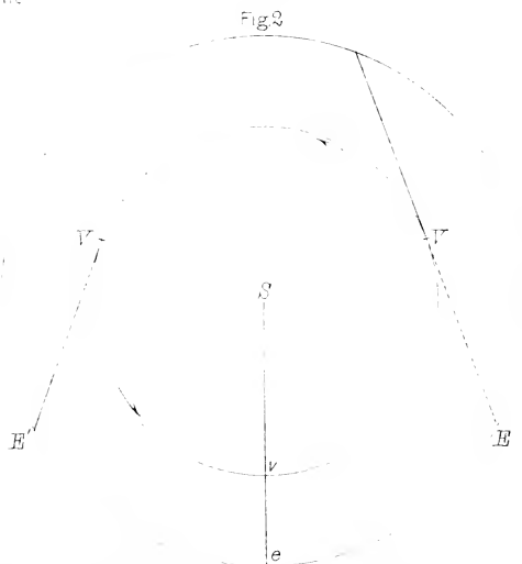
Fig 2. S the Sun, centre of solar system v, e positions of planet and Earth at conjunction V, V' stationary points of planet E, E' corresponding positions of the Earth
