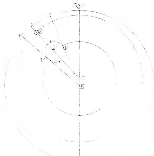
Fig 1. E the Earth (centre of universe) S the Sun C centre of eccentric D centre of planet's epicycle V, V' stationary points S, V, V' projections of S, V, V' in the ec. of which E is the centre
