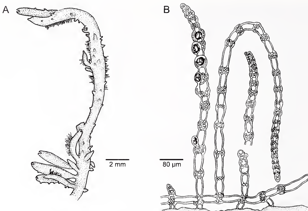
FIGURE 84. Species of Ceramium . A. Ceramium obesum : Specimen from the type collection displaying stout forcipate apices, thick and complete cortication, and numerous rhizoids (after Dawson, 1962a: pl. 22: fig. 5). B. Ceramium serpens : Erect axes with tetrasporangia above prostrate axes attached to substratum (after Dawson, 1962a: pl. 25: fig. 6).
