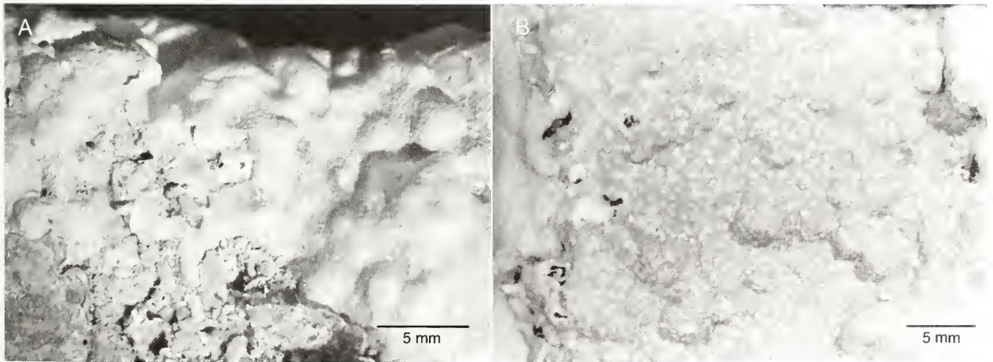
FIGURE 60. Litbothamnion microsporum : Surface view of two crusts. A. JN-3532; B. JN-3462 (both US Alg. Coll.).
