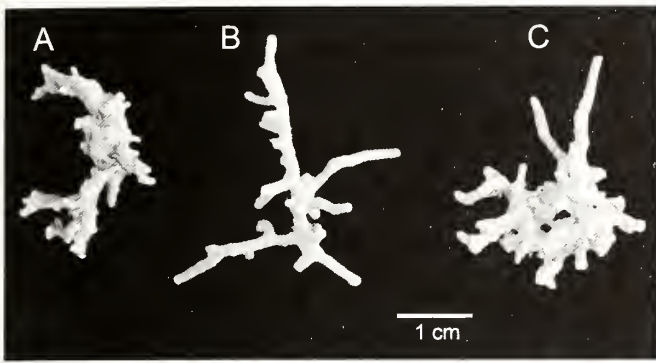
FIGURE 59. Litbothamnion australe : Free-living rhodoliths, sub-cylindrical branches with a wide range of forms. A, B. EYD-61-40; C. EYD-593a (AHFH, now UC).
