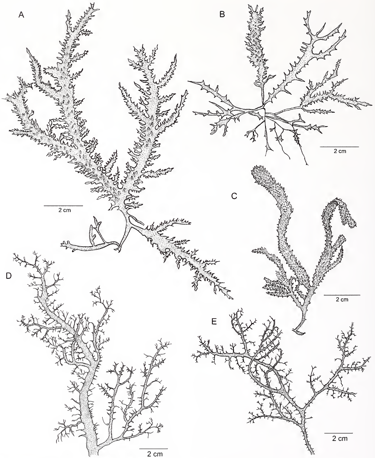
FIGURE 162. Chondracanthus squarrosus : Several thalli showing morphological variability. A. Habit (JN-3690, US Alg. Coll.-159405). B. Habit (JN-3690, US Alg. Coll.-159404). C. Habit (previously " Gigartina macdougalii ") (JN-3298, US Alg. Coll.-159444). D, E. Portions of two thalli (previously " G. pectinata ") (D, JN-3026, US Alg. Coll.-159487; E, JN-2982, US Alg. Coll.-159463).
