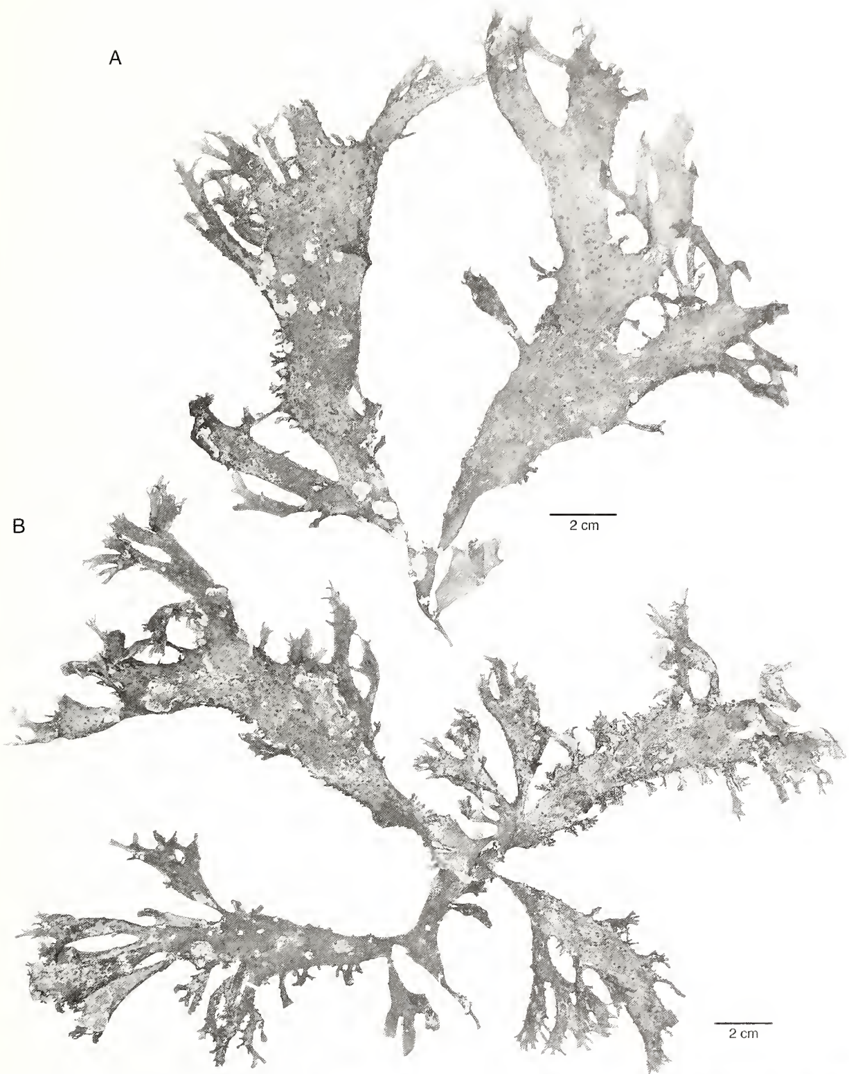
FIGURE 194. Gracilaria rubriumbra , two specimens showing morphological variability: A. Flat and wide thallus. B. Thallus with numerous finely divided and somewhat dentate marginal proliferations (A, B, both JN-3032: A, US Alg. Coll.-159638; B, US Alg. Coll.-159637).
