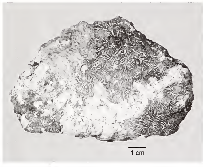
FIGURE 183. Cruoriella fissurata : Habit of the crust on rock (type specimen: EYD-6830a, AHFH, now UC).
