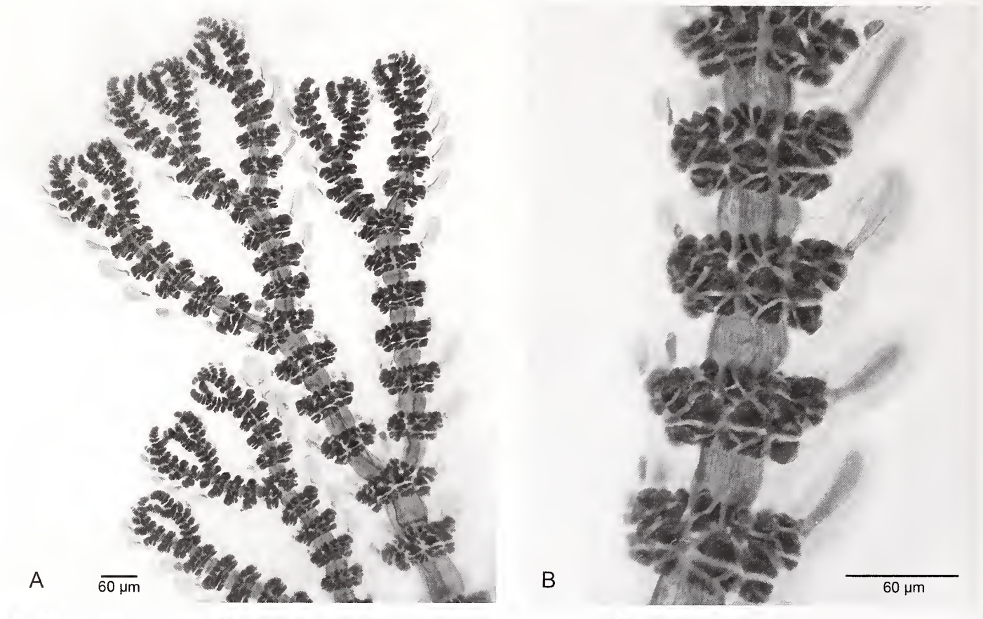
FIGURE 90. Gayliella fimbriata : A. Habit of erect axes, with series of protruding gland cells on abaxial side. B. Mature cortical pattern with clavate gland cells, some whorled about node (A, B, JN-5062, US Alg. Coll. microscope slide 5263).
