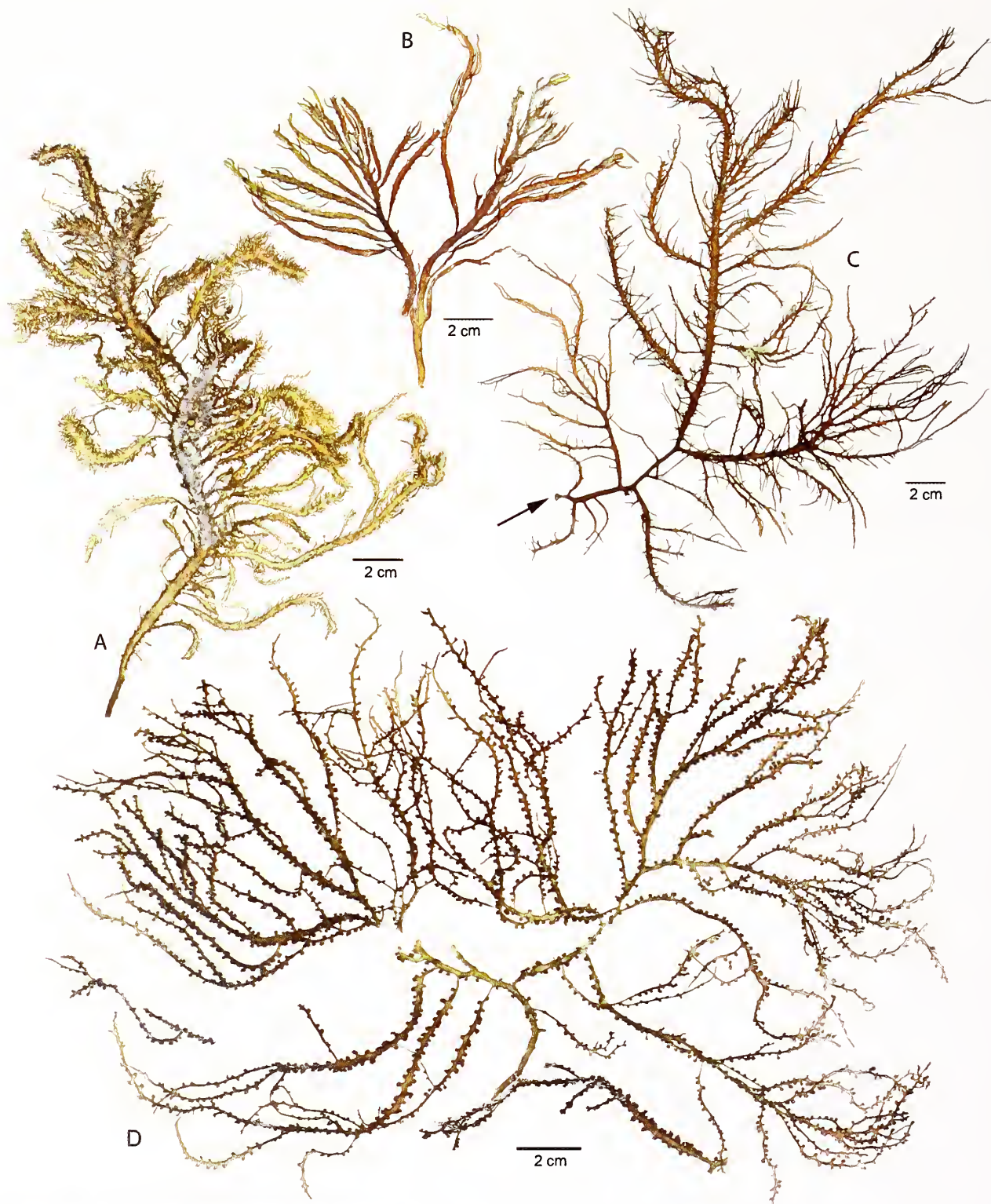
FIGURE 180. Tacanoosca gen. nov., habit variation in T. uncinata : A. Male gametophyte (EYD-1800a, US Alg. Coll.-7181). B. Tetrasporophyte (JN-238, US Alg. Coll.-89992). C. Thallus with spinose laterals and holdfast (arrow) (JN-5415, US Alg. Coll.-210494). D. Female gametophyte with protuberant cystocarps (EYD-1800b, US Alg. Coll.-7181).
