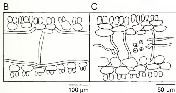
FIGURE 181. Species of Weeksia . A, B. Weeksia coccinea : A. Habit (JN-6546, US Alg. Coll.-159943). B. Diagrammatic transection of Weeksia coccinea . C. Weeksia templetonii : Diagrammatic transection.
