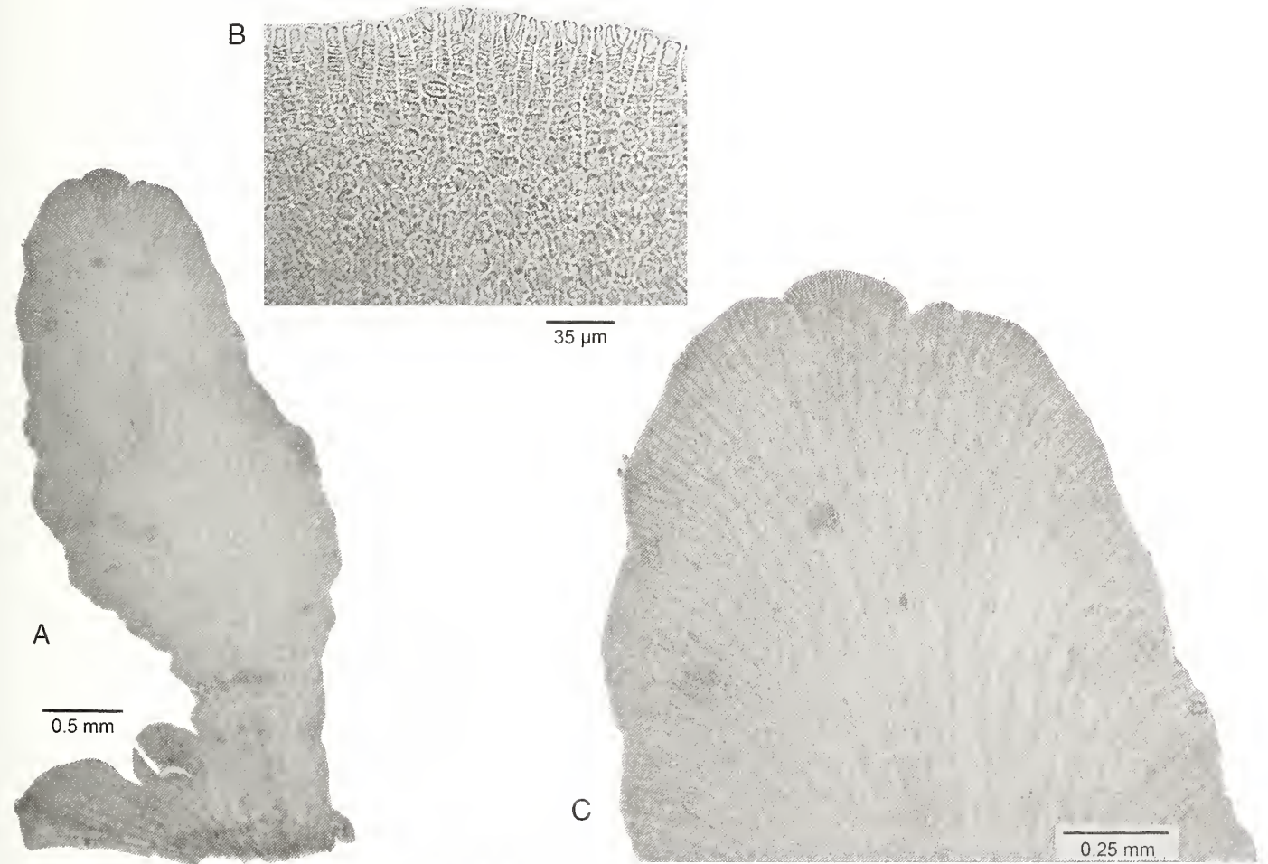
FIGURE 139. Amplisiphonia? pacifica : A. Habit of small blade. B. Margin of numerous apical cells that initiate polysiphonous axes that laterally unite behind the margin to form the flat blade. C. Dorsal surface view of blade with internal pattern of fine veins (axial filaments) (A–C, JN-4682, US Alg. Coll. microscope slide 4984).
