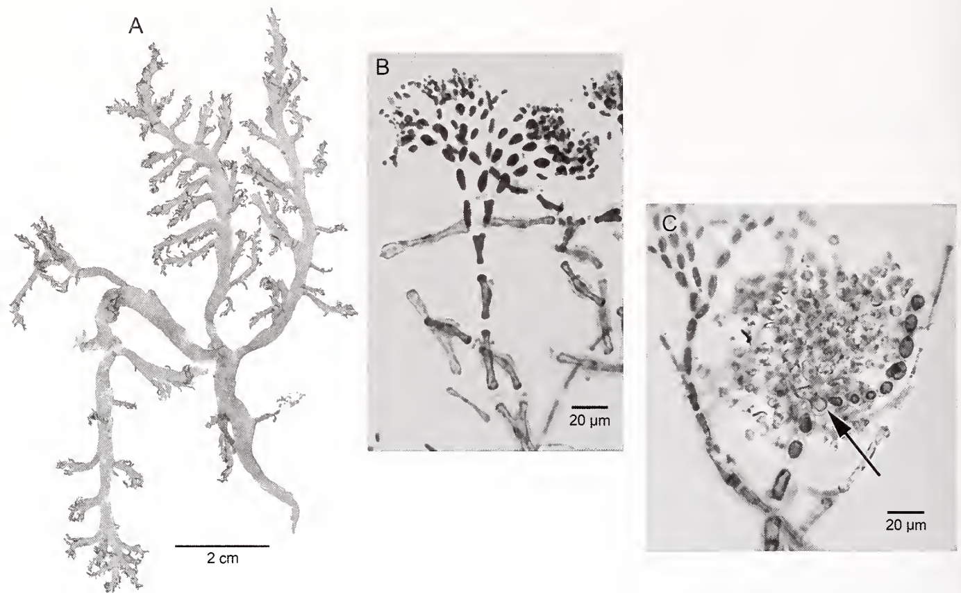
FIGURE 160. Dudesnaya colombiana : A. Habit (JN-5480, US Alg. Coll.-8760). B. Spermatangia at tips of cortical filaments (JN-5680, US Alg. Coll. microscope slide-3767). C. Mature carposporophyte on auxiliary cell (arrow) filament (JN-5480, US Alg. Coll. microscope slide_3769).
