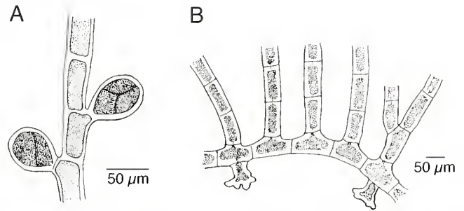
FIGURE 145. Lejolisia boshawii (holotype): A. Tetrasporangia borne on erect filaments. B. Portion of creeping filament to show attachment structures and erect axes (A, B, after Dawson, 1966b: figs. 6J, K).
