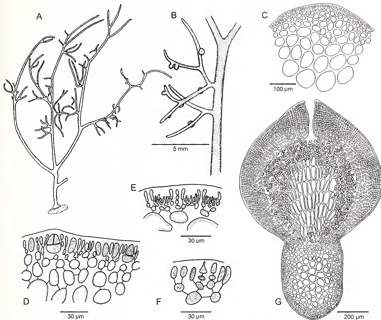
FIGURE 193. Type collection of Gracilaria ramiscunda : A. Habit of tetrasporangial alga (after Dawson 1949a: pl. 3: fig. 1). B. Part of a cystocarpic thallus (after Dawson 1949a: pl. 4: fig. 1). C. Transverse section of axis showing gradual transition from cortex to medulla. D. Transverse section of a tetrasporic branchlet showing modified cortex. E. Transverse section of spermatangial thallus showing spermatangia in shallow pits. F. An example of a carpogonial branch; others may bear more or fewer branches off carpogonial branch cells (C–F after Dawson 1949a: pl. 3: figs. 4–6, 8). G. Transverse section of bearing branch and mature cystocarp showing the fusion cell, pseudoparenchymatous gonimoblast, and numerous traversing filaments to the pericarp (After Dawson, 1949a: pl. 5: fig. 2).
