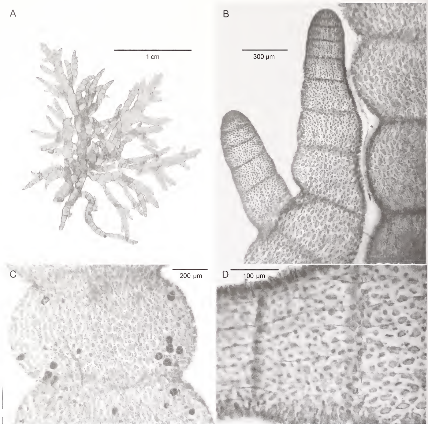
FIGURE 222. Champia cf. parvula : A. Habit, showing branching pattern and segments at consistent intervals (JN-5311, US Alg. Coll.-158921). B. Branch originating from septal region and intermixed cortical pattern of larger cells cutting off small cells. C. Surface view of tetrasporangia scattered in cortex. D. Several segments with focus on the longitudinal filaments connecting with monostromatic septa cell layer (note orientation of this figure is perpendicular to the previous figures; B-D, JN-4001, US Alg. Coll. microscope slide 4583).
