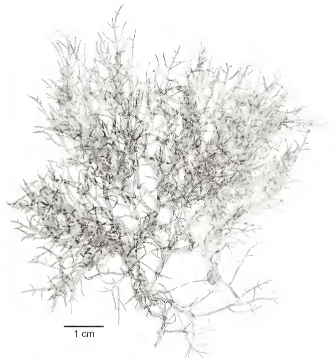
FIGURE 230. Lomentaria bakodatensis : Habit (EYD-10896, US Alg. Coll.-12228).
