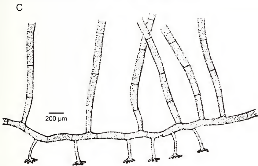
FIGURE 146. Species of Tiffaniella . A, B. Tiffaniella saccorbiza : A. Erect filaments arising from creeping portion attached by distinctive inflated rhizoids. B. Polysporangia on lateral branches off erect filaments (A, B, EYD-46-1330, US Alg. Coll. microscope slide 917). C, D. Tiffaniella snyderae : C. Erect filaments arising from creeping portion showing rhizoids. D. A group of developing polysporangia (C, D, after Dawson, 1962a: pl. 16: figs. 4, 3).
