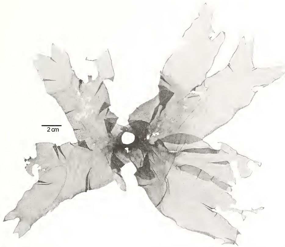
FIGURE 167. Mazzaella bancockii : Habit (JN-5563, US Alg. Coll.-160803).
