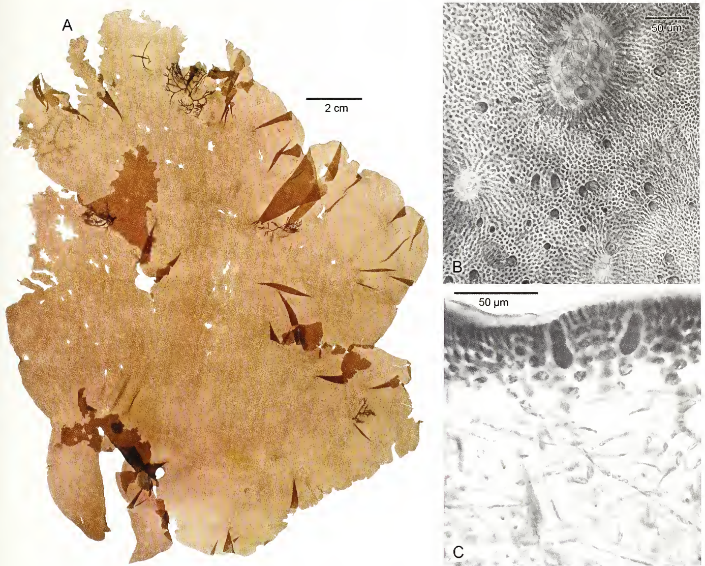
FIGURE 218. Schizymenia pacifica : A. Habit (female gametophyte) (JN-5759, US Alg. Coll.-160898). B. Surface view showing gland cells in cortex and several carpospores of cystocarps, the largest with carposporangia visible within (JN-5747c, US Alg. Coll. microscope slide 4524). C. Portion of transection showing elongate gland cells terminating cortical filaments (JN-5747, US Alg. Coll. microscope slide 4526).
