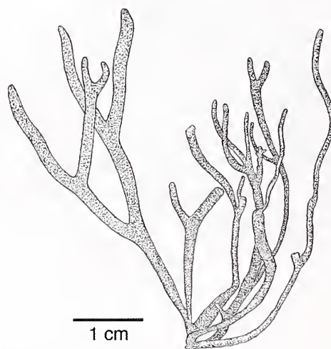
FIGURE 172. Abnfeltiopsis serenei : Part of a tufted plant (EYD-12058; after Dawson, 1954: pl. 3: fig. 6, as Gymnogongrus serenei ).
