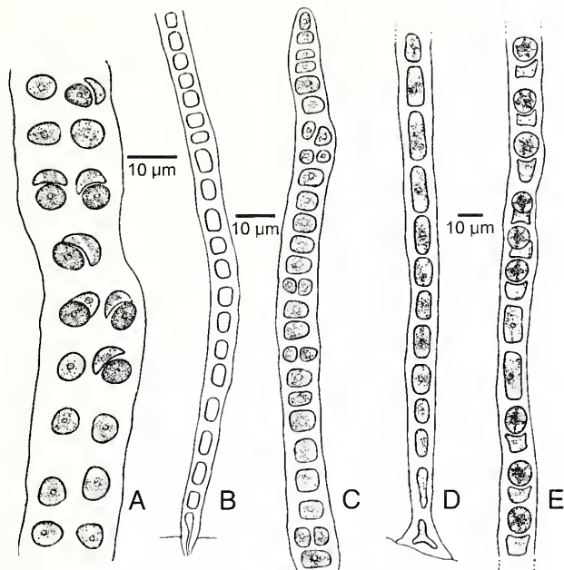
FIGURE 12. Species of Erythrotrichia . A–C. Erythrotrichia biseriata : A. Part of a filament with monosporangia. B. Basal portion of young filament with elongate basal cell. C. Upper part of biseriate filament (A–C after Tanaka, 1952: fig. 8E, F, H). D, E. Erythrotrichia carnea f. tenuis : D. Basal portion of young filament. E. Mature filament with monosporangia (D, E after Tanaka, 1944: fig. 13).
