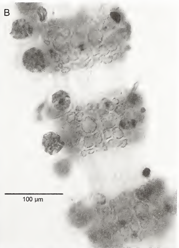
FIGURE 75. Ceramium aduncum : A. Upper portion with circinate apices and conspicuous gland cells ( JN-5060 , US Alg. Coll. microscope slide 8701). B. Several emergent tetrasporangia (with a thick hyaline envelope), borne off one side of node ( JN-3098 , US Alg. Coll. microscope slide 8690).
