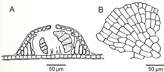
FIGURE 55. Heteroderma subtilissima : A. Transection through mature tetrasporangial conceptacle. B. Surface view of portion of crust (A, B, after Dawson, 1960a: pl. 49: figs. 5,6).
