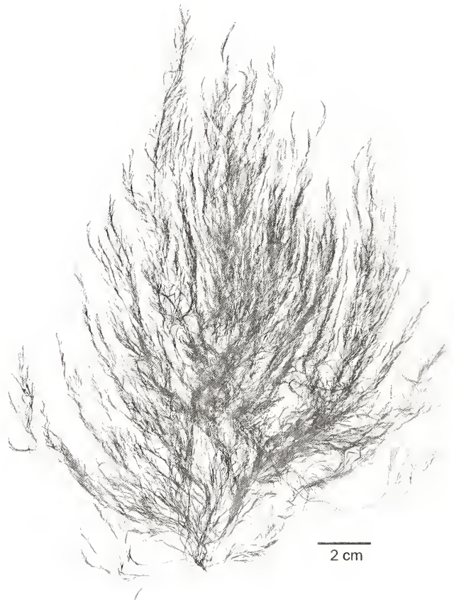
FIGURE 133. Neosiphonia paniculata : Habit (JN-4552, US Alg. Coll.-160578).
