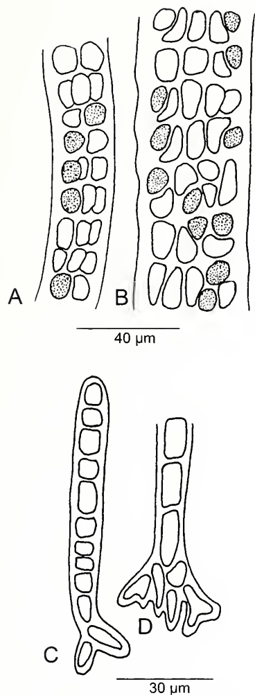
FIGURE 14. Erythrotrichia tetraseriata : A, B. Portion of mature filaments seen with sporangia. C. Young filament with attaching cells. D. Basal portion with multicellular attachment structure (A–D after Kylin, 1941: fig. 1A–D, as Erythrotrichia californica ).
