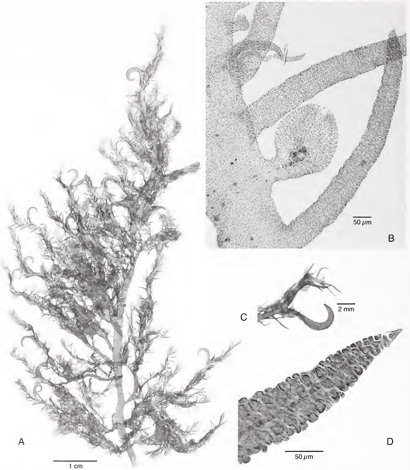
FIGURE 65. Bonnemaisonia hamifera : A. Habit (gametophyte) with hook-shaped branchlets for entangling attachment (JN-5438, US Alg. Coll.-158653). B. Branch with developing and young cystocarps terminating short branches (JN-2989, US Alg. Coll. microscope slide 4277). C. Close-up of a hook branchlet (from A; JN-5438). D. Ultimate branchlet showing central axial filament surrounded by cortical cells, tapering to acute apex (JN-2989, US Alg. Coll. microscope slide 4277).
