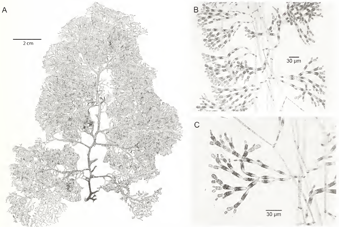
FIGURE 31. Liagora magnivolucra : A. Habit of gametophyte (R.D. Staker, s.n., US Alg. Coll.-204280). B, C. Slender longitudinal medullary filaments bearing subdichotomously branched anticlinal assimilatory filaments that form the cortex (JN-4046, US Alg. Coll. microscope slide 4283).
