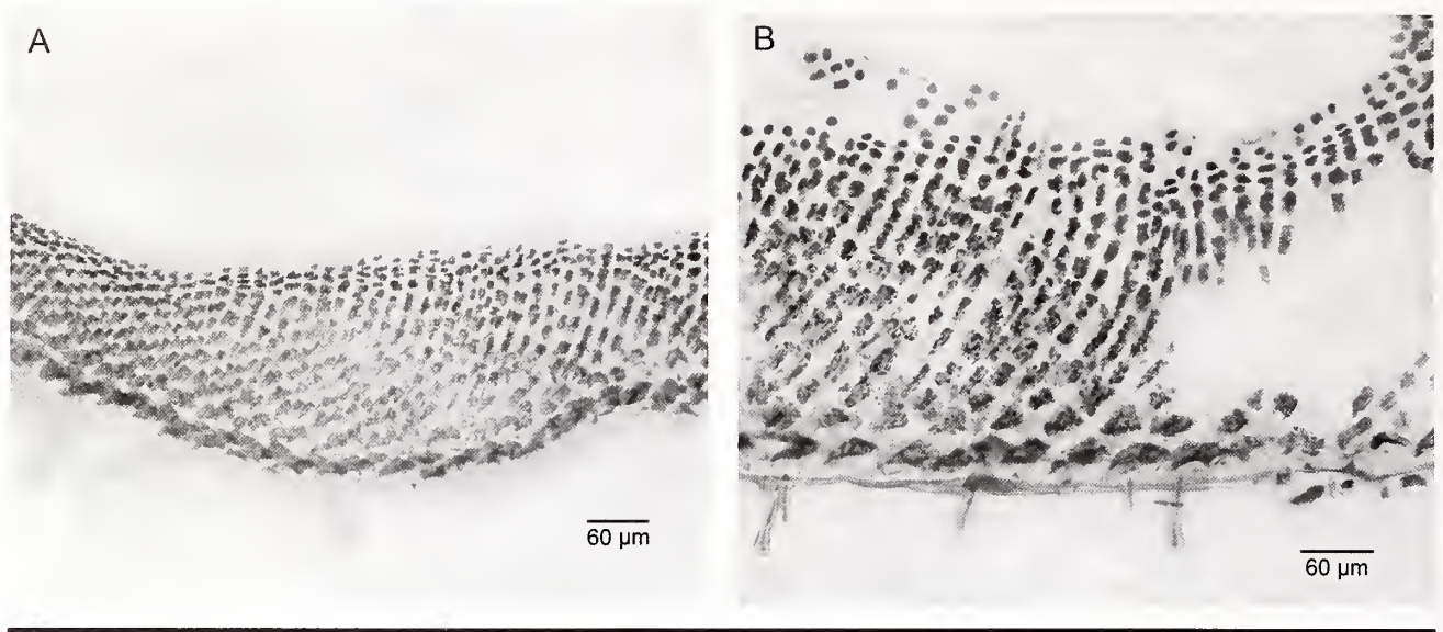
FIGURE 185. Metapeyssonnellia mexicana : A, B. Vertical sections, showing some unicellular rhizoids, and the perithallus of more or less assurgent filaments that become slightly more vertical near crust surface (GJH-67-54, US Alg. Coll. microscope slide 3109).
