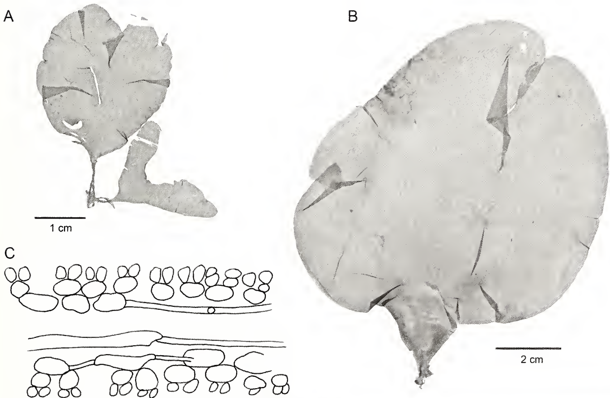
FIGURE 205. Cryptonemia obovata : A. Habit of small blade (JN-4729, US Alg. Coll.-158996). B. Habit of large blade (EYD-21577, US Alg. Coll.-7069). C. Diagrammatic transection of C. obovata .
