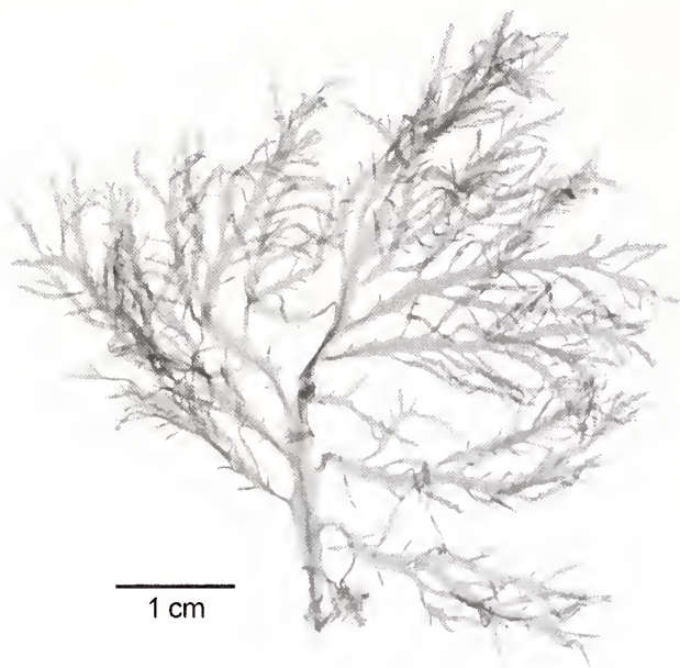
FIGURE 106. Erythroglossum californicum : Habit (JN-6578a, US Alg. Coll.-217358).
