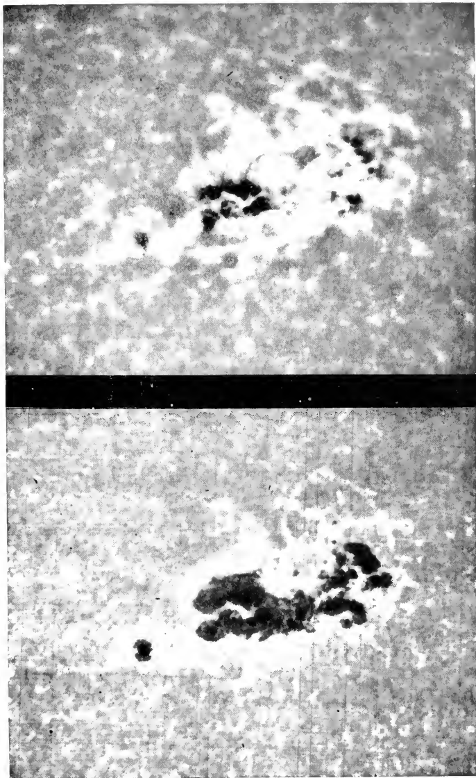
FIG. 2 October 9, 3 h 30 m . Calcium flocculi as shown with second slit set on H 2
