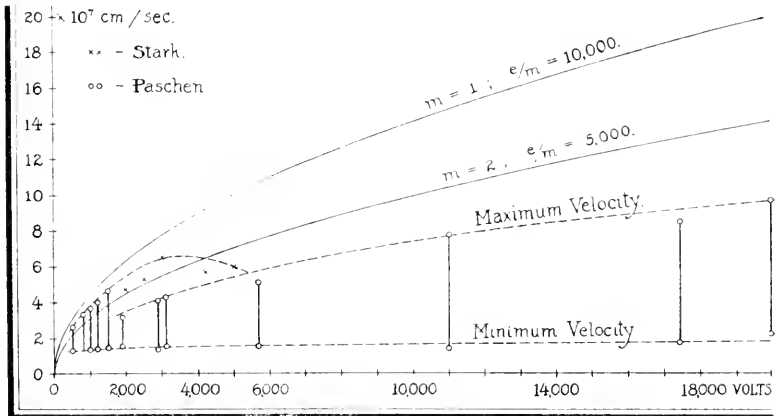
FIG. 61.—Range of velocities of sources of H lines as a function of the cathode fall in volts. Full lined curves are calculated, using formula (1).
