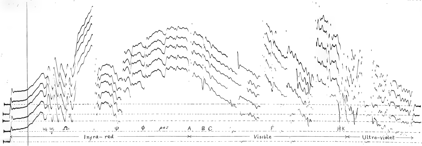
P. 4 graphs of the Solar Energy Spectrum. Observed at Montezuma, Colo. July 7, 1924. Precipitable water 103 centimeters.
