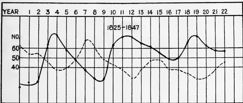
FIG. 30.—7½-year sun-spot cycle. Means of 3 cycles, showing apparent inversion.
