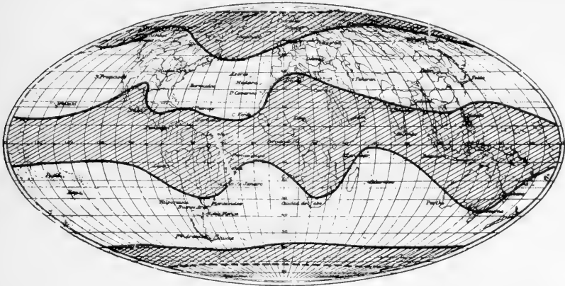
FIG. 2.—Zonal effect of increased solar activity. Shaded areas show regions where the pressure falls and the temperature rises with short period changes of solar radiation. Unshaded areas show regions where the reverse conditions occur.
