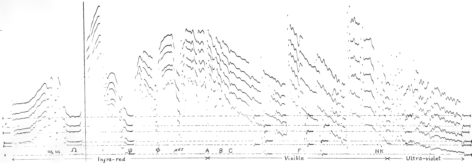
Diagrams of the Solar Energy Spectrum. Observed at M. Azunus, Chile, March 18, 1925. Precipitable water, 1.47 centimeters.
