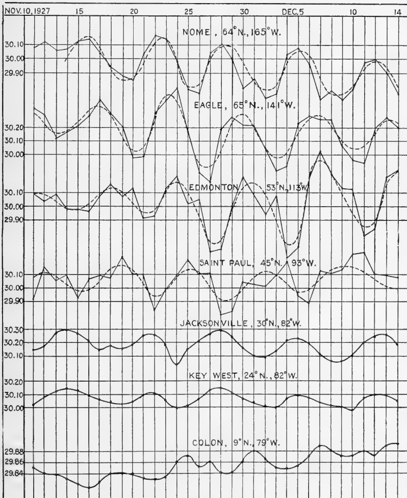
FIG. 12.—7-day pressure wave.
