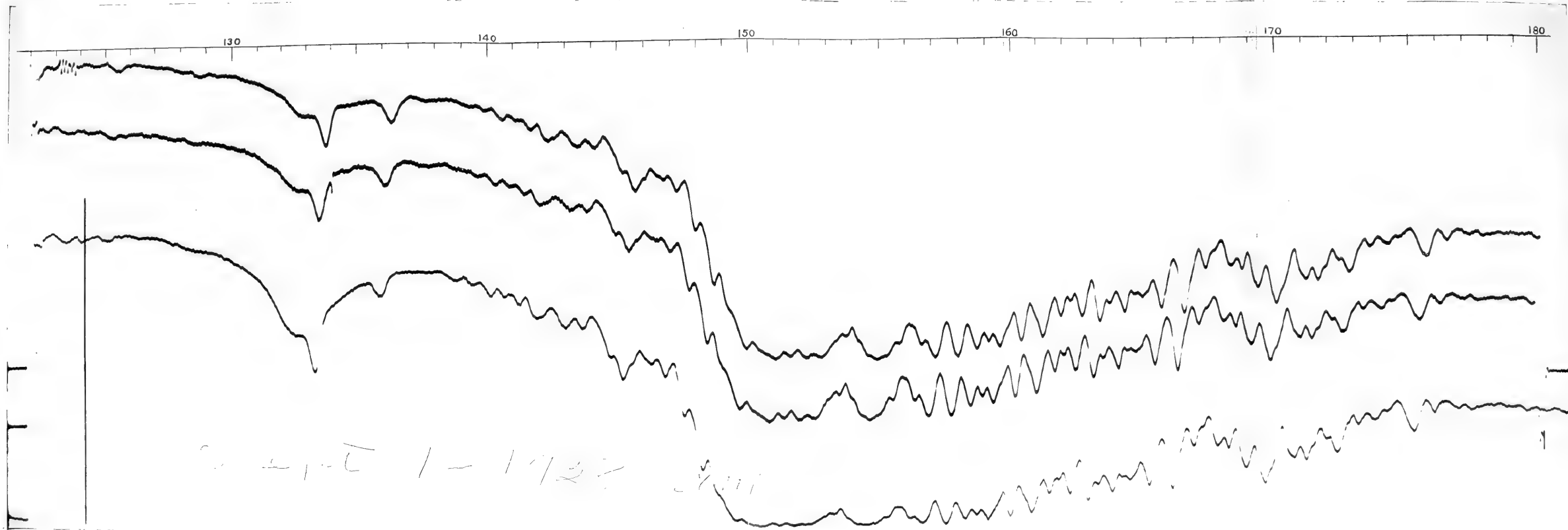
PHOTOGRAPHS OF THE ISAACS-RICE DISMATIC SOLAR SPECTRUM The \gamma region, Wave lengths 1200 to 1800 Angstroms
