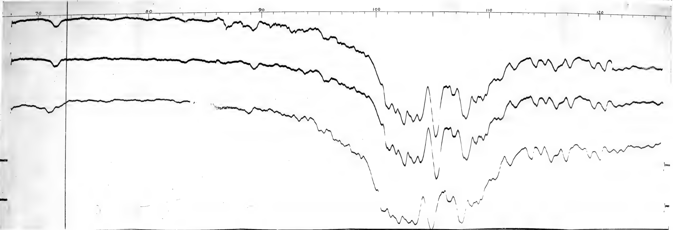
Electron spectra of the INDIAN P... AND S... The ... .. 12200 Angstroms
