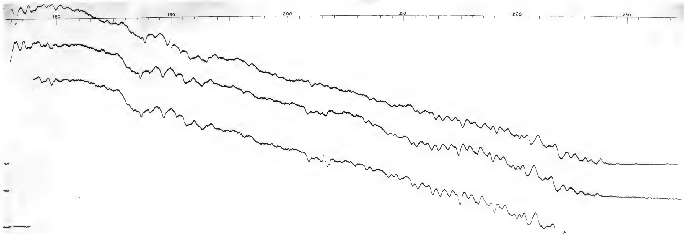
FIG. 1. SOLAR SPECTRUM Wavelengths in Angstroms
