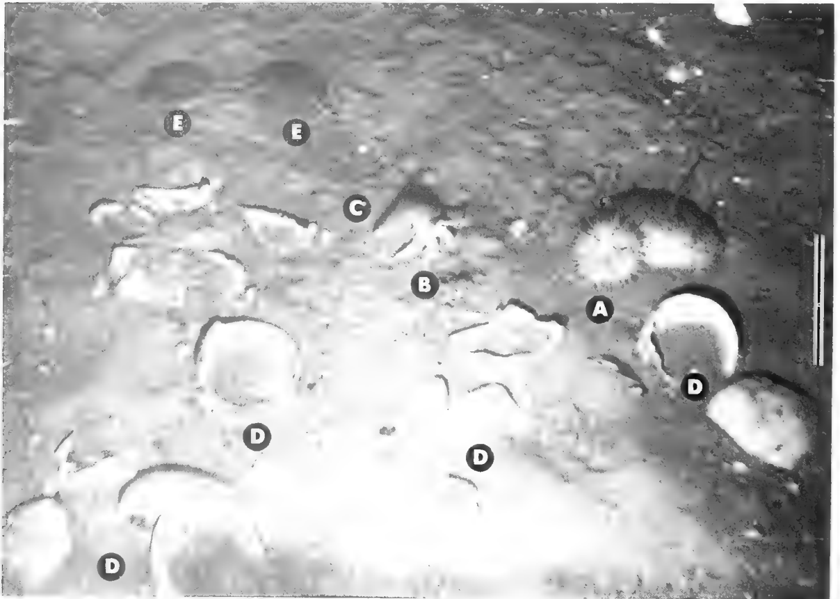
Figure 6.--Sea floor at station 45, southeastern Georges Bank, water depth 82 m. Identifiable animals: A. green sea urchin, Strongylocentrotus drobachiensis ; B. Acadian hermit crab, Pagurus acadianus ; C. Stimpson's distaff shell, Colus stimpsoni ; D. ocean quahog; E. sand dollar. Scale bar is 10 cm. long.
