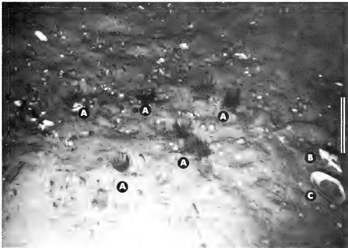
Figure 5.--Sea floor at station 44, southeastern Georges Bank, water depth 64 m. Identifiable animals: A. burrowing sea anemone, Cerianthus borealis ; B. waved whelk, Buccinum undatum ; C. surf clam, Spisula solidissima ; plus numerous tubes of polychaetes and amphipods. Scale bar is 10 cm. long.
