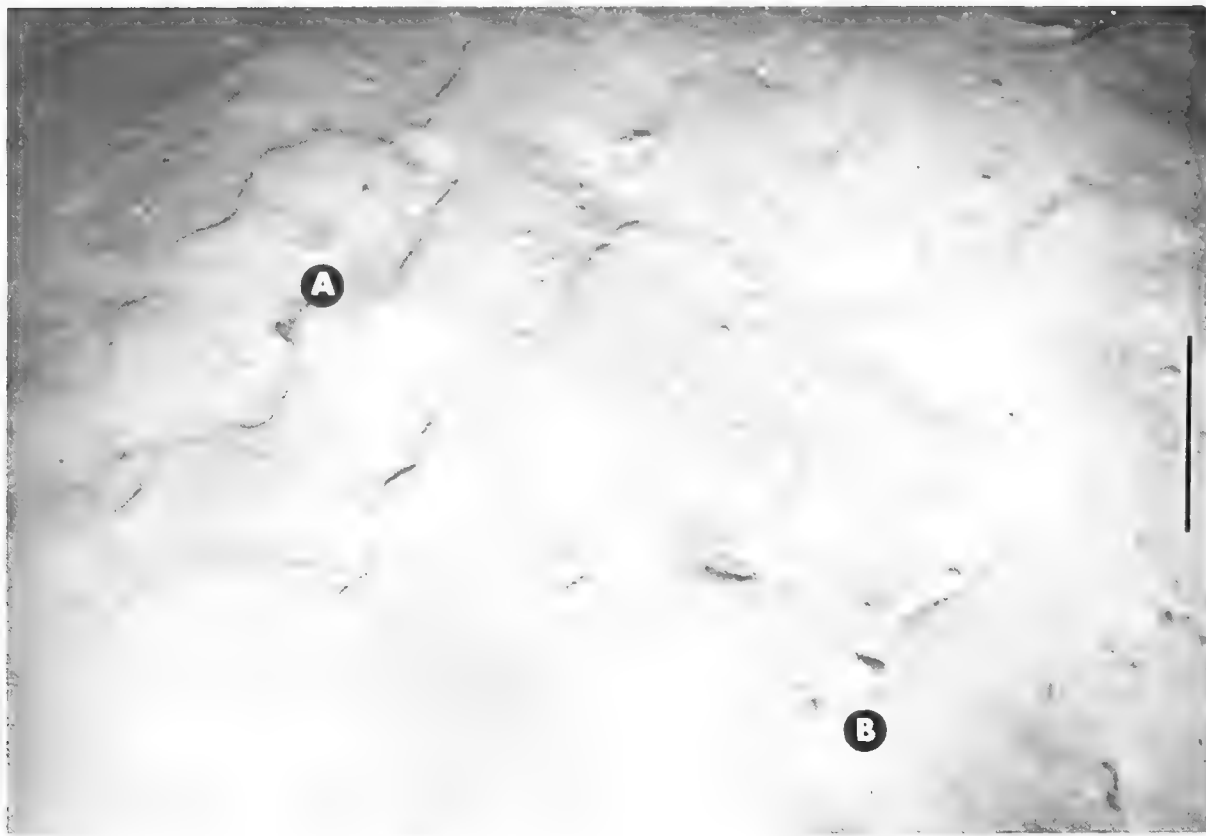
Figure 8.--Asymmetric ripple marks on the sea bottom at station 44. Direction of view is northeast, and the water current that formed the ripples flowed toward the northwest. Identifiable animals: A. burrowing sea anemone; B. hermit crab. Scale bar is 10 cm. long.
