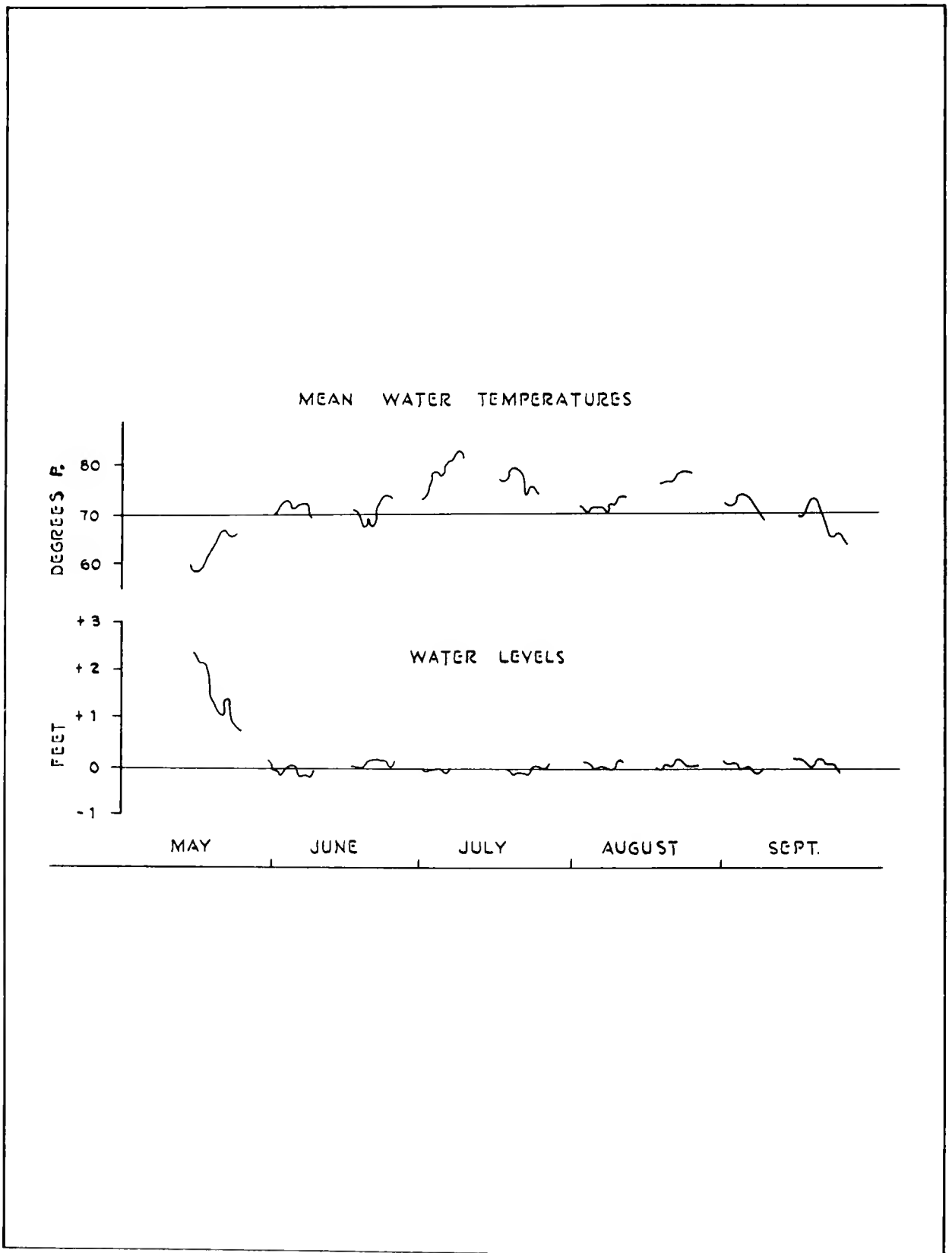
Fig. 5--Fluctuation in water levels and mean water temperature in Pool 8 of the Mississippi River during the summer of 1948. "0" water level in normal pool stage.
