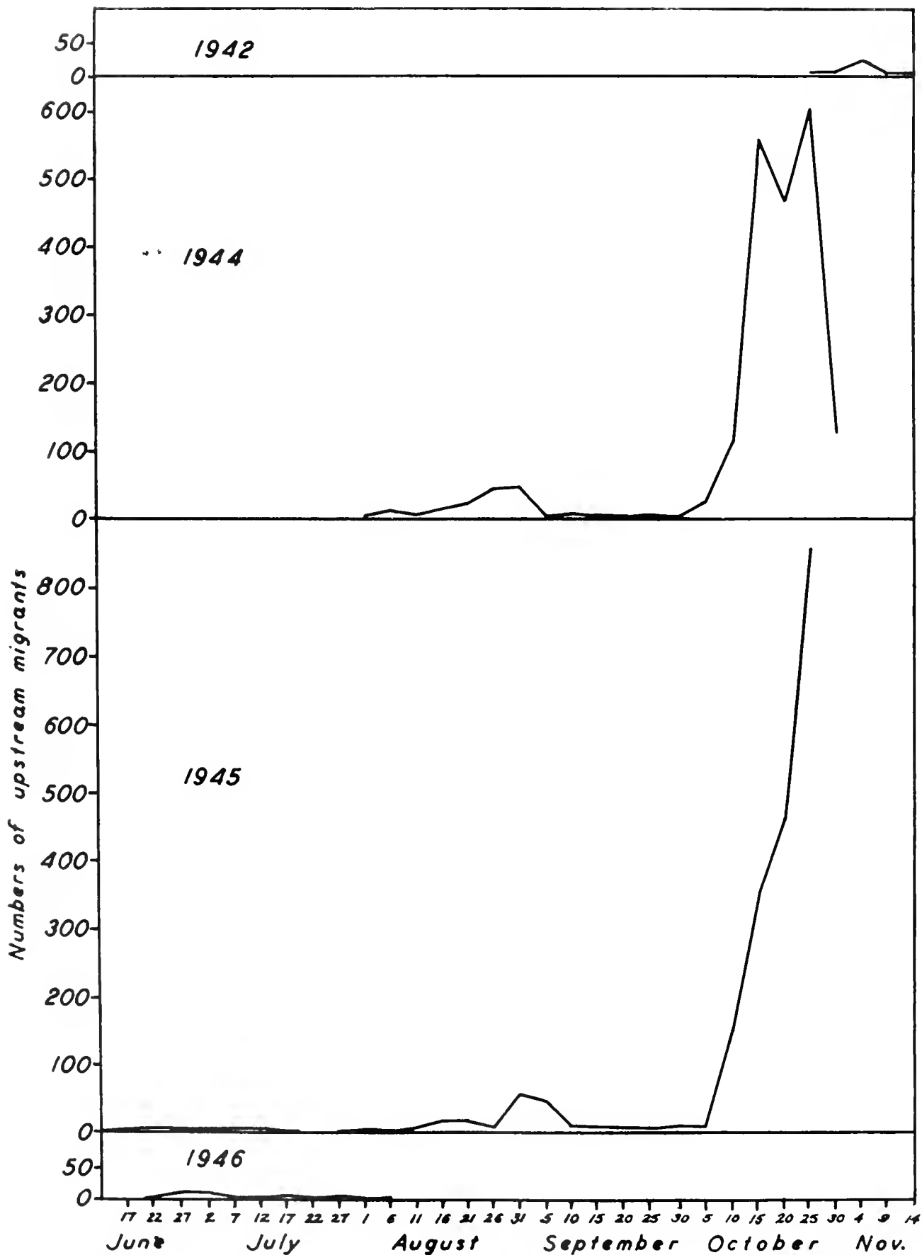
Figure 5. Numbers of adult king salmon passing through the Lewiston weir in 1942, 1944, 1945 and 1946, Trinity River. 24
