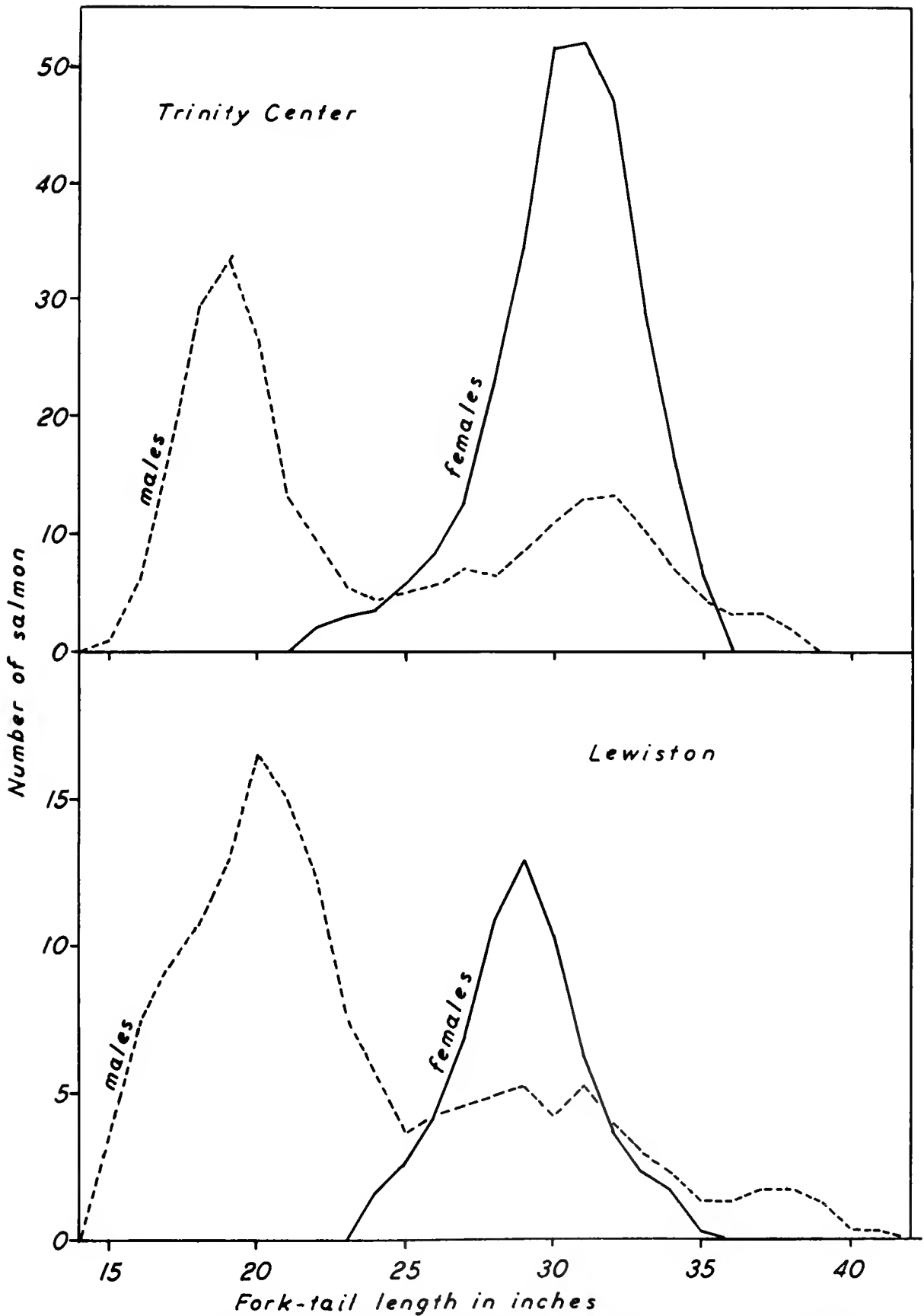
Figure 7. Length-frequency distribution of male and female king salmon from two different sections of Trinity River.
