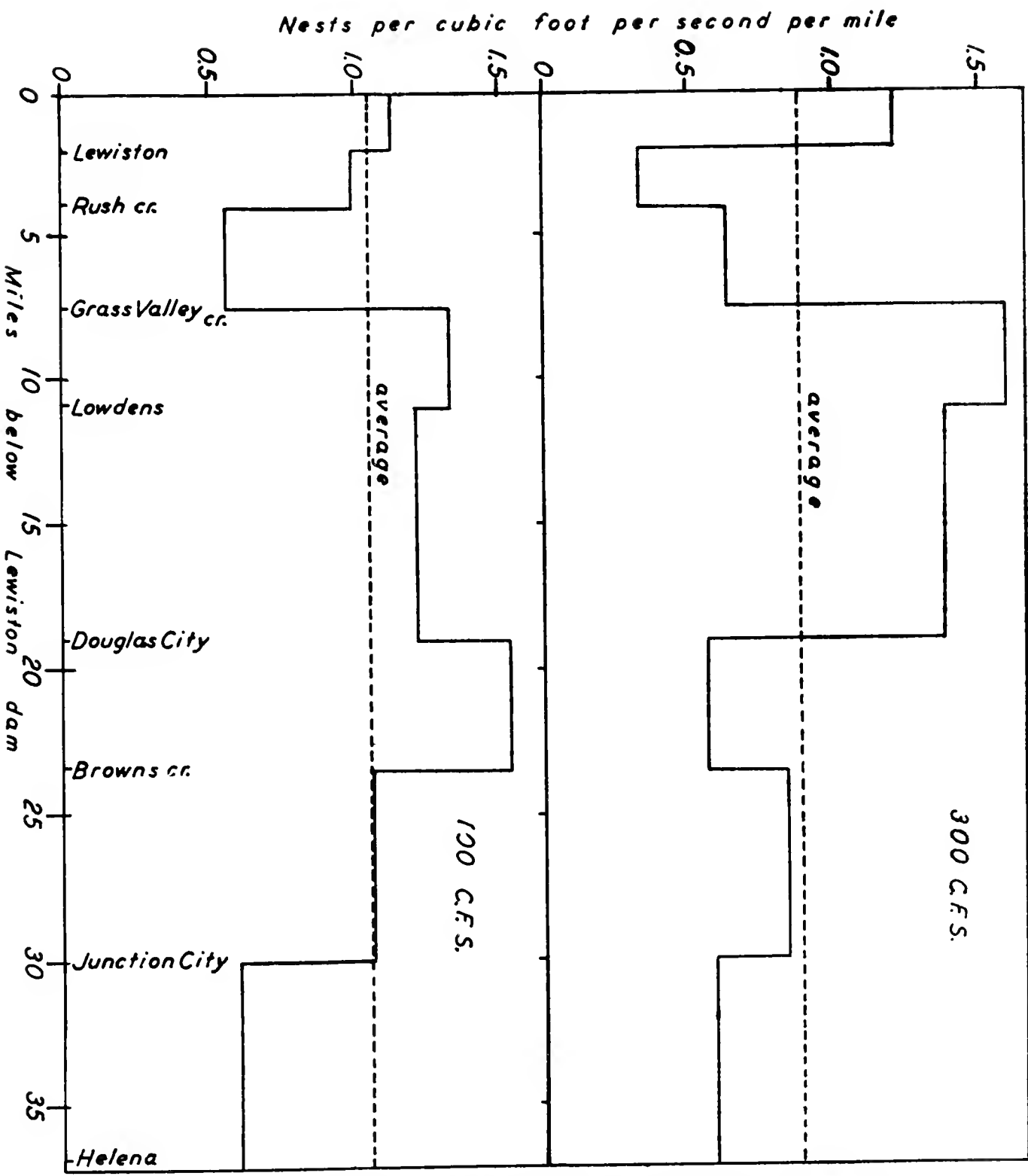
Figure 10. Number of salmon nests in Trinity River between Lewiston and North Fork as determined at two different river flows.
