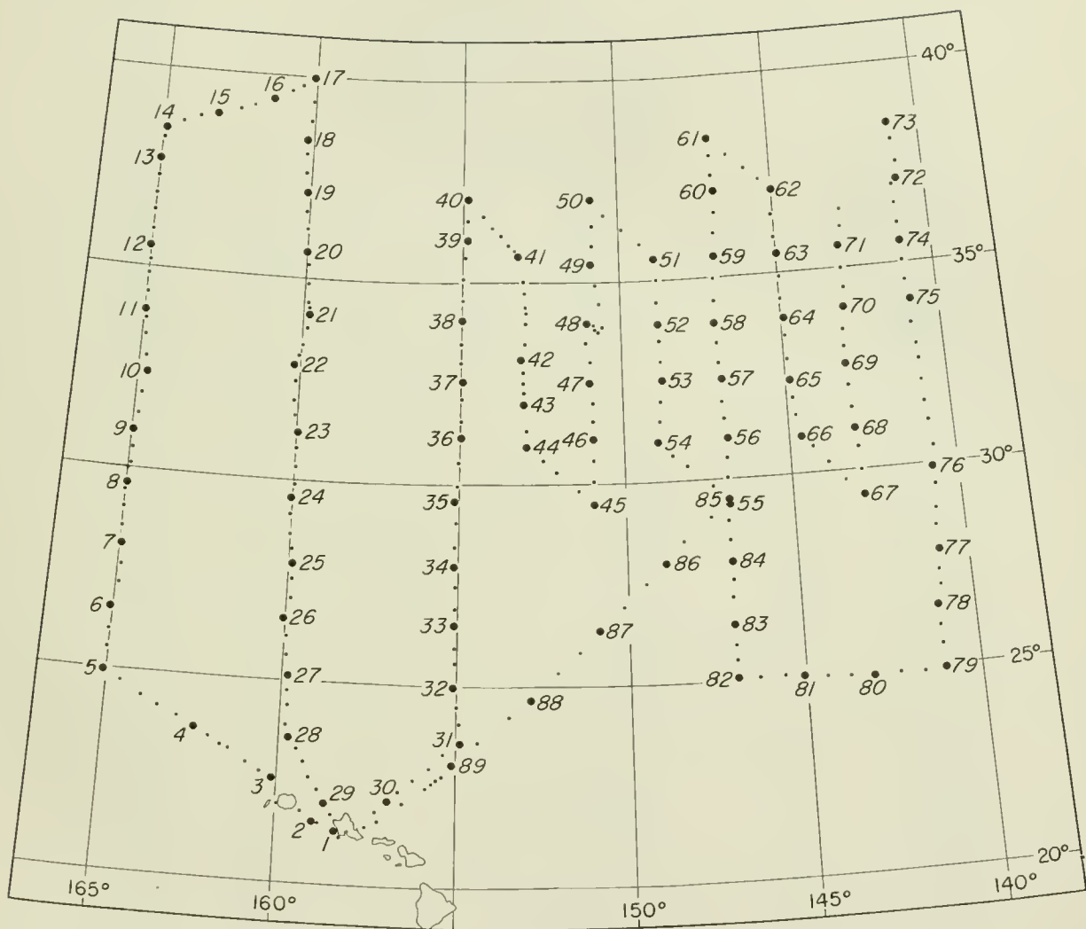
Figure 1.--Oceanographic station positions, Hugh M. Smith cruise 25, January-March 1954. Large numbered dots indicate oceanographic stations. Small dots indicate positions of BT lowerings between stations.
