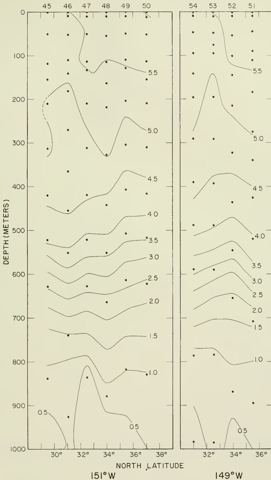
Figure 76.--Vertical section of oxygen in milliliters per liter along 151°W. longitude, stations 45-50. Points indicate observed values. Figure 77.--Same for 149°W. longitude, stations 51-54.
