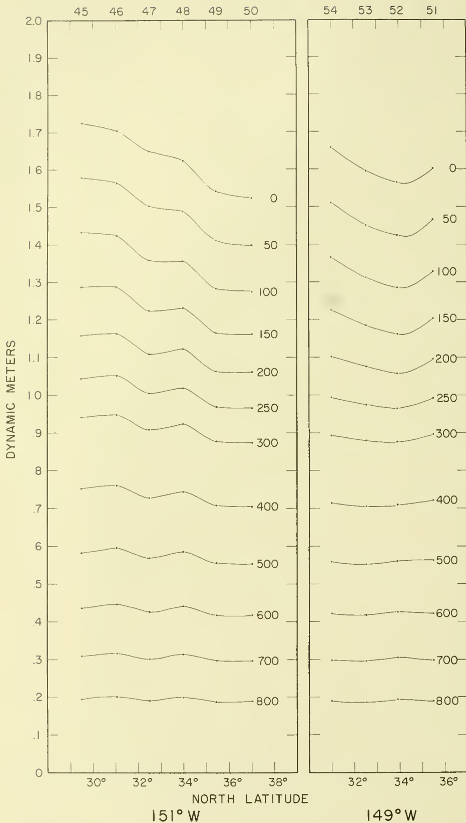
Figure 11.--Smoothed geopotential anomaly of isobaric surfaces relative to the 1,000-db. surface, along 151°W. longitude, stations 45-50. Points represent computed values. Figure 12.--Same for 149°W. longitude, stations 51-54.
