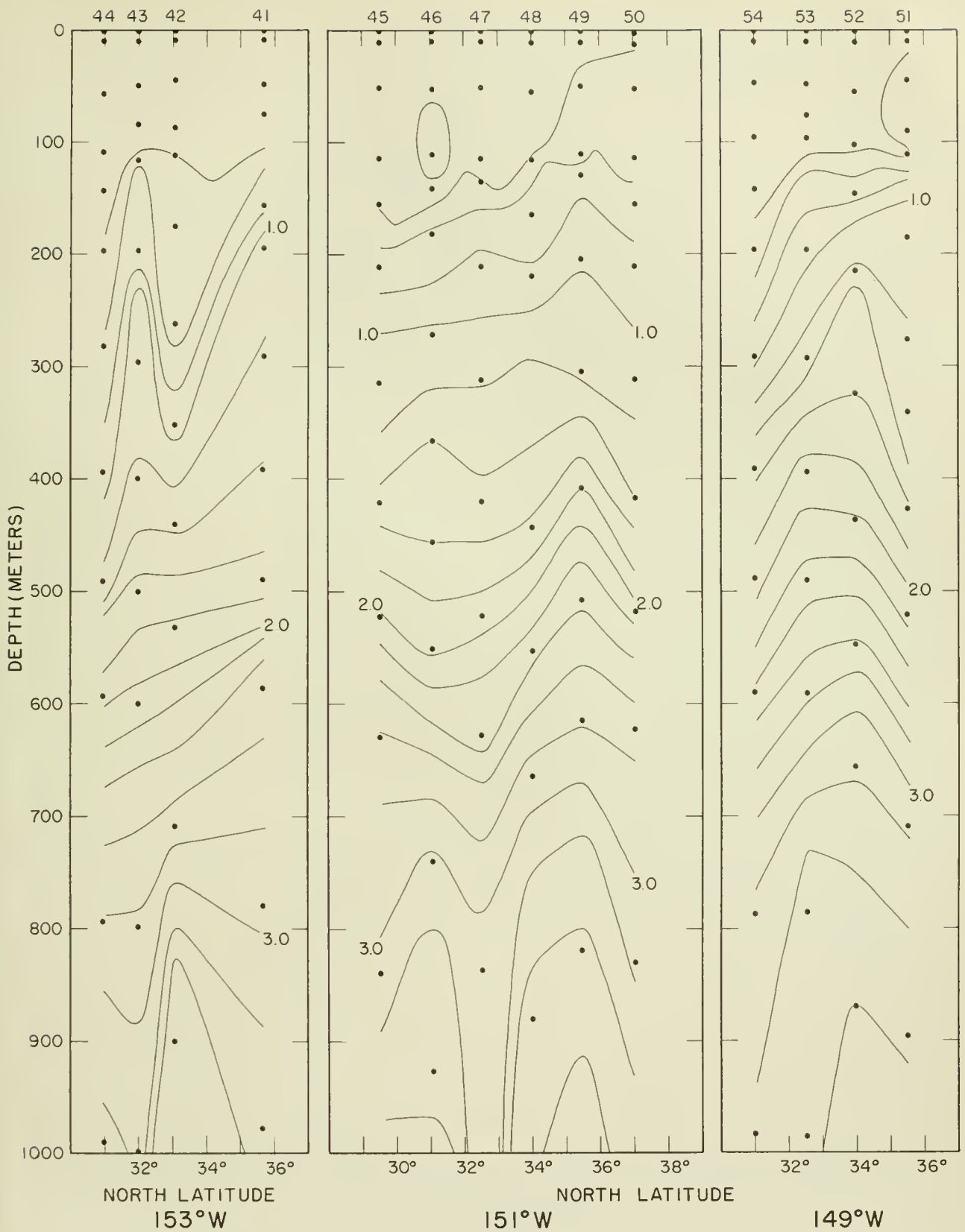
Figure 87.--Vertical section of inorganic phosphate in microgram-atoms per liter along 153°W. longitude, stations 41-44. Points indicate observed values. Figure 88.--Same for 151°W. longitude, stations 45-50. Figure 89.--Same for 149°W. longitude, stations 51-54.
