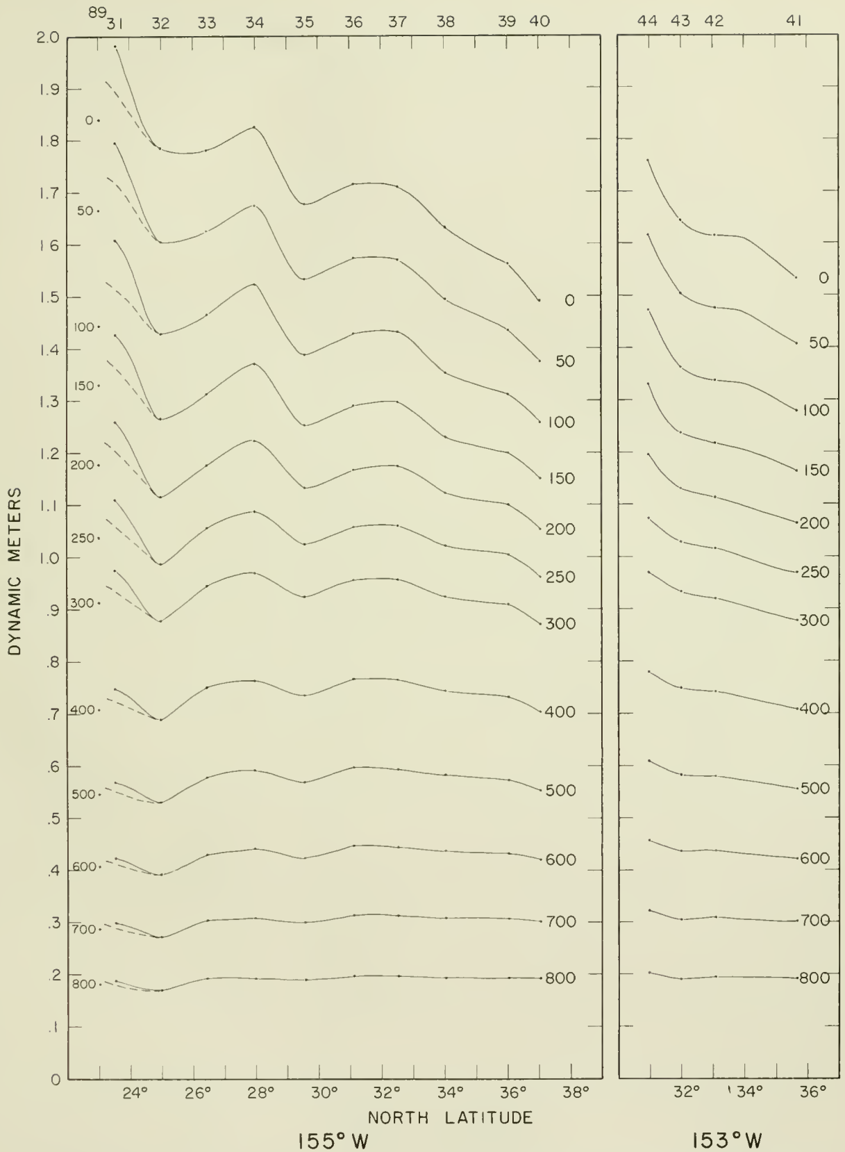
Figure 9. --Smoothed geopotential anomaly of isobaric surfaces relative to the 1,000-db. surface, along 155° W. longitude, stations 31-40. Points represent computed values. Figure 10. --Same for 153° W. longitude, stations 41-44.
