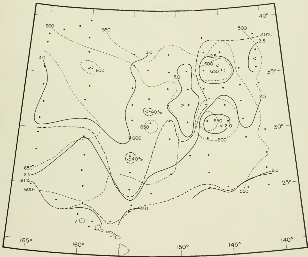
Figure 83.--Oxygen in milliliters per liter (solid lines) and percentage of oxygen saturation (heavy dotted lines) on 26.8 sigma-t surface (depth in meters, light dotted lines). Points indicate station positions.
