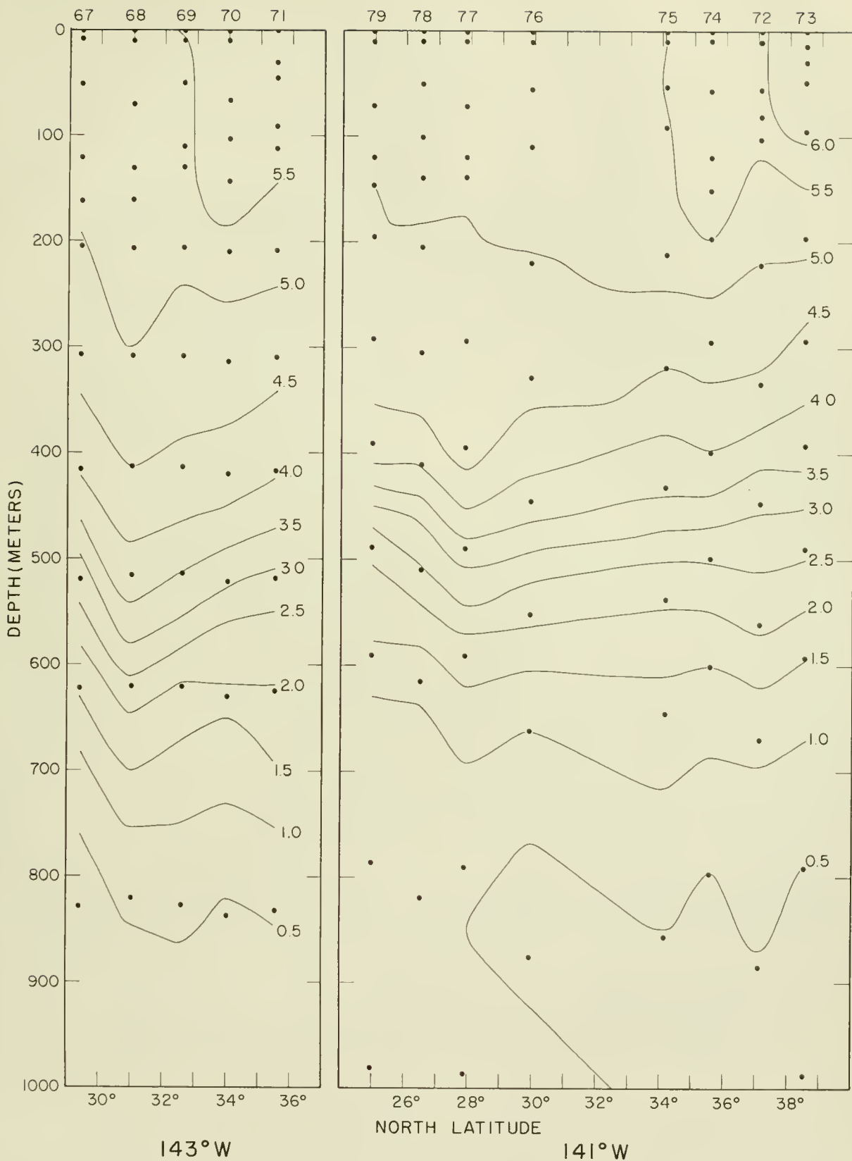
Figure 80.--Vertical section of oxygen in milliliters per liter along 143°W. longitude, stations 67-71. Points indicate observed values. Figure 81.--Same for 141°W. longitude, stations 72-79.
