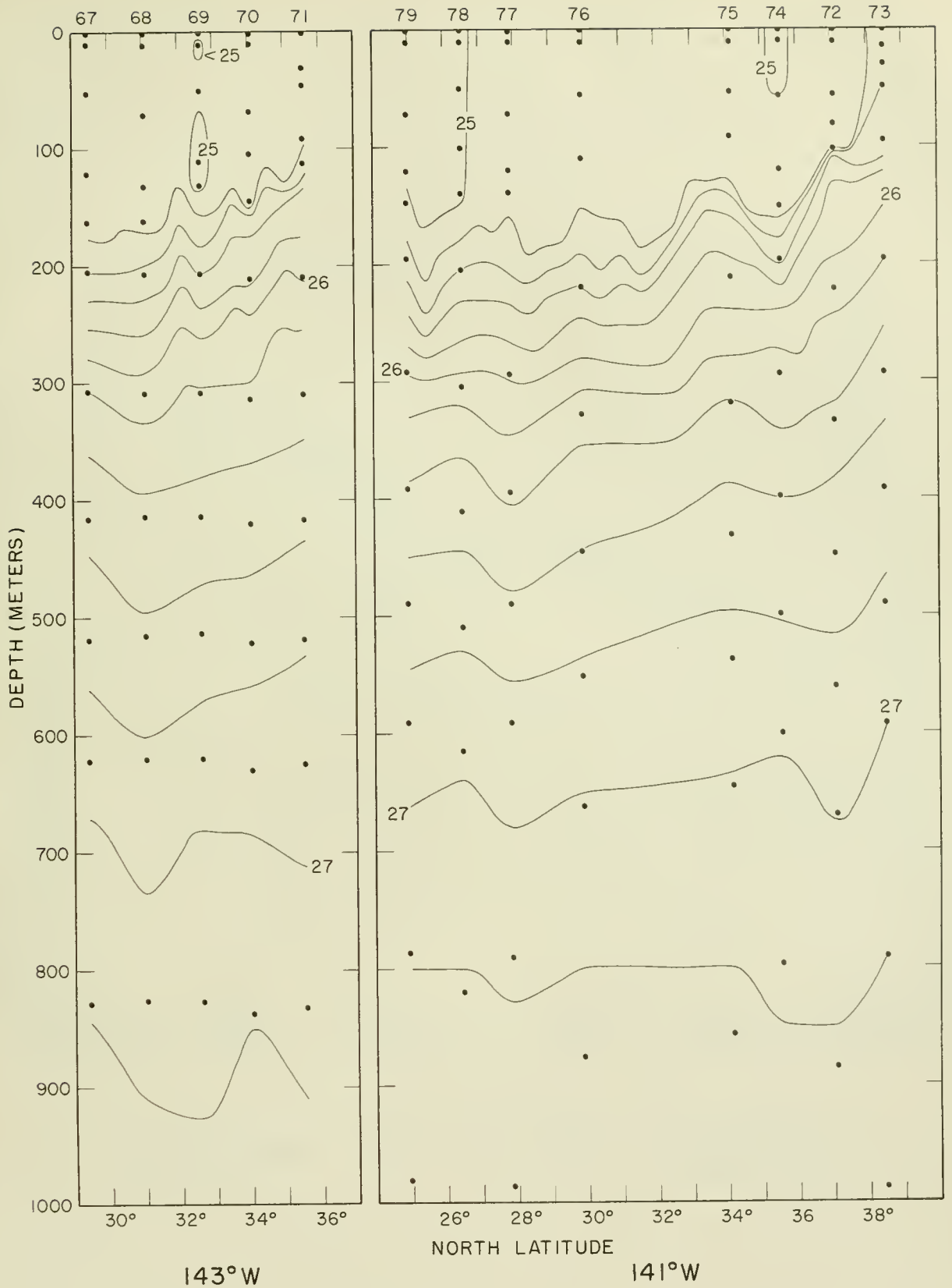
Figure 46.--Vertical section of \sigma_t along 143^\circ\text{W} . longitude, stations 67-71. Points indicate observed values. Figure 47.--Same for 141^\circ\text{W} . longitude, stations 72-79.
