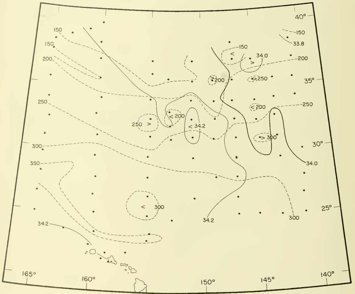
Figure 66.--Salinity in parts per thousand (solid lines) on the 26.0 sigma-t surface (depth in meters, dotted lines). Points indicate station positions.
