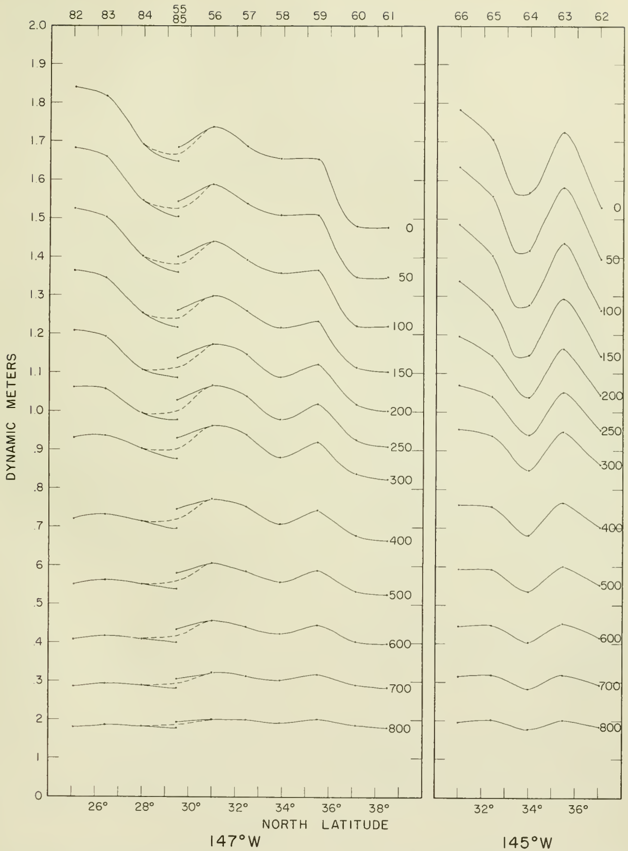
Figure 13.--Smoothed geopotential anomaly of isobaric surfaces relative to the 1,000-db. surface along 147°W. longitude, stations 55-61 and 82-85. Points represent computed values. Figure 14.--Same for 145°W. longitude, stations 62-66.
