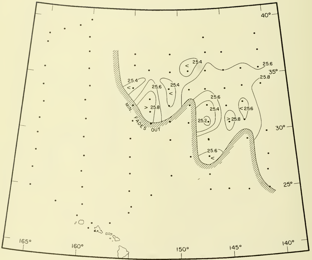
Figure 64.--Sigma-t at the shallow salinity minimum. Points indicate station positions.
