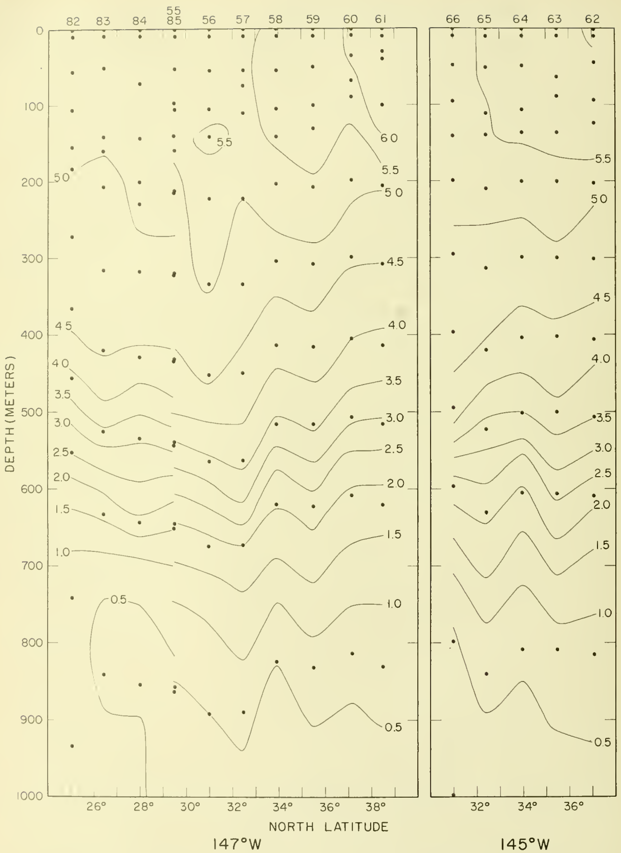
Figure 78. --Vertical section of oxygen in milliliters per liter along 147°W. longitude, stations 55-61 and 82-85. Points indicate observed values. Figure 79. --Same for 145°W. longitude, stations 62-66.
