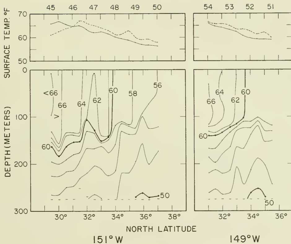
Figure 28.--Temperature sections from BT casts along 151°W. longitude, stations 45-50. Upper panel air (dotted) and surface (solid) temperatures. Lower panel temperatures from BT slides. Dashes indicate depth of casts.
