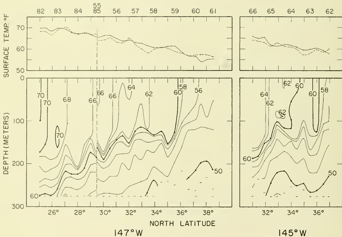
Figure 30.--Temperature sections from BT casts along 147^{\circ}\text{W} . longitude, stations 55-61 and 82-85. Upper panel air (dotted) and surface (solid) temperatures. Lower panel temperature from BT slides. Dashes indicate depth of casts.
