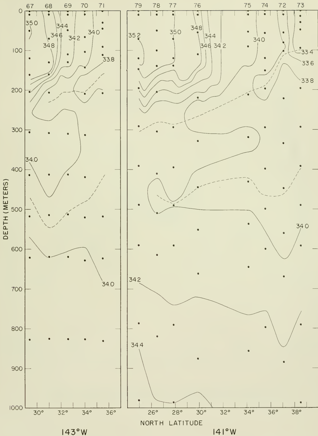
Figure 60.--Vertical section of salinity in parts per thousand along 143°W. longitude, stations 67-71. Dotted lines indicate depths of salinity minima. Points indicate observed values. Figure 61.--Same for 141°W. longitude, stations 72-79.
