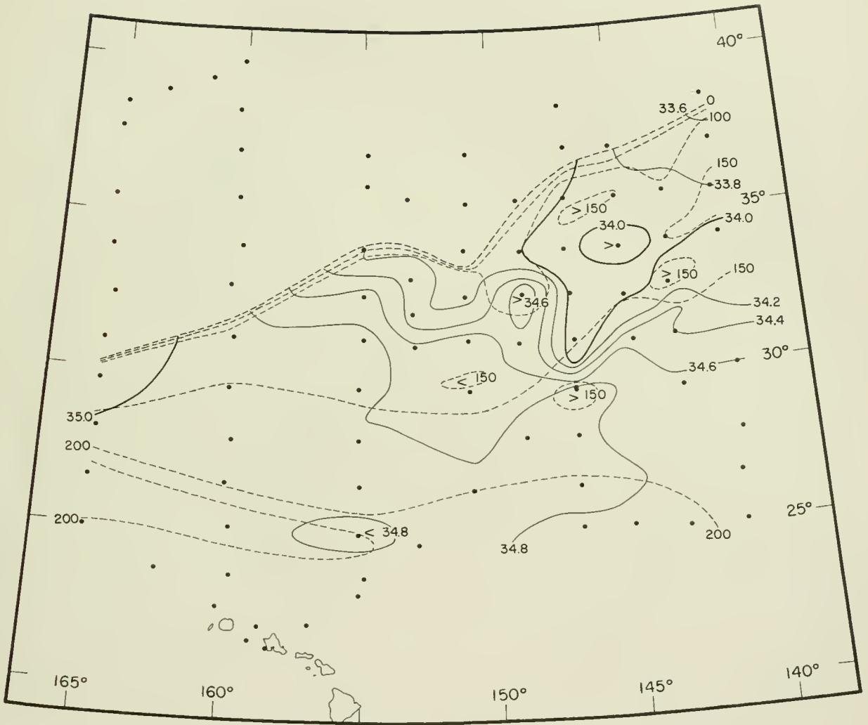
Figure 65.--Salinity in parts per thousand (solid lines) on the 25.2 sigma-t surface (depth in meters, dotted lines). Points indicate station positions.
