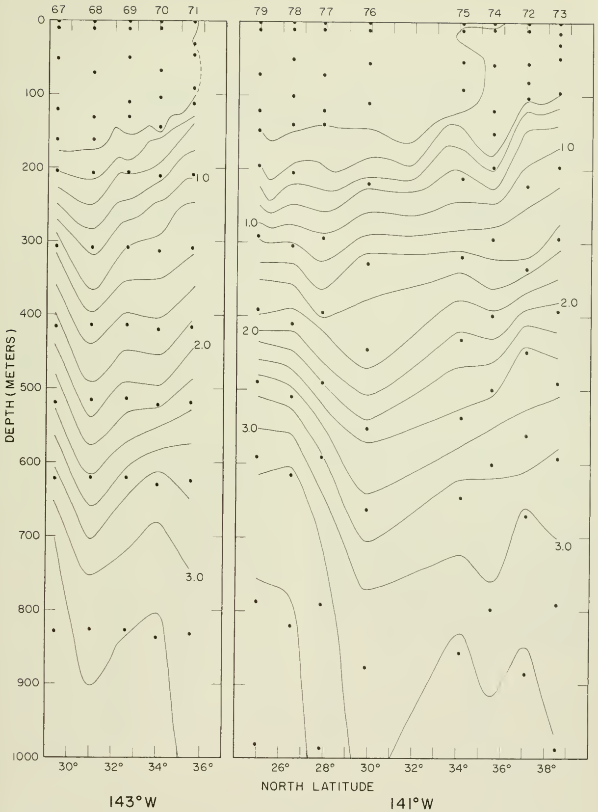
Figure 92. --Vertical section of inorganic phosphate in microgram-atoms per liter along 143^{\circ} W. longitude, stations 67-71. Points indicate observed values. Figure 93. --Same for 141^{\circ} W. longitude, stations 72-79.
