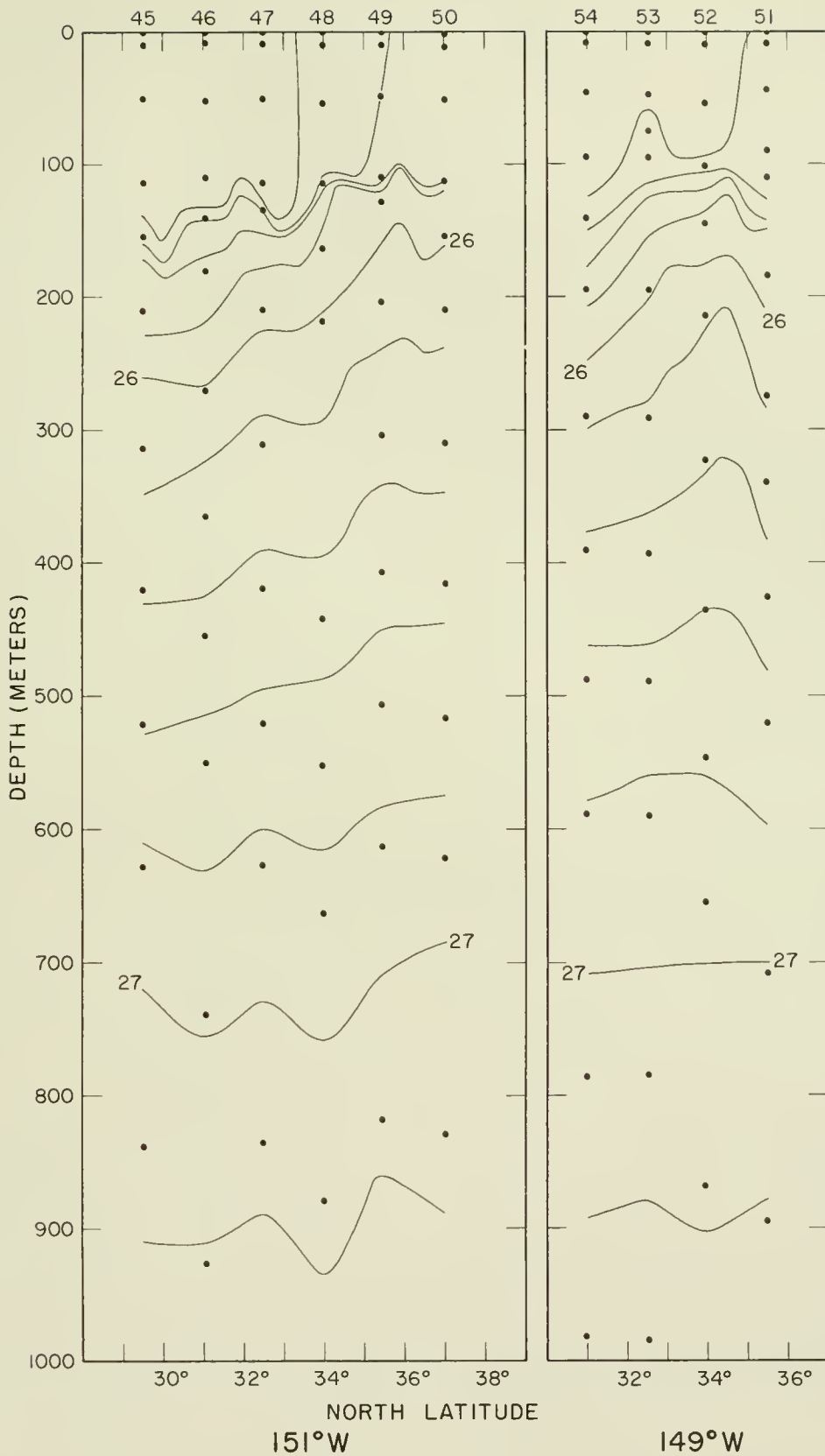
Figure 42.--Vertical section of sigma-t along 151°W. longitude, stations 45-50. Points indicate observed values. Figure 43.--Same for 149°W. longitude, stations 51-54.
