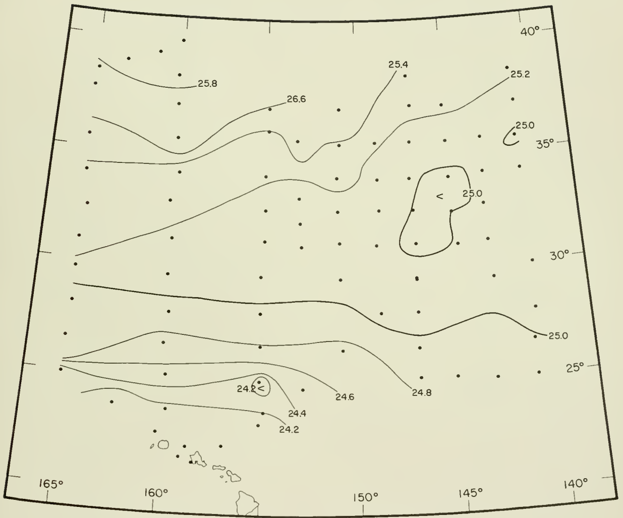
Figure 37.--Surface sigma-t. Points indicate station positions.
