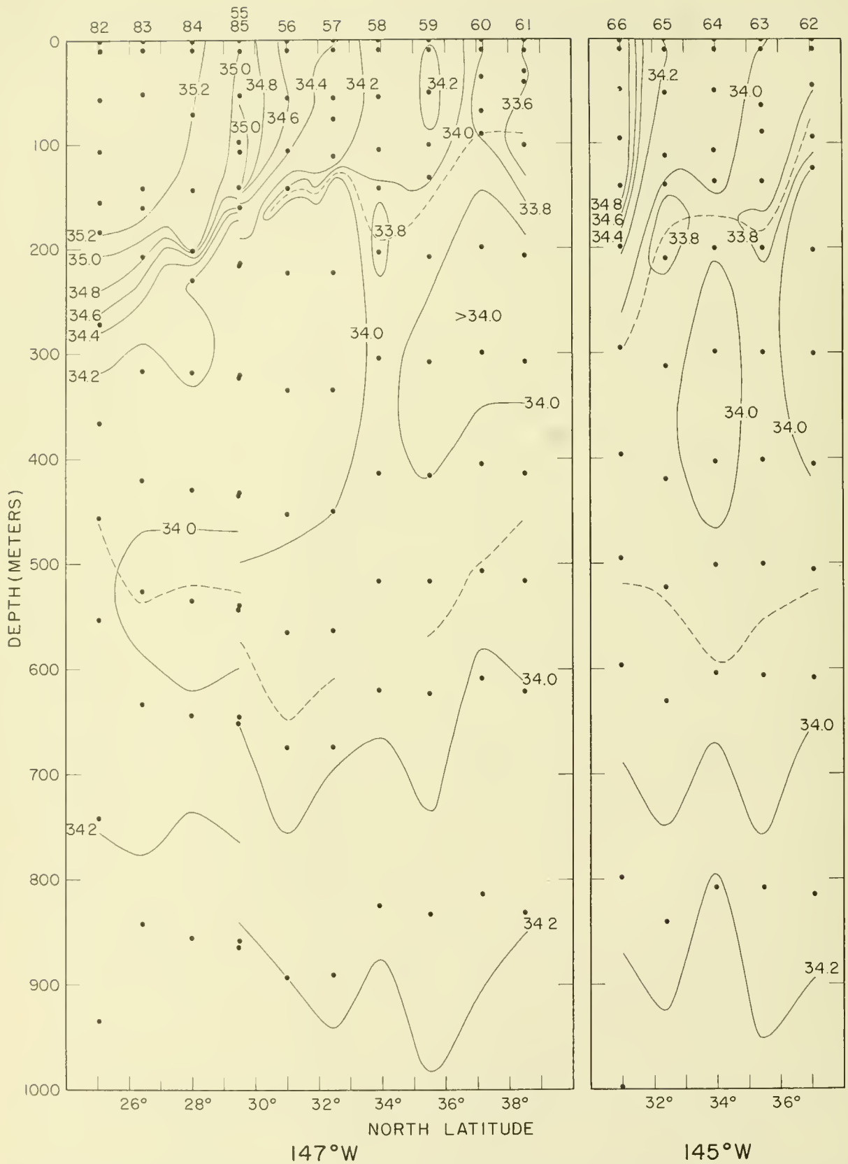
Figure 58.--Vertical section of salinity in parts per thousand along 147°W. longitude, stations 55-61 and 82-85. Dotted lines indicate depths of salinity minima. Points indicate observed values. Figure 59.--Same for 145°W. longitude, stations 62-66.
