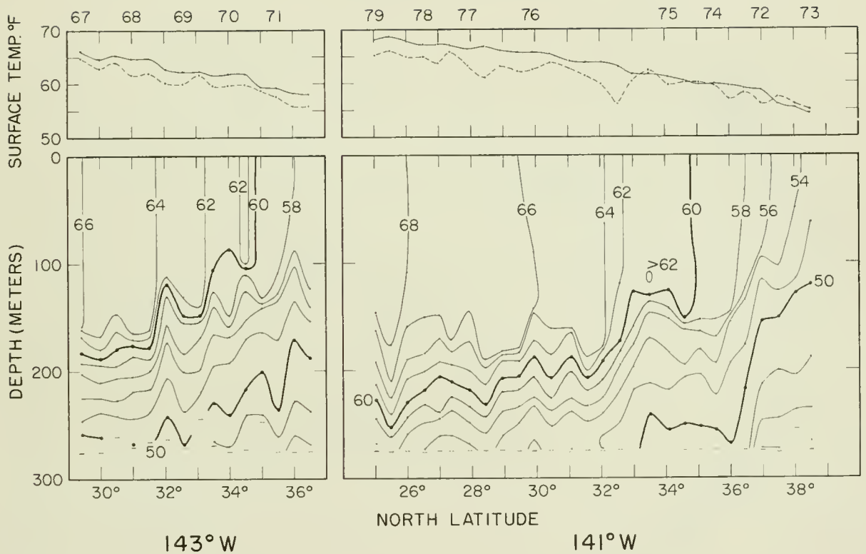
Figure 32.--Temperature sections from BT casts along 143°W. longitude, stations 67-71.
