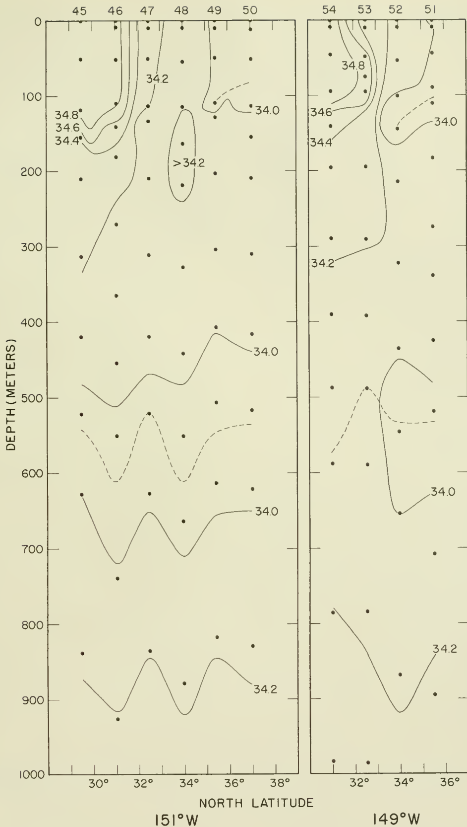
Figure 56. --Vertical section of salinity in parts per thousand along 151°W. longitude, stations 45-50. Dotted lines indicate depths of salinity minima. Points indicate observed values. Figure 57. --Same for 149°W. longitude, stations 51-54.
