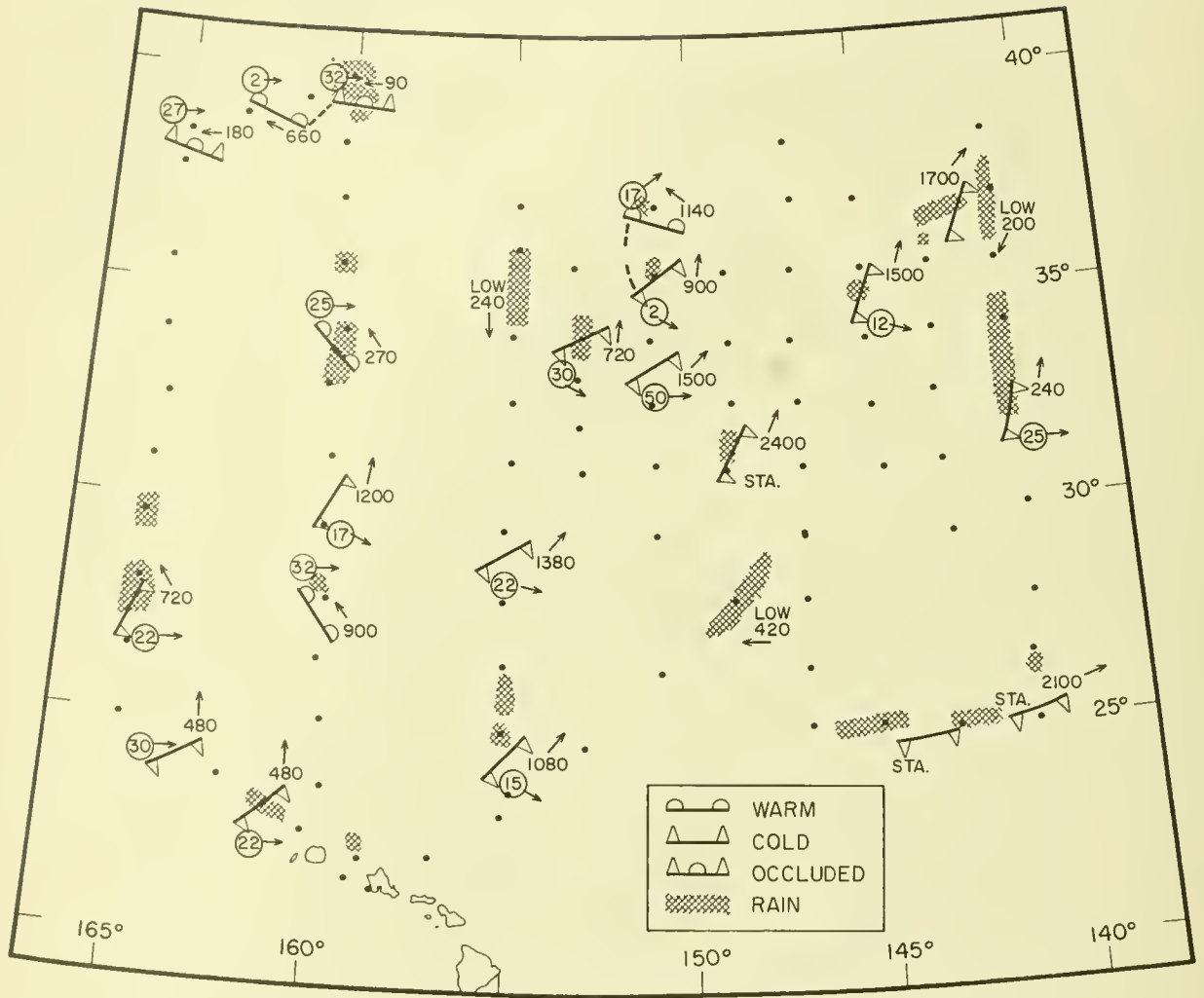
Figure 6. --Location, type, and motion of frontal systems passing over vessel and areas of observed precipitation. Larger values and adjacent arrows indicate the distance (mi.) and direction to the center of the low; the smaller encircled values and adjacent arrows indicate the direction and speed (knots) of the frontal movement. Points indicate station positions. Abbreviations: sta. - stationary, dis. - dispersing.
