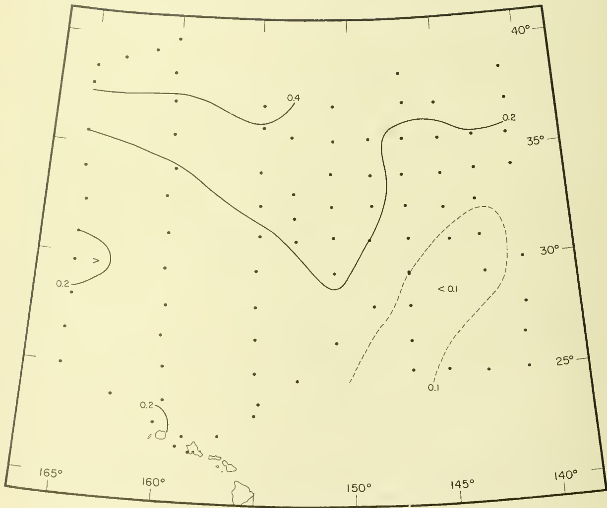
Figure 84.--Surface inorganic phosphate distribution in microgram-atoms per liter. Points indicate observed values.
