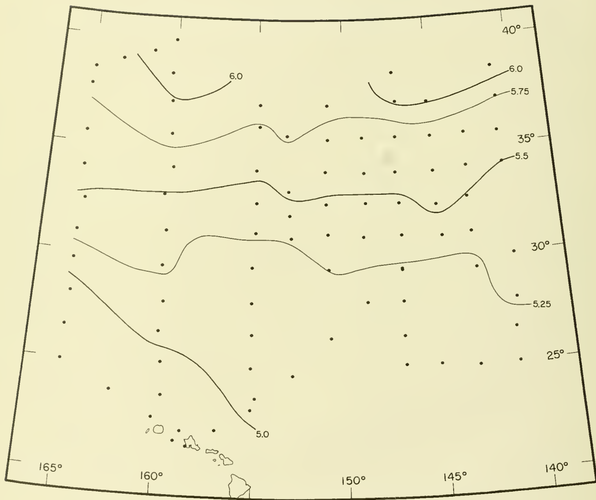
Figure 82. --Oxygen at 10 meters in milliliters per liter. Points indicate observed values.
