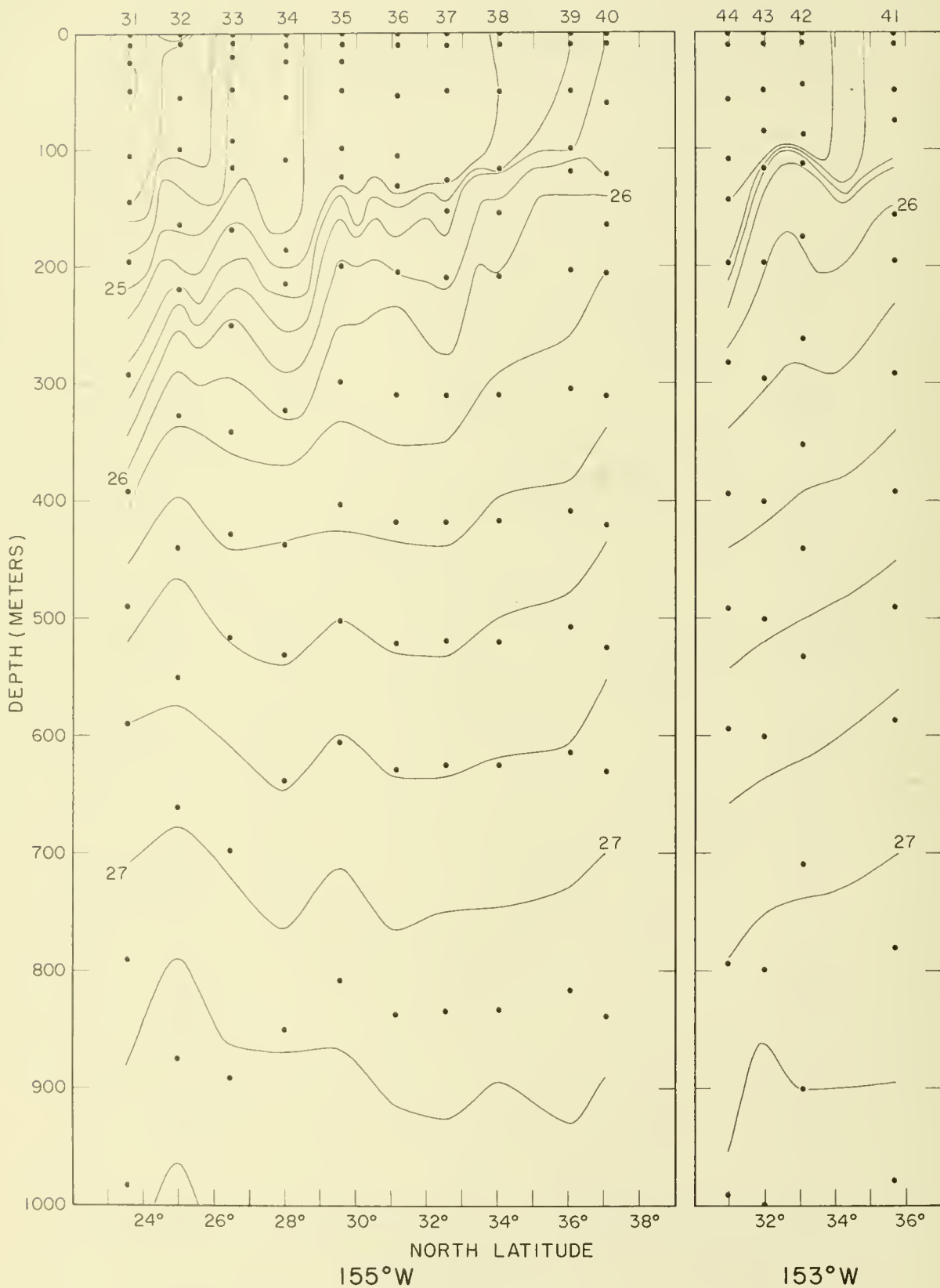
Figure 40. --Vertical section of sigma-t along 155°W. longitude, stations 31-40. Points indicate observed values. Figure 41. --Same for 153°W. longitude, stations 41-44.
