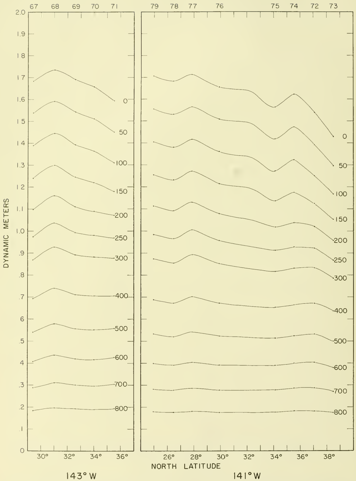
Figure 15.--Smoothed geopotential anomaly of isobaric surfaces relative to the 1,000-db. surface along 143°W. longitude, stations 67-71. Points represent computed values. Figure 16.--Same for 141°W. longitude, stations 72-79.
