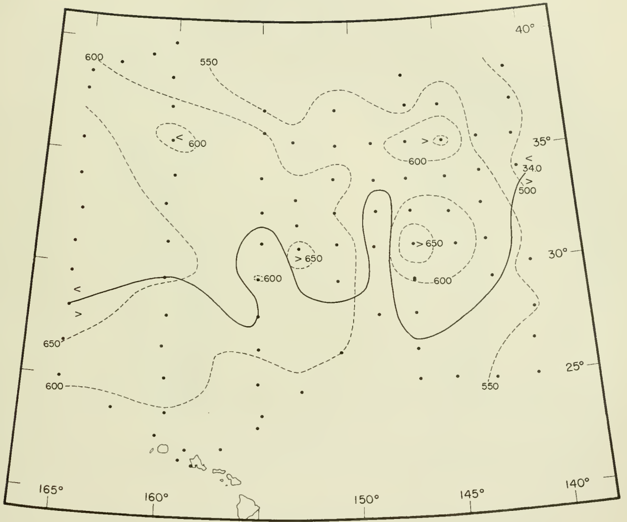
Figure 67. --Salinity in parts per thousand (solid lines) on the 26.8 sigma-t surface (depth in meters, dotted lines). Points indicate station positions.
