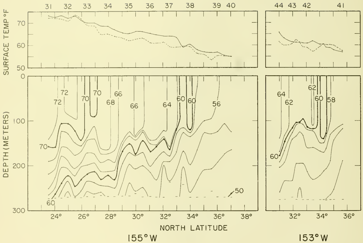
Figure 26.--Temperature sections from BT casts along 155°W. longitude, stations 31-40. Upper panel air (dotted) and surface (solid) temperatures. Lower panel temperatures from BT slides. Dashes indicate depth of casts.
