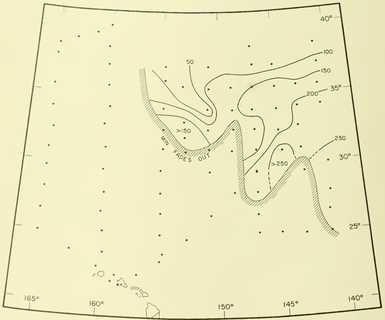
Figure 62. --Depth in meters of the shallow salinity minimum. Points indicate station positions.
