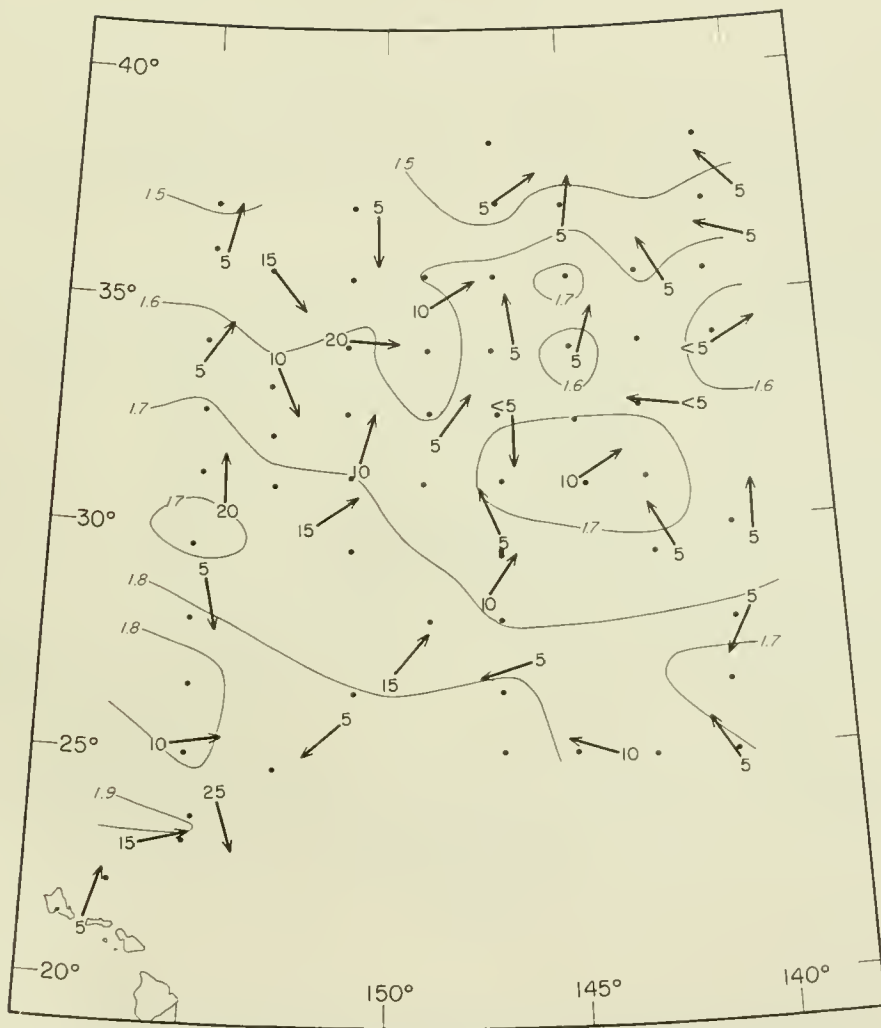
Figure 23.--Currents by Geomagnetic Electrokinetograph. Arrows show the direction of the current; speed is given to the nearest 5 cm./sec. Values averaged by calendar day. Contours show surface dynamic topography (see fig. 17). Points indicate station positions.
