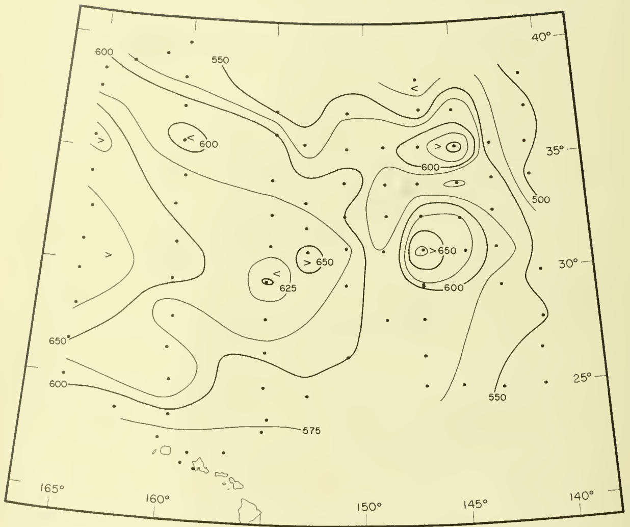
Figure 50. --Depth of 26.8 sigma-t surface in meters. Points indicate station positions.
