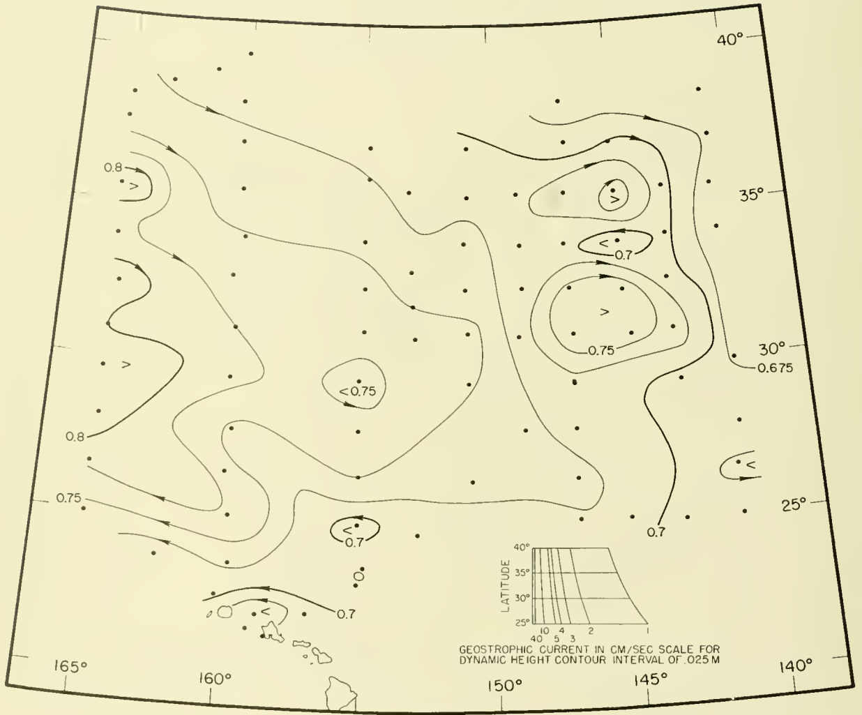
Figure 20.--Anomaly of geopotential topography of the 400-db. surface relative to the 1,000-db. surface. Points indicate computed values.
