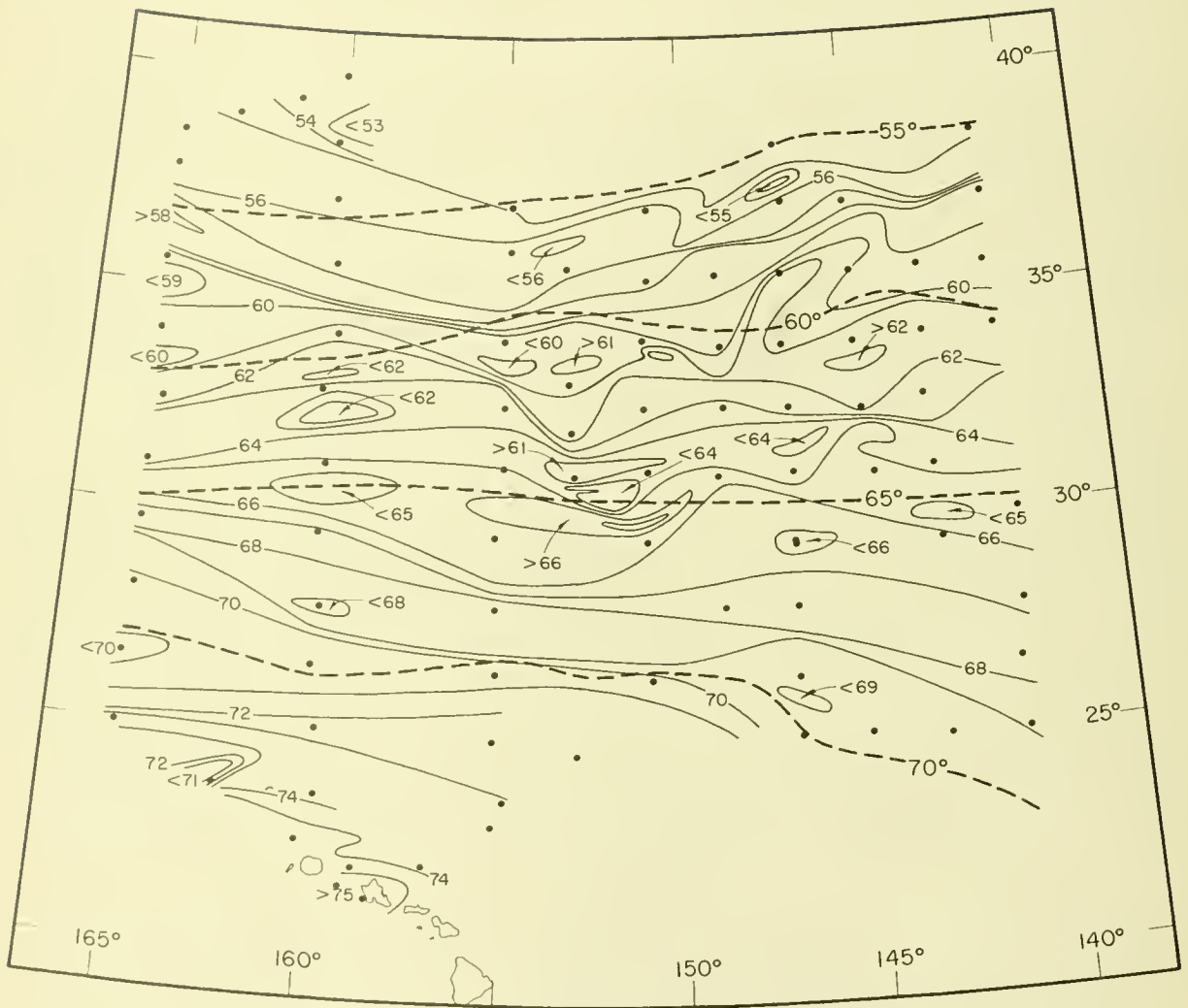
Figure 34. --Surface (bucket) temperatures in ^{\circ}\text{F} . (solid) and mean positions of selected isotherms (dotted). Points indicate station positions.
