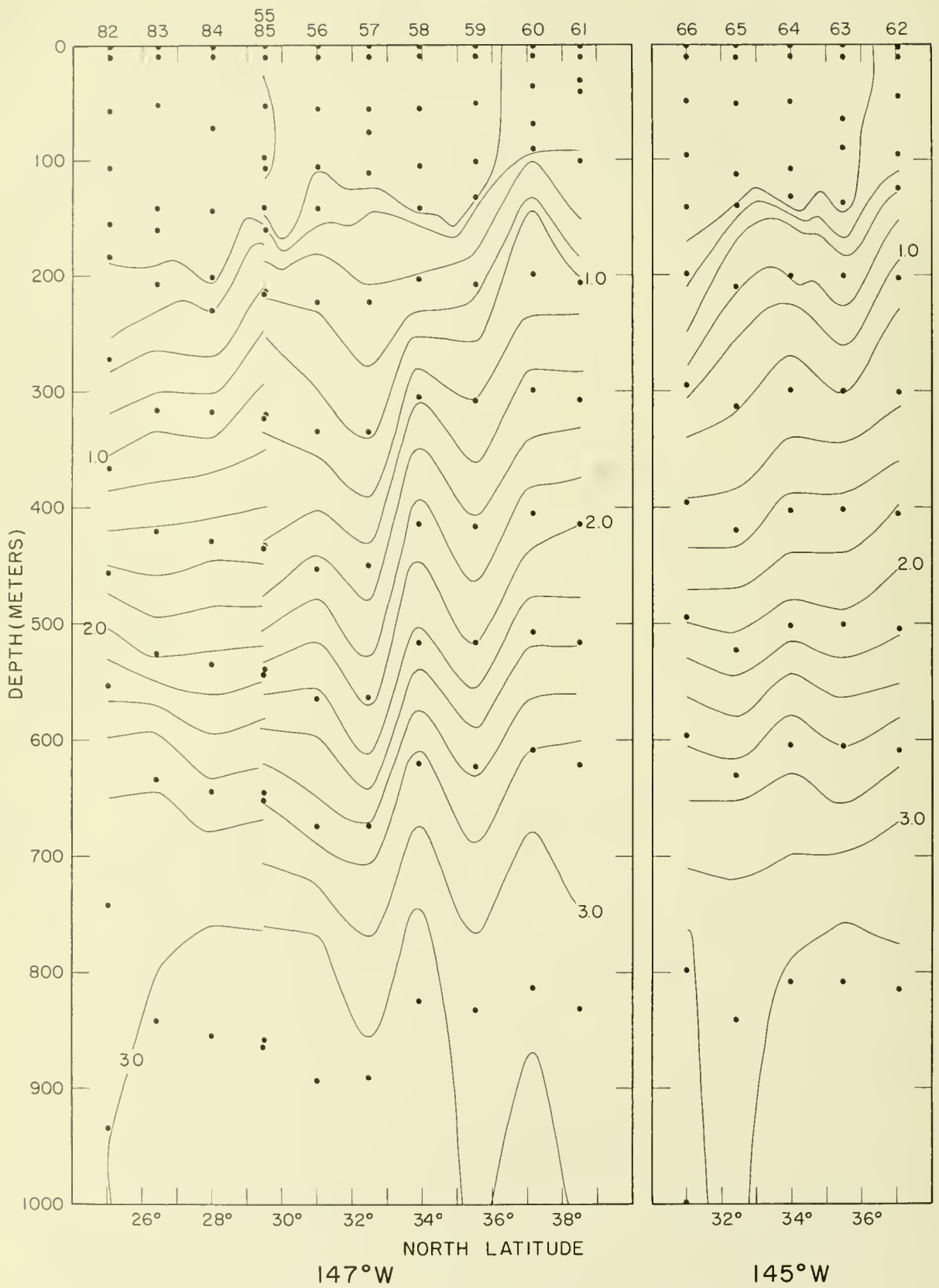
Figure 90.--Vertical section of inorganic phosphate in microgram-atoms per liter along 147°W. longitude, stations 55-61 and 82-85. Points indicate observed values. Figure 91.--Same for 145°W. longitude, stations 62-66.
