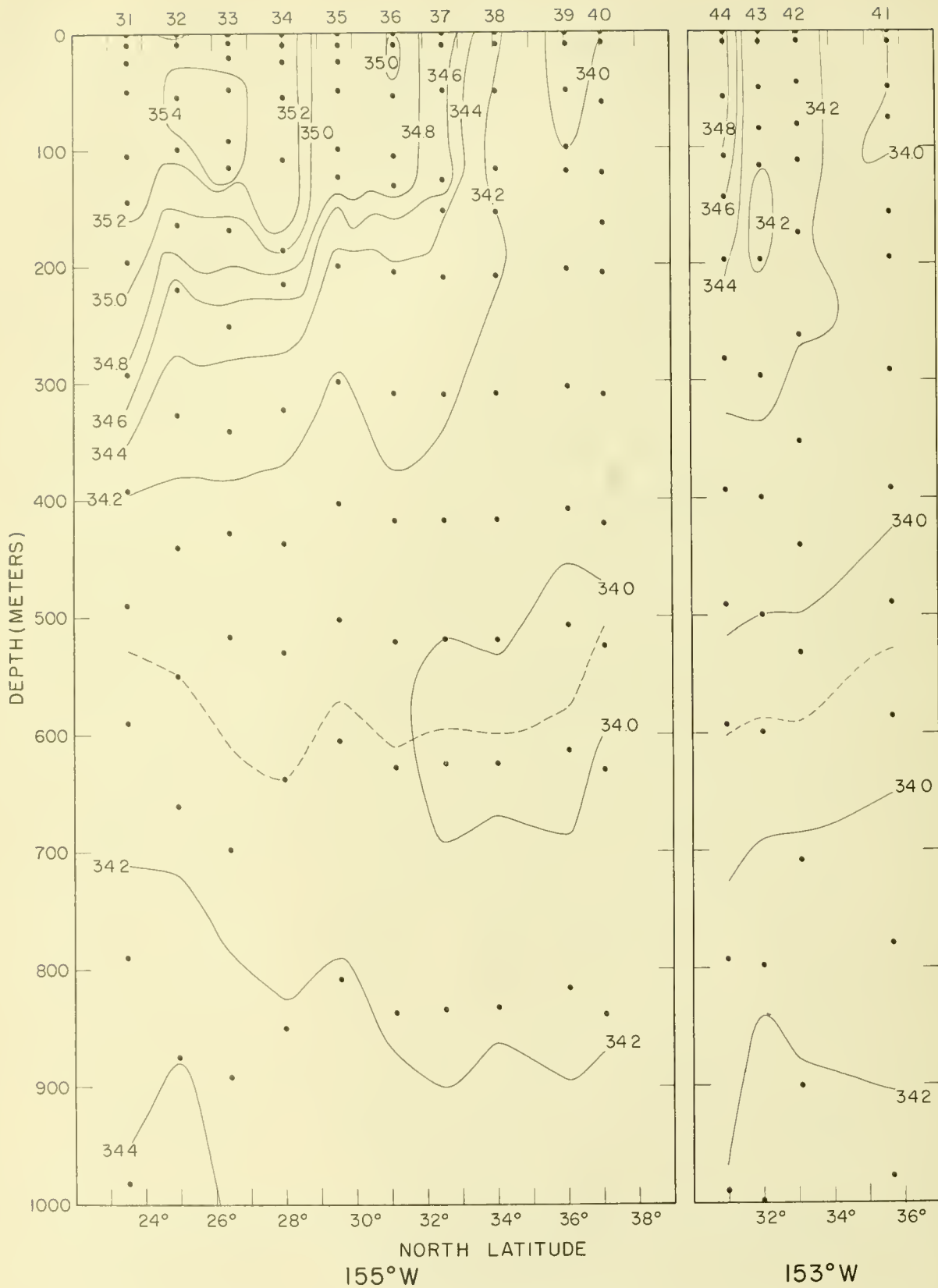
Figure 54. --Vertical section of salinity in parts per thousand along 155°W. longitude, stations 31-40. Dotted line indicates depth of salinity minima. Points indicate observed values. Figure 55. --Same for 153°W. longitude, stations 41-44.
