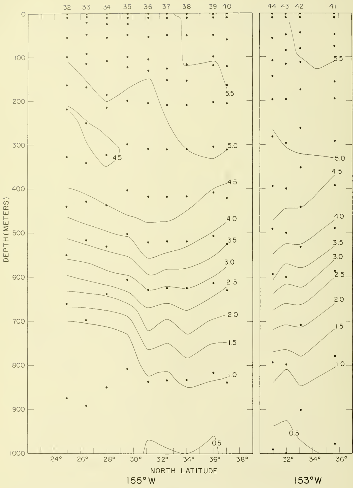
Figure 74. --Vertical section of oxygen in milliliters per liter along 155°W. longitude, stations 32-40. Points indicate observed values. Figure 75. --Same for 153°W. longitude, stations 41-44.
