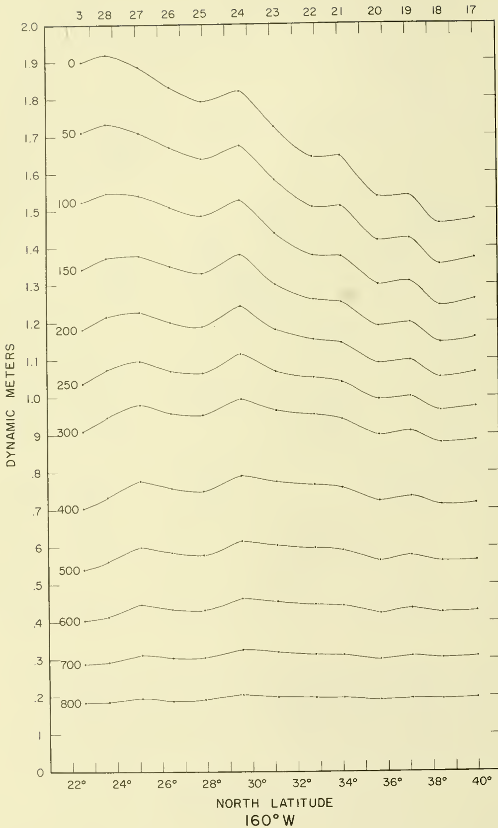
Figure 8. --Smoothed geopotential anomaly of isobaric surfaces relative to the 1,000-db. surface, 160°W. longitude, stations 17-28. Points represent computed values.
