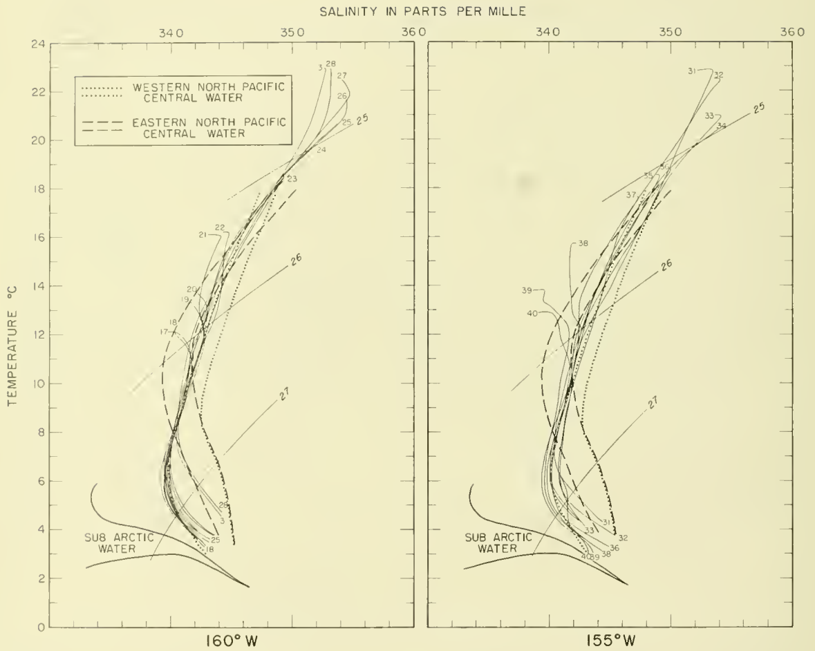
Figure 68.--Superimposed temperature-salinity curves for the meridional station series along 160°W. longitude, stations 17-28.
