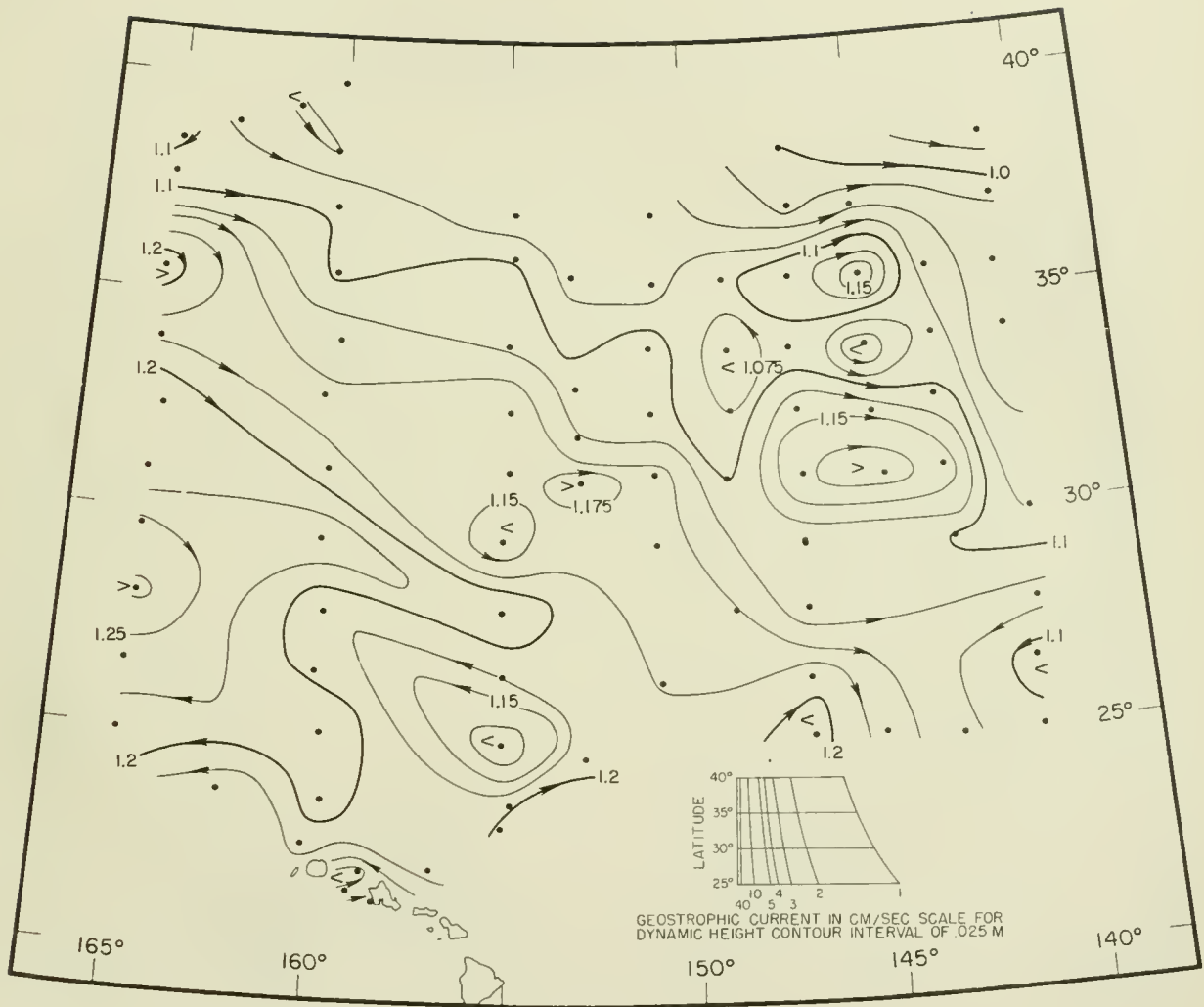
Figure 19.--Anomaly of geopotential topography of the 200-db. surface relative to the 1,000-db. surface. Points indicate computed values.
